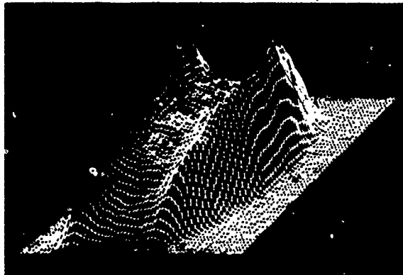
Sample intensity distribution of an x-ray tube focal spot scanned with microdensitometer-computer system. Scan shows lack of uniformity of focal spot intensity, which can contribute to poor quality x-ray film.
