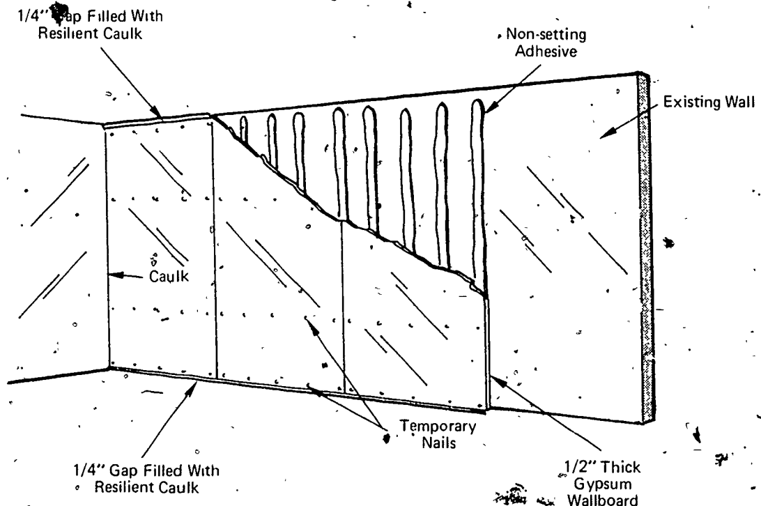
Fig. 4-13. IMPROVING THE SOUND INSULATION OF AN EXISTING WALL
