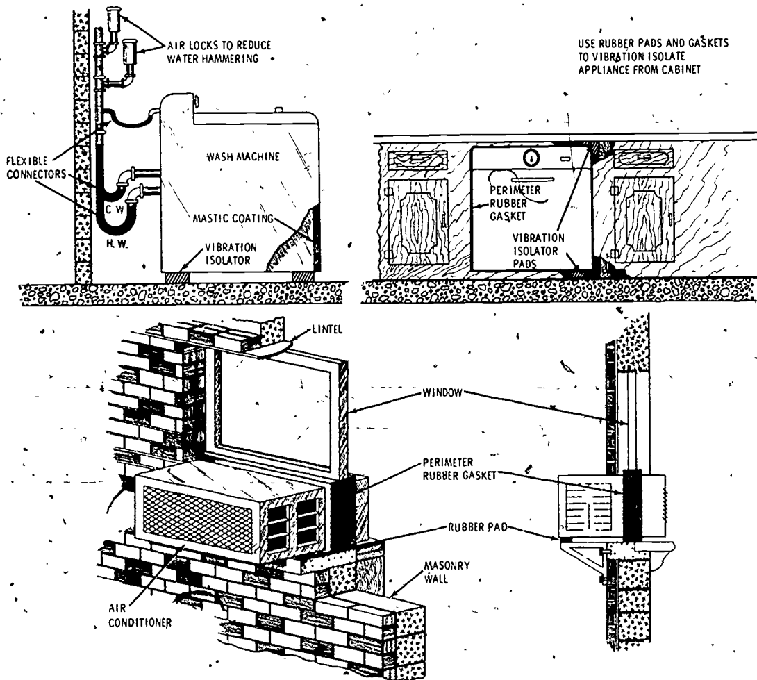
Fig. 4-10. PROPER INSTALLATION OF APPLIANCES FOR QUIET OPERATION
