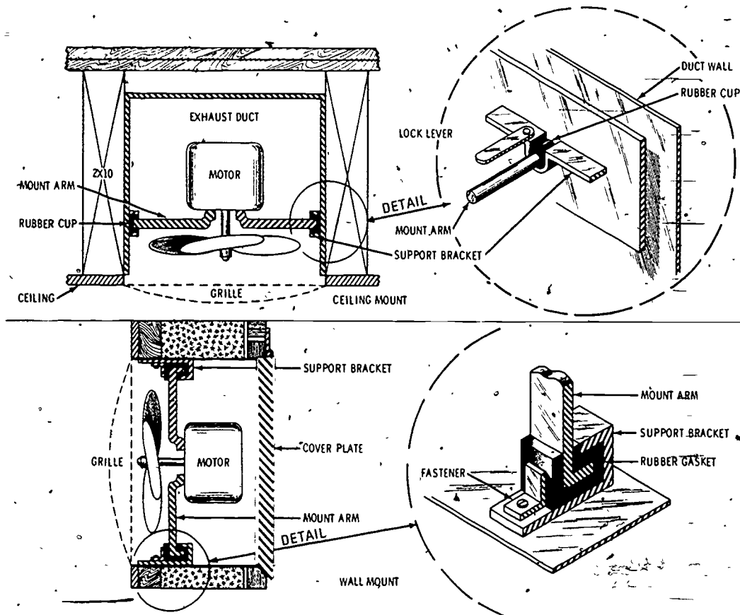
Fig. 4-9. PROPER INSTALLATION OF AN EXHAUST FAN
