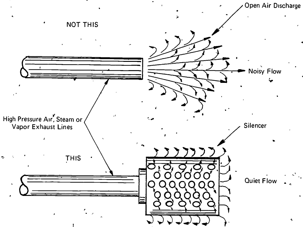
Fig. 3-17. SILENCER FOR HIGH PRESSURE EXHAUST LINE
