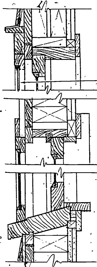
Fig. 5-1. DETAILS OF A DOUBLE-HUNG WINDOW WITH A STORM SASH
