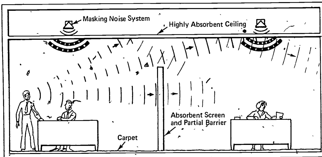
Fig. 8-3. FACTORS CONTROLLING SPEECH PRIVACY IN OPEN-PLAN OFFICES: ACOUSTICAL CEILING, SCREEN AND CARPET MINIMIZE SOUND REFLECTION. PARTIAL BARRIER ATTENUATES AND DEFLECTS DIRECT SOUND. MASKING NOISE RENDERS INTRUDING SPEECH UNINTELLIGIBLE.
