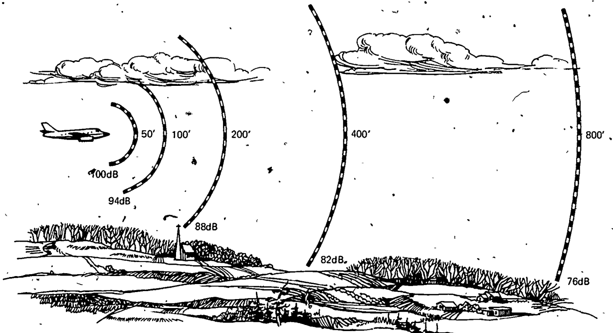
Fig. 3-14a. REDUCTION IN NOISE LEVEL WITH DISTANCE FROM A POINT SOURCE
