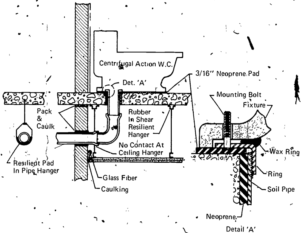
Fig. 4-28. PROPER INSTALLATION OF A TOILET FOR QUIET OPERATION
