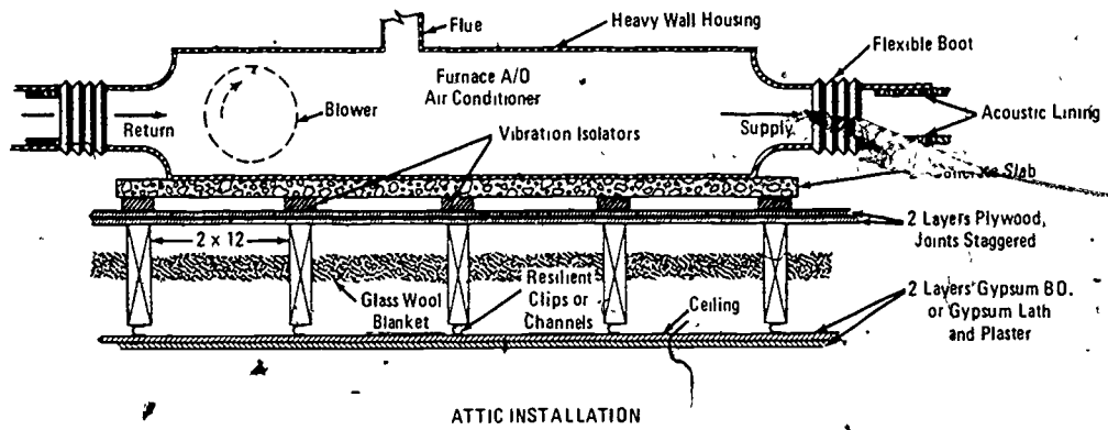
ATTIC INSTALLATION
