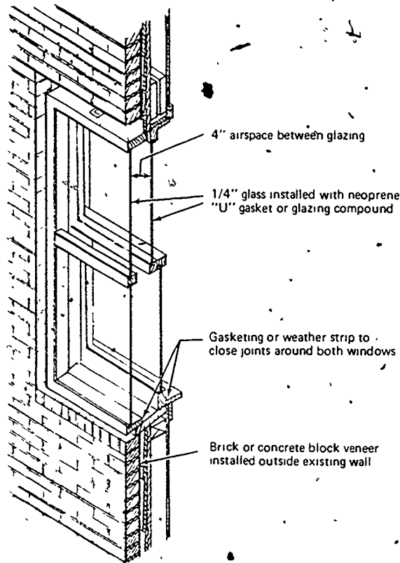
Fig. 5-2. INSTALLATION OF BRICK VENEER AND DOUBLE 1/4-INCH WINDOW GLAZING
