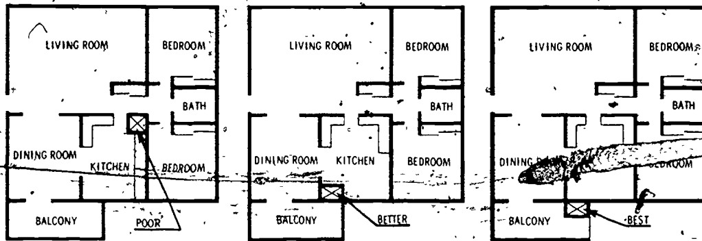
SELECTING PROPER LOCATION FOR CLOSET-INSTALLED FURNACE UNIT
