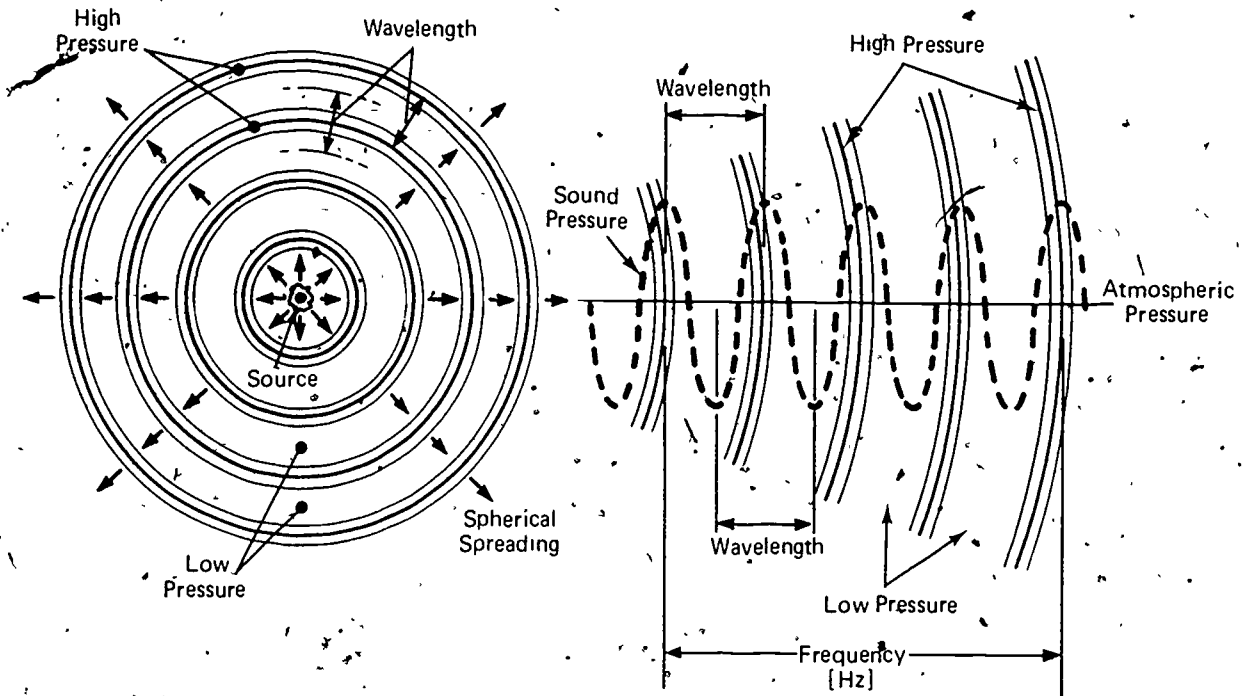
Fig. 3-11. PROPERTIES OF SOUND WAVES
