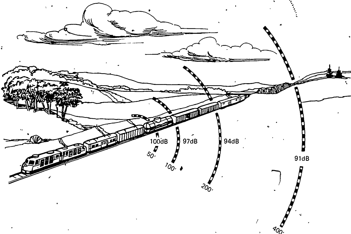
Fig. 3-14b. REDUCTION IN NOISE LEVEL WITH DISTANCE FROM A LINE SOURCE
