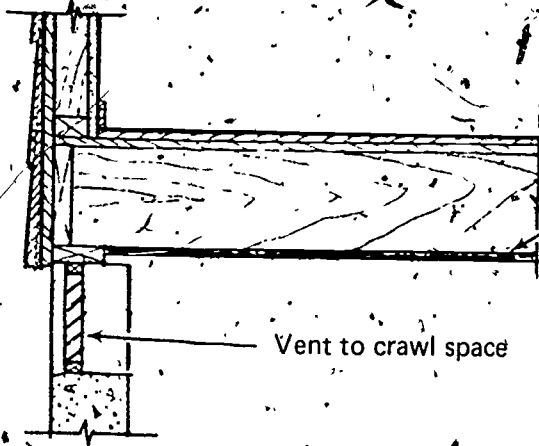
A—Added Floor Construction
