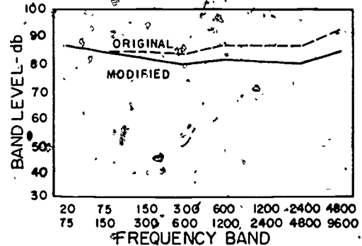
Fig. 3-20 EFFECTIVENESS OF VARIOUS NOISE REDUCTION TECHNIQUES
