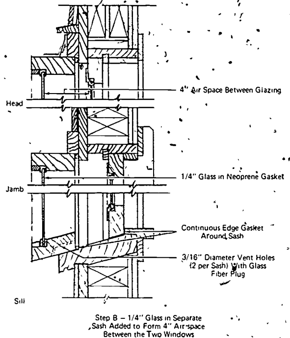
Fig. 5-3. DETAILS OF DOUBLE 1/4-INCH WINDOW GLAZING
