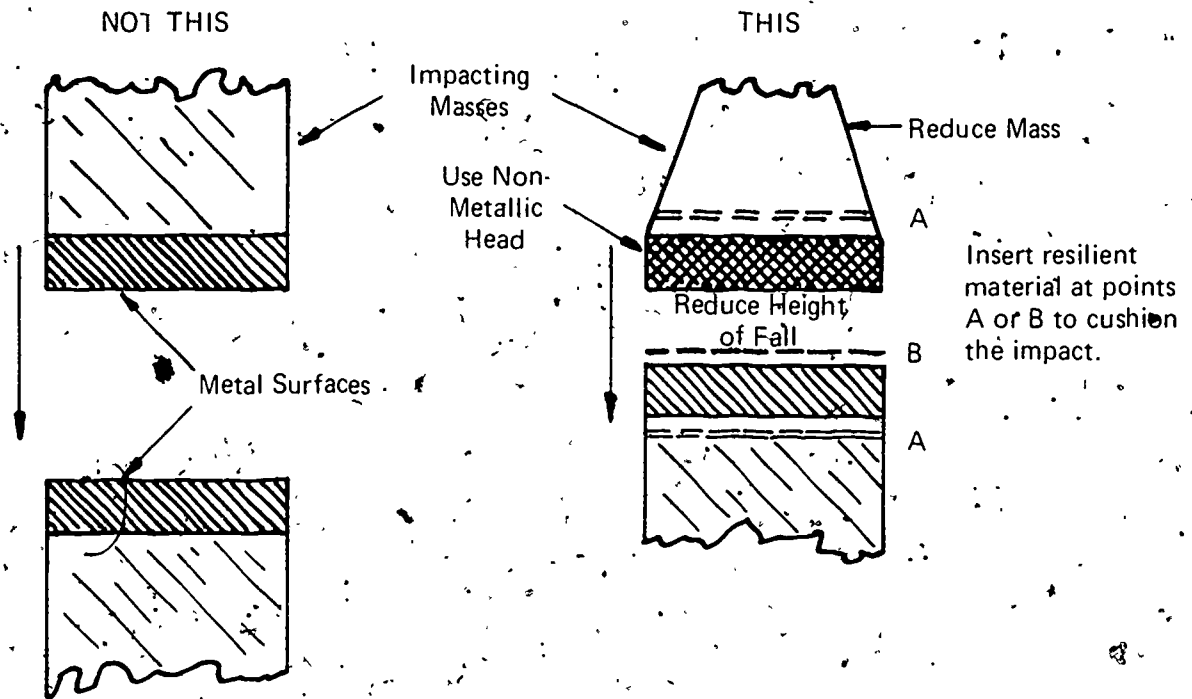
Fig. 3-1. METHODS OF REDUCING IMPACT FORCES TO LOWER NOISE RADIATION
