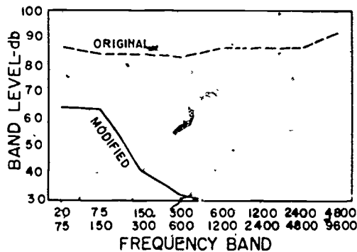
Fig. 3-20. EFFECTIVENESS OF VARIOUS NOISE REDUCTION TECHNIQUES
