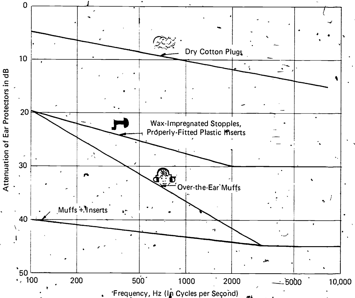
Fig. 2.4. SOUND ATTENUATION CHARACTERISTICS OF VARIOUS TYPES OF EAR PROTECTORS
