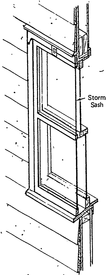
Fig. 5-1. DETAILS OF A DOUBLE-HUNG WINDOW WITH A STORM SASH
