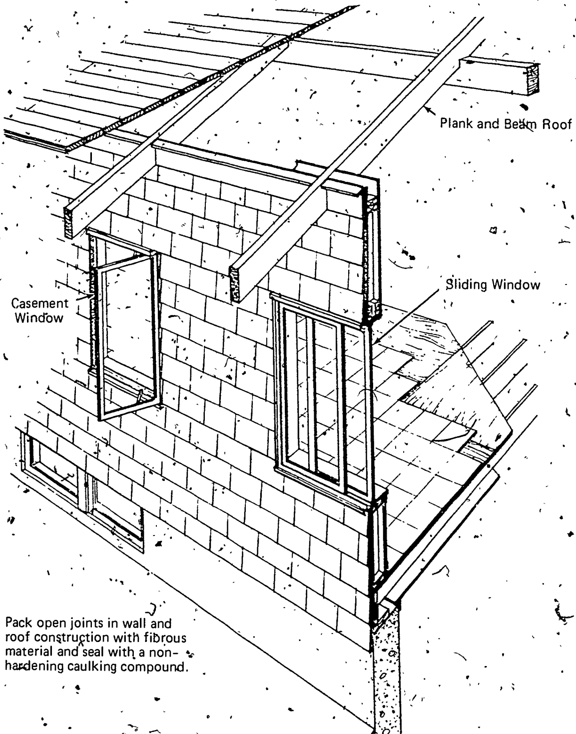
Fig. 5-8. HOUSE WITH A BASEMENT AND PLANK AND BEAM ROOF
