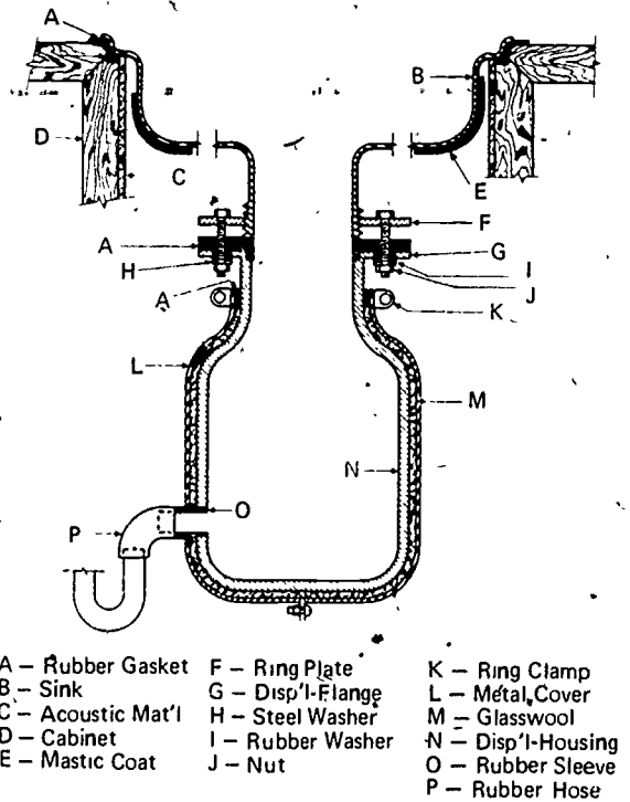
Fig. 4-8. DESIGN AND INSTALLATION OF A GARBAGE DISPOSER FOR QUIET OPERATION
