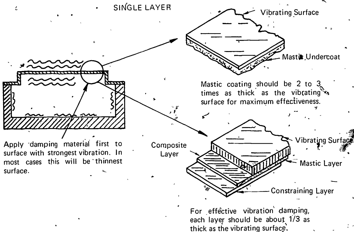
Fig. 3-9. REDUCING VIBRATION WITH DAMPING MATERIALS
