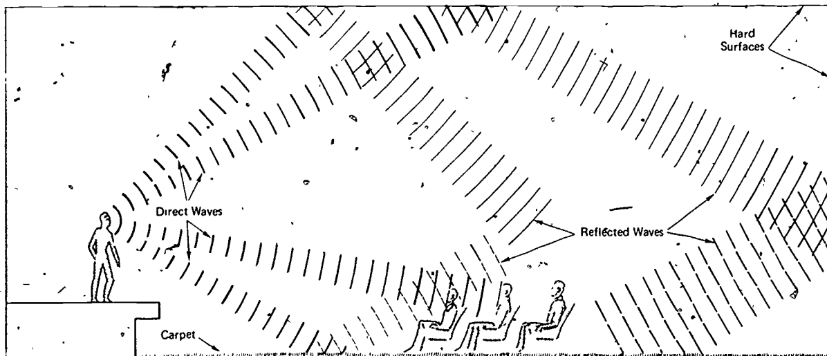
Fig 3-12. PROPAGATION OF DIRECT AND REFLECTED SOUND WAVES IN A ROOM
