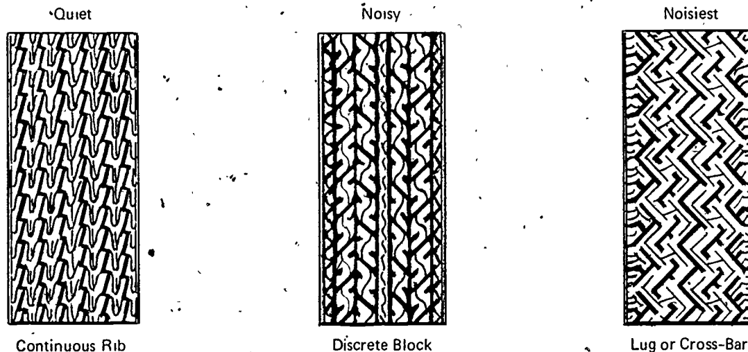
Fig. 9-1. BASIC TIRE TREAD DESIGNS IN ORDER OF RELATIVE NOISINESS
