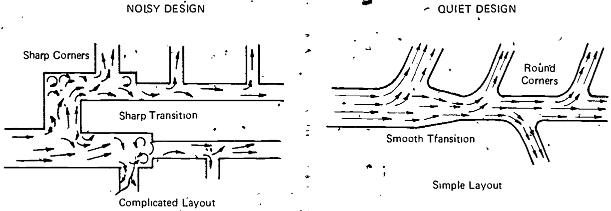
Fig. 3-5b. DESIGN OF QUIET FLOW SYSTEMS
