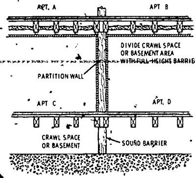
Fig. 4-16. METHODS OF CONTROLLING FLANKING SOUND TRANSMISSION PATHS
