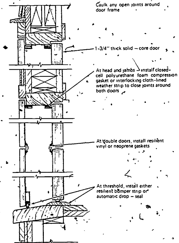
Fig. 5-5. DETAILS OF DOOR MODIFICATIONS
