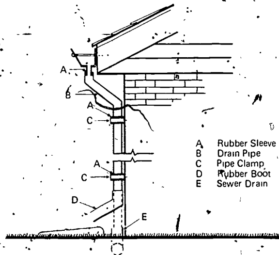
Fig. 4-29. METHODS OF CONTROLLING NOISE FROM RAIN GUTTERS AND DOWNSPOUTS
