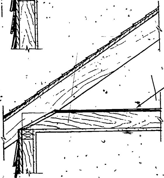
B—Ventilated Attic Space
