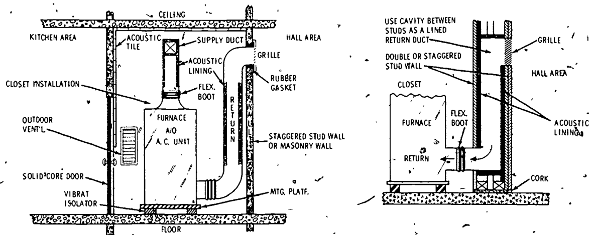
RECOMMENDED DESIGN OF CLOSET AND INSTALLATION OF FURNACE UNIT
