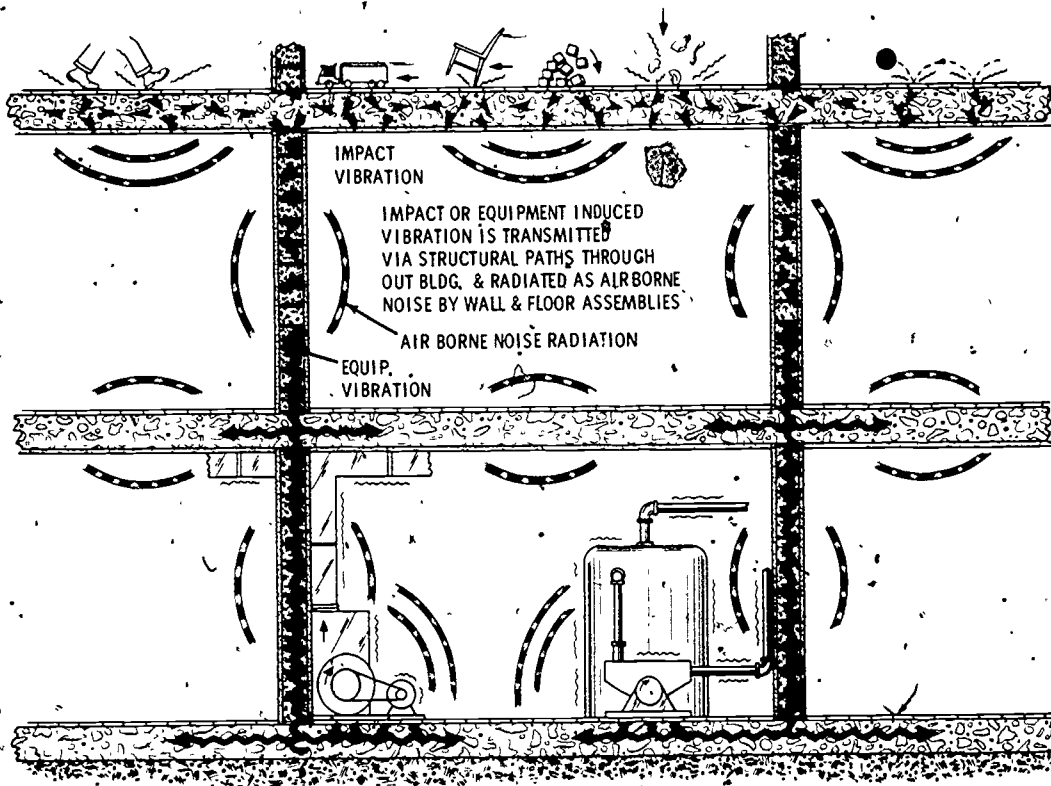
Fig. 4-4. COMMON STRUCTURE-BORNE NOISE AND VIBRATION PATHS IN BUILDINGS.
