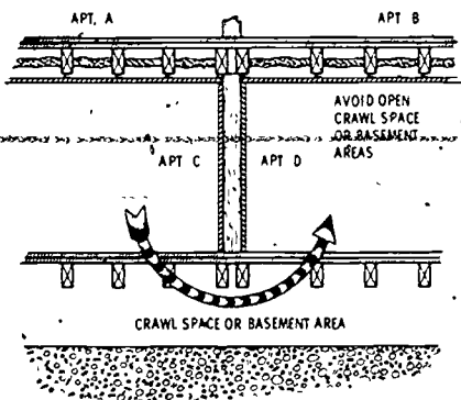
Fig. 4-16. METHODS OF CONTROLLING FLANKING SOUND TRANSMISSION PATHS
