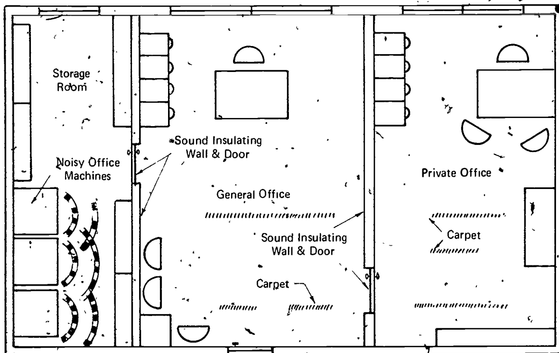
Fig. 8-2. A WELL-PLANNED OFFICE COMPLEX WHICH AFFORDS PRIVACY AND A QUIET ENVIRONMENT
