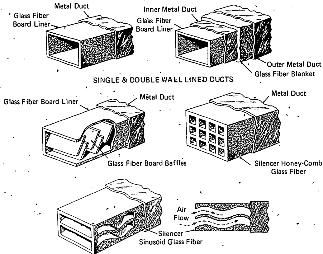
Fig. 3-16. VARIOUS TYPES OF ACOUSTICAL DUCT LINING, BAFFLES AND SILENCERS
