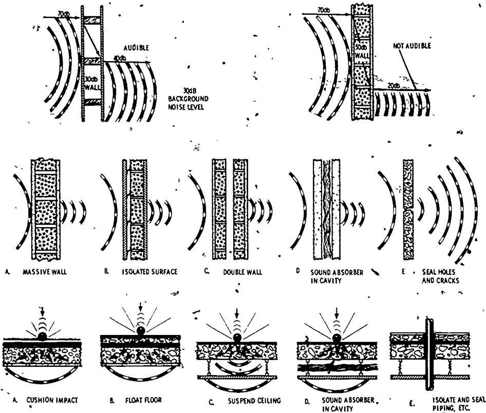
Fig. 4-5. METHODS OF CONTROLLING AIRBORNE AND IMPACT SOUND TRANSMISSION THROUGH WALLS AND FLOORS
