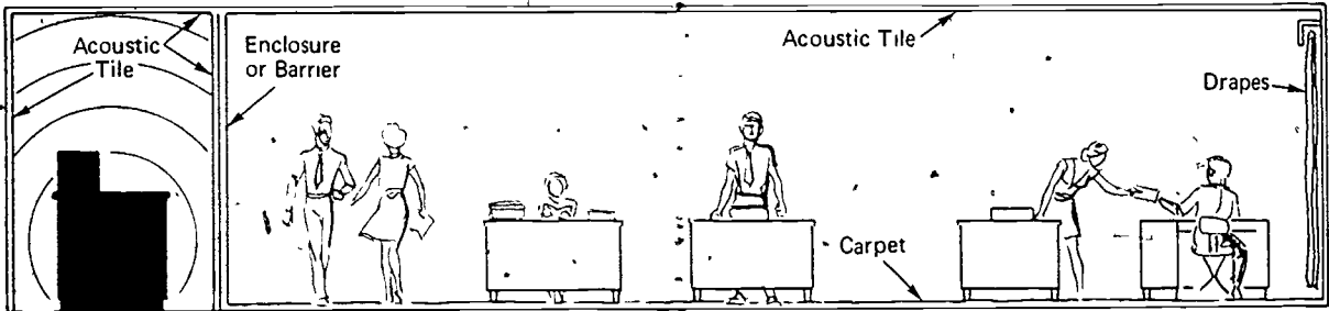
Fig. 3-15. NOISE CONTROL OF THE TRANSMISSION PATH
