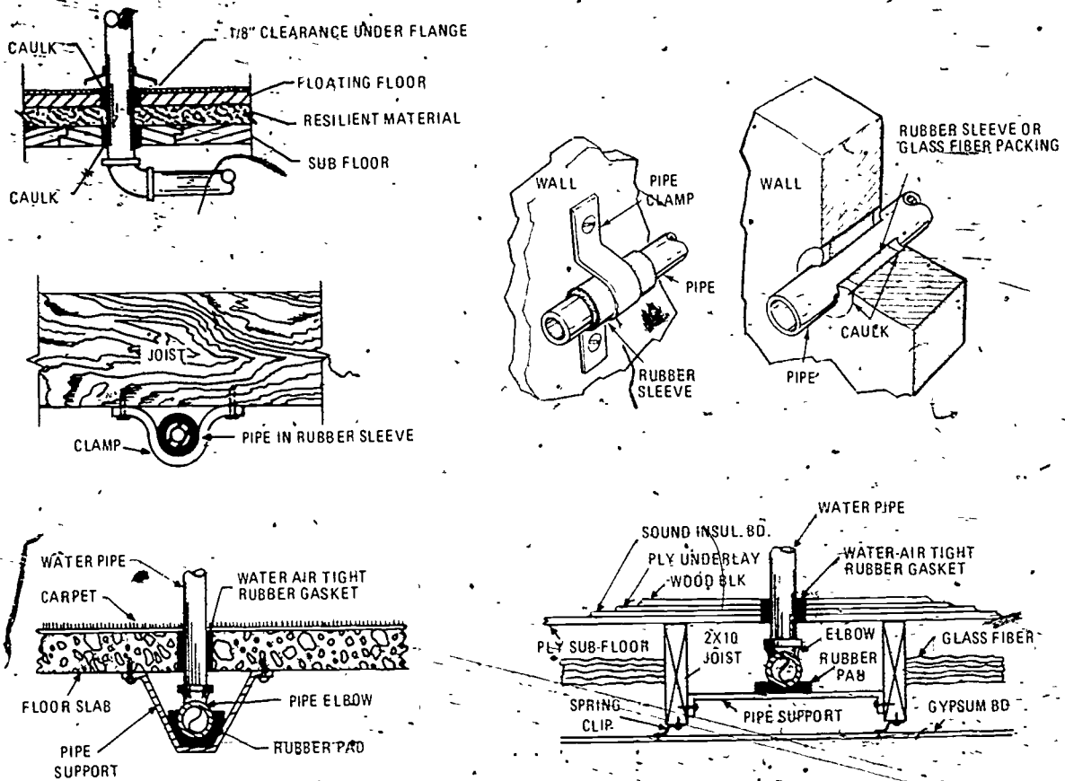
Fig. 4-26. METHODS OF INSTALLING PIPES FOR QUIET OPERATION
