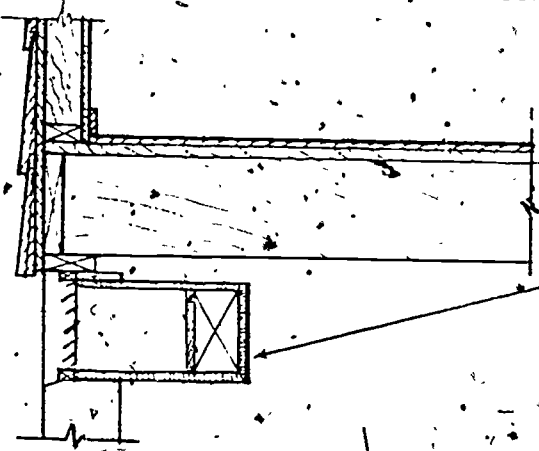
B—Vent Attenuators
