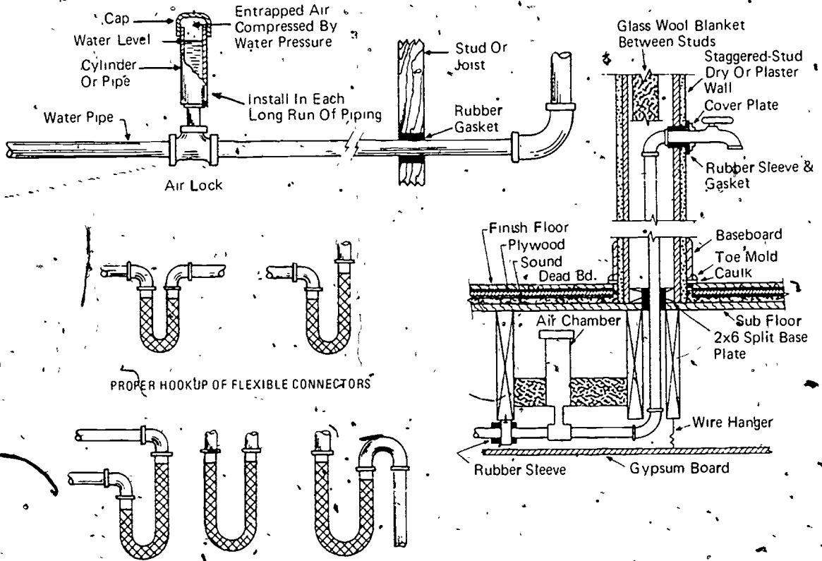
Fig. 4-25. TECHNIQUES FOR CONTROLLING NOISE IN PLUMBING SYSTEMS
