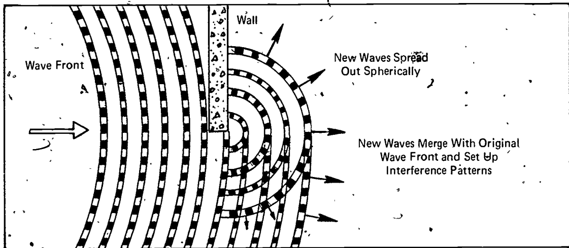
Fig. 3-13a. DIFFRACTION OF A SOUND WAVE PASSING THROUGH A SMALL HOLE
