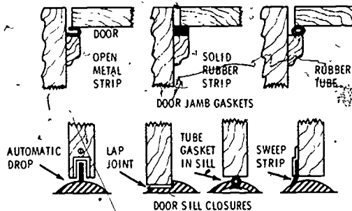
Fig. 4-7. PROPER INSTALLATION OF SOUND-INSULATING DOORS
