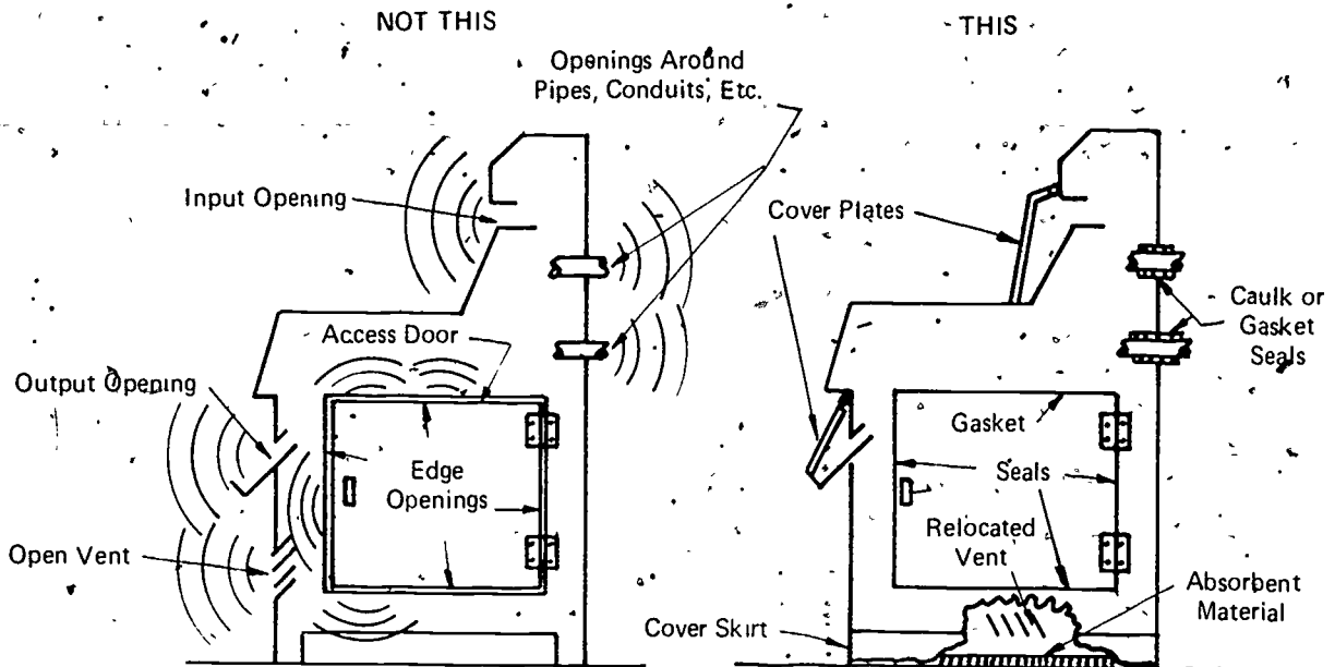
Fig. 3-10. TECHNIQUES FOR REDUCING THE RADIATION OF NOISE FROM OPENINGS IN A MACHINE
