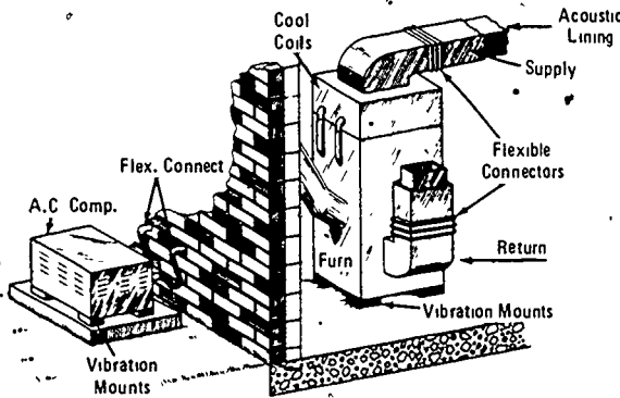
BASEMENT INSTALLATION
