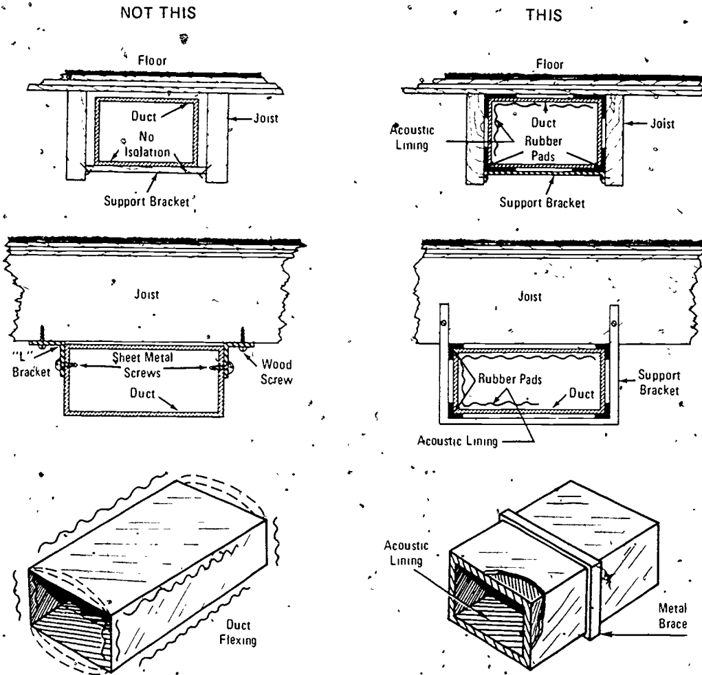
Fig. 4 23. METHODS OF REDUCING NOISE DUE TO AIR FLOW AND VIBRATION IN DUCT SYSTEMS
