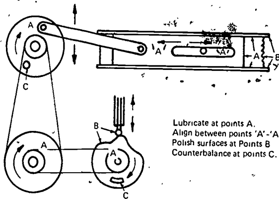
Fig 34. REDUCING FRICTION OF ROTATING AND SLIDING PARTS TO DECREASE NOISE RADIATION
