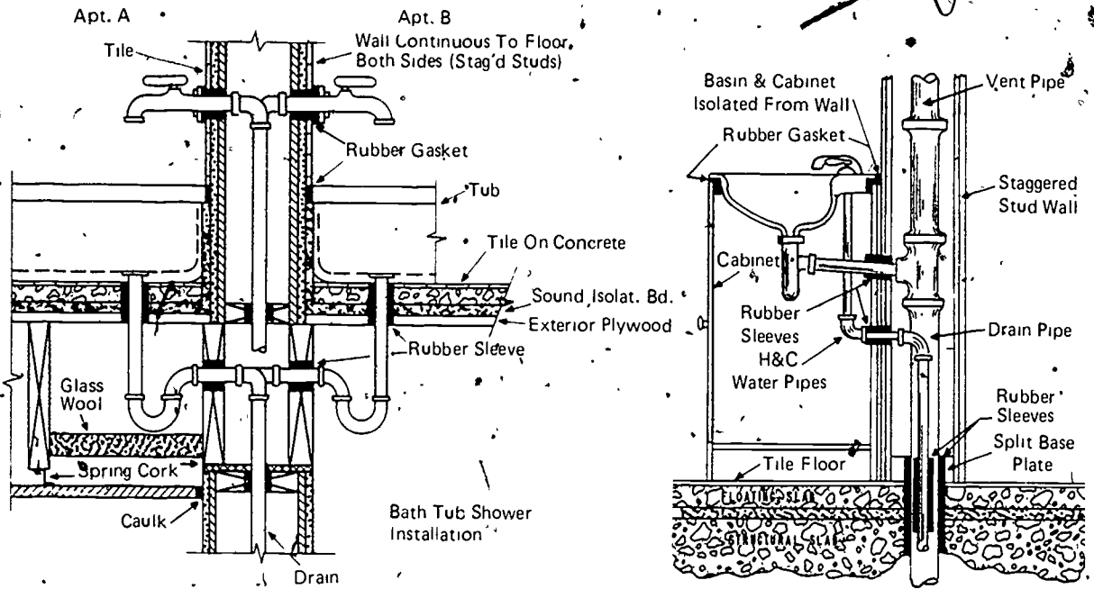
Fig. 4-27. PROPER INSTALLATION OF BATH TUBS AND WASH BASINS
