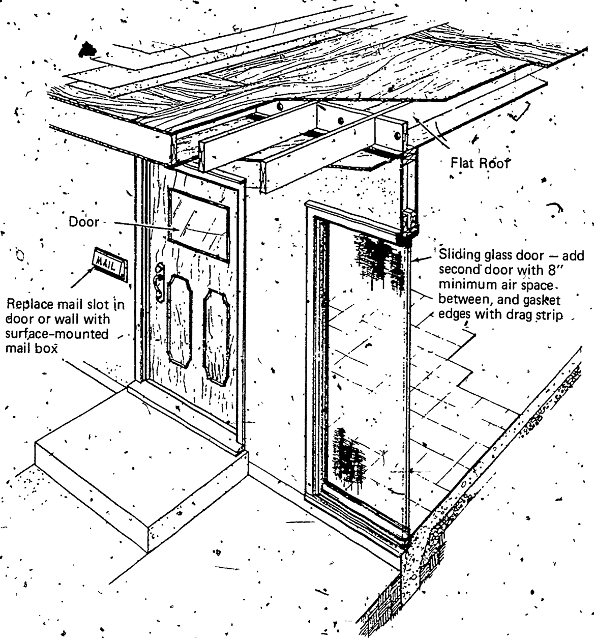
Fig. 5-9. HOUSE WITH SLAB ON GRADE AND A FLAT ROOF
