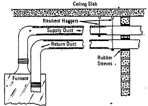
Fig. 4-21. TECHNIQUES FOR THE CONTROL OF NOISE FROM EXISTING ATTIC OR BASEMENT INSTALLATIONS OF FURNACES AND AIR-CONDITIONING UNITS
