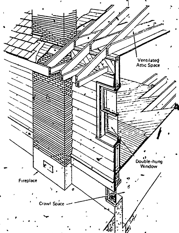
Fig 5-7 HOUSE WITH A CRAWL SPACE AND VENTILATED ATTIC
