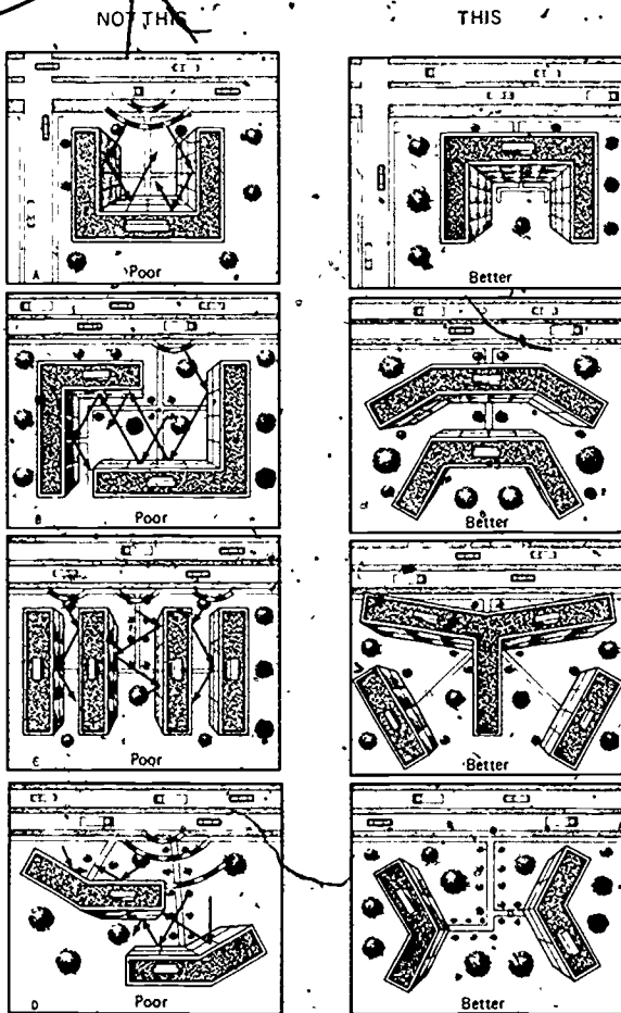
Fig 6-4. ORIENTATION OF APARTMENT BUILDINGS FOR OPTIMUM ACOUSTICAL SHIELDING
