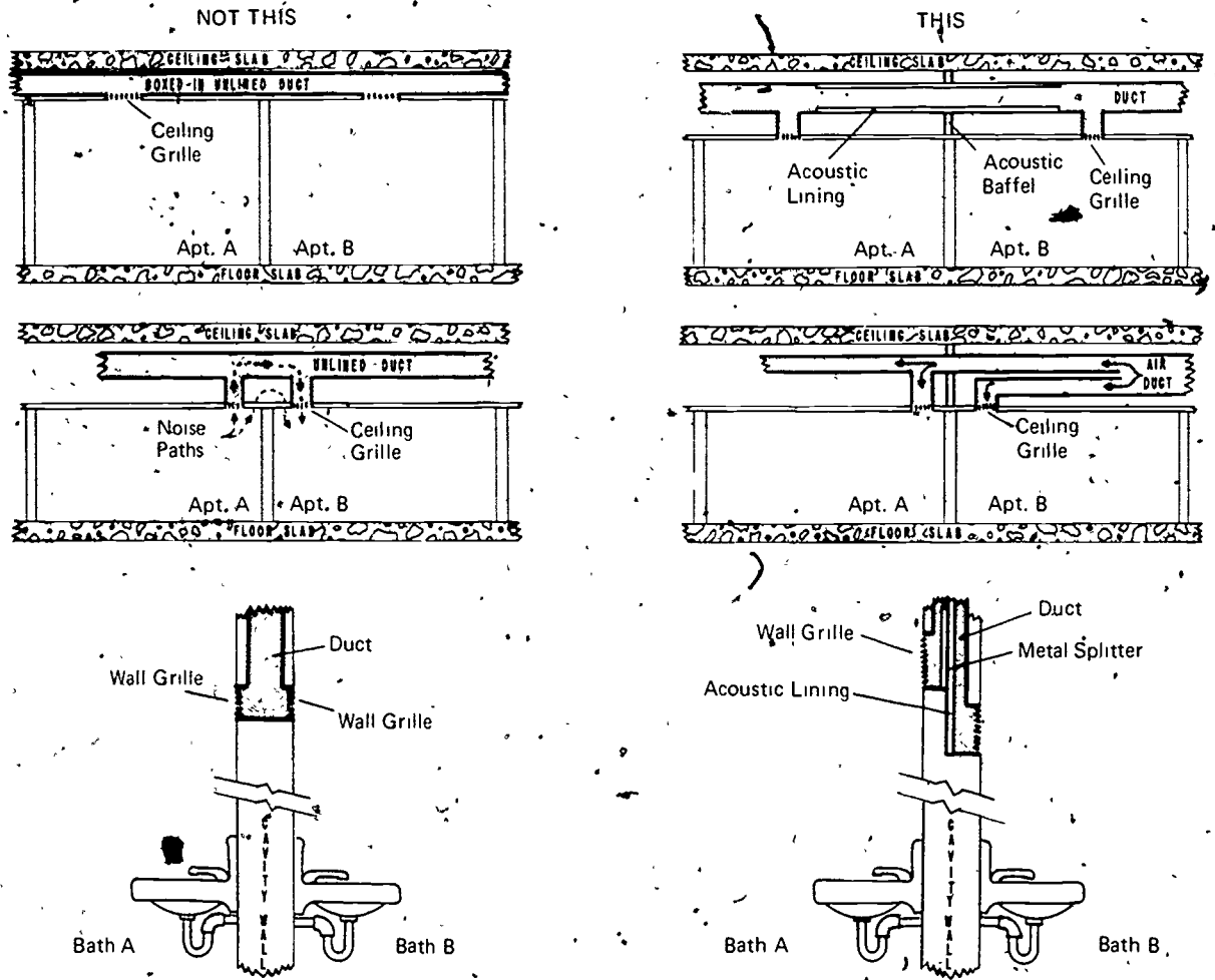
Fig. 4-24. METHODS OF CONTROLLING CROSS TALK AND THE TRANSMISSION OF FLANKING NOISE IN DUCTS
