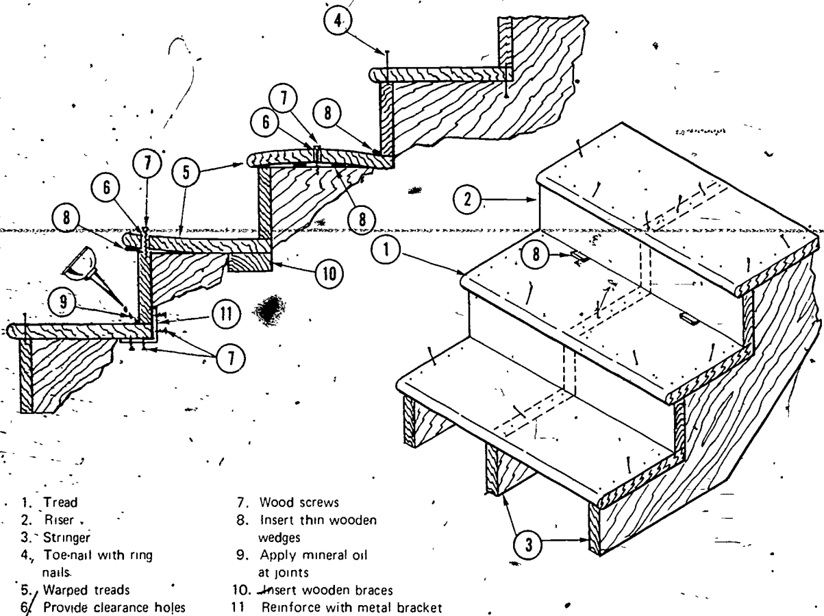
Fig. 4-20. TECHNIQUES FOR THE CONTROL OF STAIR SQUEAKING
