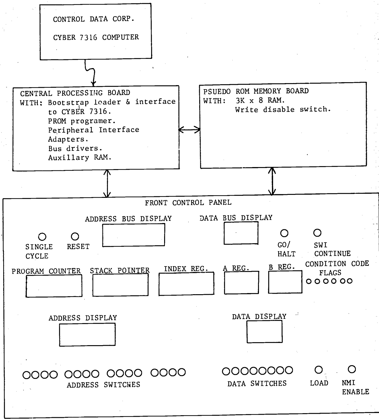
Figure 5. Hardware development system.
