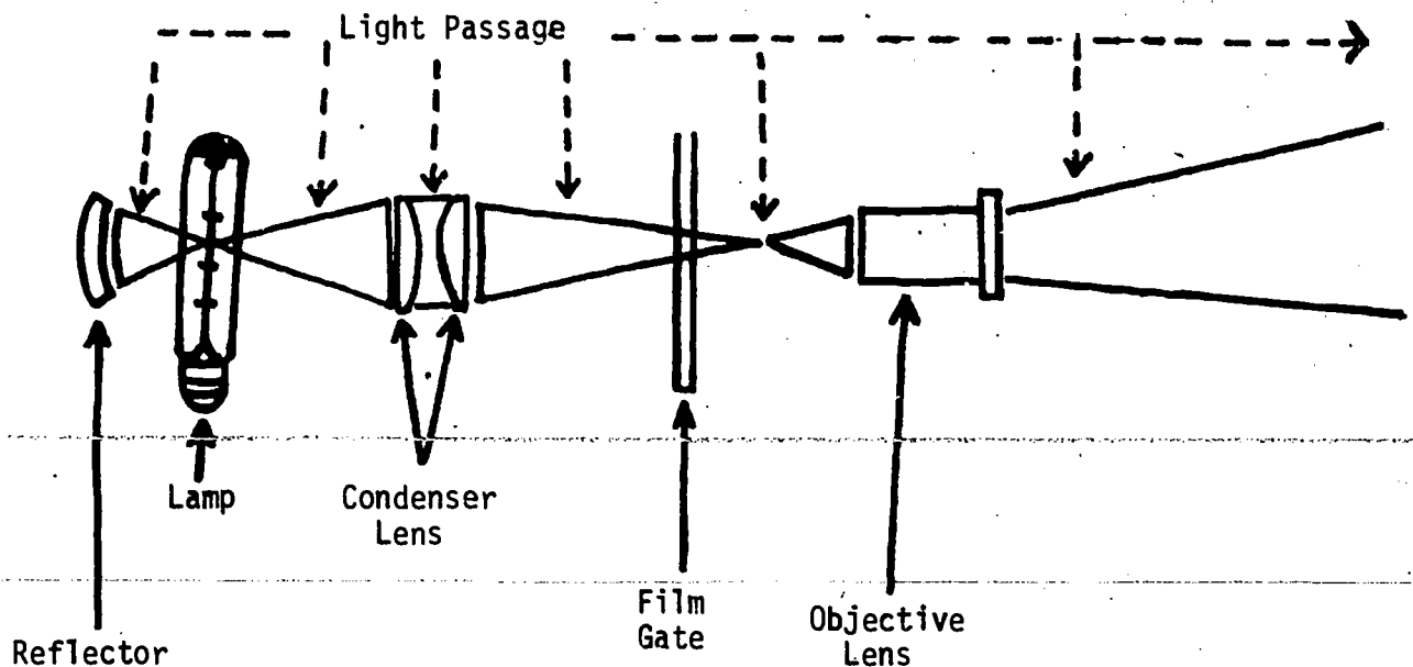
Older type projector lamp without built-in reflector:
