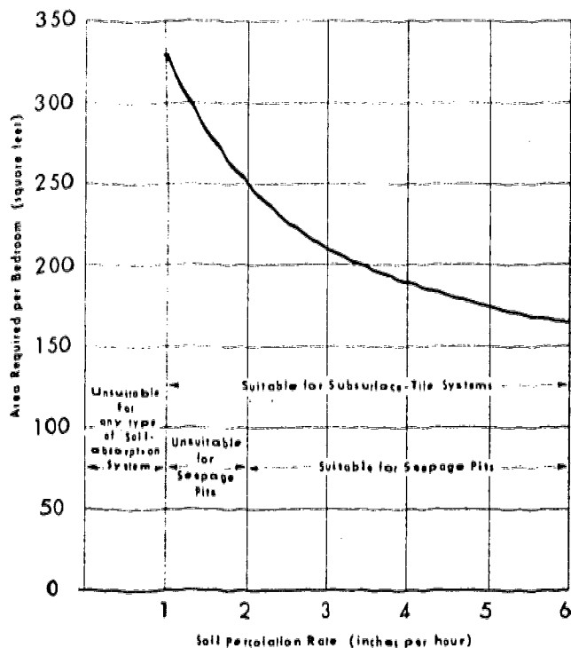
Size of absorption field needed for private residences. Adapted from Manual of Septic Tank Practice (1, p. 9)
