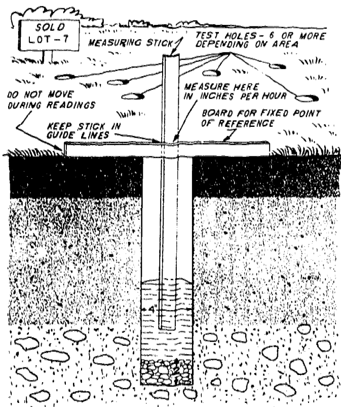
A percolation test hole with measuring stick is shown in the foreground; other test holes properly distributed over the field are in the background.
