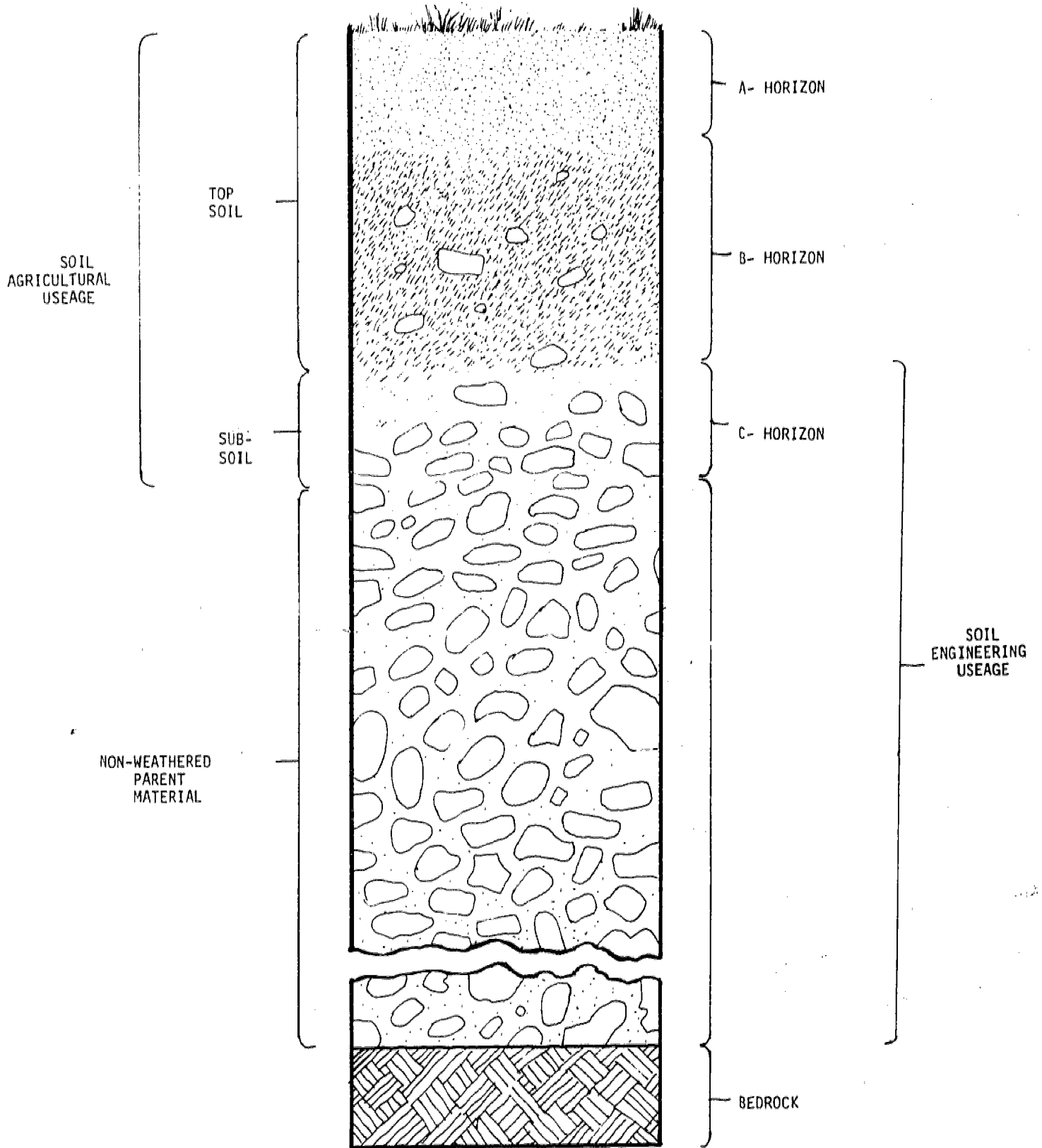
SOIL PROFILE DEVELOPED IN A GLACIAL TILL
