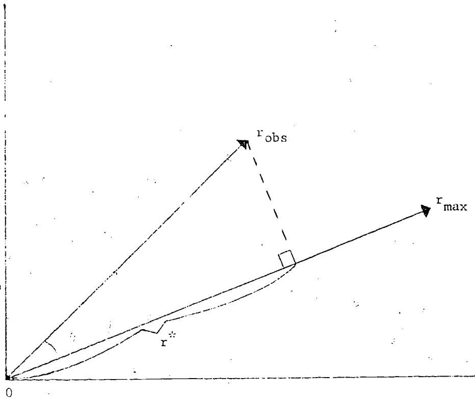
Figure 2. Spatial Representation of Projection of a Shorter Vector r_{\text{obs}} on a Longer Vector r_{\max}
