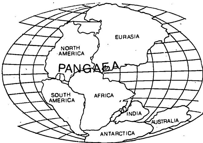
Fig. 2 Pangaea - about 200 million years ago
