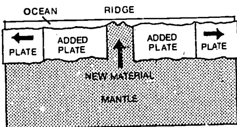
Fig. 4 Plates moving apart
