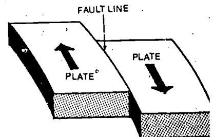
Fig. 6 Plates moving along a fault
