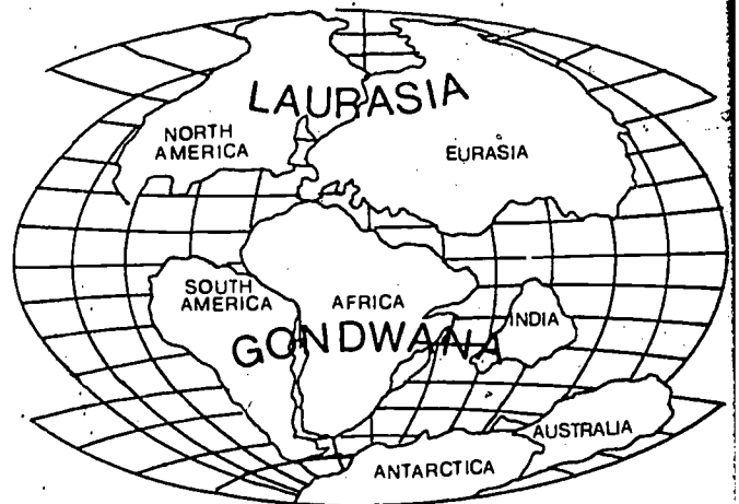
Fig. 3 Laurasia and Gondwanaland - about 135 million years ago
