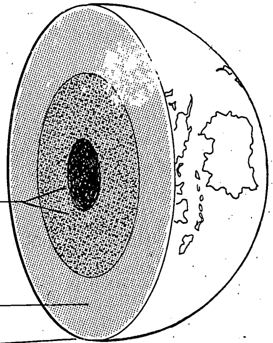
Fig. 1 inner and outer core - about 2,150 miles thick
