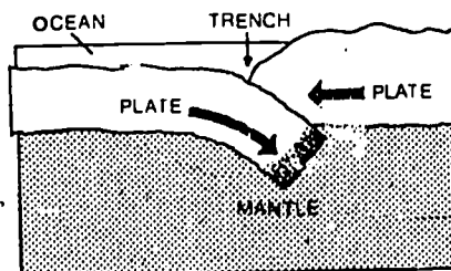
Fig. 5 Plates colliding
