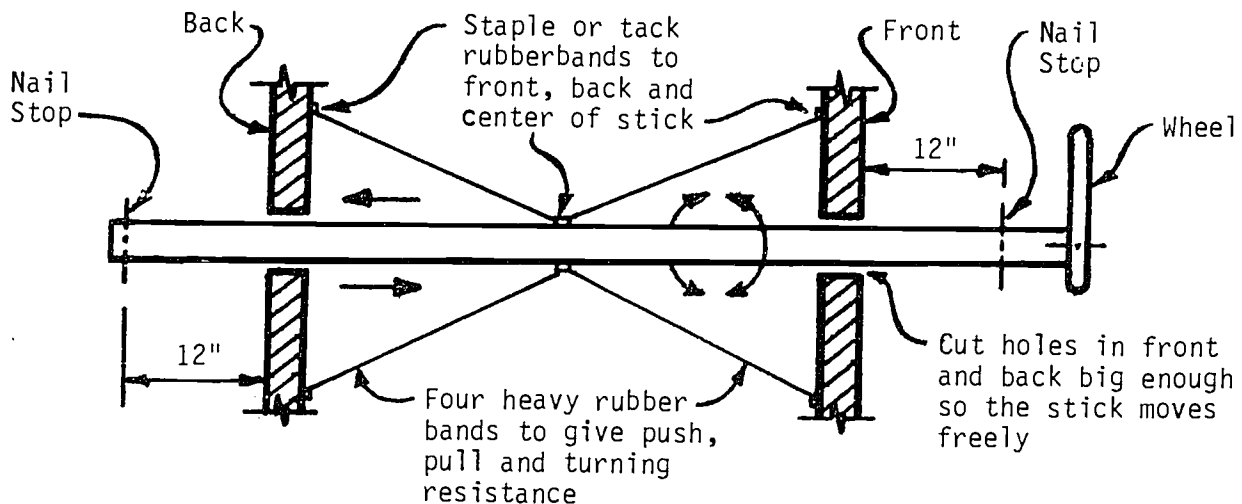
CONTROL WHEEL INSTALLATION
