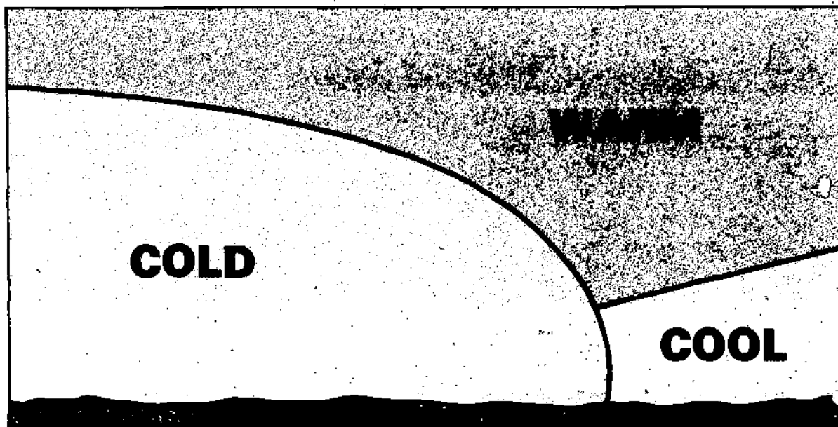
FIGURE 64. Cross section of a cold-front occlusion. Its weather map symbol is the same as for a warm-front occlusion shown in Figure 63. In the cold-front occlusion, the coldest air is under the cold front. When it overtakes the warm front, it lifts the warm front aloft; and cold air replaces cool air at the surface.
