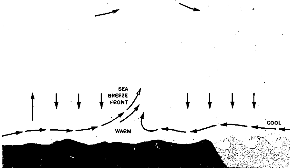
FIGURE 165. Schematic cross section through a sea breeze front. If the air inland is moist, cumulus often marks the front.
