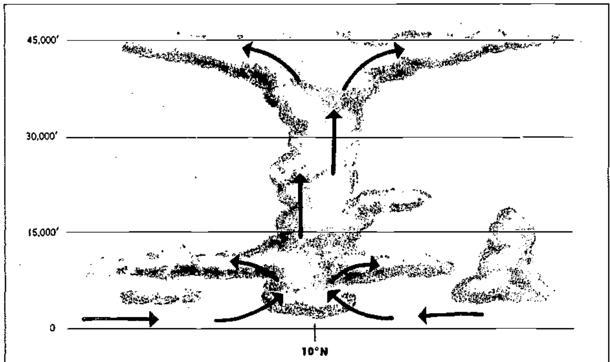
FIGURE 139. Prevailing winds in the Tropics in January.
