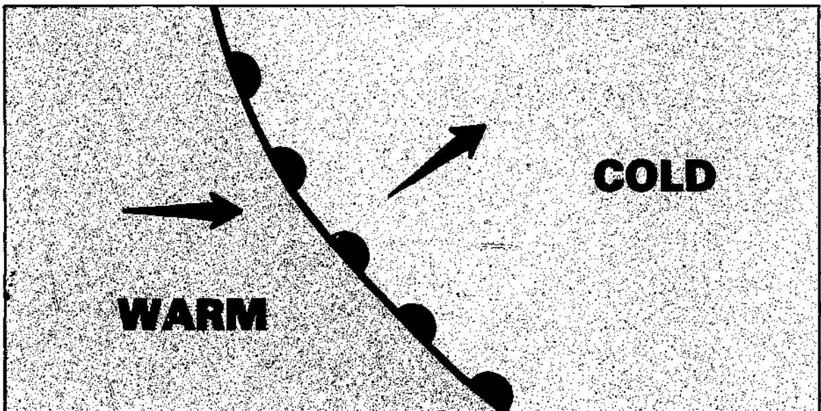
FIGURE 60. Cross section of a warm front (top) with the weather map symbol (bottom). The symbol is a line with rounded barbs pointing in the direction of movement. If a map is in color, a red line represents the warm front. Slope of a warm front generally is more shallow than slope of a cold front. Movement of a warm front shown by the heavy black arrow is slower than the wind in the warm air represented by the light solid arrows. The warm air gradually erodes the cold air.
