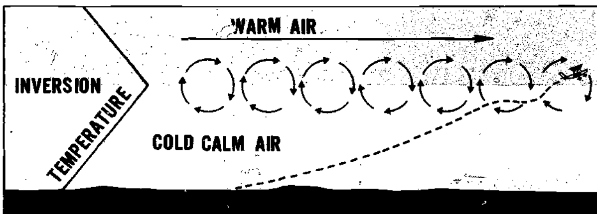
FIGURE 86. Wind shear in a zone between relatively calm wind below an inversion and strong wind above the inversion. This condition is most common at night or in early morning. It can cause an abrupt turbulence encounter at low altitude.
