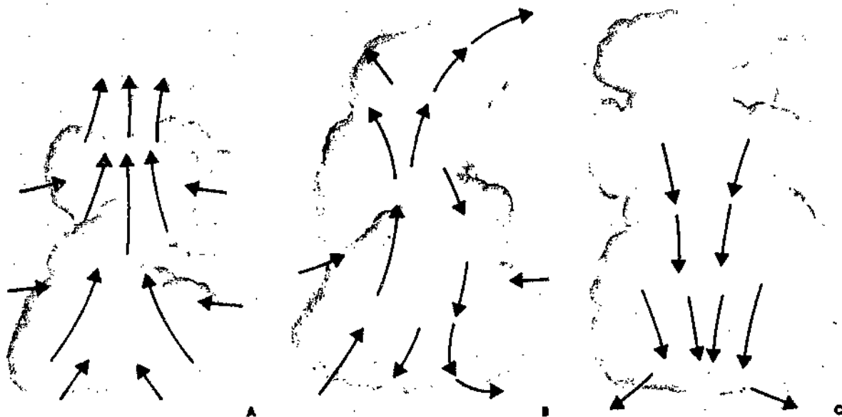
FIGURE 105. The stages of a thunderstorm. (A) is the cumulus stage; (B), the mature stage; and (C), the dissipating stage. Arrows depict air flow.
