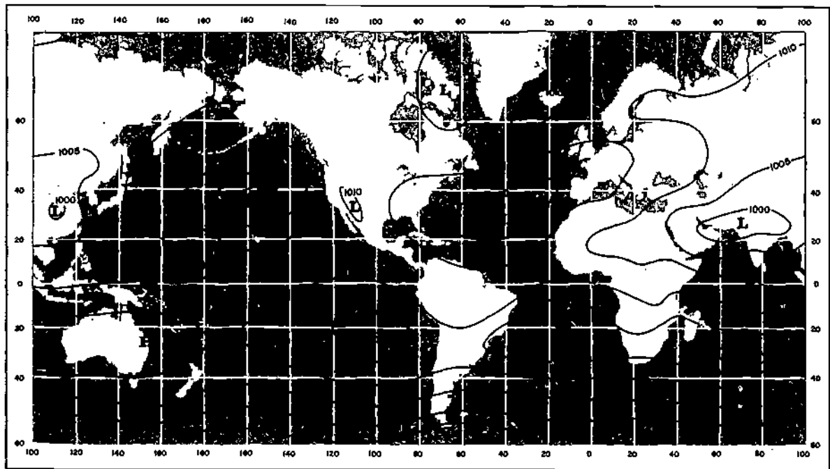
FIGURE 23. Mean worldwide surface pressure distribution in July. In the warm Northern Hemisphere, warm land areas tend to have low pressure, and cool oceanic areas tend to have high pressure. In the cool Southern Hemisphere, the pattern is reversed; cool land areas tend to have high pressure; and water surfaces, low pressure. However, the relationship is not so evident in the Southern Hemisphere because of relatively small amounts of land. The subtropical high pressure belts are clearly evident at about 30° latitude in both hemispheres.
