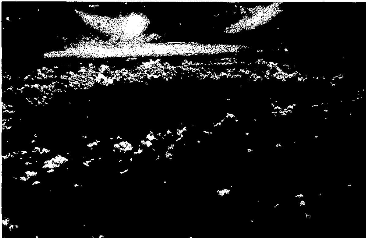
FIGURE 39. A view of clouds from 27,000 feet over Lake Okechobee in southern Florida. Note the lake effect. During daytime, cool air from the lake flows toward the warmer land forming convective clouds over the land.
