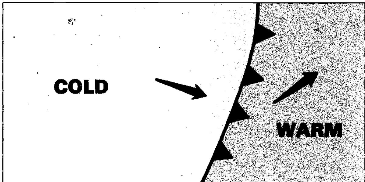
FIGURE 59. Cross section of a cold front (above) with the weather map symbol (below). The symbol is a line with pointed barbs pointing in the direction of movement. If a map is in color, a blue line represents the cold front. The vertical scale is expanded in the top illustration to show the frontal slope. The frontal slope is steep near the leading edge as cold air replaces warm air. The solid heavy arrow shows movement of the front. Warm air may descend over the front as indicated by the dashed arrows; but more commonly, the cold air forces warm air upward over the frontal surface as shown by the solid arrows.
