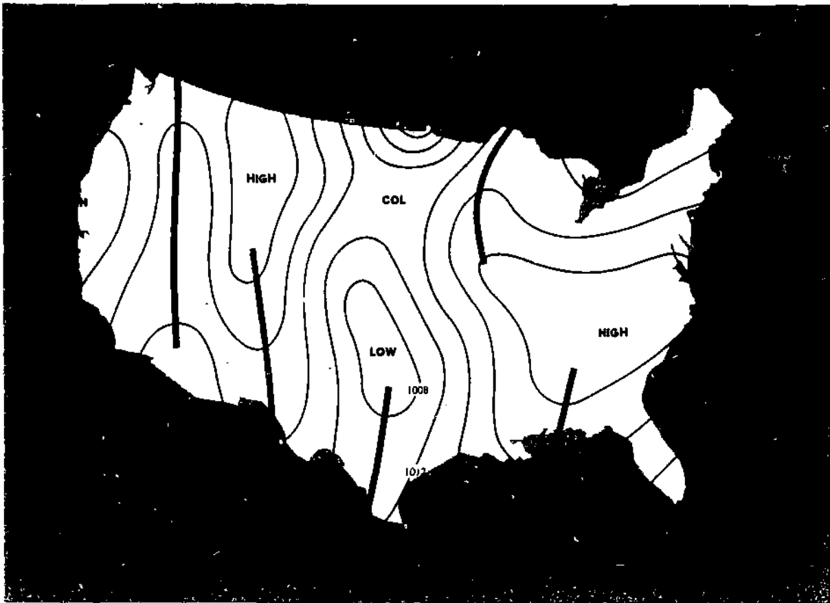
FIGURE 13. Pressure systems.
