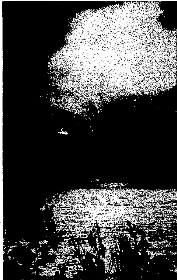
FIGURE 108. A waterspout.
