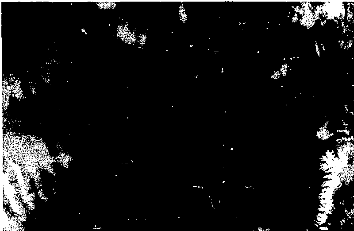
FIGURE 84. Mountain wave clouds over the Tibetan Plateau photographed from a manned spacecraft.
