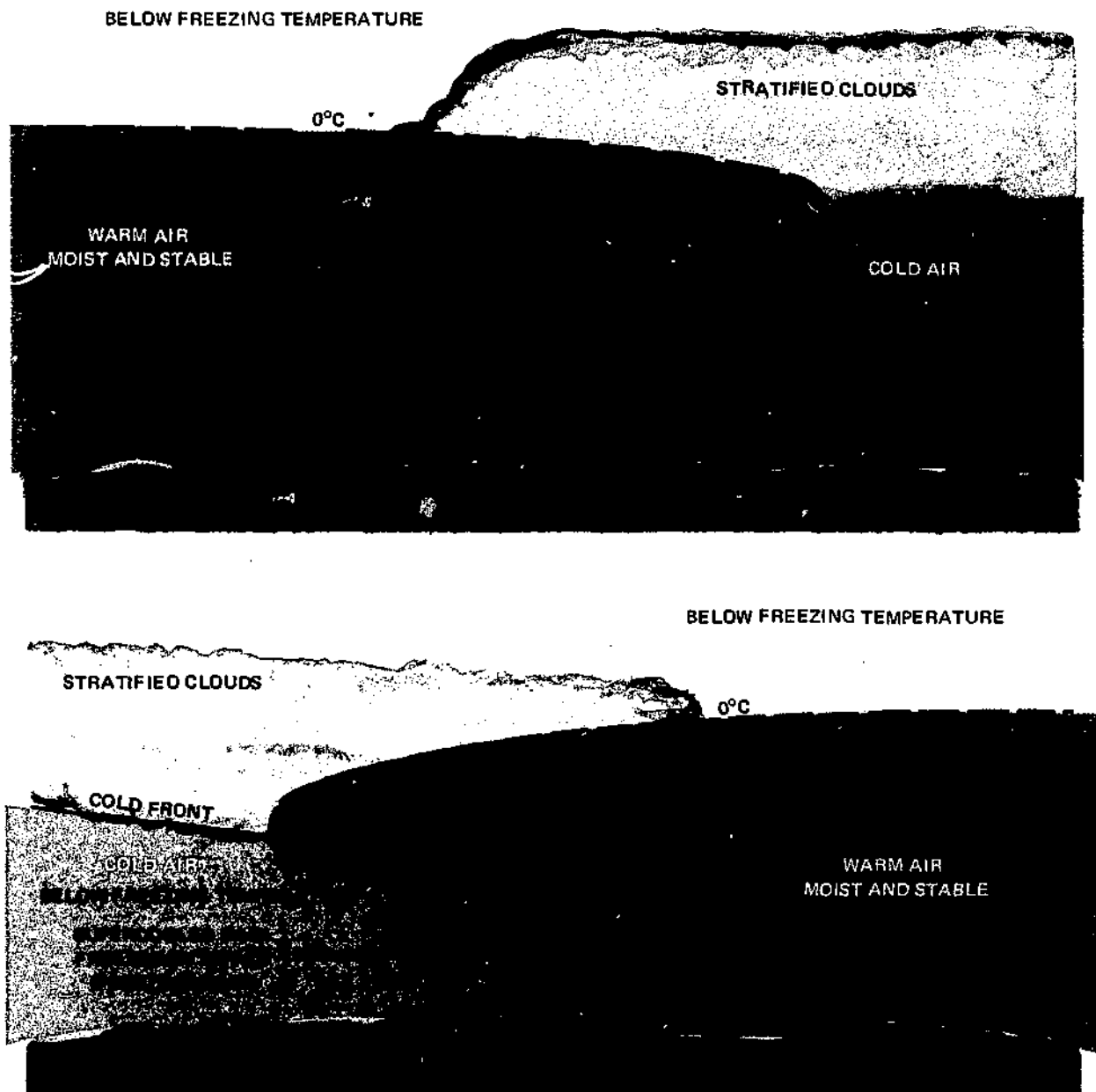
FIGURE 98. Freezing rain with a warm front (top) and a cold front (bottom). Rainfall through warm air aloft into subfreezing cold air near the ground. The rain becomes supercooled and freezes on impact.
