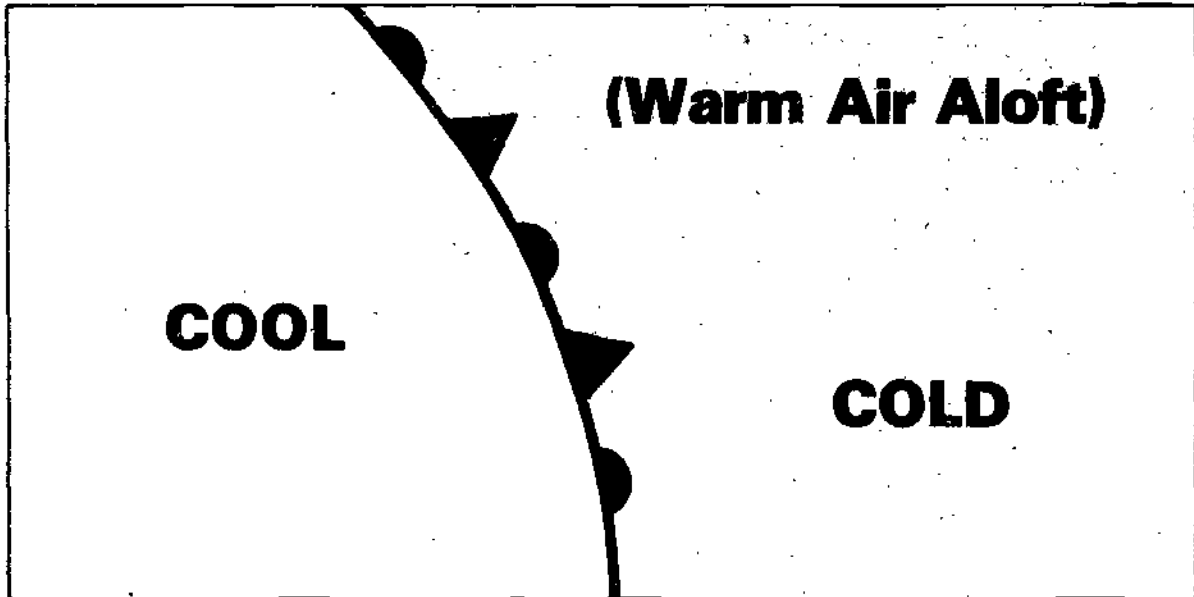
FIGURE 63. Cross section of a warm-front occlusion (top) and its weather map symbol (bottom). The symbol is a line with alternating pointed and rounded bars on the same side of the line pointing in the direction of movement. Shown in color on a weather map, the line is purple. In the warm front occlusion, air under the cold front is not as cold as air ahead of the warm front; and when the cold front overtakes the warm front, the less cold air rides over the colder air. In a warm front occlusion, cool air replaces cold air at the surface.
