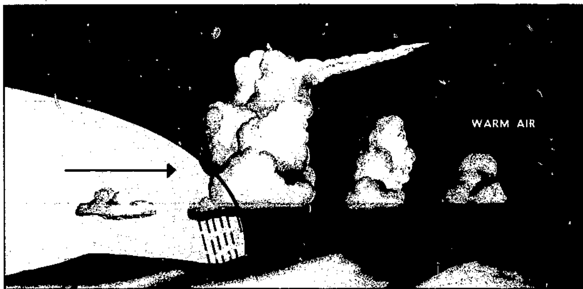
FIGURE 68. A cold front underrunning warm, moist, unstable air. Clouds are cumuliiform with possible showers or thunderstorms near the surface position of the front. Convective clouds often develop in the warm air ahead of the front. The warm, wet ground behind the front generates low-level convection and fair weather cumulus in the cold air.
