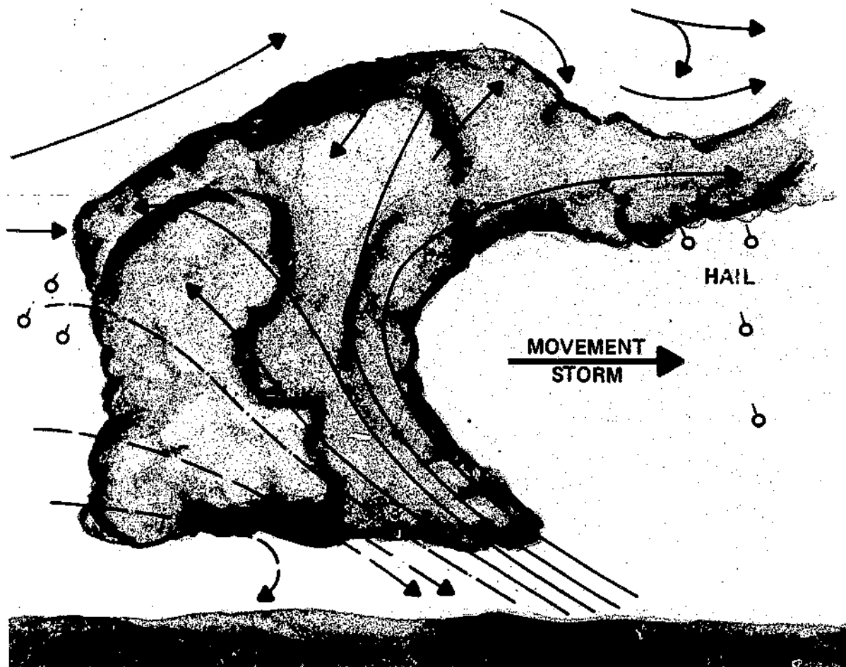
FIGURE 106. Schematic of the mature stage of a steady state thunderstorm cell showing a sloping updraft with the downdraft and precipitation outside the updraft not impeding it. The steady state mature cell may continue for many hours and deliver the most violent thunderstorm hazards.
