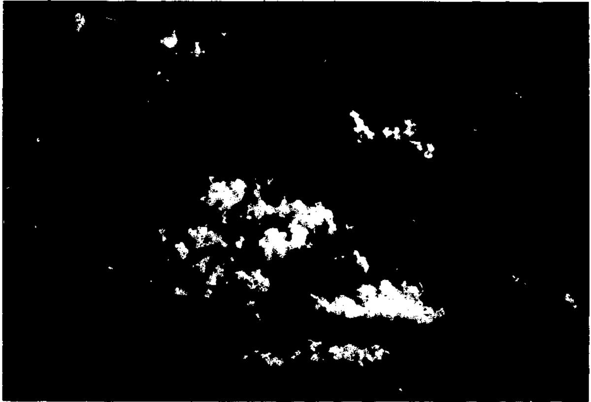
FIGURE 50. ALTOCUMULUS CASTELLANUS Altocumulus castellanus are middle level convective clouds. They are characterized by their billowing tops and comparatively high bases. They are a good indication of mid-level instability. Rough turbulence with some icing.
