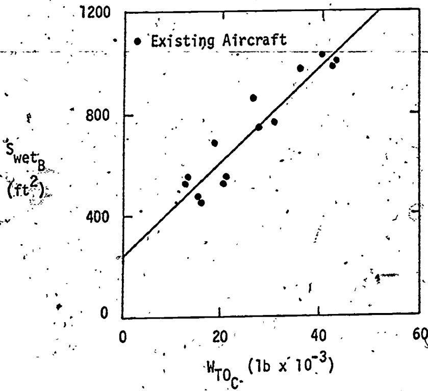
Fig. 2. Statistical Relation for Body Wetted Area.
