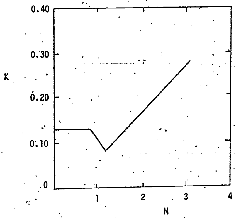
Fig. 5 Induced Drag Factor.
