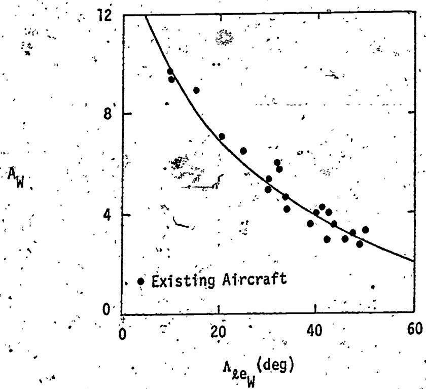
Fig. 3. Statistical Relation for Wing Aspect Ratio.
