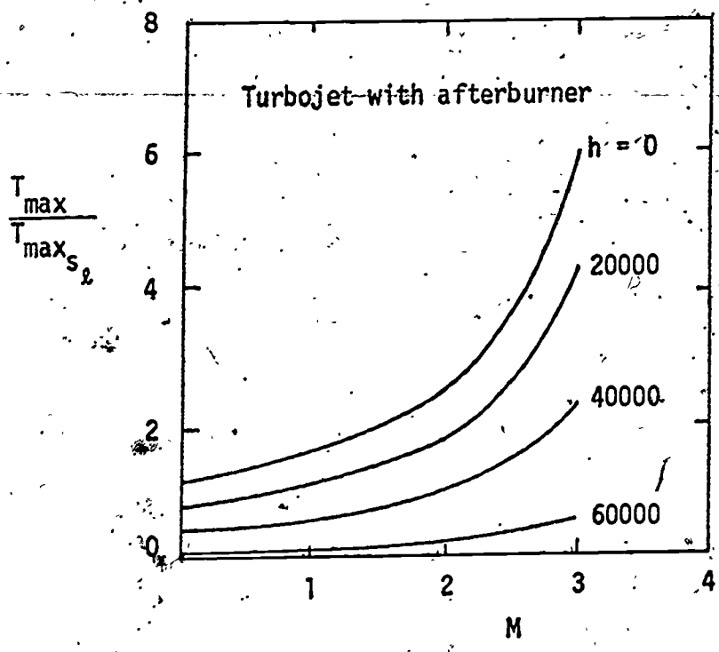
Fig. 6 Thrust.
