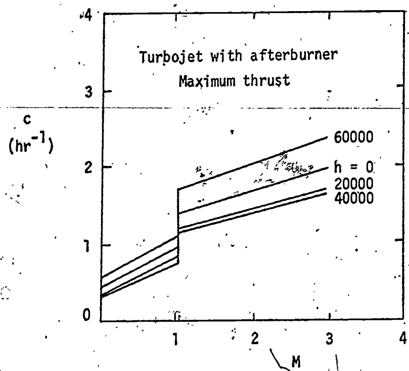
Fig. 7 Specific Fuel Consumption.
