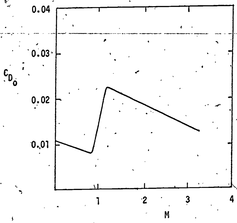
Fig. 4 Zero-Lift Drag Coefficient.
