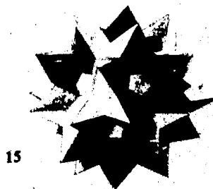
GREAT ICOSIDODECAHEDRON
