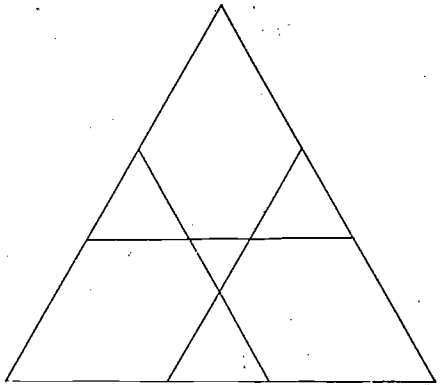
FIG. 50 (Model 15, p. 29)
