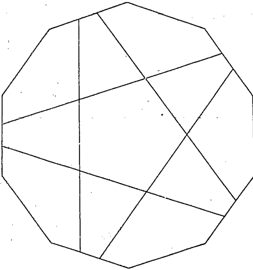
FIG. 46 (Model 11, p. 29)
