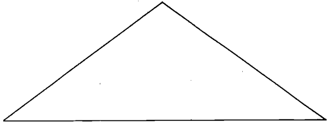
GREAT DODECAHEDRON
