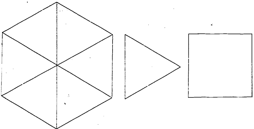
FIG. 38 (Model 7, p. 28)
