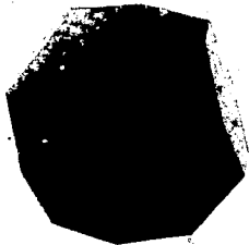
TRUNCATED CUBE
