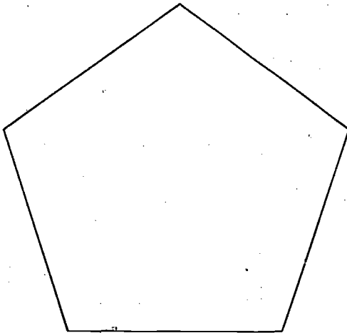
DODECAHEDRON
