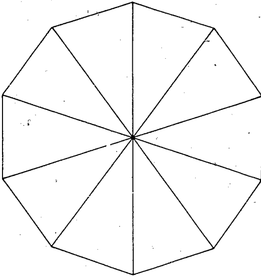
FIG. 43 (Model 3, p. 28)
