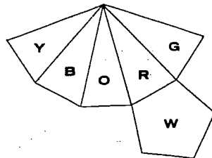
FIG. 10 Pentagonal pyramid
