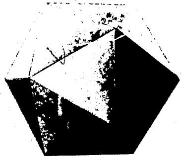
ICOSAHEDRON
