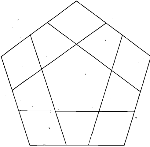
FIG. 45 (Model 10, p. 29)
