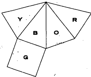
FIG. 9 Square pyramid
