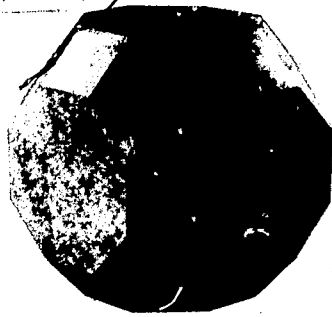
GREAT RHOMBICUBOCTAHEDRON
