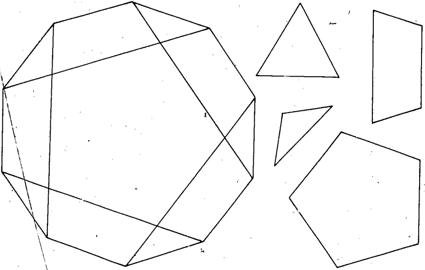
FIG. 41 (Model 8, p. 28)
