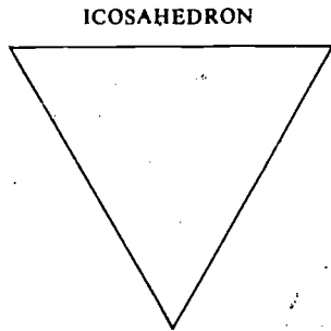
ICOSAHEDRON
