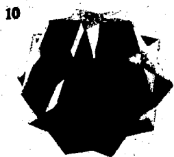
DODECADODECAHEDRON
