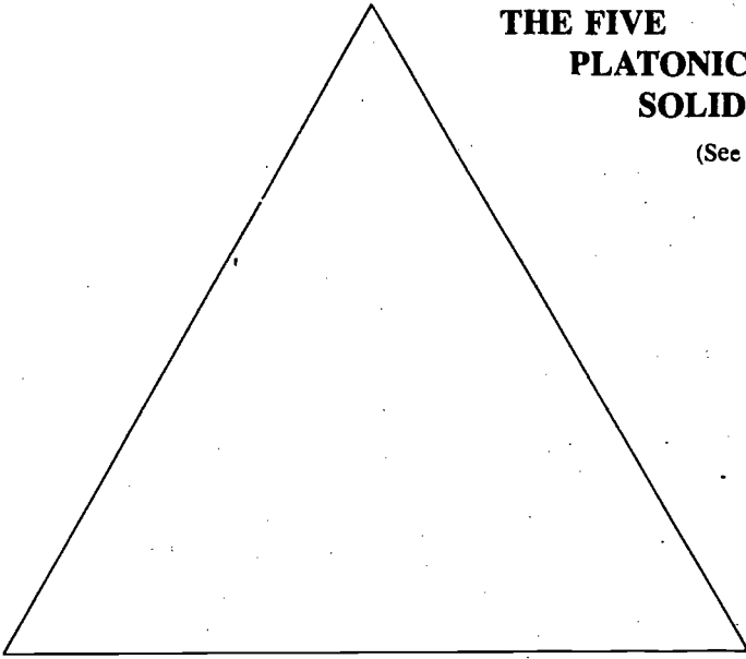
TETRAHEDRON
