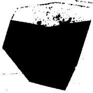
TRUNCATED TETRAHEDRON
