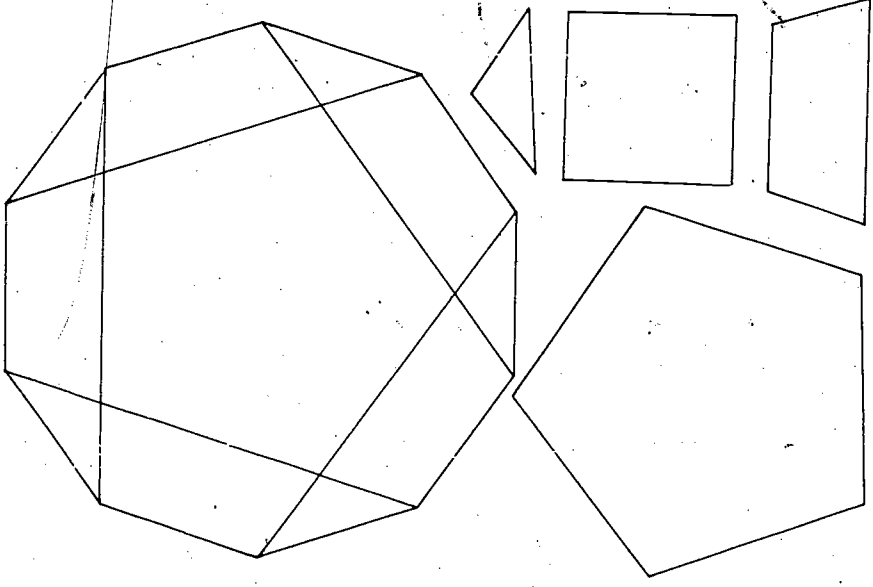
FIG. 41 (Model 8, p. 28)
