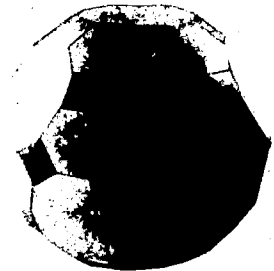
GREAT RHOMBICOSIDODECAHEDRON
