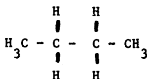
n-butane
