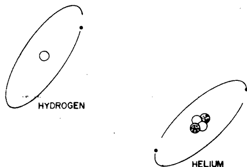
FIGURE 2.39a.—Atoms of the element hydrogen and the element helium.
