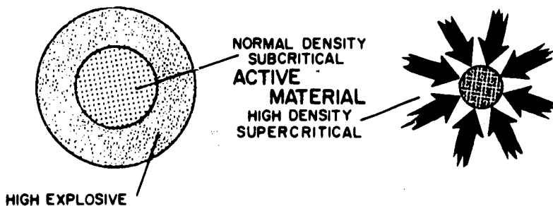
FIGURE 3.16a.—Implosion principle.
