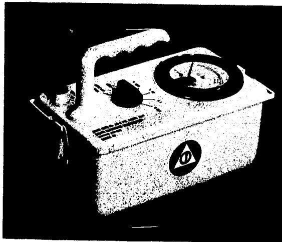
FIGURE 5.22.—CD V-715, high-range gamma survey meter.
