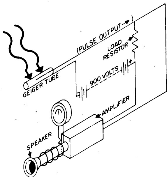
FIGURE 4.51.—Simplified circuit of a Geiger counter.
