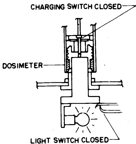
FIGURE 4.25c.—Charging position.
