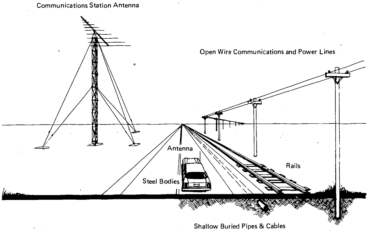
FIGURE 3.95.—EMP ENERGY COLLECTOR.
