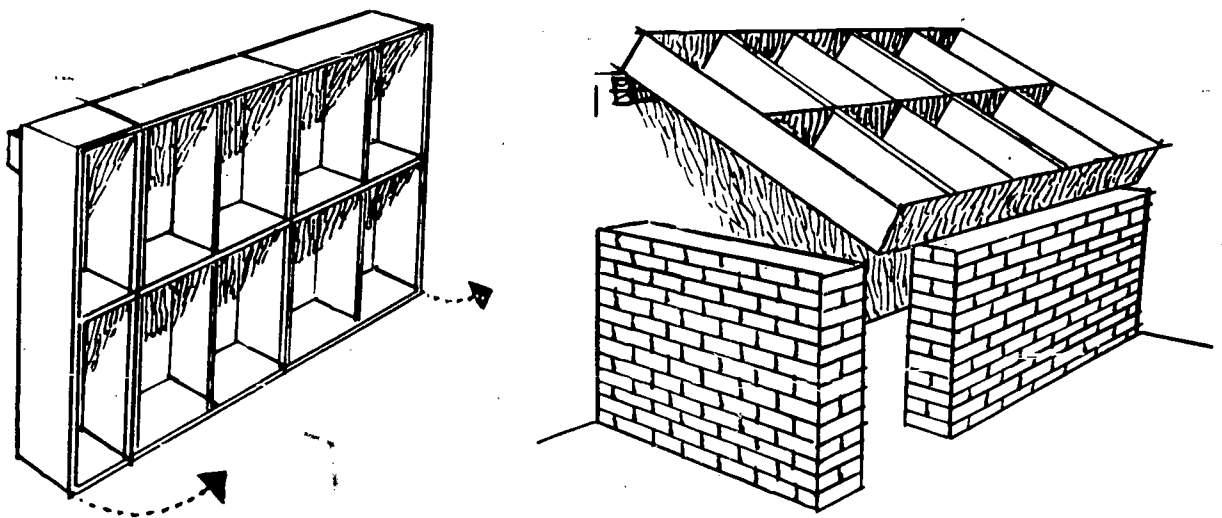
FIGURE 10.51.—Preplanned tilt-up storage unit plan E
