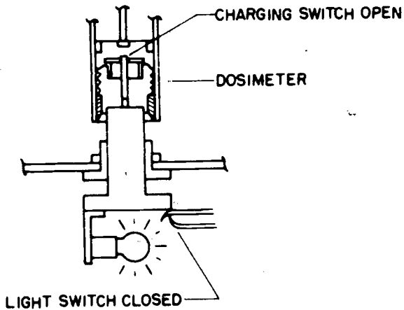
FIGURE 4.25b.—Reading position.
