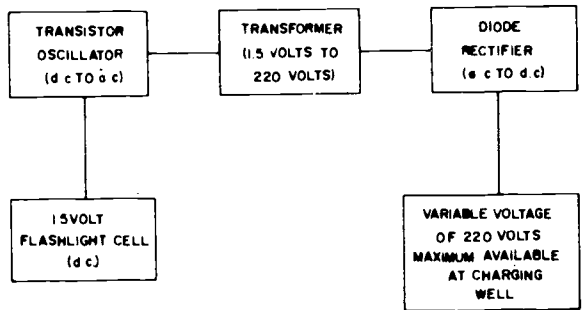
FIGURE 4.25d.—Simplified diagram of a CD V-750 dosimeter charger.
