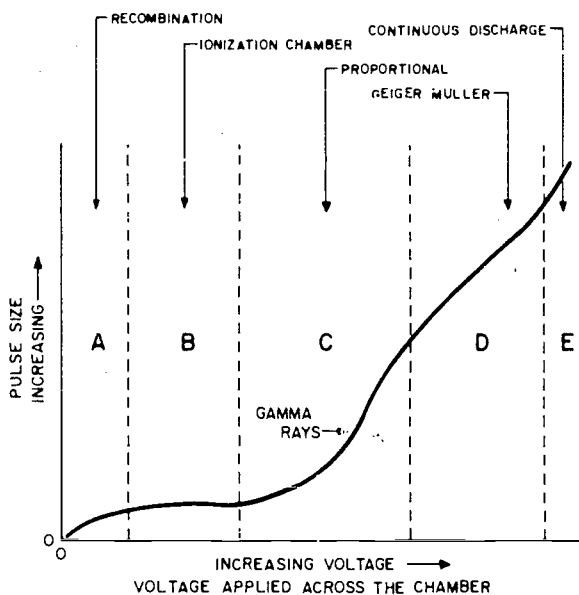
FIGURE 4.29—Pulse size vs. applied voltage for gamma radiation.
