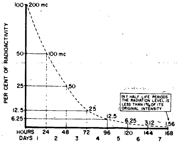
FIGURE 2.49.—Decay curve.
