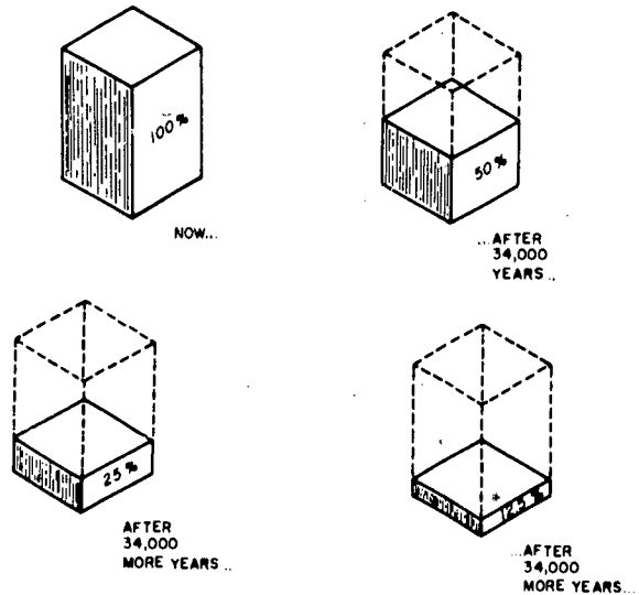
FIGURE 2.50.—Another view of half-life.
