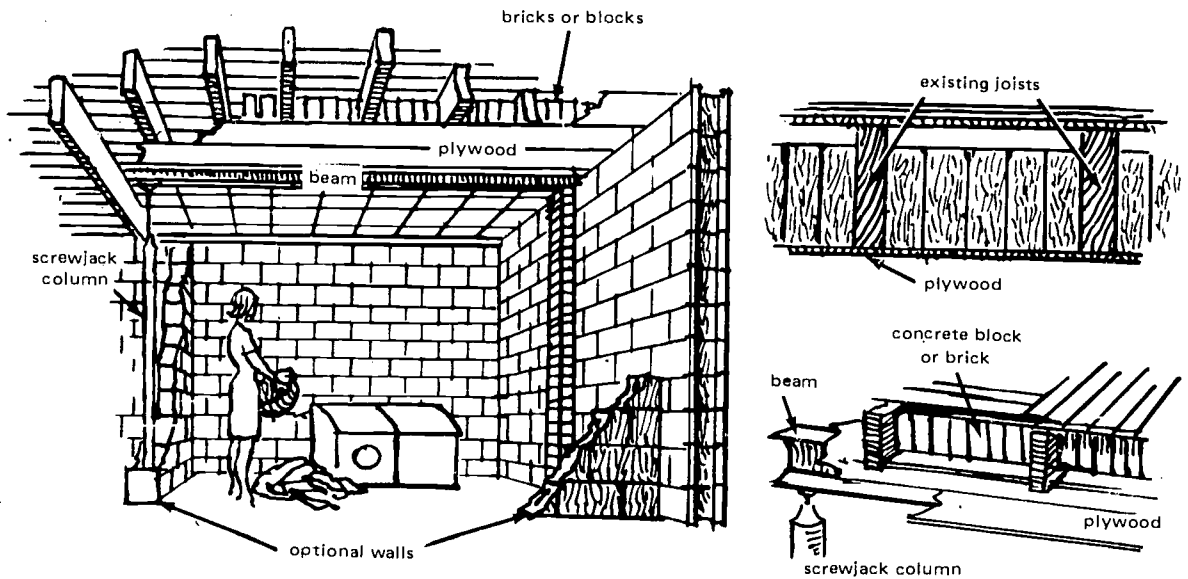
FIGURE 10.33.—Ceiling modification plan A.
