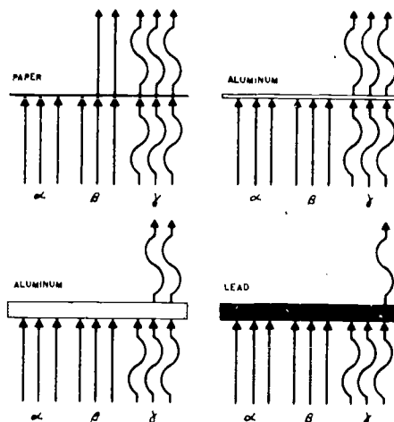
FIGURE 2.76.—Penetration-absorption of nuclear radiation.
