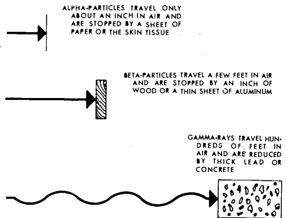
FIGURE 10.2.—Three kinds of nuclear radiation.
