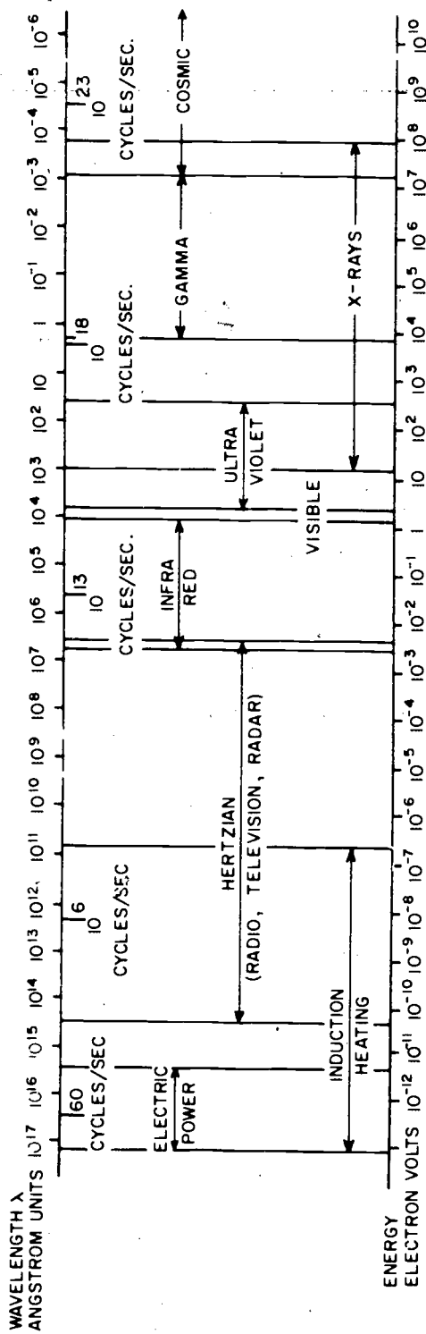
FIGURE 2.42.—Electromagnetic spectrum.
