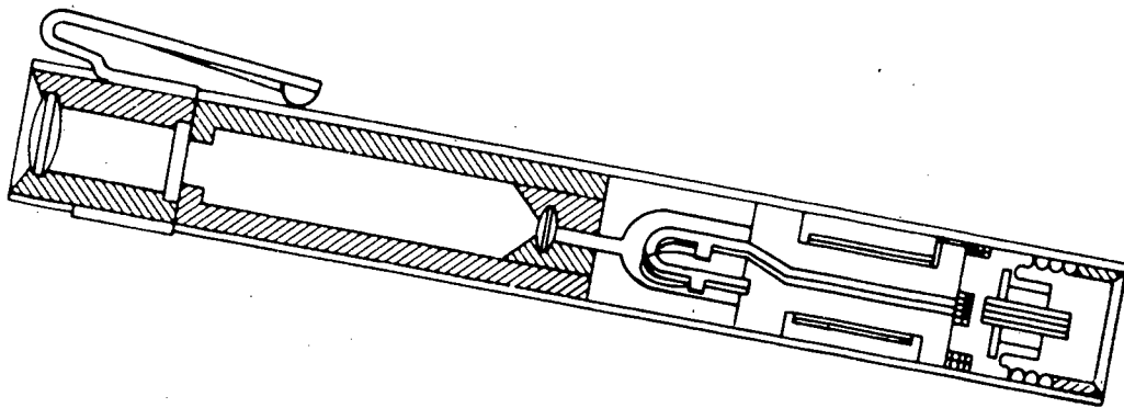
FIGURE 4.17.—Construction principles of an electrostatic self-indicating dosimeter.
