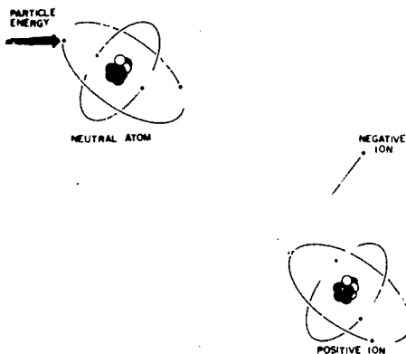
FIGURE 2.44.—Ionization.
