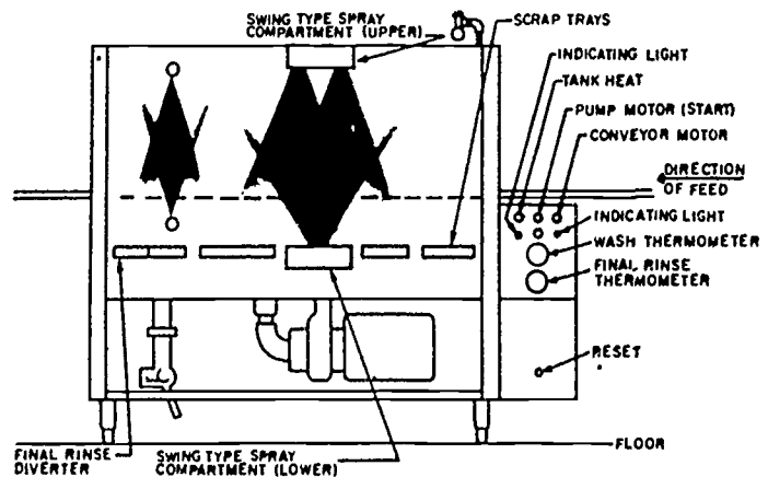
INSIDE OF WASHING MACHINE
