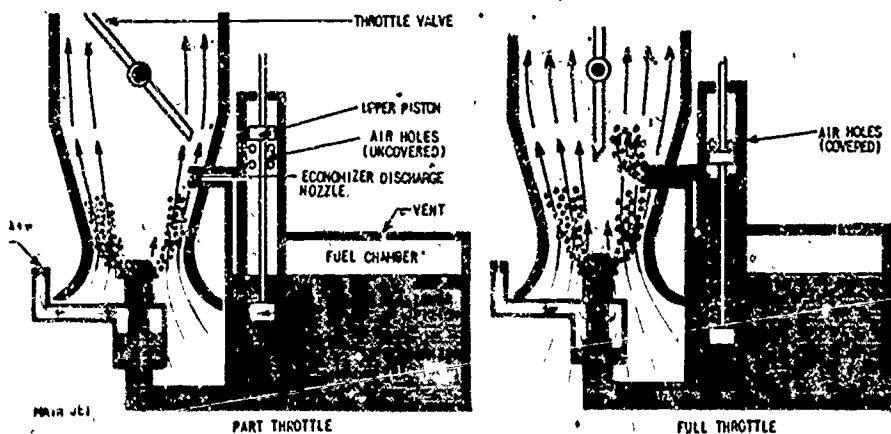
Figure 23. Operation of the piston type economizer system. Economizers come in several types, but all of them respond to the pressure differential produced when the throttle is opened.
