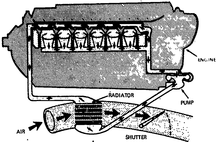
Figure 14. The liquid cooling system is more complex than the air cooling method, requiring plumbing, pumps, and radiators to keep the engine cool. Its performance is superior, however, on non-radial engines with many cylinders. This drawing traces the flow of the liquid coolant through the engine.
