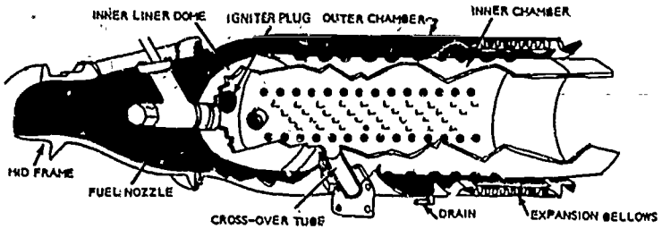
Figure 55. The combustion chamber of a jet engine includes an inner chamber, where the fuel is burned, and an outer chamber. Cooling air flow through the space between the two chambers. The igniter (spark) plug is used for initial ignition only, after which the flame is fed from chamber to chamber through the crossover tube.
