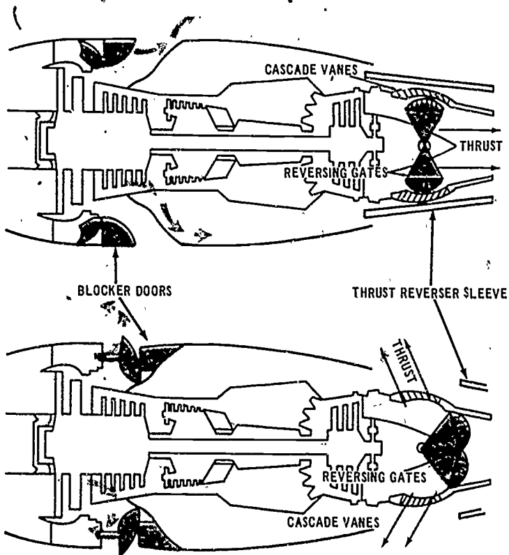
Figure 65. During normal flight, the airflow of the turbofan engine flows rearward without obstruction, as in the top drawing. When the fan and aft thrust reverser is in operation (bottom) blocker doors reverse the bypass air flow and reversing gates in the exhaust section turn the exhaust gases back through cascade vanes. With the thrust reversed, the reaction stops and the aircraft is braked.
