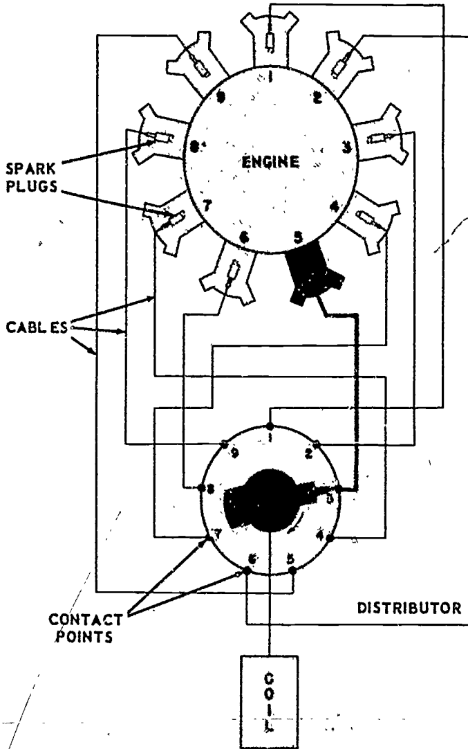
Figure 36. The electrical current goes from the magneto coil to the distributor, and from the distributor through the contact points to the spark plugs in the cylinders. As noted earlier, the cylinders do not fire in straight numerical sequence. The firing order of the cylinders is calculated to provide the smoothest flow of power from the pistons to the crankshaft.
