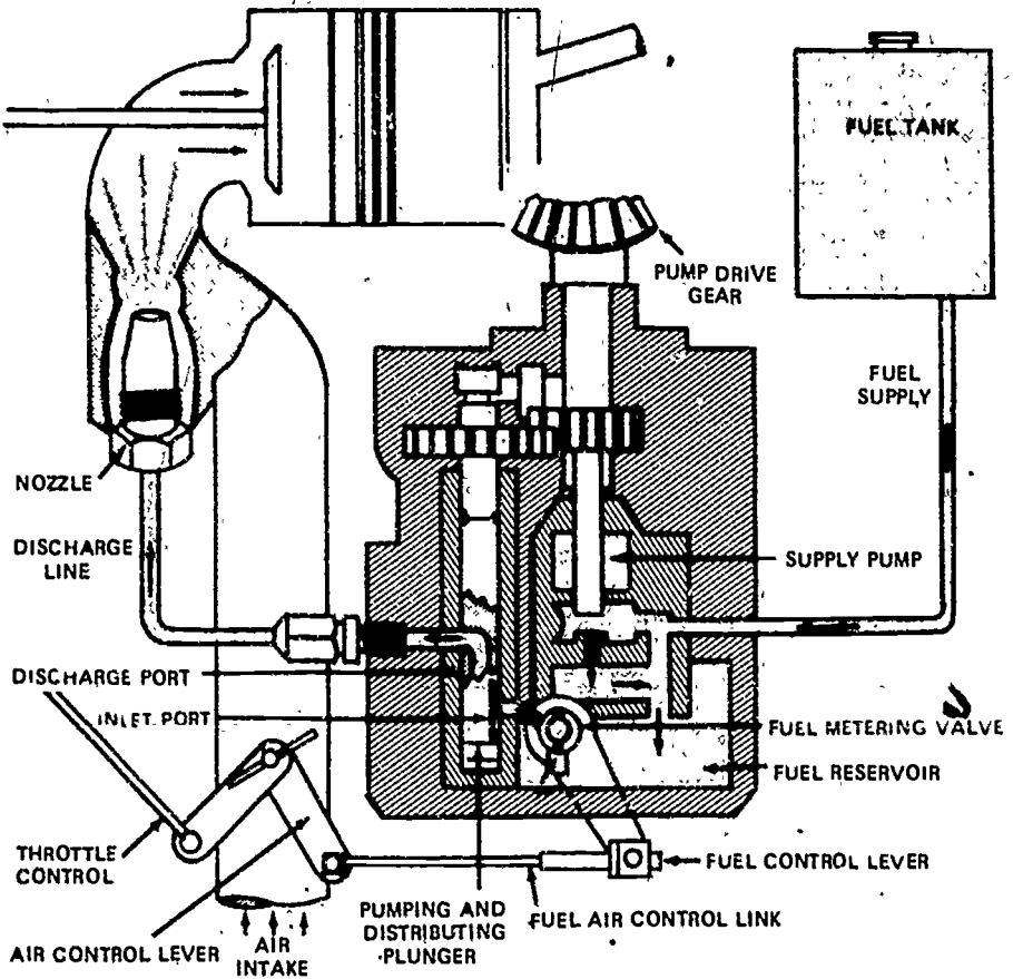
Figure 29. The intake metering system of fuel injection is used on smaller aircraft engines. It includes a mechanical linkage between the air metering throttle section and the fuel metering section and pump. Injection of the fuel charge occurs in the intake manifold just above the cylinder's intake valve, and not into the cylinder itself.
