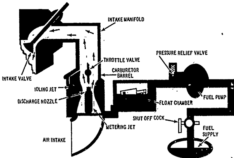
Figure 21. Outlined section shows how the carburetor works in connection with the other engine parts to feed fuel to the cylinder through the intake valve opening.
