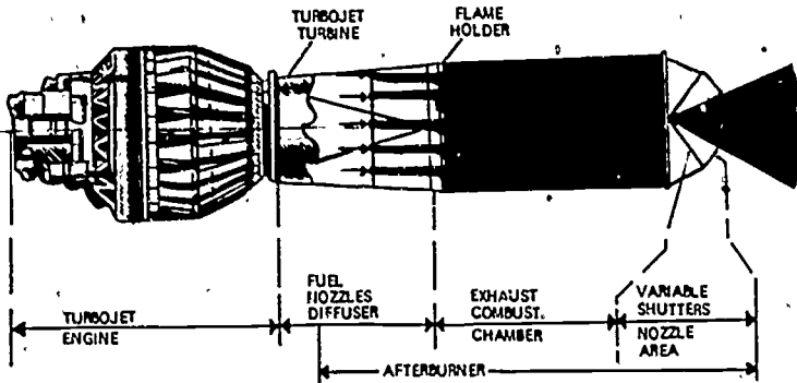
Figure 58. The afterburner, sometimes called the exhaust re-heat, provides additional thrust to an engine by injecting fuel into the high-temperature exhaust gases, mixing the fuel with the unburned oxygen in those gases, and burning the resulting mixture. When not operating, the afterburner acts as a tailpipe extension.
