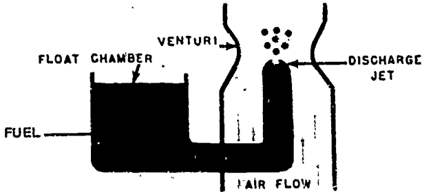
Figure 20. When the air flow speeds up to get through the carburetor's venturi (sometimes called a choke tube), pressure drops in the venturi, allowing fuel to be pushed through the discharge jet.
