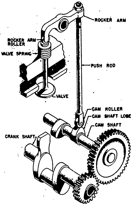
Figure 10. The camshaft, connected to the crankshaft through gears, moves a push rod in a timed sequence. The push rod operates a rocker arm. The rocker arm forces the intake and exhaust valves in the cylinder to open at the proper time in the four-stroke cycle. When the rocker arm lifts, the valves spring closed.
