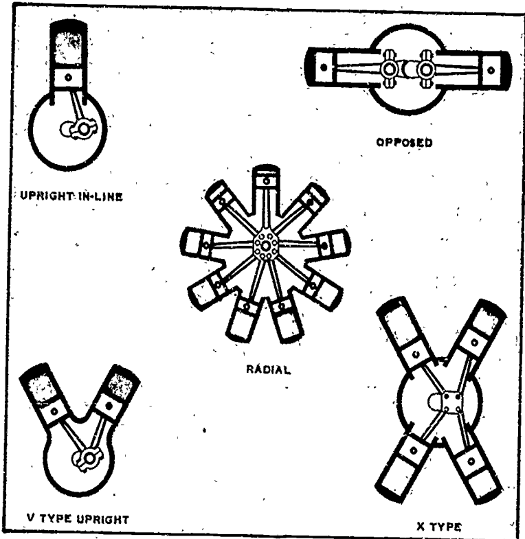
Figure 11. The most common arrangements of aircraft engine cylinders are shown here. Generally, the heavier and more powerful aircraft are fitted with radial engines, the smaller craft with the other types.
