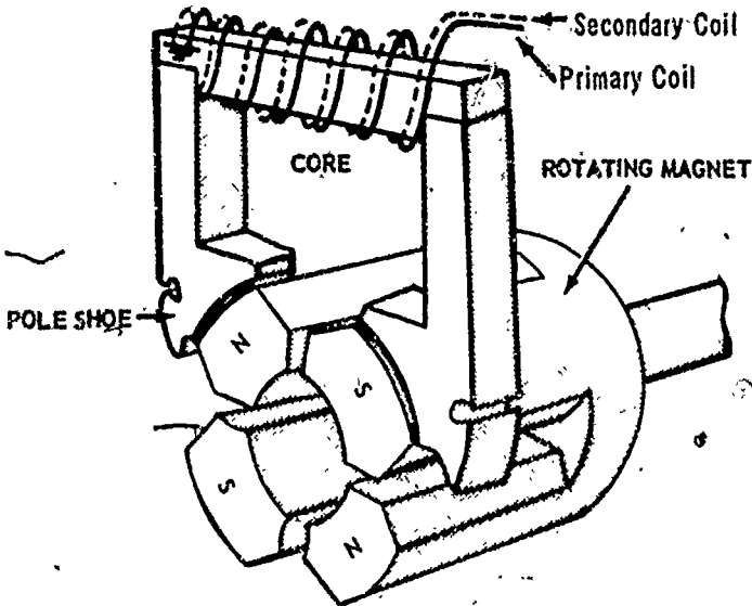
Figure 34. The movable magnets in the magneto spin between the ends of the conductor (poles and core), cutting many lines of flux and inducing an electrical current in the primary coil. The current is intensified in the secondary coil until it is strong enough to fire the spark plug and ignite the fuel, air charge in the cylinder.
