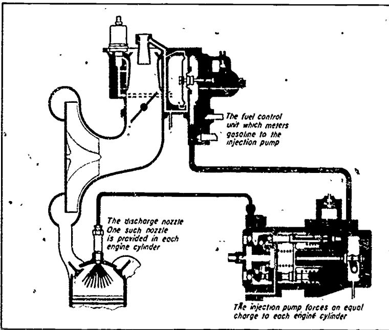
Figure 28. The mass air flow fuel injection system shown here features direct discharge of the fuel into the cylinder through the nozzle built into the cylinder head. The fuel measurement is controlled by a fuel control unit similar in operation to that of the pressure injection carburetor. Instead of delivering the fuel charge to the carburetor barrel, this system sends it to an injection pump, which divides the charge and distributes it to individual cylinders.
