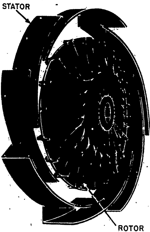
Figure 50. The centrifugal compressor used in the early models of the turbojet engine, hurled the air outward from the whirling rotors onto the stationary stators, and the stators guided the compressed air to the combustion section.
