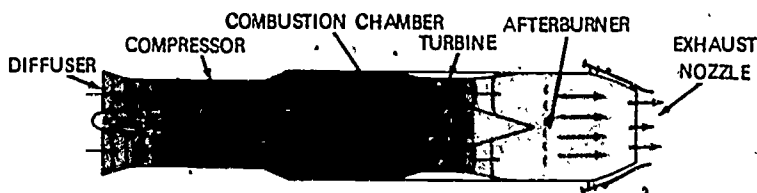
Figure 49. The turbojet engine features an air compressor which is operated by a turbine, which in turn is powered by high-velocity exhaust gases on their way to the tailpipe. The engine in this simple illustration is equipped with an afterburner for extra power.
