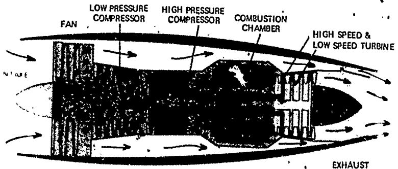
Figure 61. The turbofan engine is a true jet propulsion engine, since its principle thrust is produced by exhausting gases. The turbofan is designed to move great volumes of air, as the propeller does, but it does not have the propeller's tip speed limitations.
