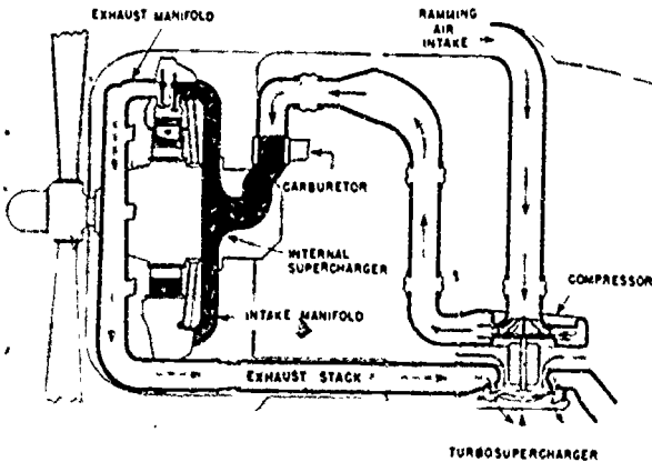
Figure 25. The supercharger's system external fan compresses intake air before it reaches the carburetor, and the fuel impeller further compresses the air mixture before it enters the intake manifold. The stronger charge means extra power in the engine.
