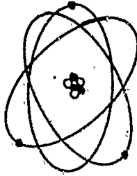
Figure 30. The atom is a miniature planetary system. Its nucleus is made up of protons and (in all elements except hydrogen) neutrons. Electrons orbit this nucleus.
