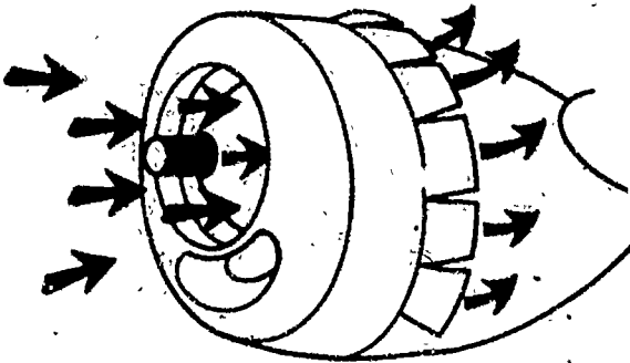
Figure 13. The cowling structure of an air-cooled engine is designed to get the cooling air to where it is needed and keep the air circulating around the cylinders. The pilot can control the air flow by opening or closing the cowl flaps.
