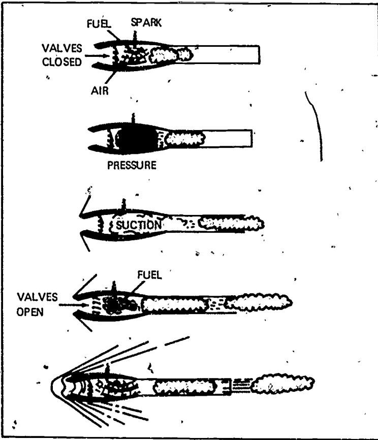
Figure 48. The pulsejet is of strictly historical interest. Cheap and simple, it was one of the earliest jet engines to be used operationally, but it was quickly abandoned when the turbojet was developed. The pulsejet's characteristic sound was responsible for the nickname "buzz bomb" being given to the V-1 missile used by the Germans in World War II.
