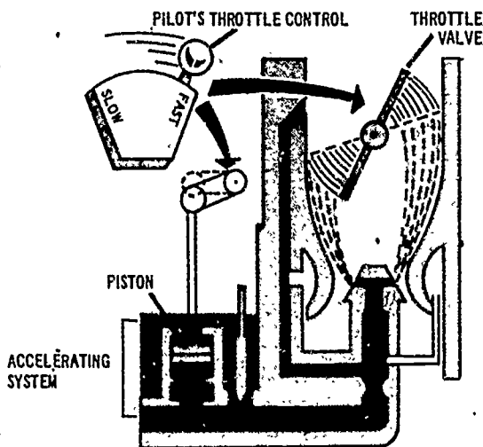
Figure 24. When the throttle is suddenly thrown open, the piston in the accelerating system pushes out extra fuel into the discharge stream to prevent "leaning" of the fuel/air mixture.
