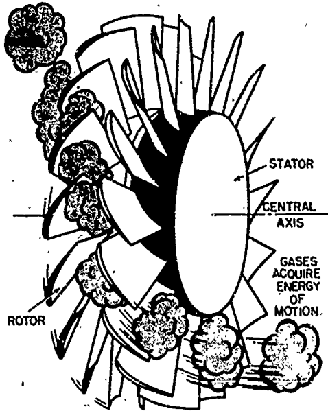
Figure 52. In the axial compressor, the airfoil-shaped rotor blades hurl the intake air rearward, and not outward as in the centrifugal compressor. The stator blades in the axial compressor are also airfoil-shaped.
