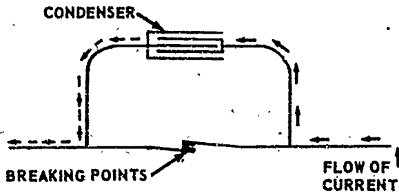
Figure 35. The condenser absorbs the self-induction ("inertia") current and prevents undesirable arcing when the breaker points open. It then discharges that current back to the primary coil, helping accomplish flow reversal.
