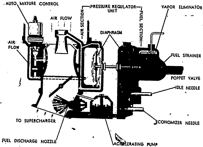
Figure 27. The pressure injection carburetor uses a system of diaphragms in the measurement of fuel. The diaphragms respond to the air flow and to the force of the fuel, which is pumped into the carburetor under pressure. The pressure regulating unit of this carburetor includes the air section and the fuel section of the metering system.
