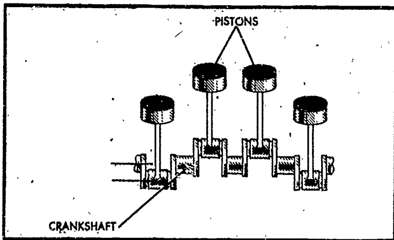
Figure 9. The piston is connected to the crankshaft by connecting rods. The throws, or bends, in the crankshaft are staggered to obtain a continuing turning motion from the piston power.
