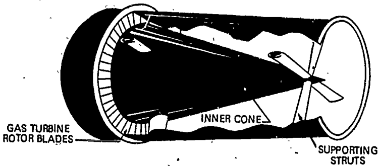
Figure 57. The exhaust section of the engine straightens the exhaust gas flow and sends it out the rear of the engine in a concentrated stream. This is the business part of jet propulsion.
