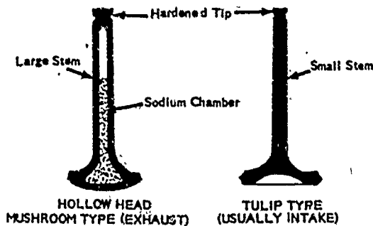
Figure 15. The cut away drawing of engine valves shows two different types of valves in use today. The sodium chamber inside the hollow head mushroom valve helps to get the high heat of the exhaust gases away from the valve head quickly.
