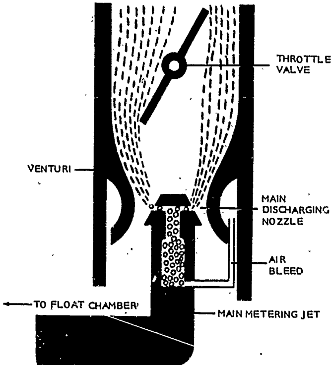
Figure 22. The throttle valve regulates the opening in the carburetor barrel in response to the pilot's movement of his throttle controls. The air bleed helps the fuel to flow freely out the discharge nozzle.
