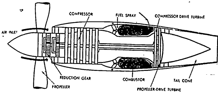
Figure 60. The turboprop engine combines the advantages of the gas turbine powerplant with the efficiency of the propeller to get a relatively quiet, cheap, and powerful propulsion system. It is not strictly a jet propulsion system.
