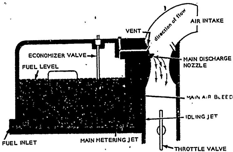
Figure 26. The downdraft carburetor is essentially the same as the updraft carburetor, except that the air intake is at the top instead of the bottom, and the air flows downward instead of upward through the carburetor barrel.
