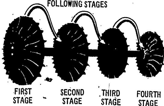
Figure 51. In the multi-stage compressor, the stators direct the compressed air onto the rotors of the next compressor stage for more air compression. The last stage, of course, sends the air into the combustion chambers.
