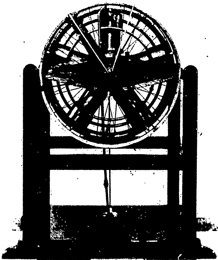
Figure 4. Charles Manly's engine was powerful and efficient enough to drive the Aerodrome, but could not overcome mistakes in the aircraft itself. A five cylinder radial engine, it used a bicycle wheel for a flywheel.
