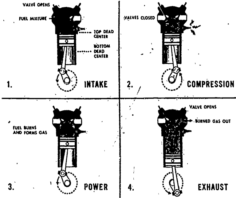
Figure 8. The movement of the piston up and down in the cylinder transmits energy to the crankshaft, which turns the propeller. The process that supplies power to the piston is the four-stroke engine cycle explained here.
