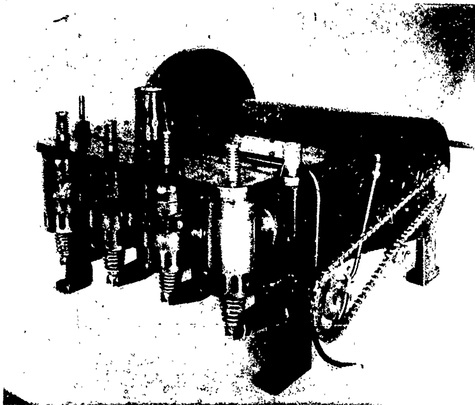
Figure 5. This engine powered the Wright brothers aeroplane at Kitty Hawk in December 1903. Although inferior to the Manley engine, it was successful because it propelled a successful aircraft.
