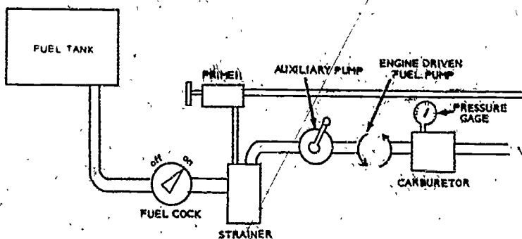
Figure 18. Fuel system with the pumps arranged in series. The auxiliary pump is used during starting of the engine, during take-off and landing, during high-altitude flight (above 10,000 ft), and in emergency operations.
