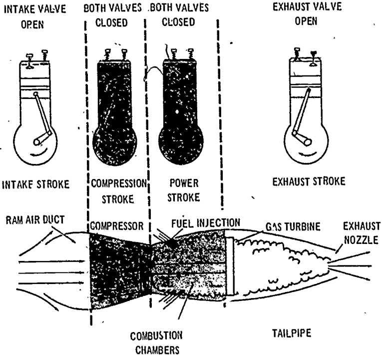
Figure 45. The power production cycle in the jet engine may be compared with the four-stroke cycle of the reciprocating engine. Like the reciprocating engine, the jet goes through intake, compression, combustion, and exhaust. But the exhaust is the force that makes the jet plane go.
