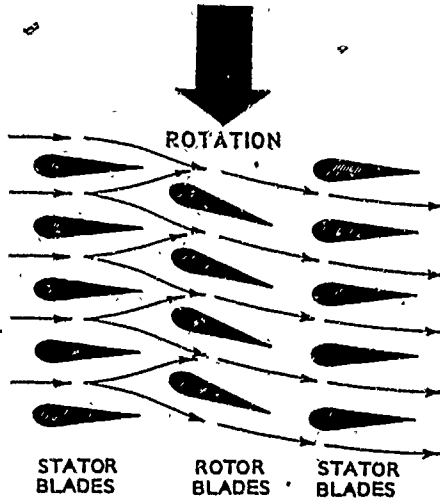
Figure 53. The stators in the axial flow compressor straighten the airflow and guide it either to the next stage of rotor blades or on to the combustion chambers. One stage of an axial flow compressor consists of a row of rotors and a row of stators.
