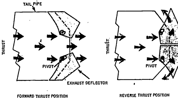
Figure 66. In the turbojet's simple tailpipe thrust reverser, the exhaust deflector acts as a part of the tailpipe when in the forward thrust position (left), but swings shut when activated and deflects the exhaust gases back toward the front of the aircraft.
