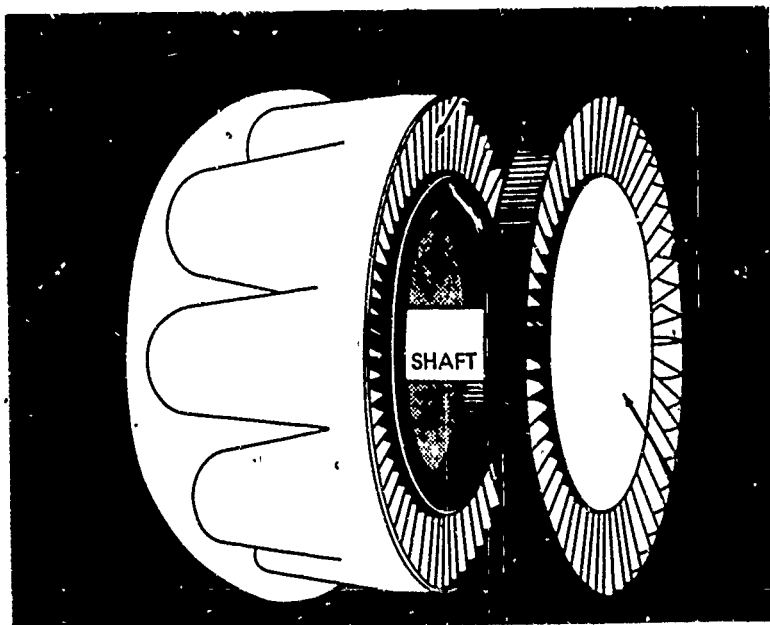
Figure 56. As with the compressor, a single stage of the turbine consists of a row of rotors and a row of stators, but in reverse order. The stators direct the exhaust gases onto the rotor blades, causing the rotor wheel to turn. The front end of the turbine shaft connects to the compressor.
