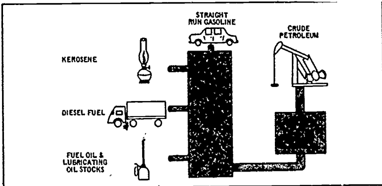
Figure 16. In the fractional distilling process, crude oil is heated to a moderate temperature under normal atmospheric pressure. The vapors from the oil are condensed to liquid compounds. The highly volatile fluids are vaporized first and the fuels with higher boiling points later.
