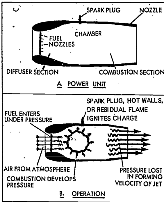
Figure 46. The ramjet, sometimes called the "flying smokstack," is the simplest jet engine in use today. Its air supply is compressed by the ramming action of the engine instead of by a mechanical compressor.
