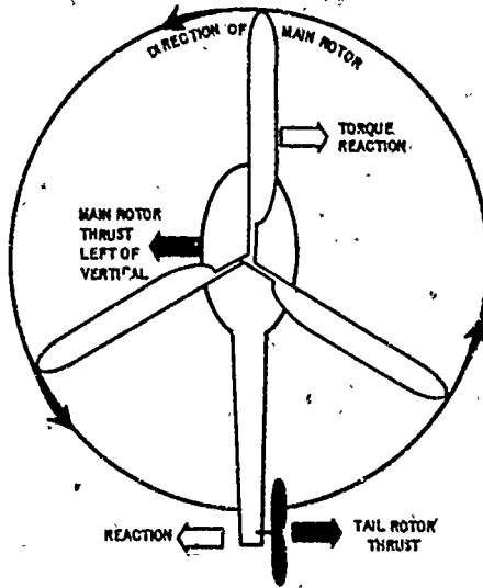
Figure 63. A tail rotor works similarly to a propeller to offset the torque from the main rotor. Reaction to the tail rotor's thrust operates in the opposite direction from the torque of the main rotor. This keeps the helicopter from spinning. Helicopters with two rotors spin the rotors in opposite directions, offsetting each other's torque.
