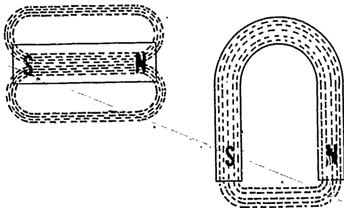
Figure 32. Bending a bar magnet into horseshoe shape makes the magnet stronger by concentrating the lines of flux.
