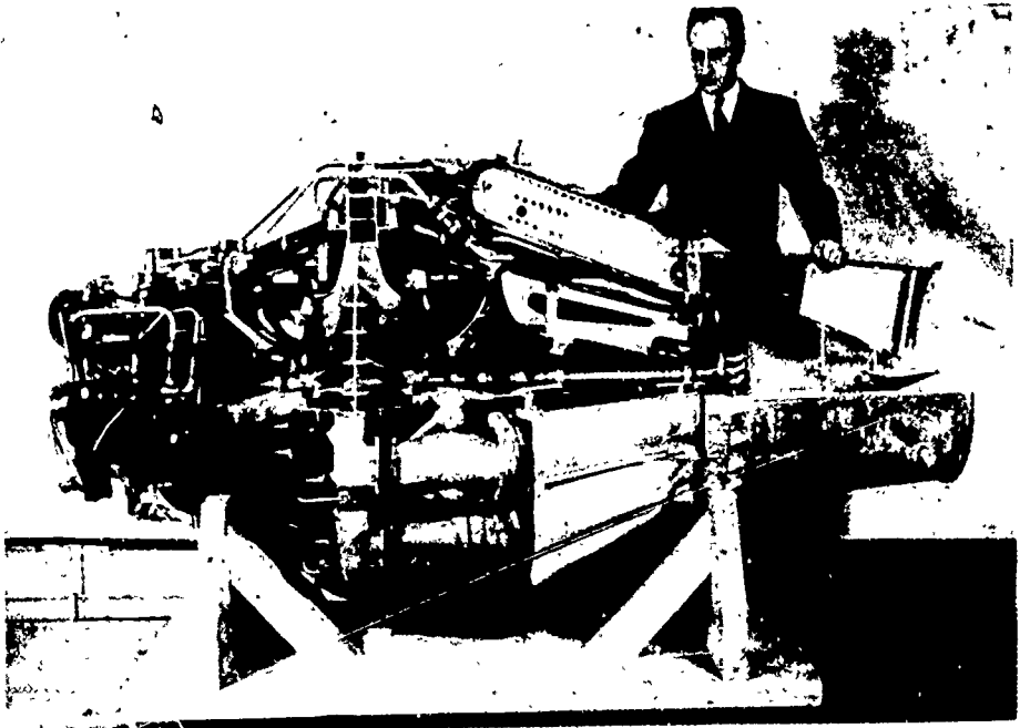
Figure 6. This jet engine powered the first operational American jet plane, the P-80. Developed by General Electric for the Army Air Force, the engine provided 4,200 pounds of thrust.
