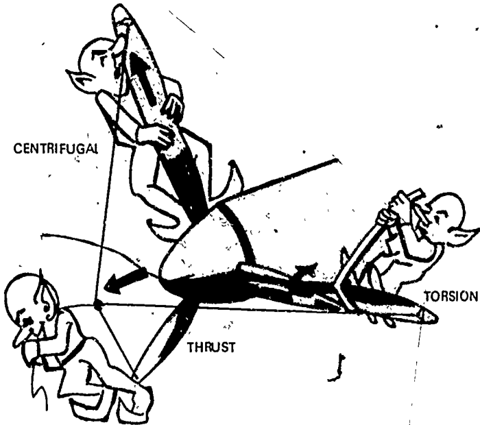
Figure 43. Three main forces act on the propeller in operation. The thrust force tends to pull the blade forward, much as the action of lift on a wing. Centrifugal force tends to pull the blades outward as a result of the turning motion. Torsion tends to twist the curve out of the blade and straighten it.
