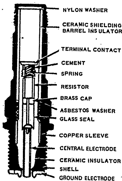
Figure 37. The spark plug must be carefully built to stand up under the stresses it is subjected to. Its job is to feed the electrical current to the cylinder. The fuel/air charge is ignited when the electrical spark jumps from the central electrode to the ground electrodes.
