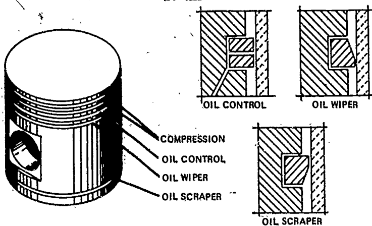
Figure 38. The piston is equipped with compression rings, which prevent gas leakage past the piston during engine operation, and oil rings, which control the amount of lubricant supplied to the cylinder walls and keep excess oil out of the combustion chamber. Oil flows to the cylinder wall through a hole in the oil control ring, and the wiper ring scrapes the excess away.
