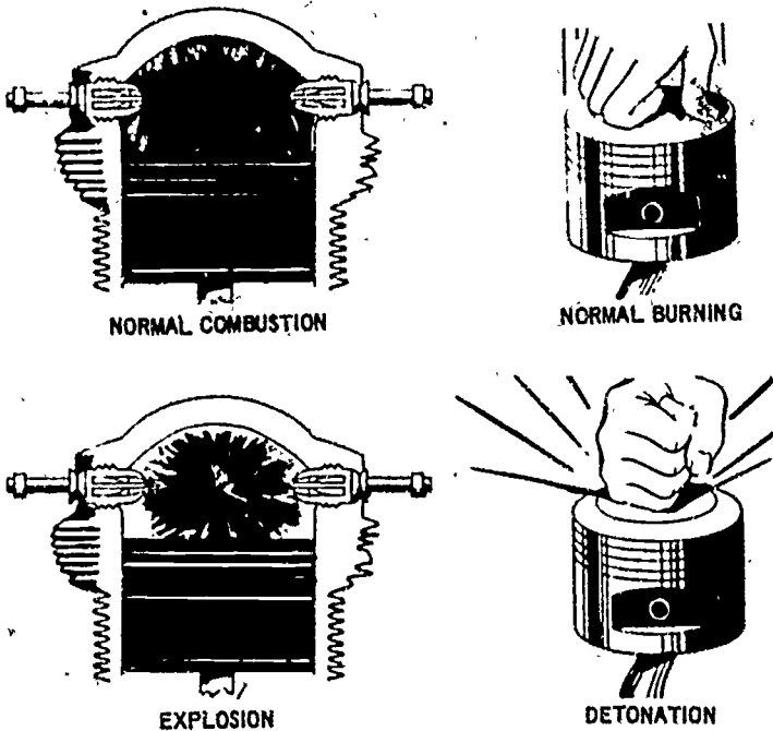
Figure 17. Under conditions of normal combustion, downward pressure on the piston is smooth and even. When detonation occurs, the pressure is sudden and violent.
