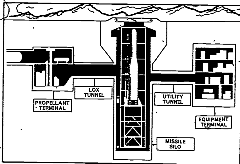
Figure 3. A Titan launch station, hard site.
