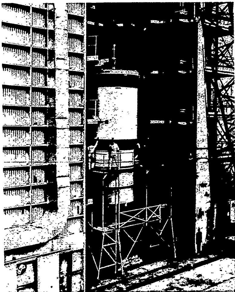
Figure 31. A 1.2 million-pound thrust solid rocket being assembled. Rockets of this size are used in pairs as the booster stage of the Air Force Titan III- and -D.
