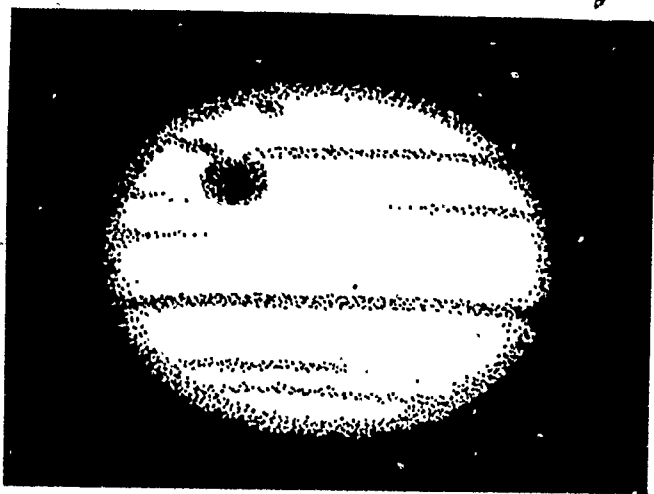
Figure 40. Diagram of Jupiter, showing the "Great Red Spot" and the bands.
