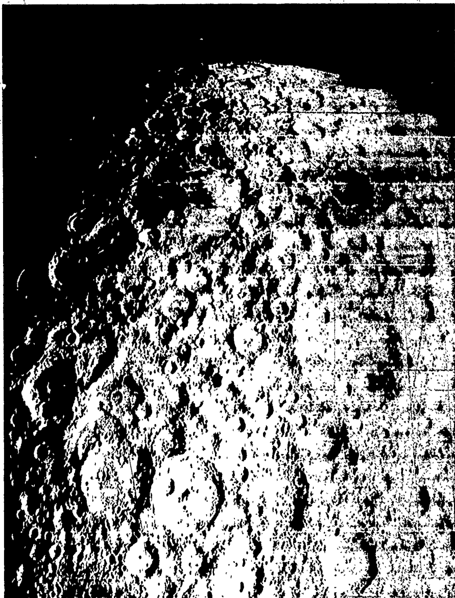
Figure 23. Luna Orbiter II was located about 900 miles above the Moon when it turned its wide angle lens on the southern half of the Moon's hidden side.
