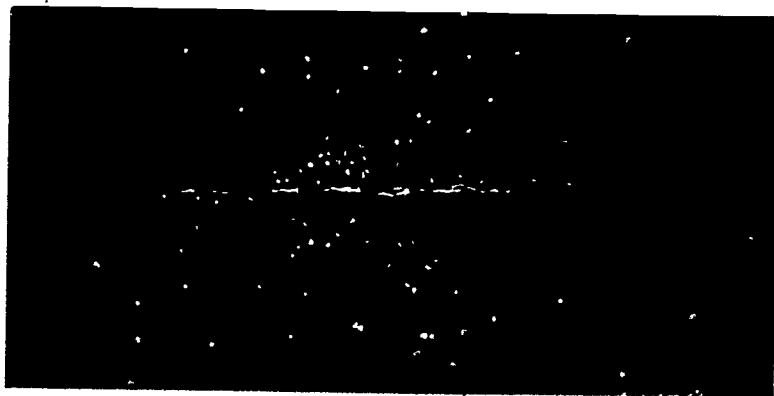
3: Side view of a Population II star system.
