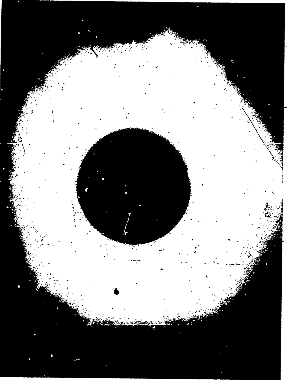
Figure 38. Solar eclipse of 7 March 1970, taken at Mishuatlan, Mexico. The Moon totally blocked out the Sun for three and one-half minutes.
