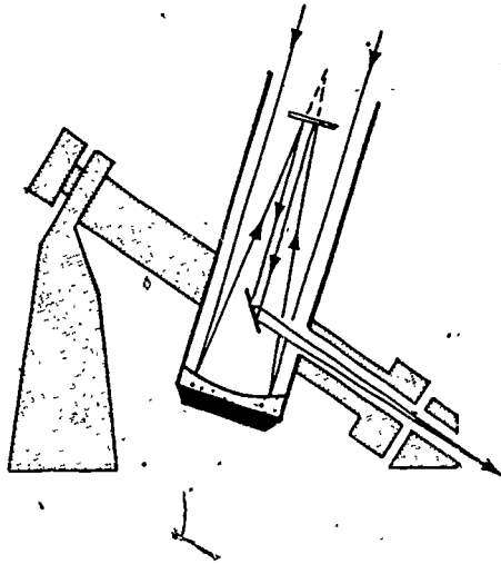
Figure 33. Still another type of telescope uses the so-called Coudé focus. This type of focus is quite similar to the Cassegrainian focus with one major exception. It uses a third slanting mirror near the bottom of the tube to deflect light rays Newtonian fashion through the side of the instrument tube.
