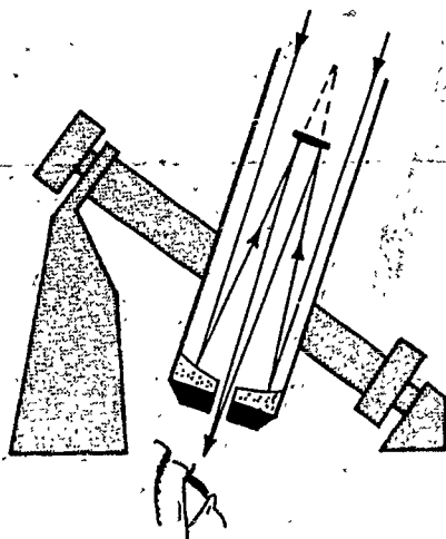
Figure 32. Another type of reflecting telescope uses a large, concave primary mirror at the bottom of the instrument tube and a smaller, concave secondary mirror near the top of the tube. The large mirror reflects concentrated light to the small mirror which further concentrates the light rays and reflects them back through a small hole in the large mirror. The observer is located behind this hole at the bottom of the instrument tube. This arrangement is known as the Cassegrainian focus.
