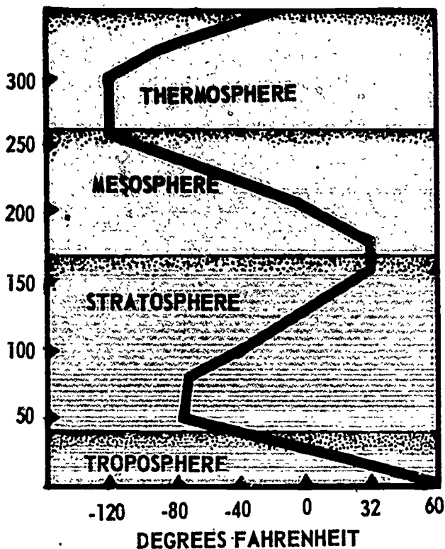
Figure 9. Layers of the atmosphere showing temperature variations.
