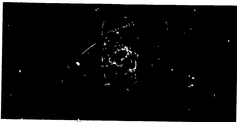
1. Orbits of stars classified as Population I stars.
