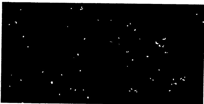
2. An oblique view of Population I star orbits in outer arms of spiral galaxies.
