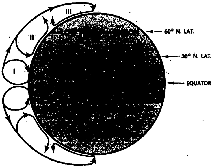
Figure 10. Global wind circulation.
