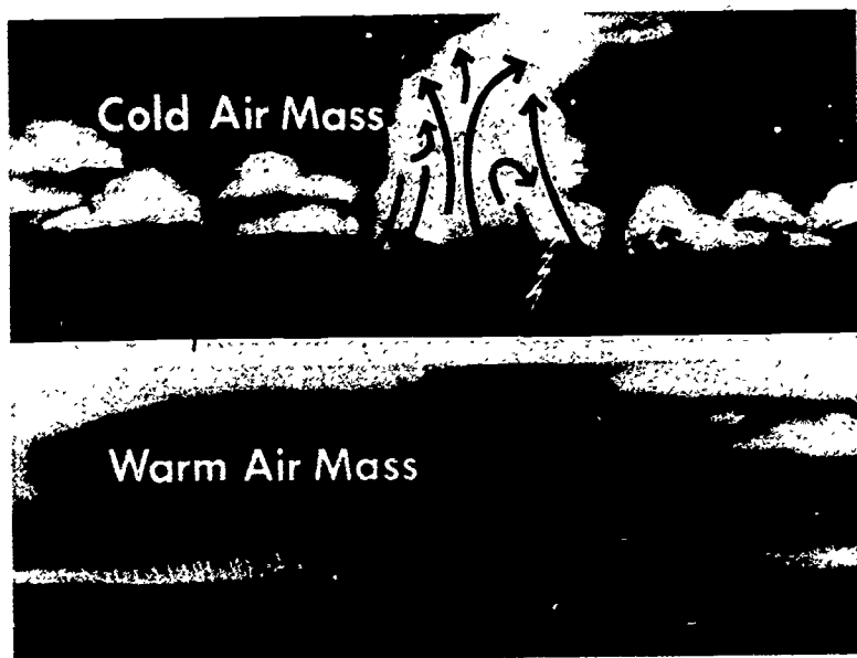
Figure 12. Characteristics of a cold and a warm air mass.
