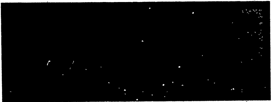
Figure 4. The light year is commonly used for measuring interstellar distances.
