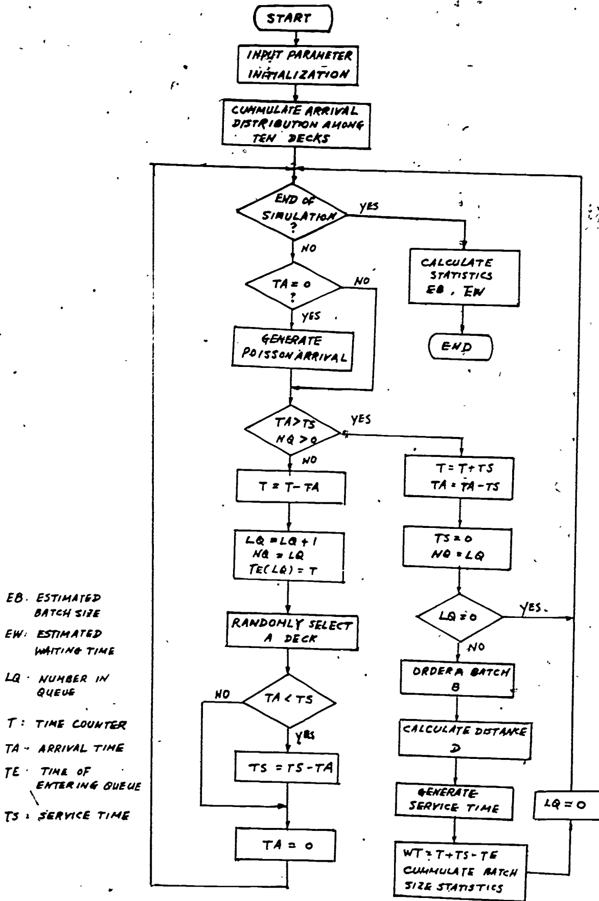
Simulation Flow Chart 35
