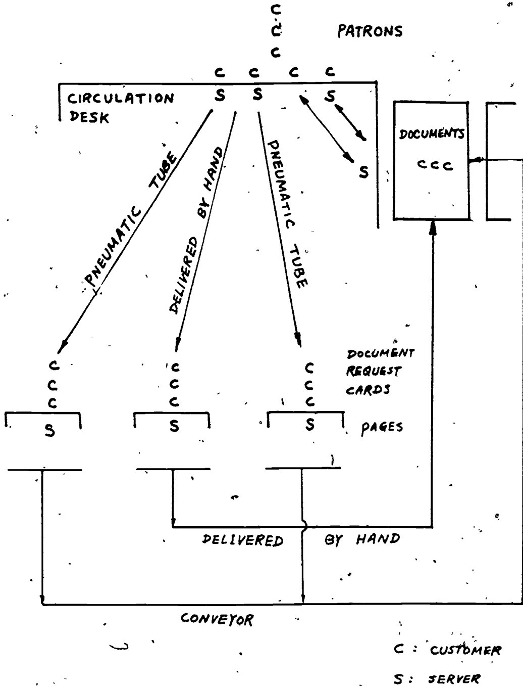
Figure 1 The Document Retrieval System as a Series of Queueing Systems
