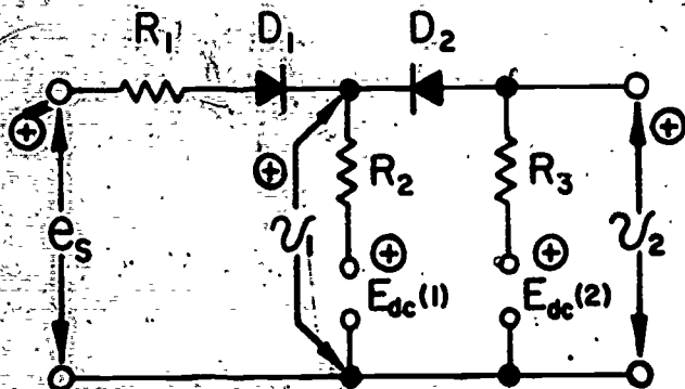
FIG. 3 A multiple-diode circuit (Orientation of diodes may also be reversed.)
