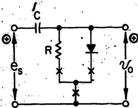
FIG. 3 A biasing voltage, or a pulsed voltage, may exist in one of the \times points in the circuit. The diode may also be oppositely oriented.
