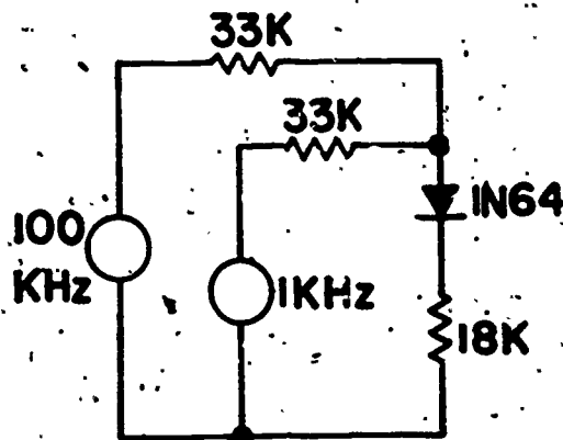
Figure 3. Modulating circuit without filtering.
