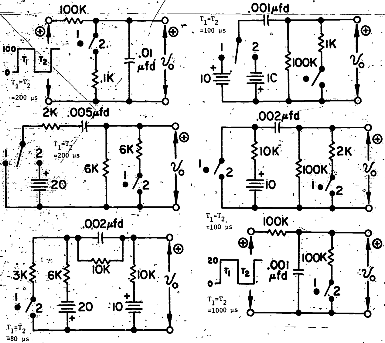
FIG. 1. Sample problems to illustrate resistance switching in RC circuits under defined switching conditions. The objective is to evaluate a steady-state cycle for the output voltage.
