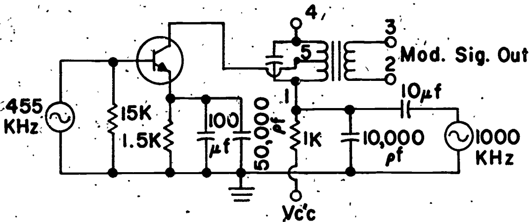
Figure 6. Collector modulation with transformer coupling to output
