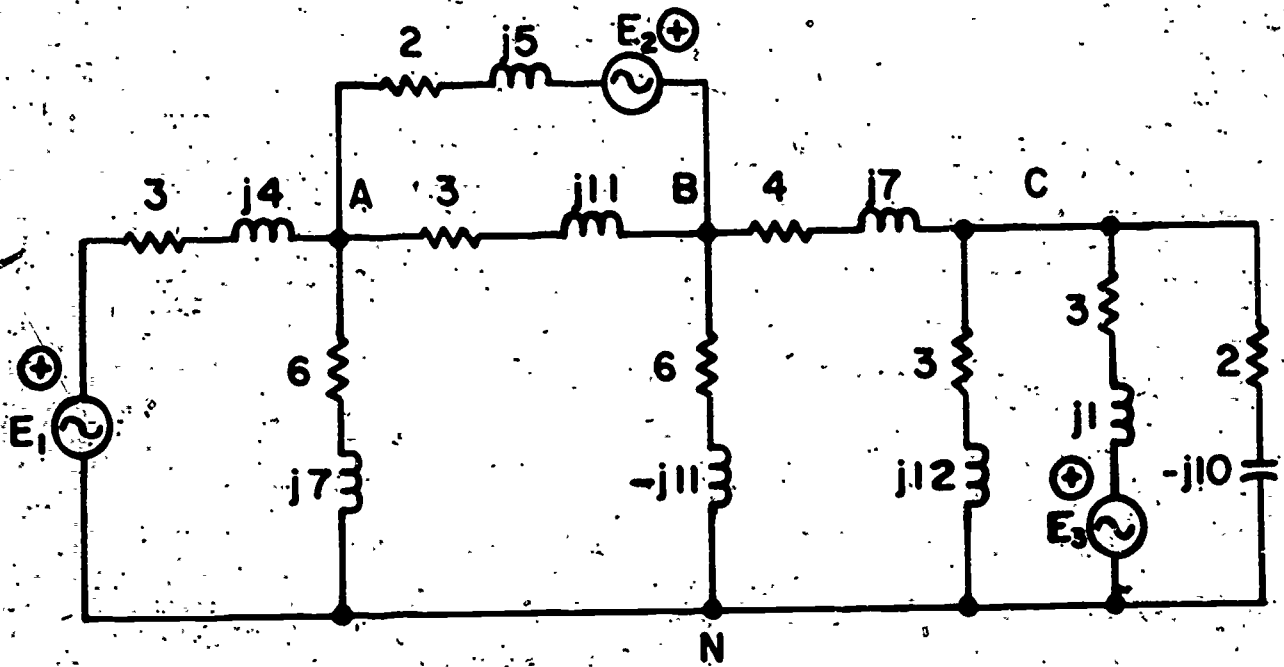
COMPLEX NETWORK
