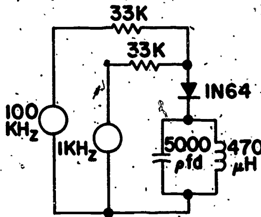
Figure 4. Non-linear mixing, or modulating circuit, with tuned load.
