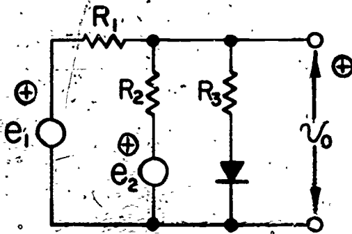
FIG 3 The given circuit model
