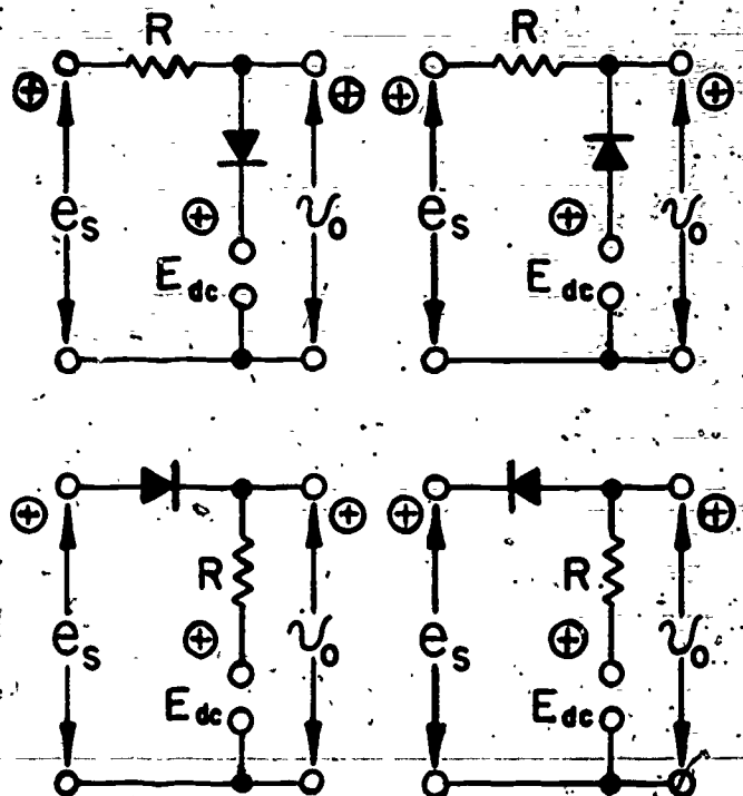
FIG. 1 The four basic diode clipping circuits
