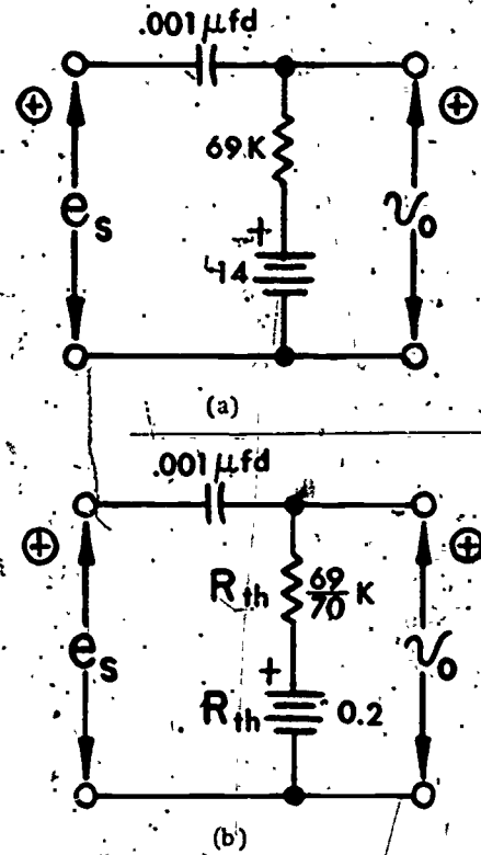
FIG 2 The two equivalent circuits, (a) The diode nonconducting and (b) The diode (ideal diode considered) conducting. Notice the application of Thevenin's theorem for circuit (b) and the advantage of the attenuation factor in find v_o from v_o . Notice, also, that the time-constant and the asymptotical values are easily determined for v_o in the first circuit and for v_o in the second circuit. Simply attenuate to get the true asymptotical value for v_o in the second circuit.
