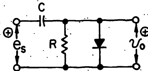
FIG. 1 The Basic R-C diode circuit (The diode may also be oriented in opposite direction.)
