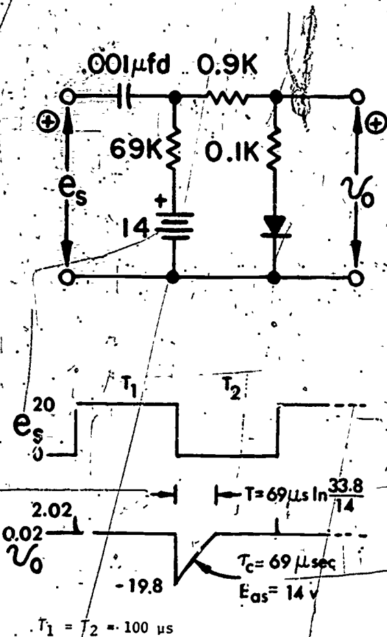
FIG 1. The given circuit model
