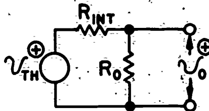
Circuits for Experiment 7
