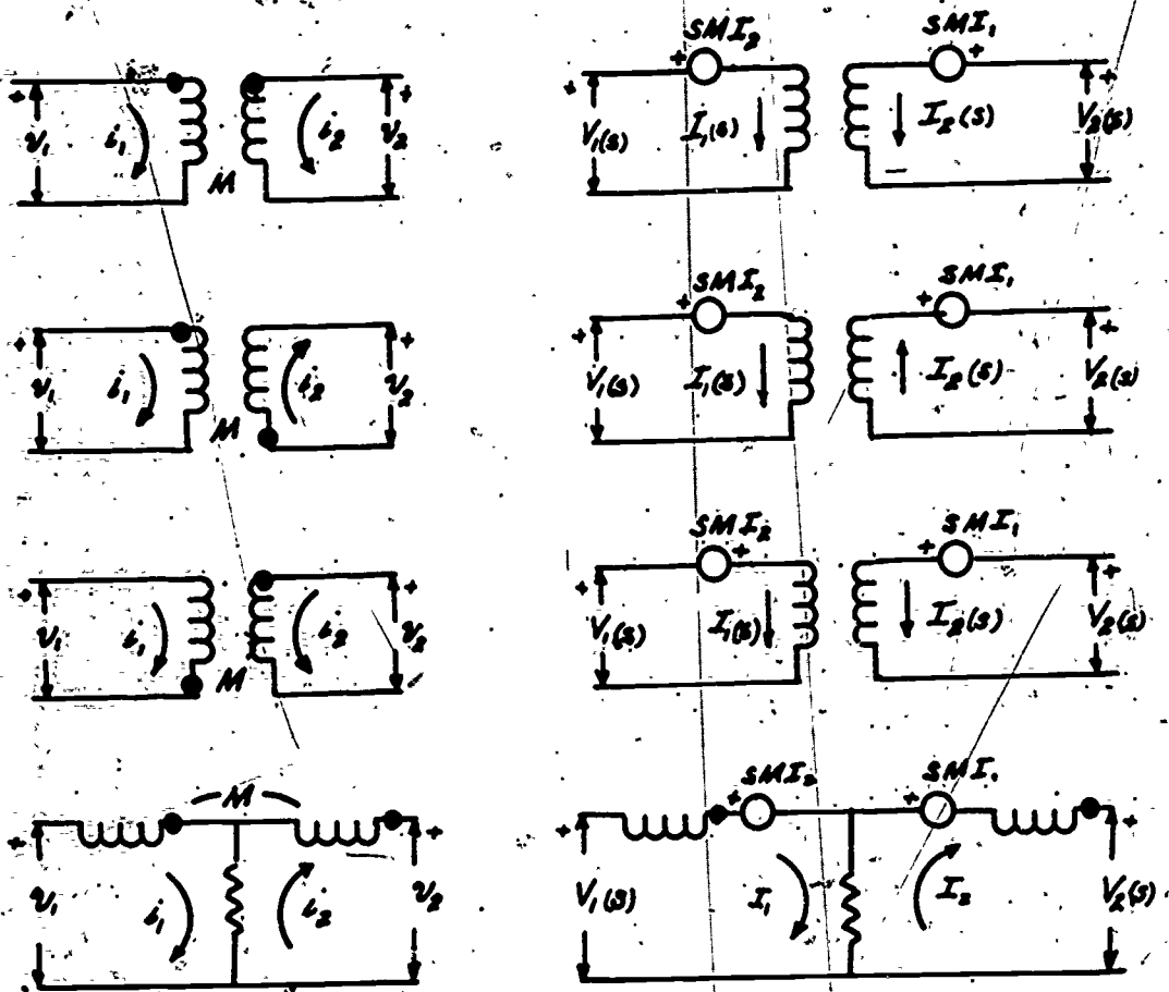
Fig. 1 Coupled circuit models showing dependent sources (right-hand column) of mutual inductance. S-operator is shown. Could use j\omega as well for sinusoidal steady-state analysis.
