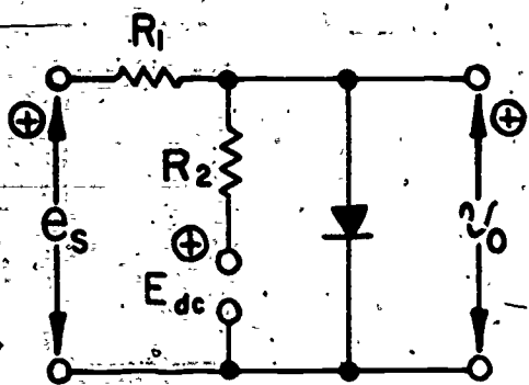
FIG. 2 A multiple-loop single diode circuit
