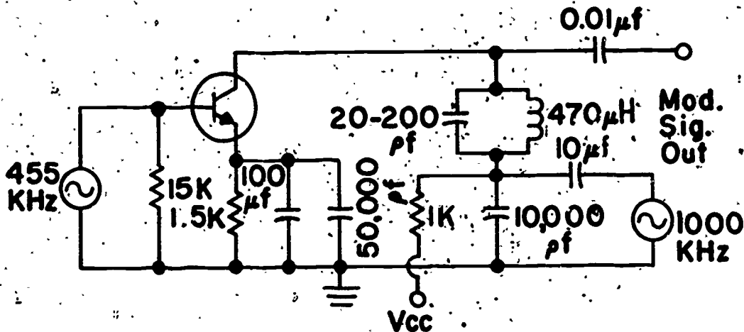
Figure 5. Circuit for simple collector modulation.
