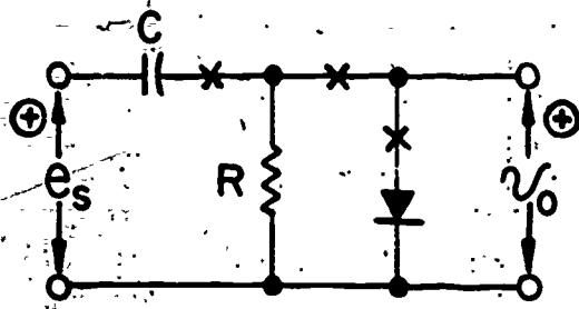
FIG. 2 An additional resistance may exist in any one or more of the \times points in the circuit (usually not all three, however, in the same circuit). The diode may be oppositely oriented.
