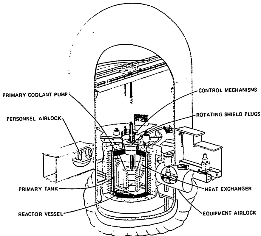
Schematic of the Experimental Breeder Reactor No. 2.
