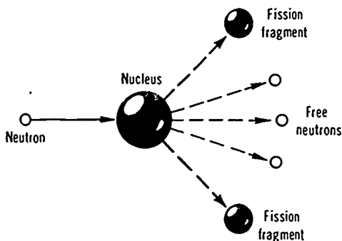
A fission reaction.
