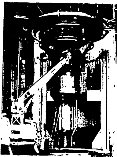
Model of an advanced Nerva engine intended to produce 60,000 to 75,000 pounds of thrust and approximately 1500 megawatts of power.
