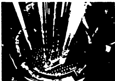
The core of the Experimental Breeder Reactor No. 2. In the foreground are the hold-down and gripper drive shafts; in the background are the control-rod drive shafts. This is a liquid-metal-cooled fast reactor.
