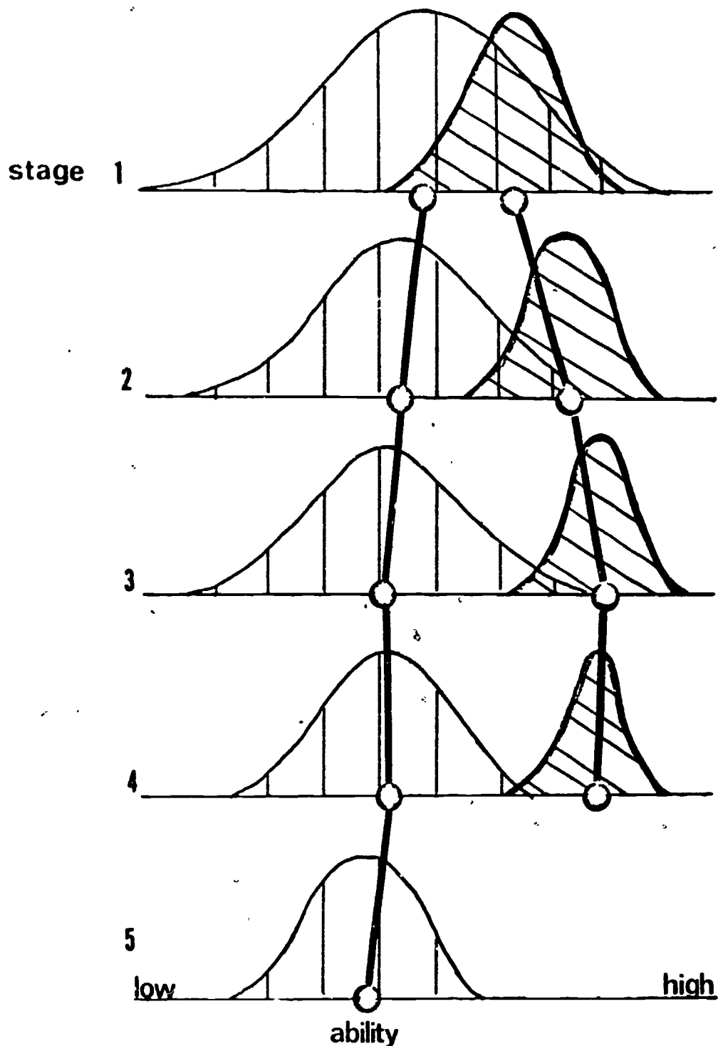
FIGURE 6: Diagrammatic representation of a Bayesian adaptive strategy. Two examinees' performances are represented. Depicted by the location and relative width of the distributions at each stage (1-5) is the reduction of the variance of the ability estimate at each stage.
