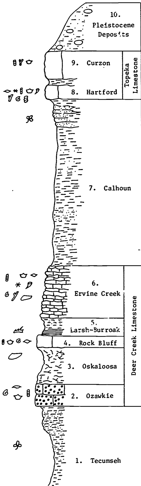
Figure 1.- Graphic description of rocks that are present at Seaman School Outdoor Laboratory. (Figure modified in part from Moore and Merriam, 1959, p. 17.)
