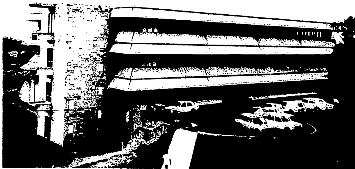
Front of Library, University of the South Pacific. Extension joints for the second stage are on the left.
