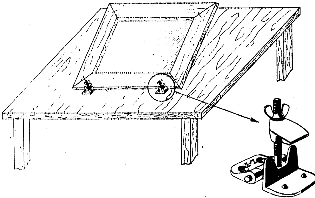
Figure 4-6.—Adjustment type hinge.
