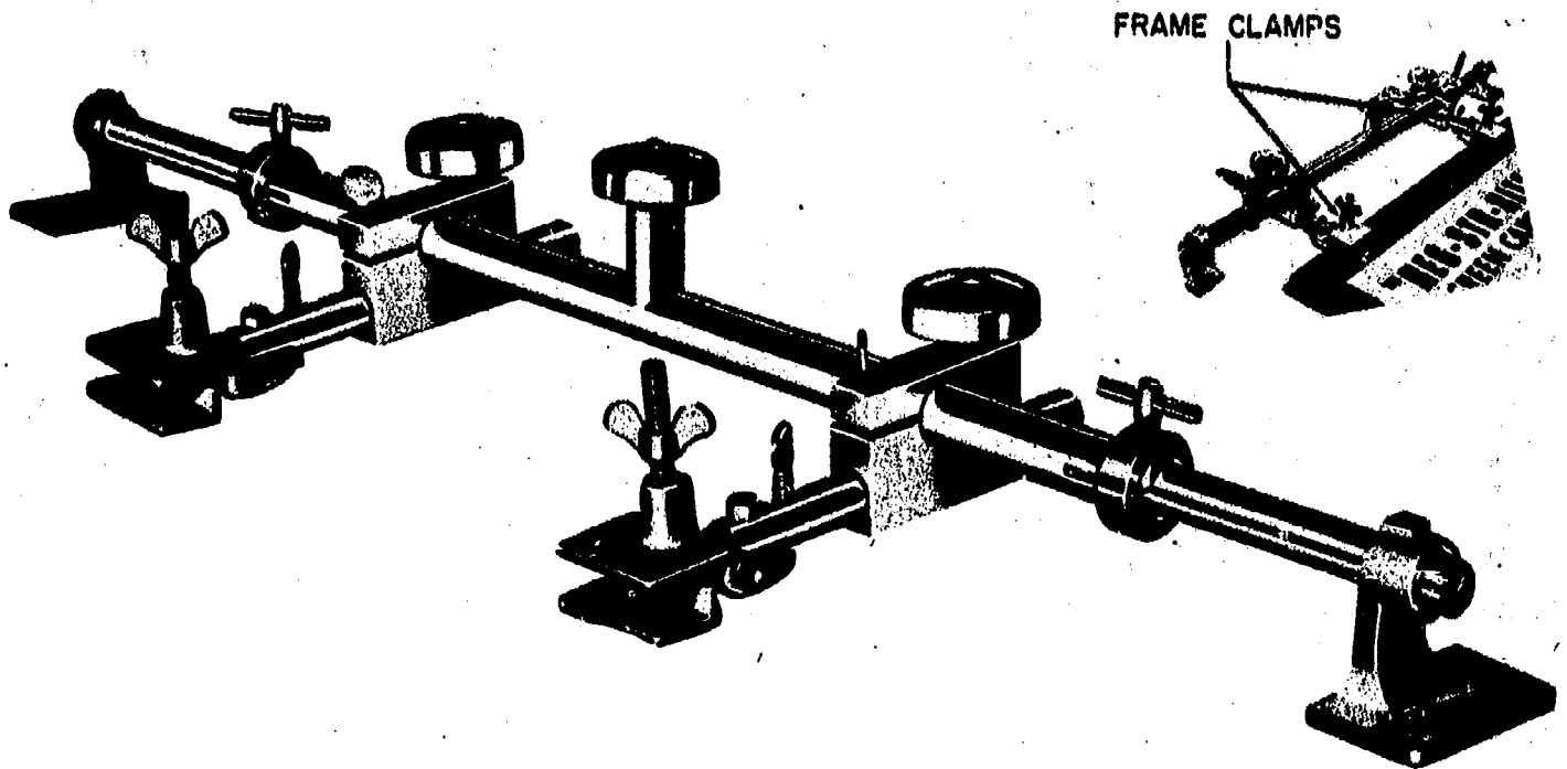
Figure 4-7.—Screen carriage.
