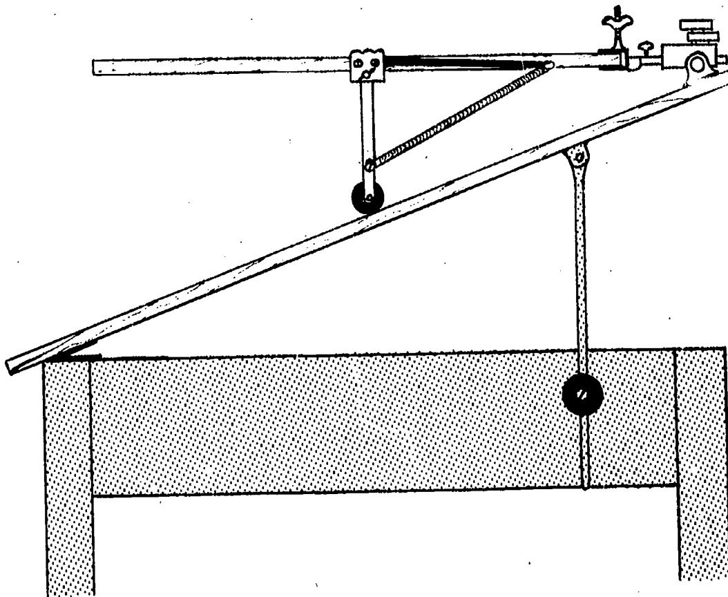
Figure 4-10.—Side kick.
