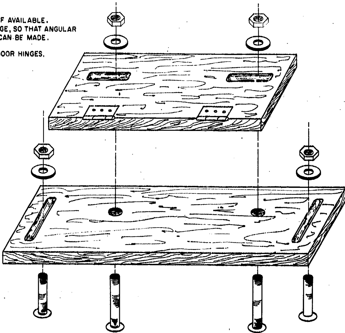
Figure 4-8.—Homemade screen carriage.
