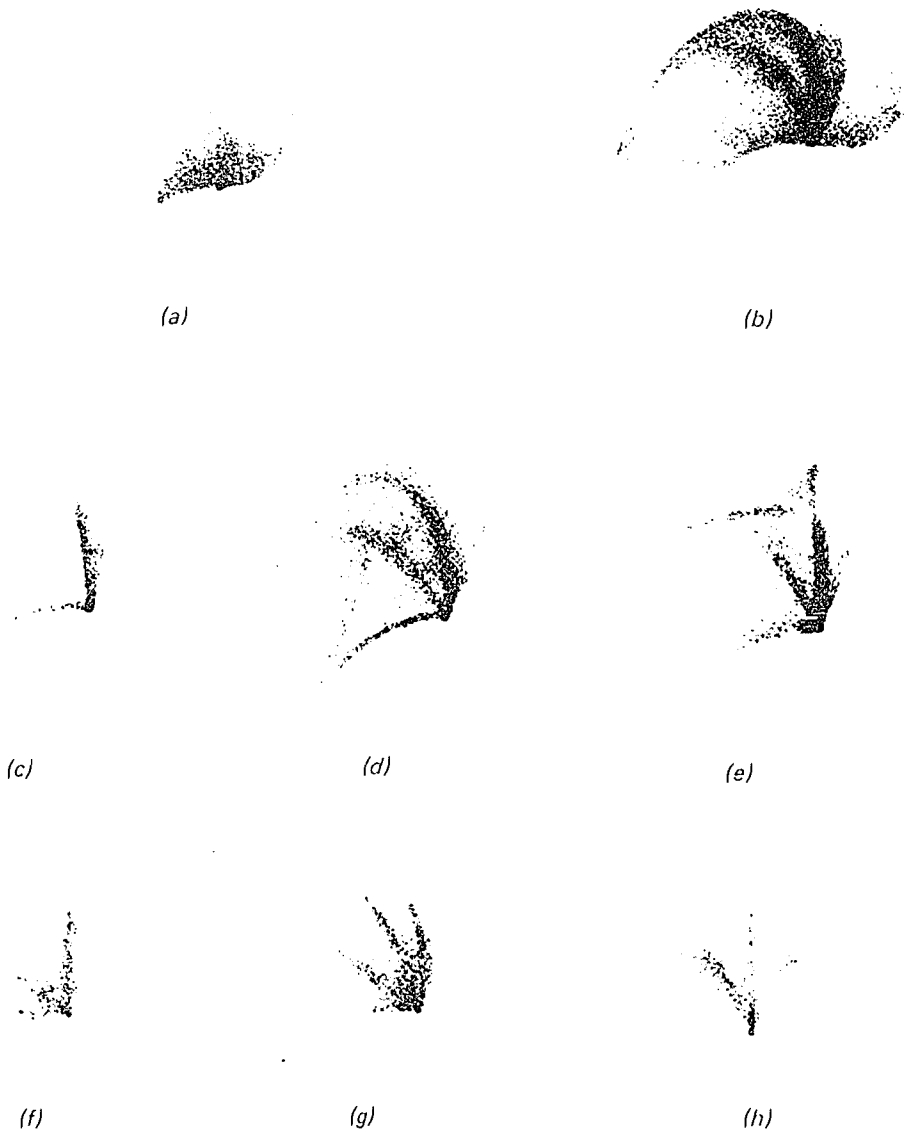
Figure 17: Drawings of Comet Tebbutt 1861 II by J. F. Julius Schmidt at the Athens Observatory in 1861.
