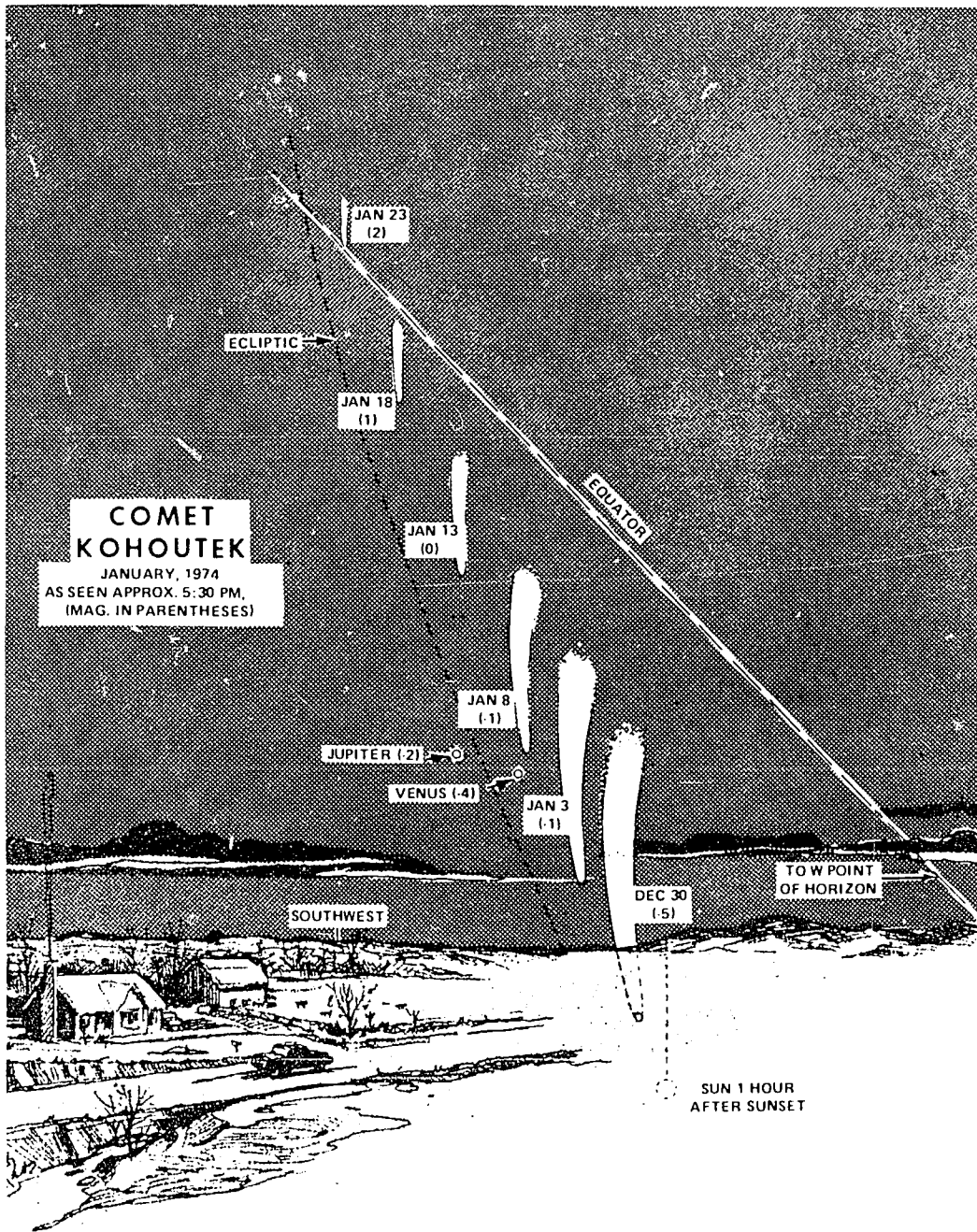
Figure 8: Comet Kohoutek as seen in the southwest during January, 1974. (Based on sketch by W. Liller, Harvard College Observatory.)
