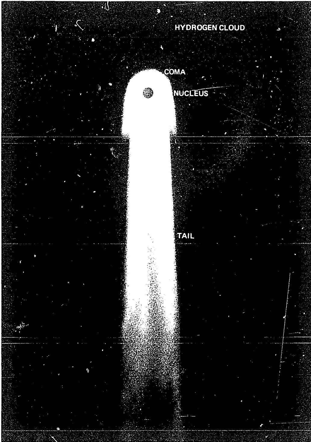
Figure 9: Artist's conception of a typical comet.
