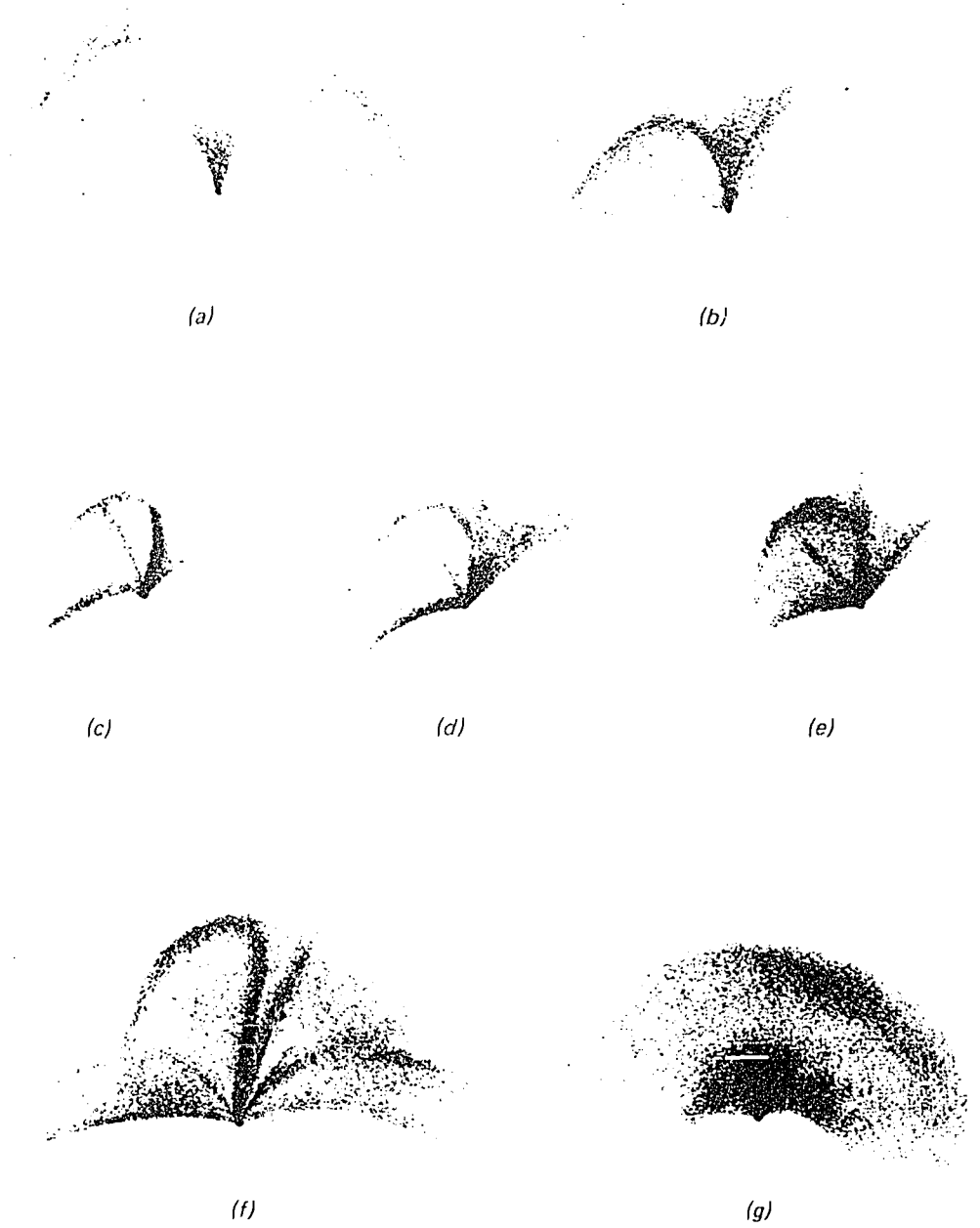
Figure 18: Drawings of Comet Tebbutt following those of Figure 17.
