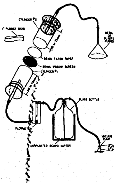
Assembly for Sampling Air (See page 8)
