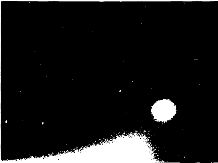
Figure 2-3 Zodiacal Light
