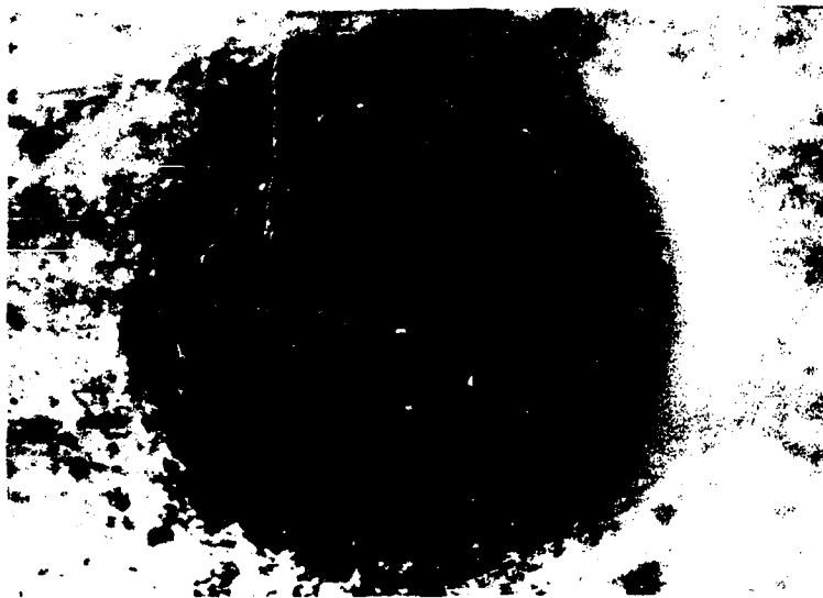
Figure 2-5 Impact Crater in Glass Plate
