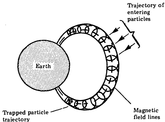
Figure 1-1 Trajectory of Nuclei and Particles as They Become Trapped in Magnetic Field
