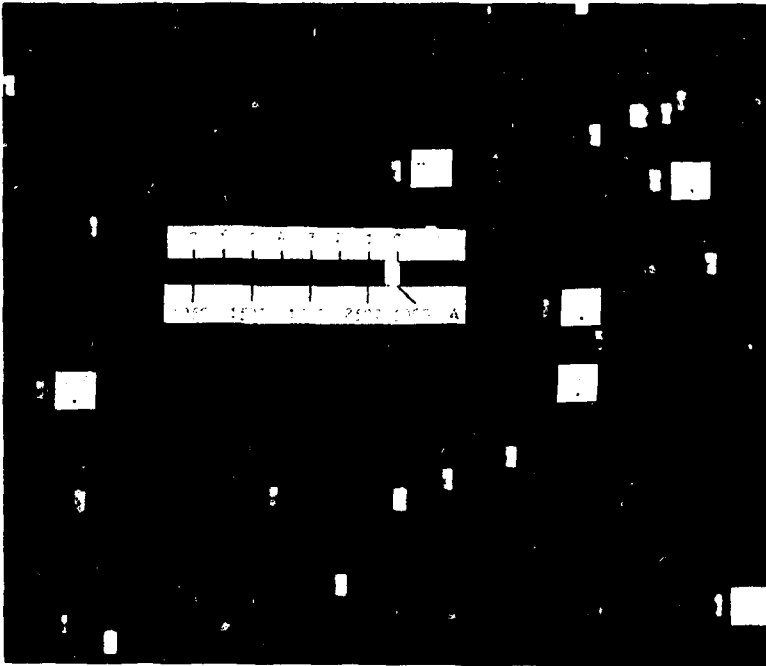
Figure 4-3 Typical UV Spectra of a Star Field
