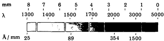
Figure 4-2 Spectrum of Stellar Astronomy Experiment
