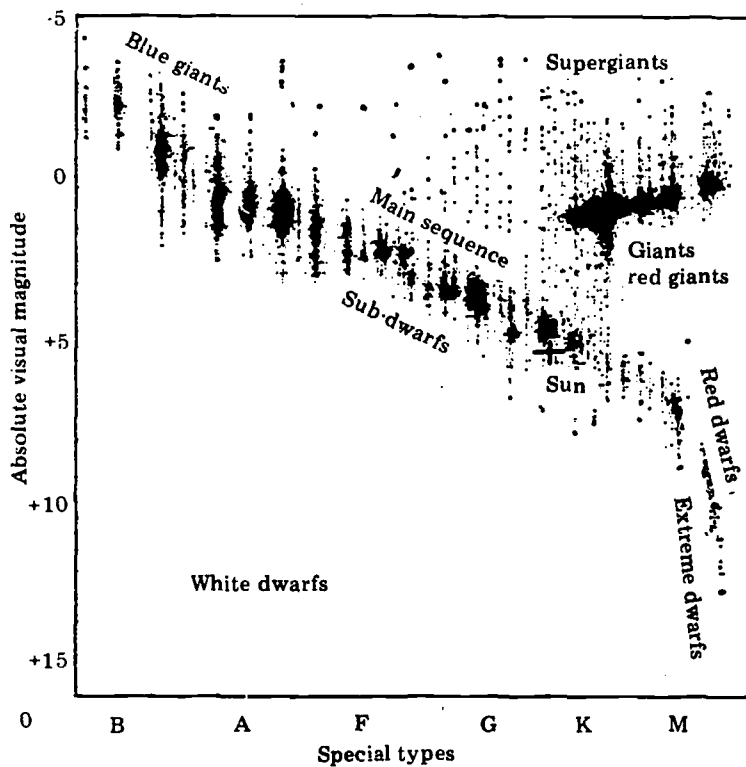
Figure 1-2 Names and General Distribution in the Hertzsprung-Russell Diagram of the Principal Categories of Stars
