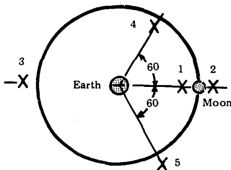
Figure 2-8 Lunar Libration Points
