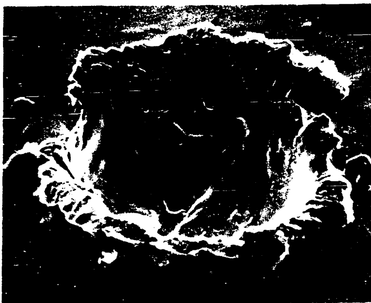
Figure 2-6 Gemini Micrometeoroid Pit
