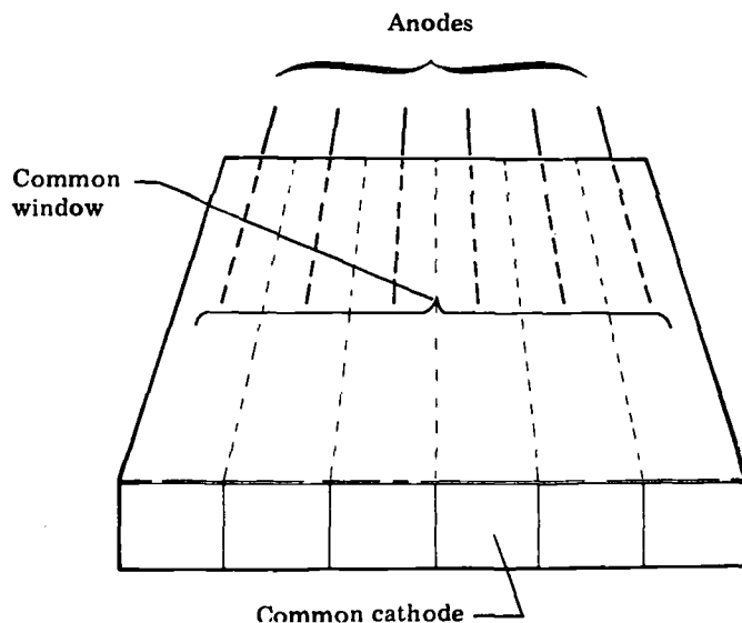
Figure 4-10 Proportional Counter Array
