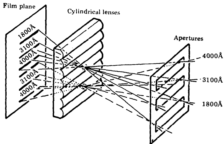
Figure 4-4 Concept of Cylindrical Lens Array
