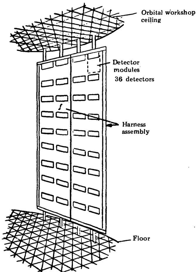
Figure 3-5 Transuranic Particle Detector in Skylab
