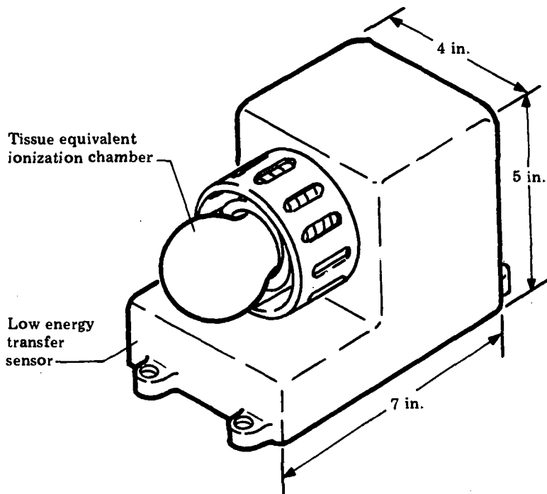
Figure 5-5 Active Dosimeter
