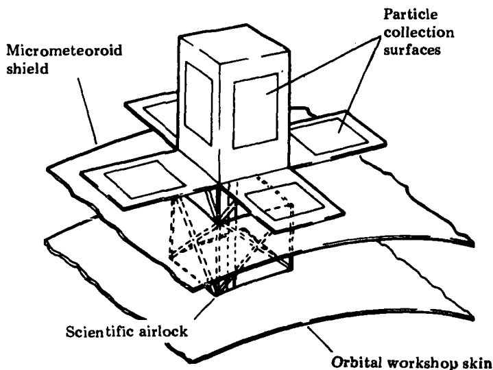
Figure 2-7 Particle Collection Experiment
