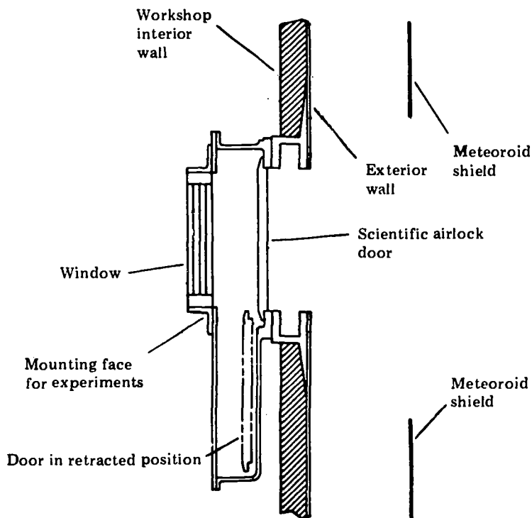
Figure 1-3 Section Through a Scientific Airlock
