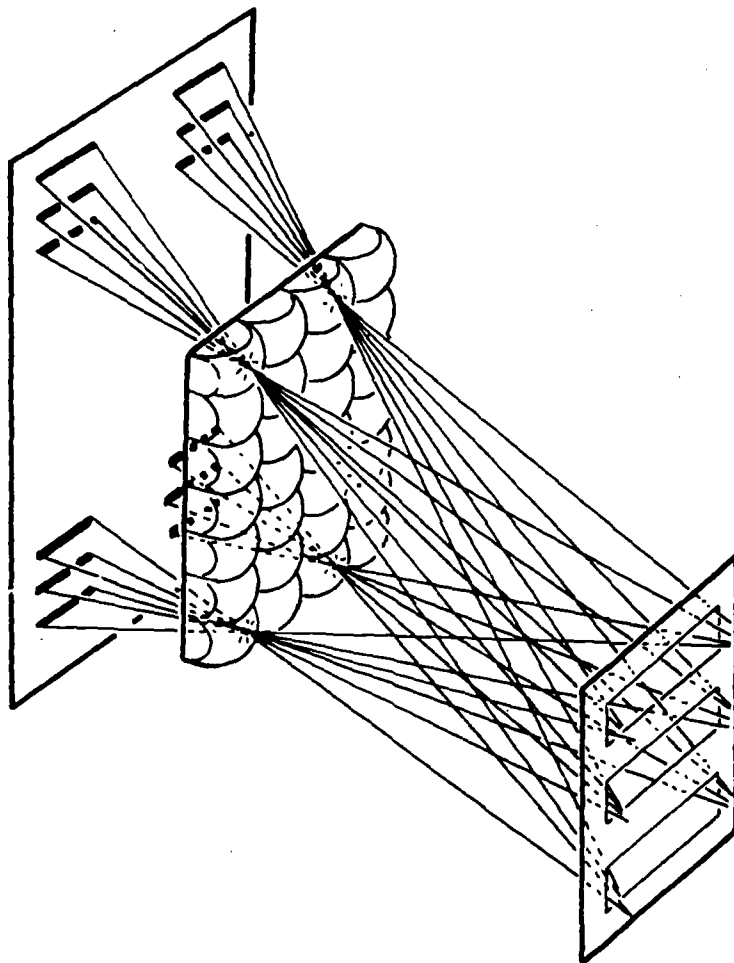
Figure 4-5 Imaging Format from Spherical Lens Array
