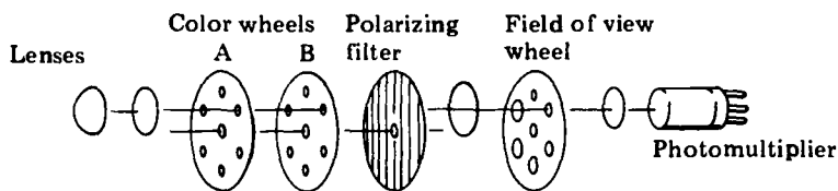
Figure 5-2 Optical Scheme of Photometer
