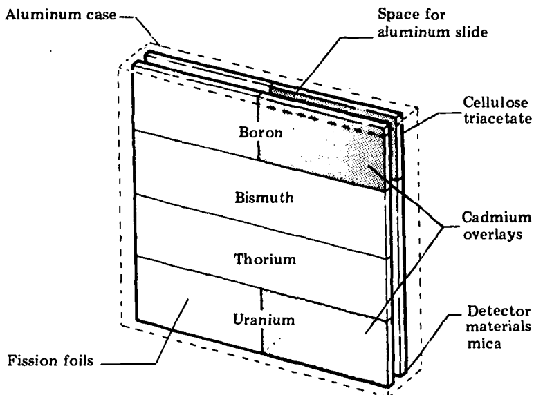
Figure 3-6 Neutron Detector
