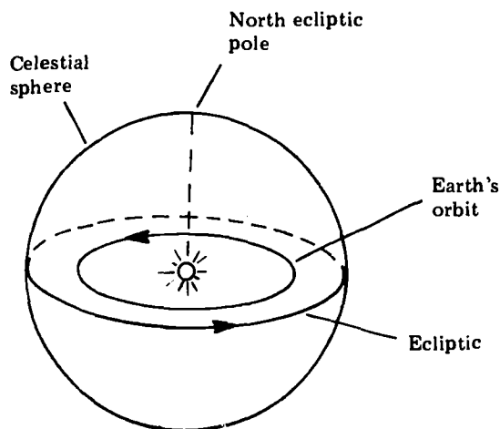
Figure 2-1 Celestial Sphere and Ecliptic
