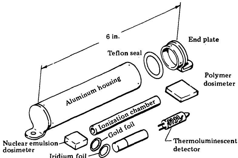
Figure 5-6 Exploded View of Passive Dosimeter
