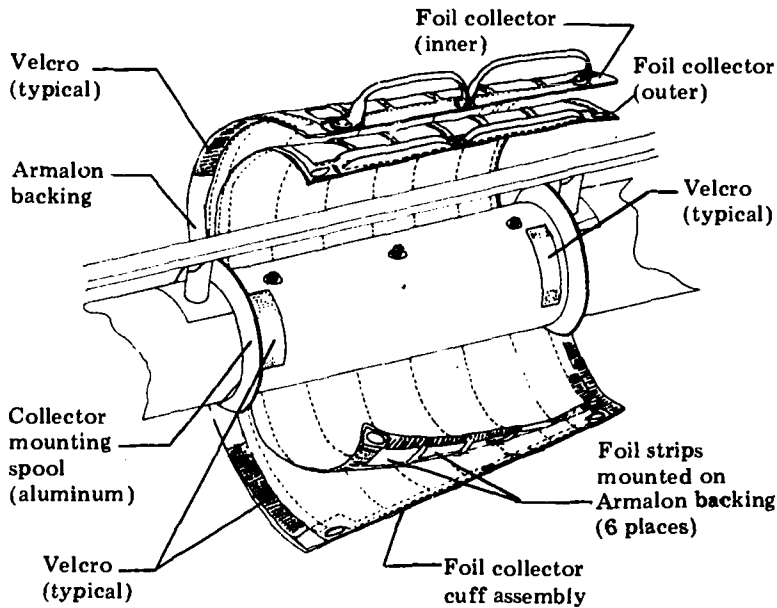
Figure 3-1 Magnetospheric Particle Collector
