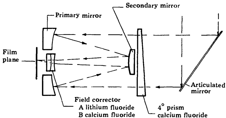
Figure 4-1 Optical Plan
