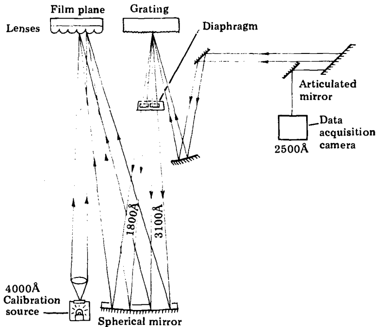
Figure 4-6 Optical Scheme of Ultraviolet Panorama
