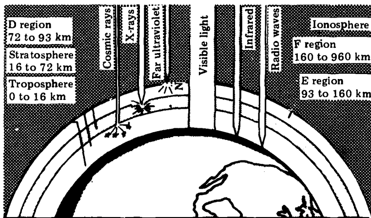
Figure 3-2 Atmospheric Absorption of Radiation
