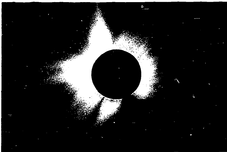
B 1970 Eclipse
