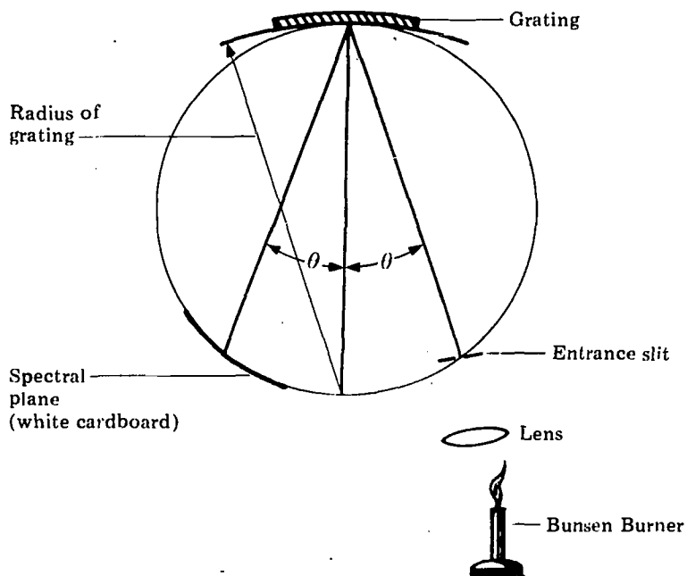
Figure 7 Experiment Layout
