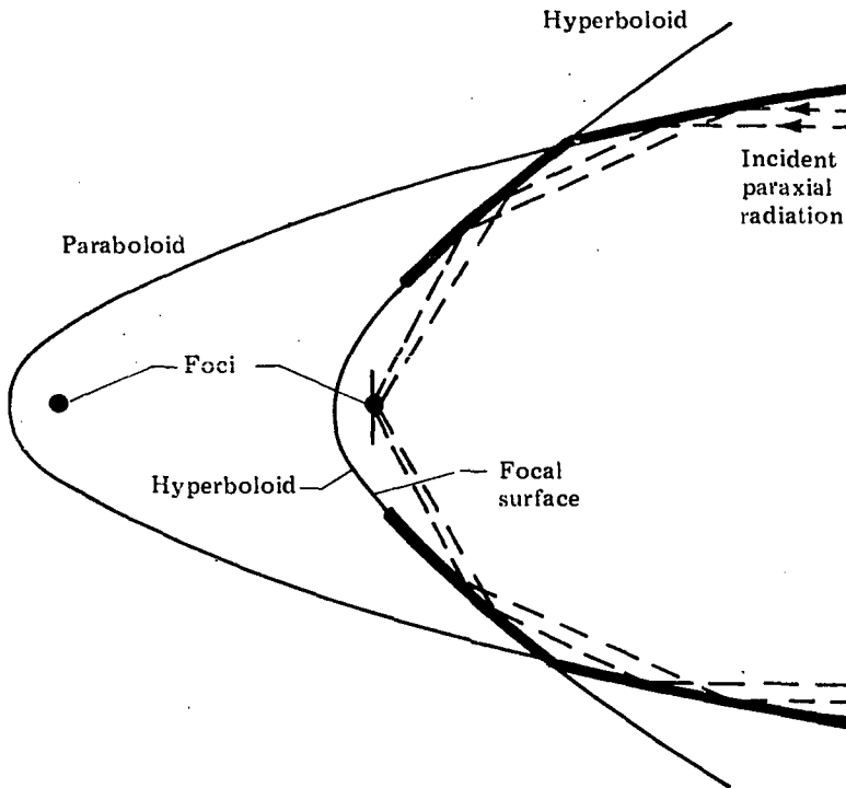
Grazing Incidence Telescope Geometry
