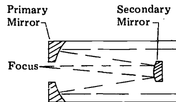
Cassegrain Telescope
