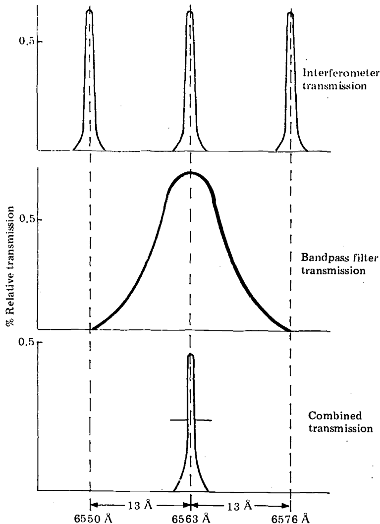
Figure 5 Interferometer Transmission
