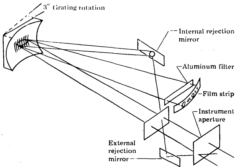
Figure 3 Optical System of the Spectroheliograph
