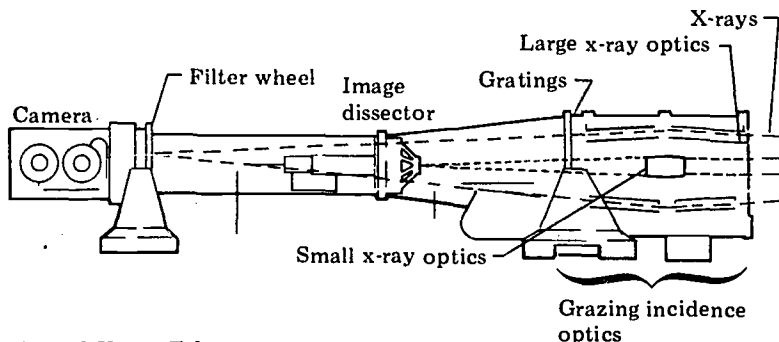
Plan of X-ray Telescope
