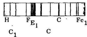
Typical spectrum
