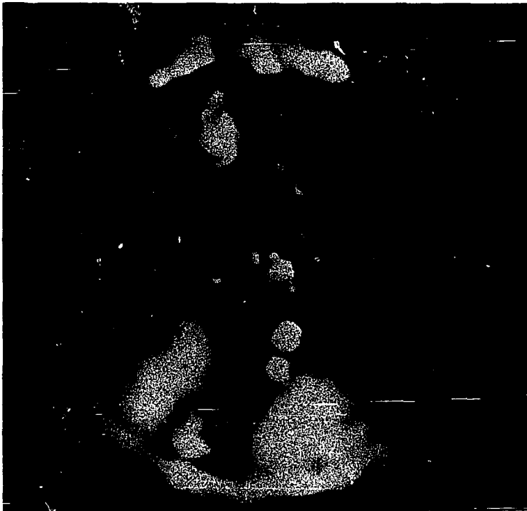
The Sun, Viewed Only as a Source of X-Rays
