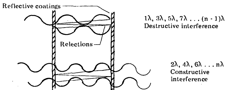
Figure 4 Interferometer Reflections
