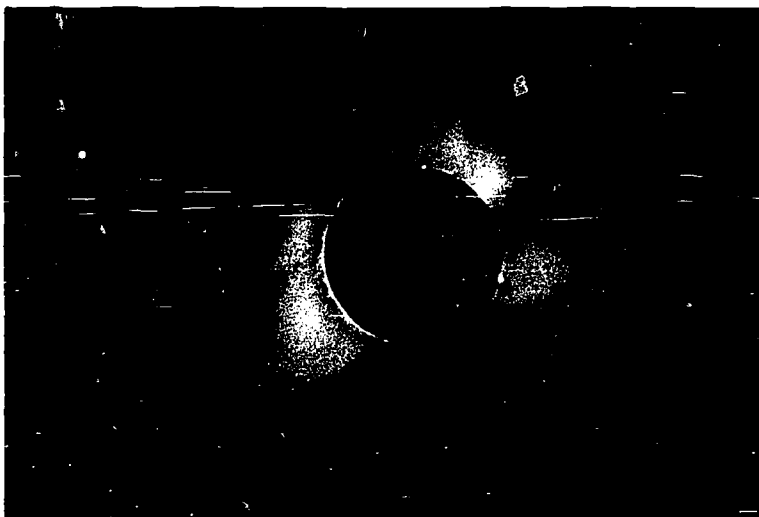
A 1966 Eclipse
