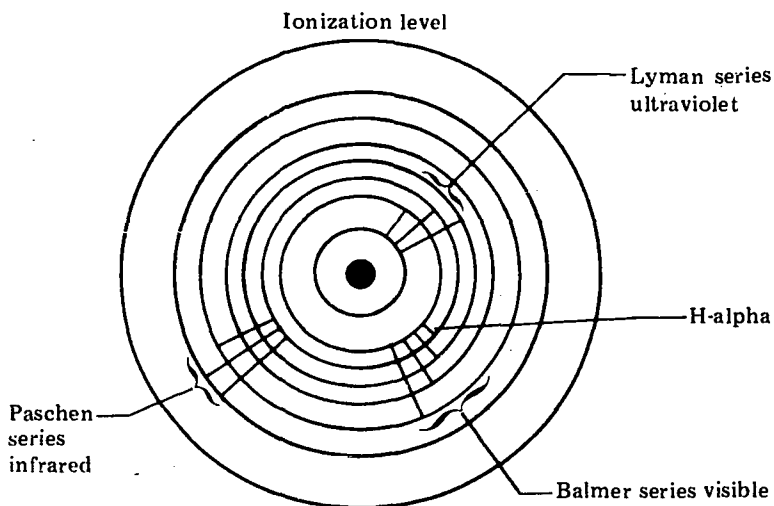
Figure 1 Hydrogen Series
