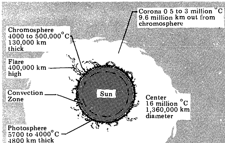
Figure 1 Solar Zones
