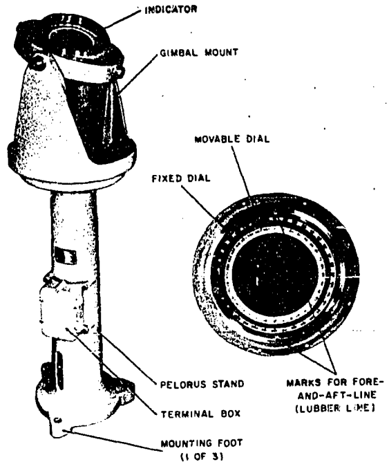
Figure 2-14. Gyro repeater. 51.131
