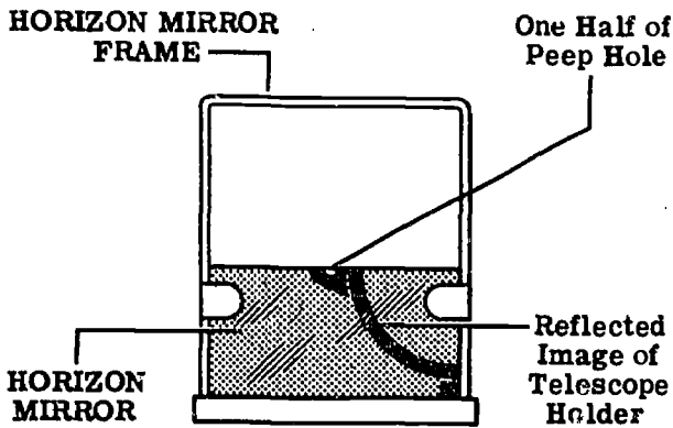
Figure 7-6. —Perpendicular adjustment of the horizon mirror.
