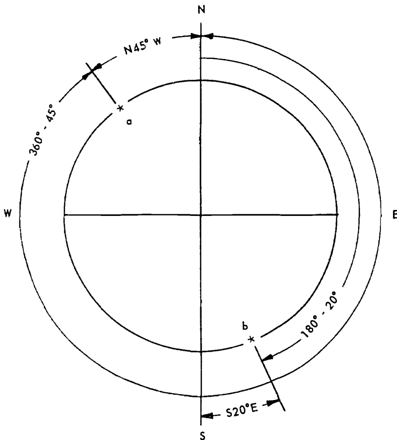
Figure 5-22.—Finding Z_n .
