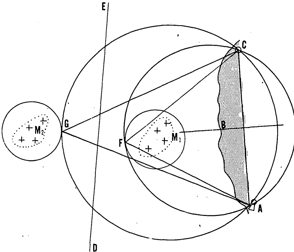
Figure 3-8.— Danger angles.
