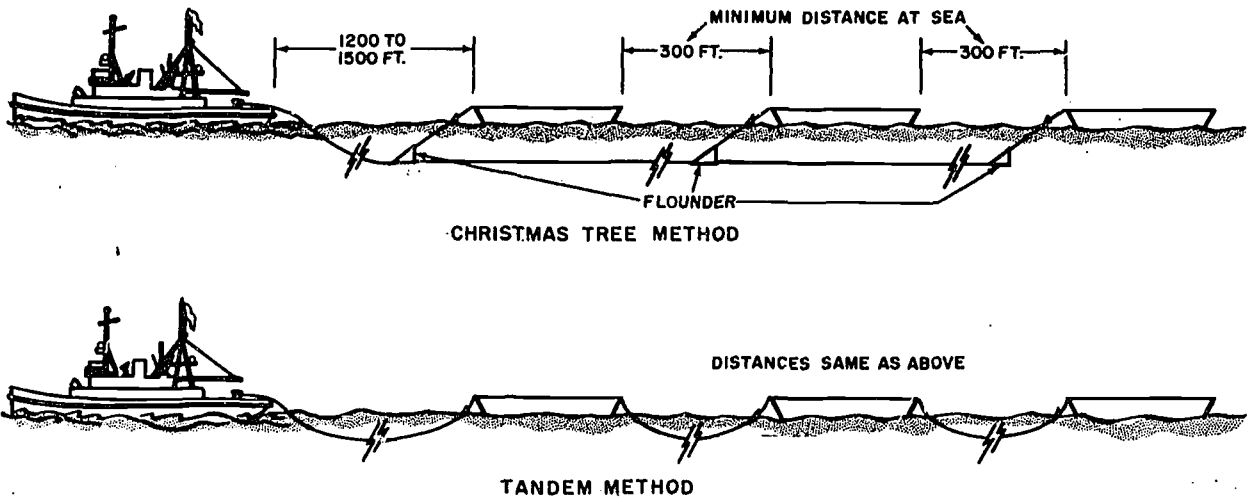
Figure 6-13.--Towing barges astern.
