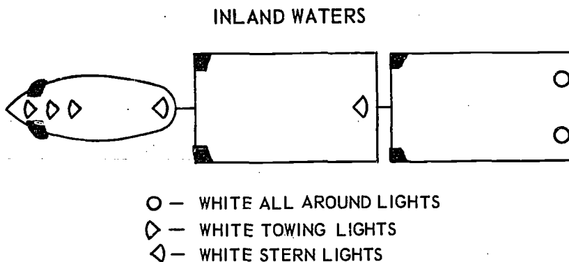
Figure 8-5. A tow in tandem. C80.121
