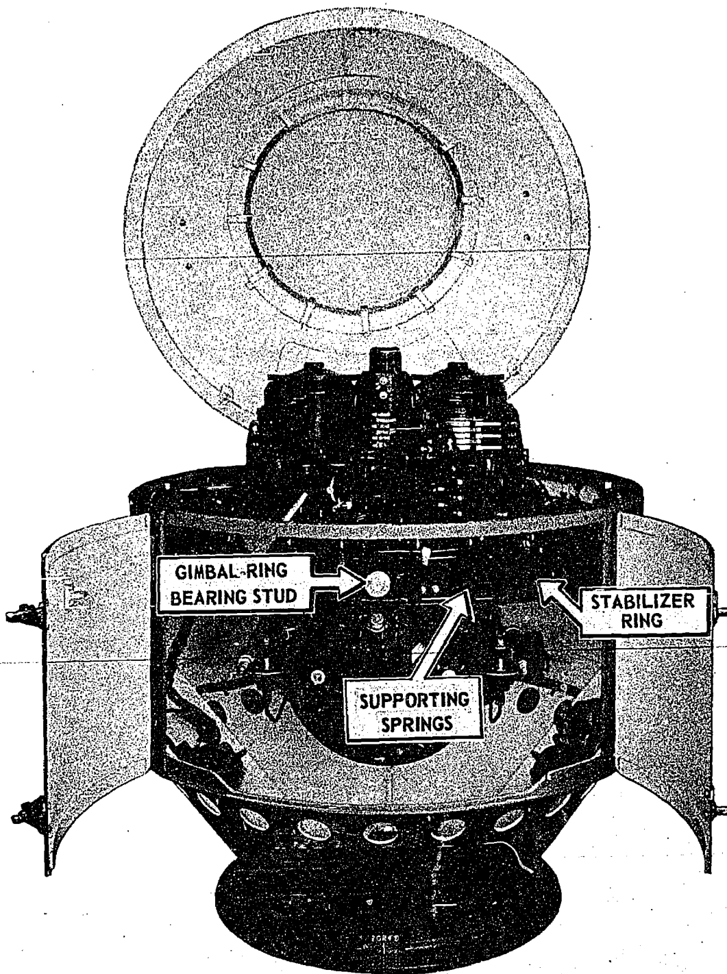
Figure 2-11. Sperry gyrocompass Mk 11 Mod 6.
