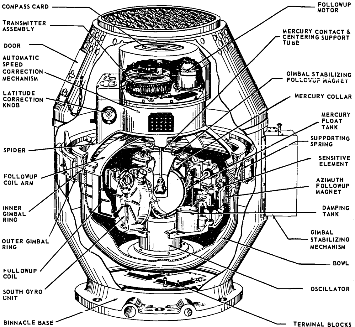
Figure 2-12.—Arma gyrocompass.
