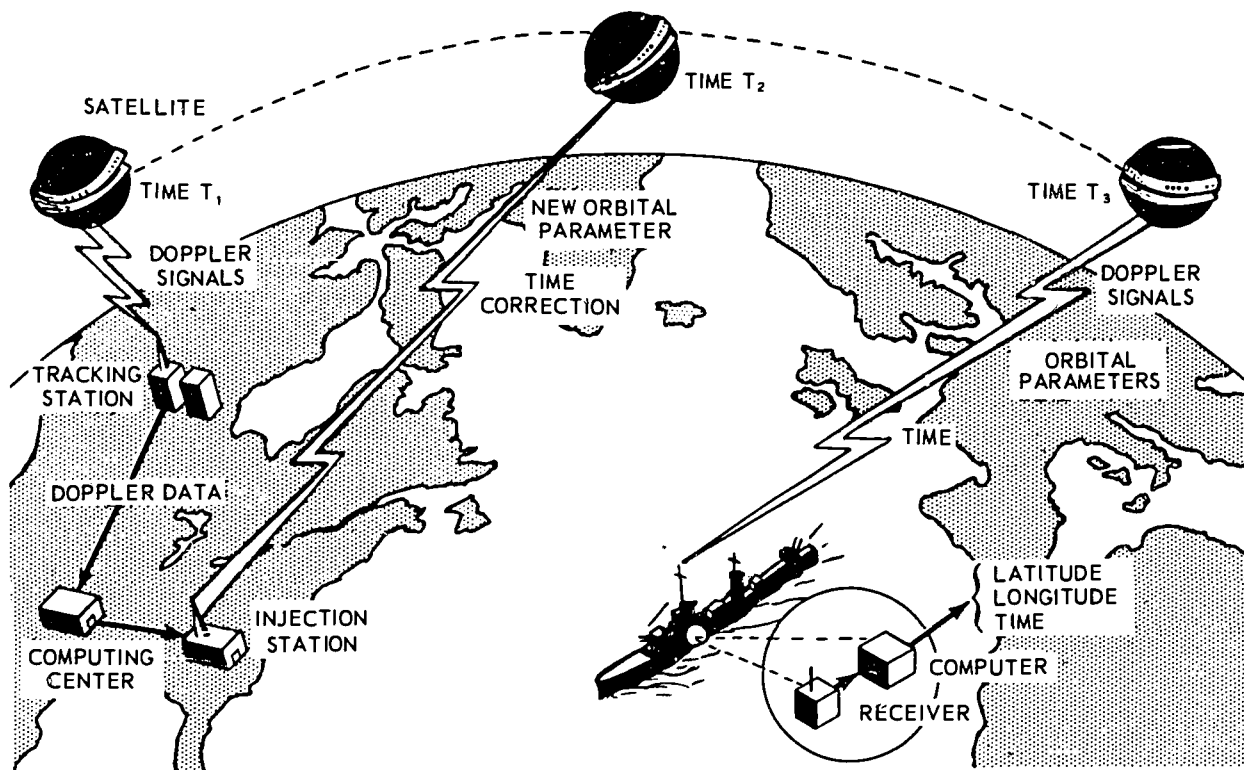
Figure 4-5. Navigational satellite system. 69.55
