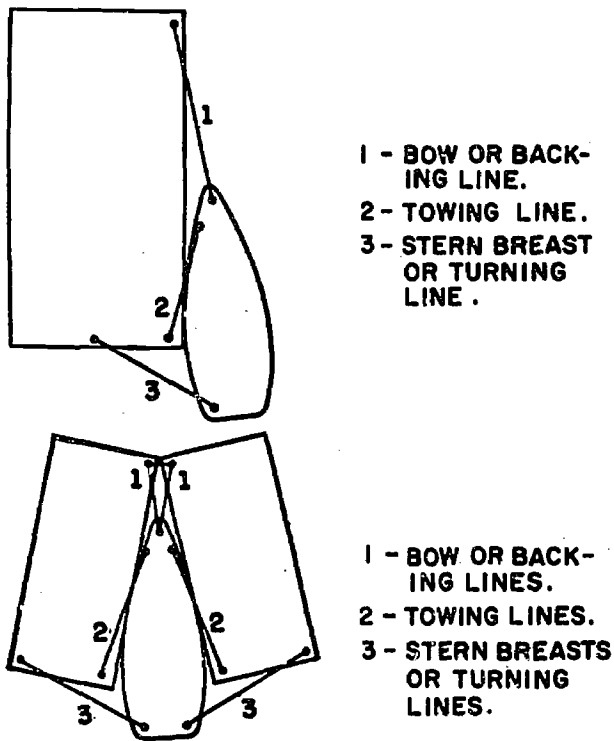
3.227(58)D Figure 6-11.—Alongside towing.
