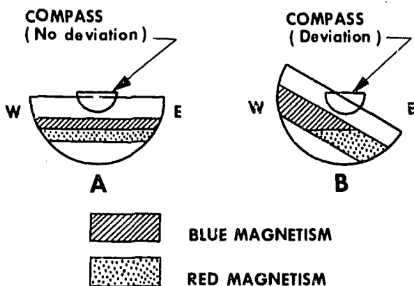
Figure 2-6.—Heeling error. 112. 5
