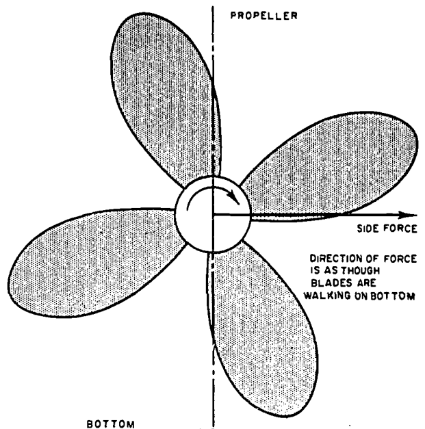
Figure 6-4.—Side force.
