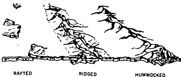
Figure 10-7.—Types of ice topography. 112.86
