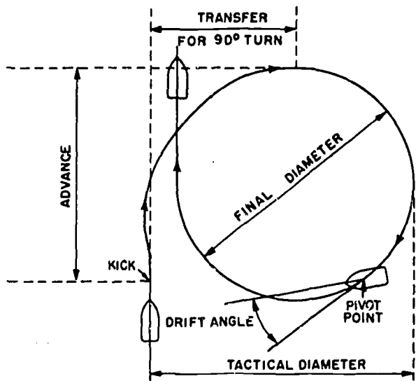
Figure 6-5.—Turning circle. 58.71
