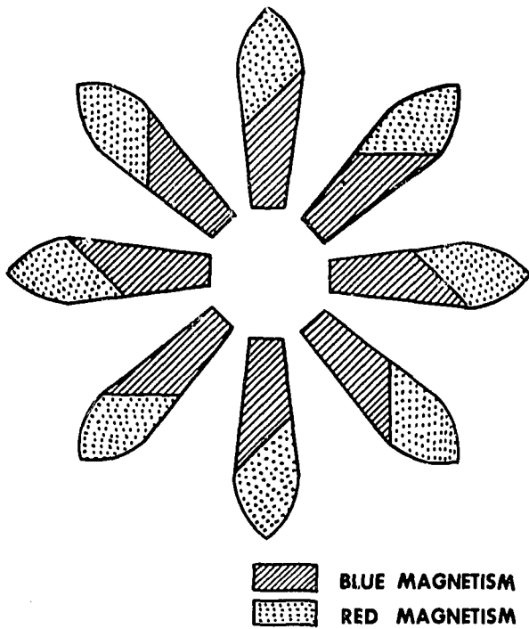
Figure 2-3. Ship built on northeast heading. 112.1
