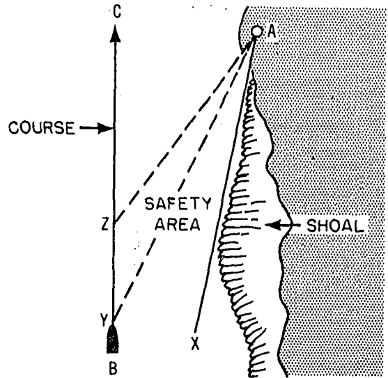
Figure 3-7.—Danger bearing.
