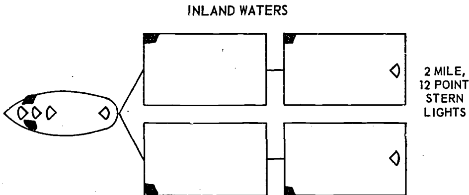
Figure 8-6. Barges abreast in tiers. C80.122
