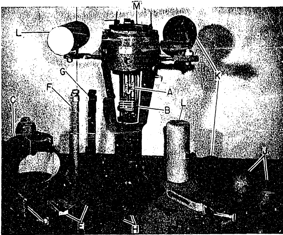
Figure 2-2. Magnetic compass binnacle with correctors. 112.2
