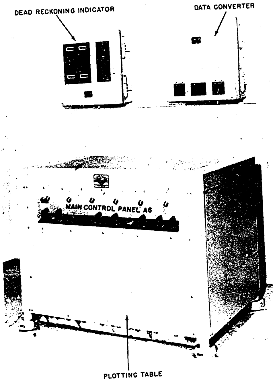
Figure 3-16. Plotting system USN Mk NC-2.
