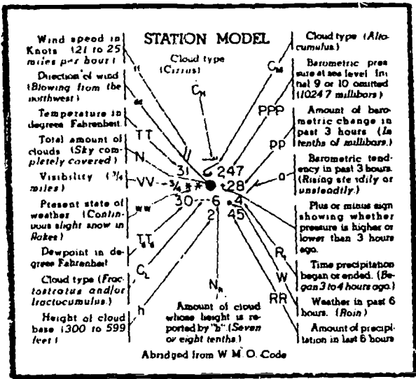
Figure 9-14.—Model of a weather station.
