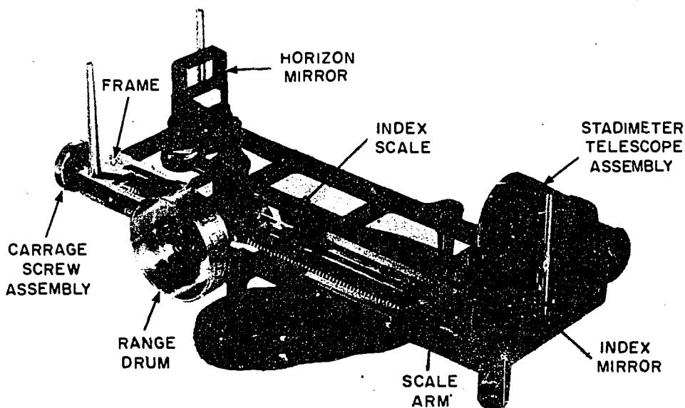
Figure 7-5. Type II Fiske stadimeter.
