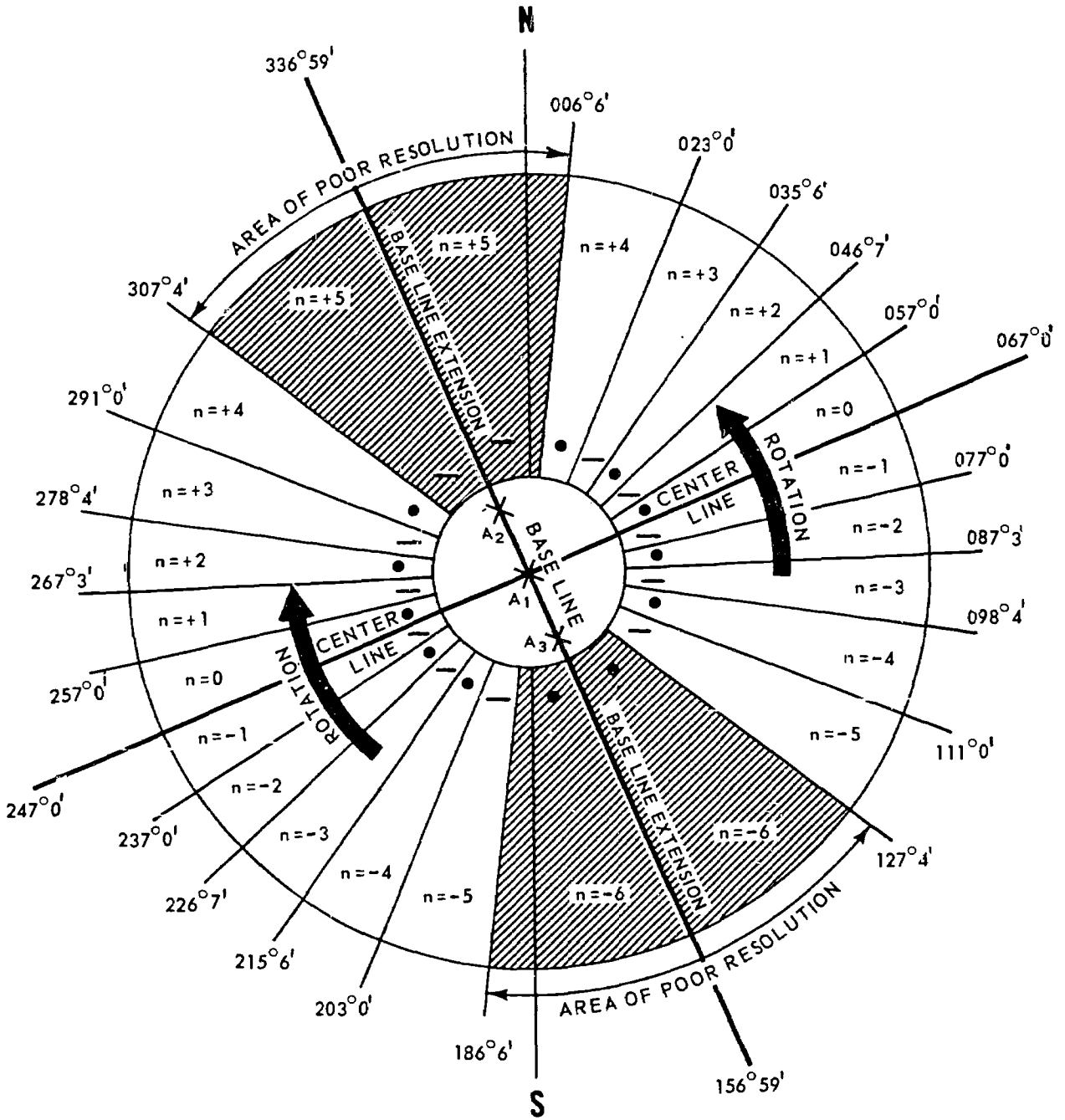
Figure 4-2. —Transmission pattern of consol stations.
