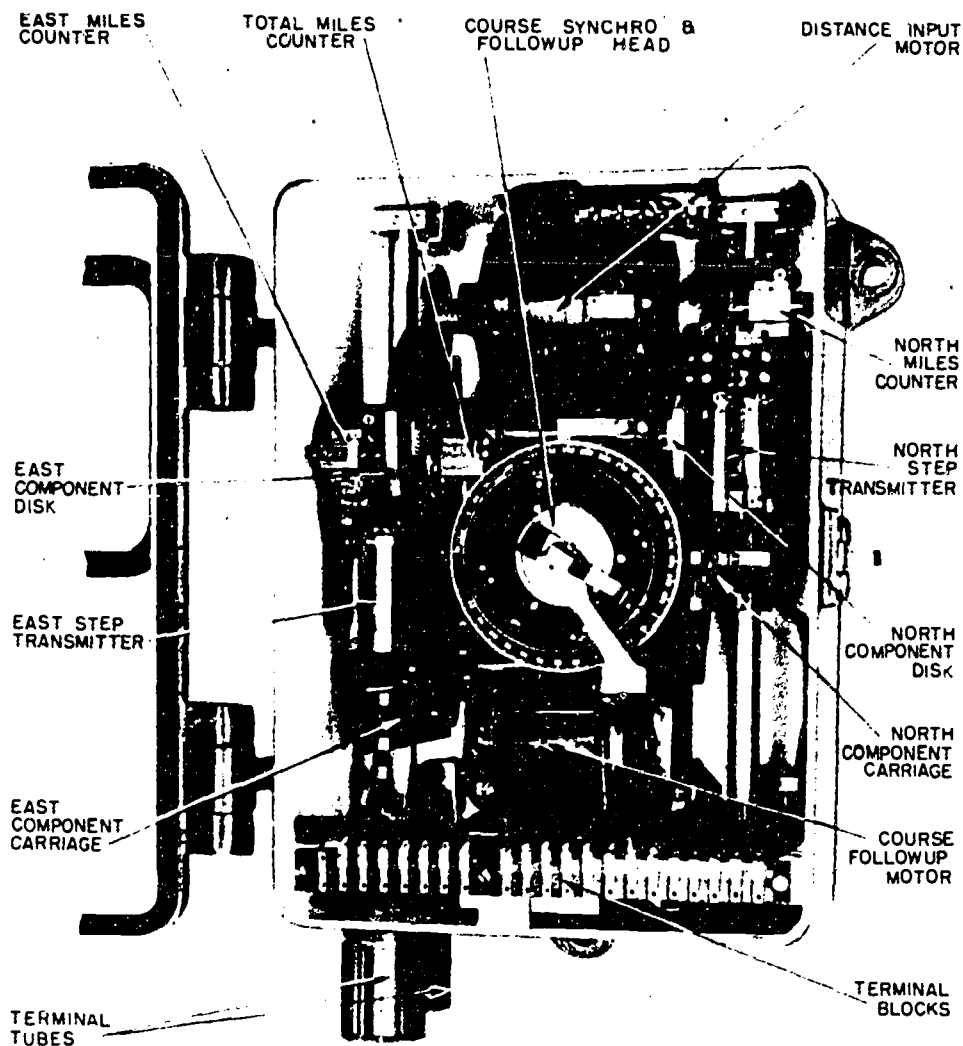
Figure 3-10. DR analyzer. 40.57
