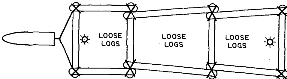
Figure 8-16.—Raft of one crib width.
