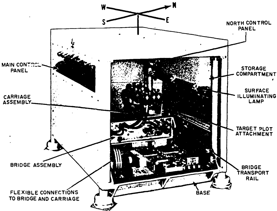
Figure 3-17. Plotting table Mk NC-2.
