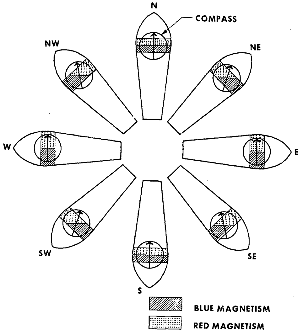
Figure 2-5.—Quadrantal deviation.
