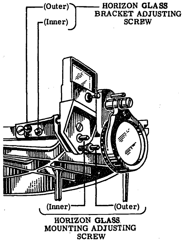
Figure 7-4.—Horizon glass mounting and adjusting screws.
