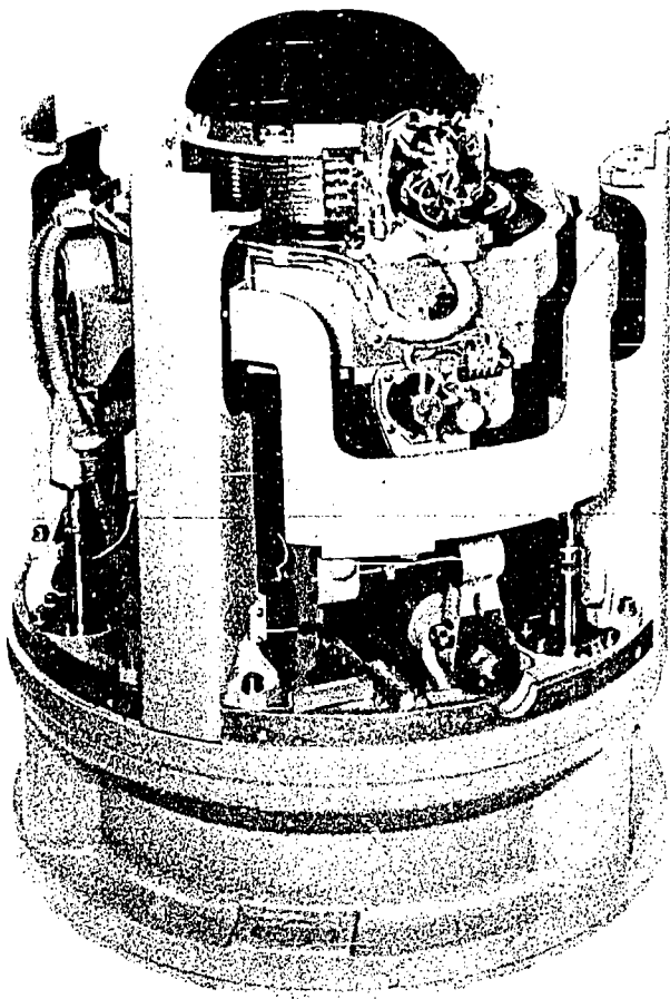
Figure 2-13. Sperry gyrocompass Mk 19. 27.170
