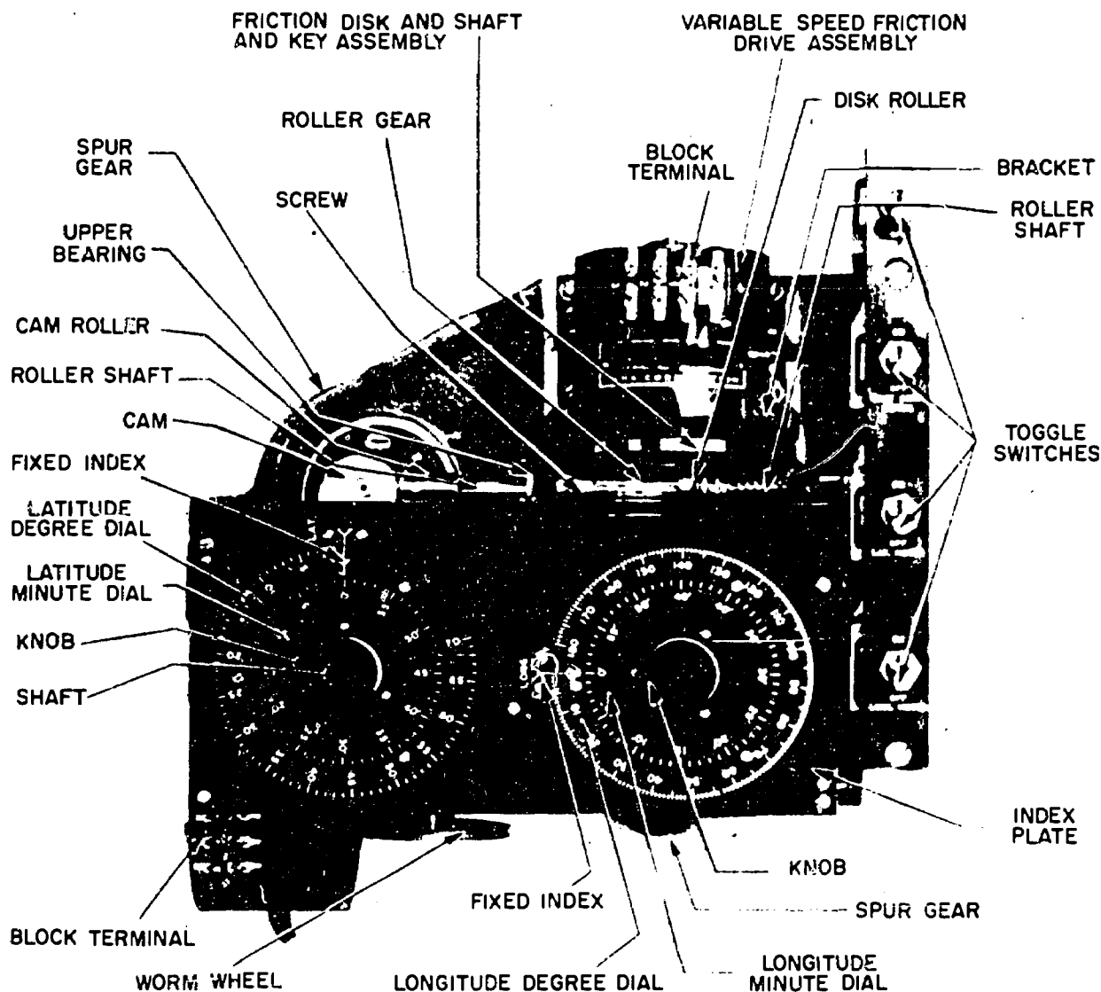
Figure 3-11. DR indicator. 40.59
