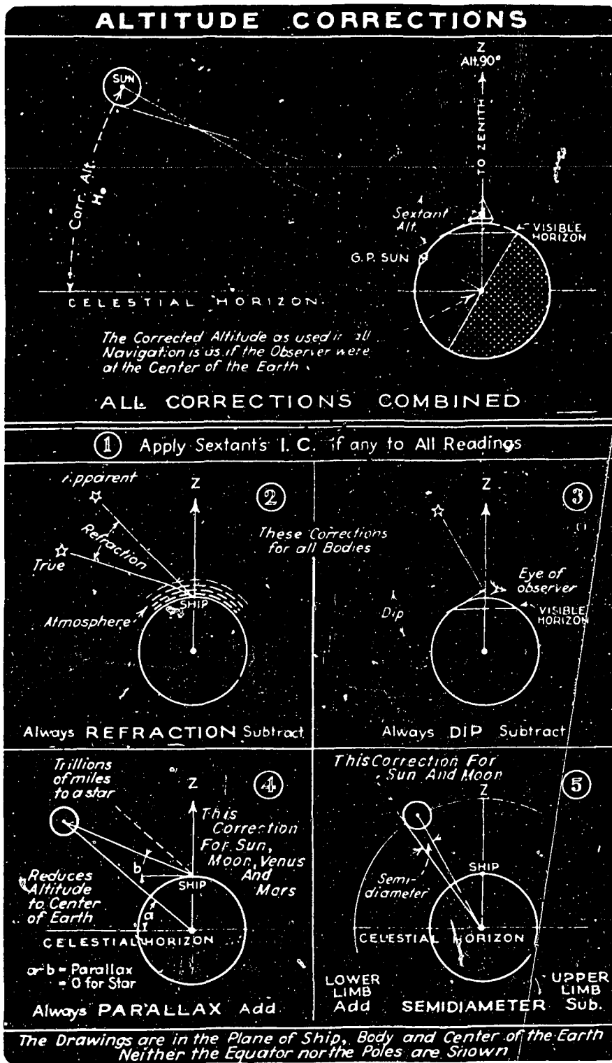
Figure 5-1.—Altitude corrections.
