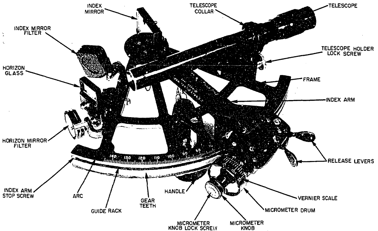
Figure 7-2. Endless tangent screw sextant. 29.268
