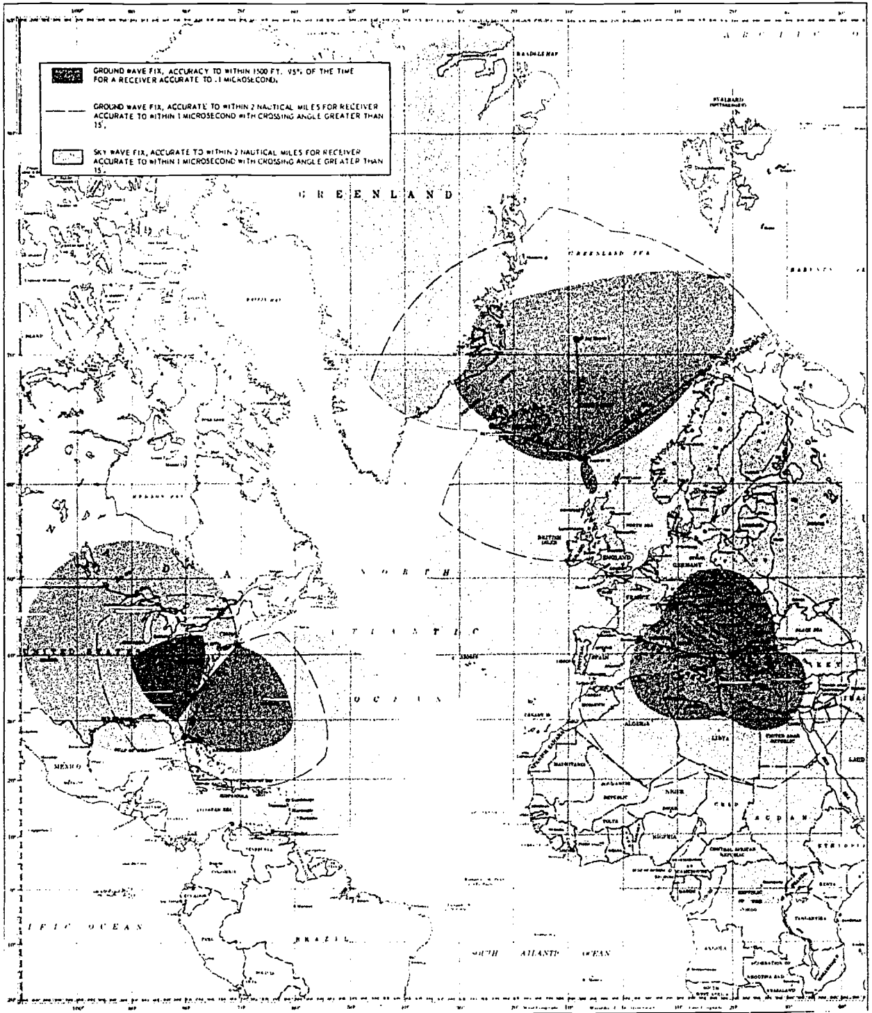
Figure 4-1. Some loran-C stations. 112.37
