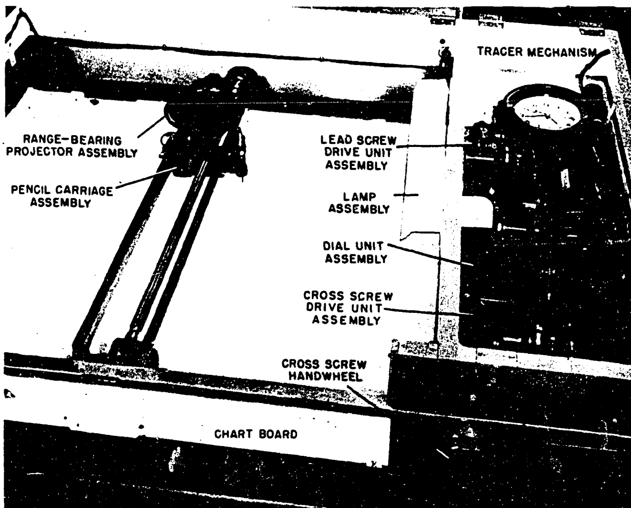
Figure 3-13. DRT plotting table. 40.61
