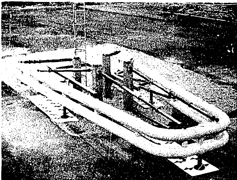
Figure 3. Highway crash barrier utilizing a shock absorption principle originally applied in cushioning astronauts' couches for splashdown impact.
