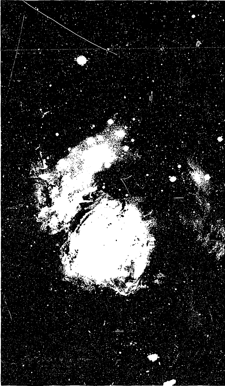
Figure 13b. The same star cluster in Sagittarius (M8), taken in ultraviolet light which emphasizes the gaseous content of the region — gives only an indication of the results to be gained from satellite astronomy (Lick Observatory Photo).
