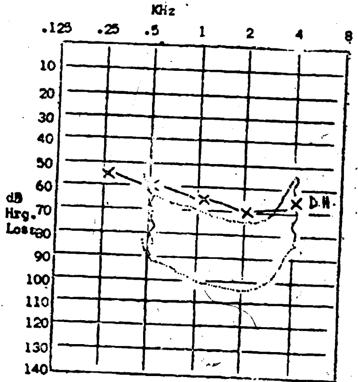
Fig. 4 Theoretical effect of D.H.'s wearing an OL 67 aid (OL 695 rec.). Maximum volume.
