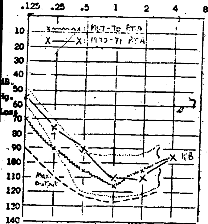
Fig. 14 Theoretical effect of K.B.'s aid.
