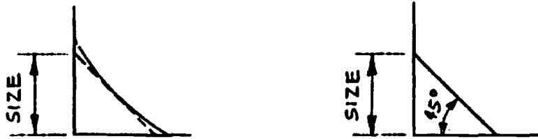
DESIRABLE FILLET WELD PROFILES
