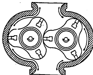
3 LOBE TYPE
