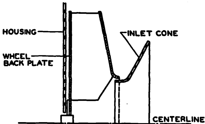
Type O Single Inlet Fans.
