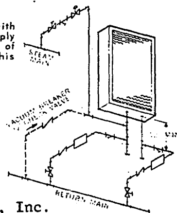
FLOAT AND THERMOSTATIC TRAP
