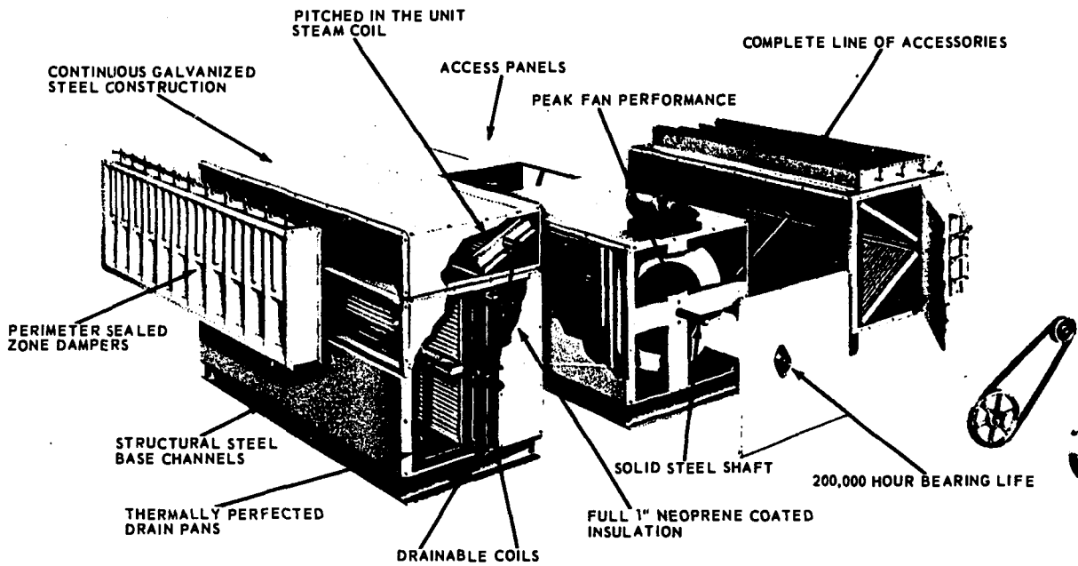
EXPLODED VIEW OF A MULTIZONE UNIT COURTESY, McQUAY, INC.
