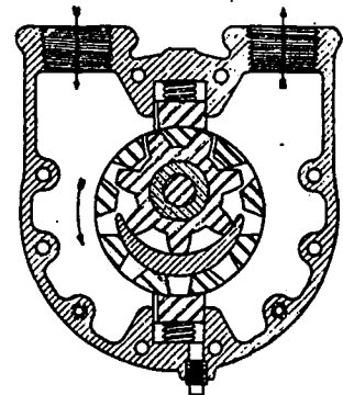
INTERNAL GEAR TYPE
