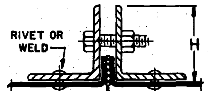
(M) COMPANION ANGLES (CAULK OR GASKET)
