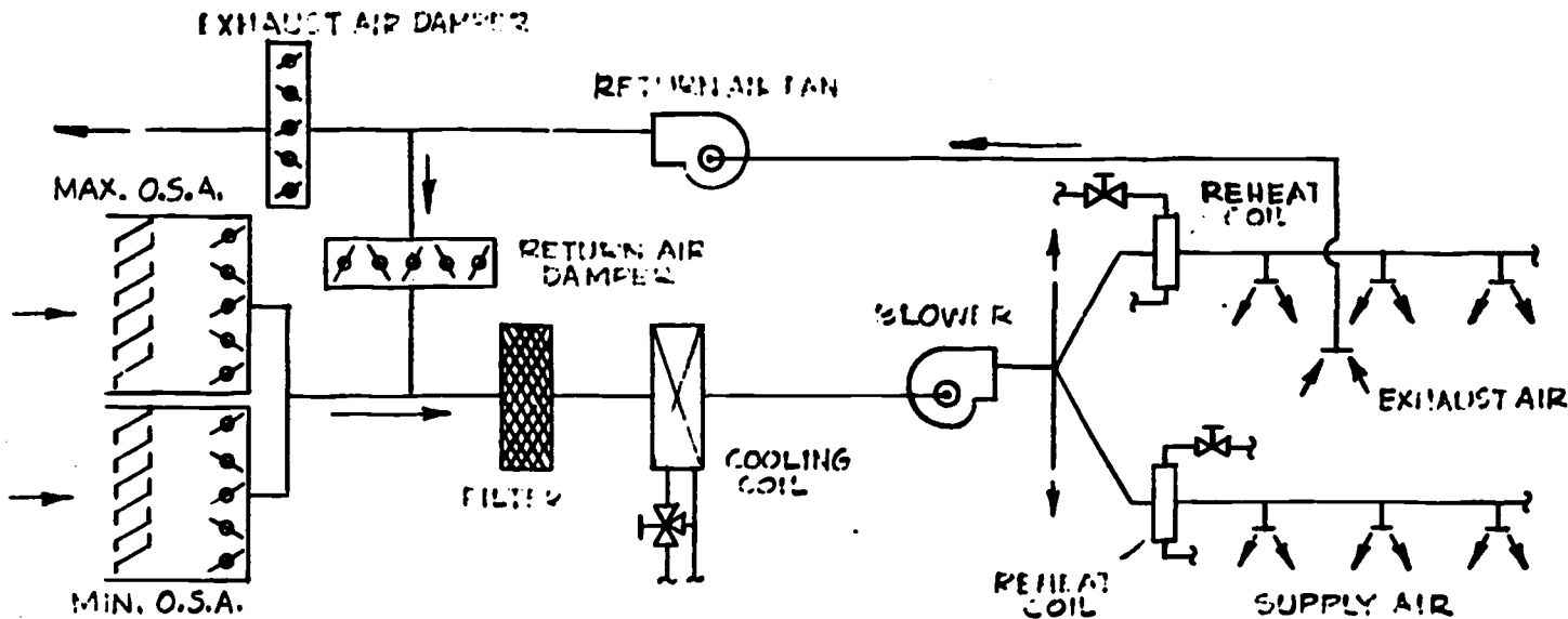
FIG 15-4 - REHEAT SYSTEM
