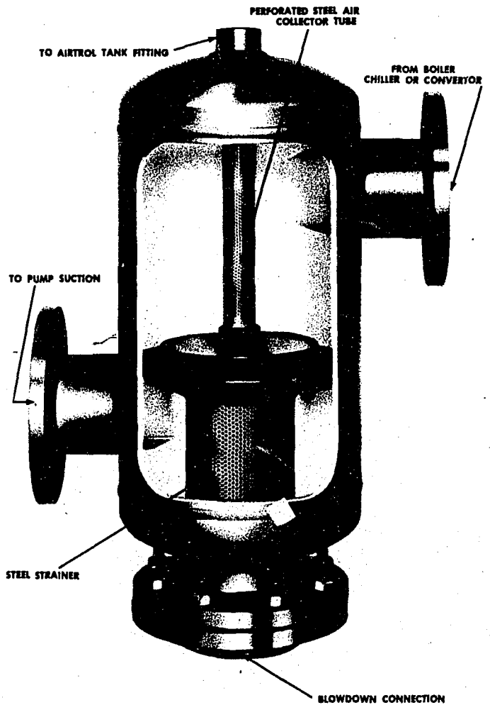
(b) Rolairtrol air separator with removeable system strainer.
