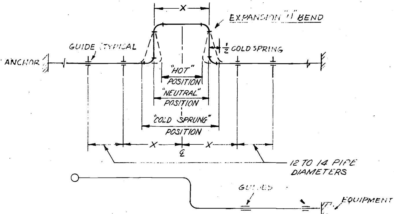
OFF-SET BEND
