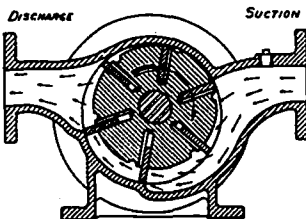
SLIDING VANE TYPE
