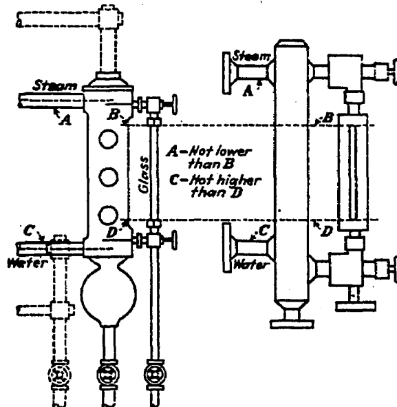
Fig. 122.1.6(d)(4) Typical Arrangement of Steam and Water Connections for a Water Column
