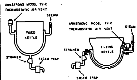
Fig. 13-4. On jacketed kettles
