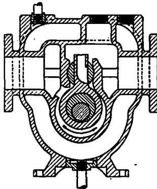
STEAM JACKETED CAM & PISTON TYPE
