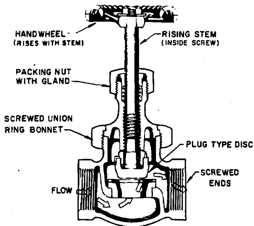
Fig. 2-26 Globe Valve
