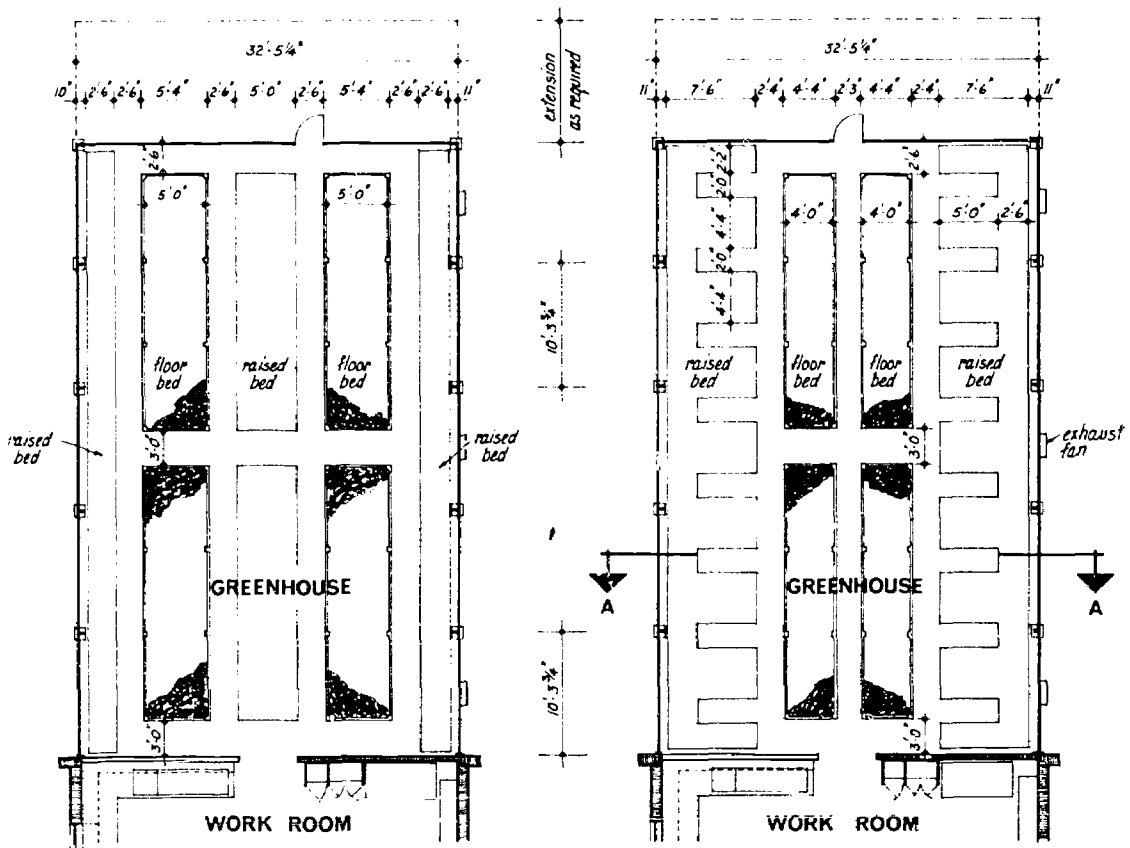
alternative plans of bed arrangements in greenhouse
