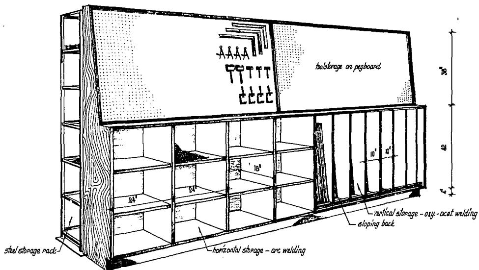
storage rack for welding rods and tools
