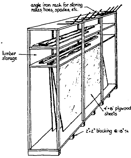
wood storage rack in workroom
