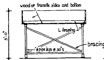
detail of raised bed in greenhouse
