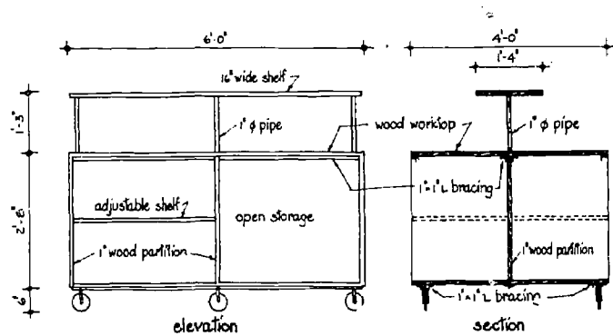
details - movable potting tables in workroom
