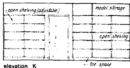
elevation K — toe space
