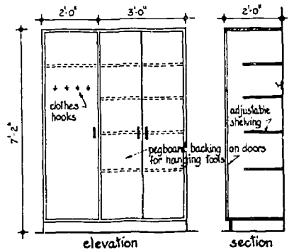
detail of clothes-tool cupboard in workroom
