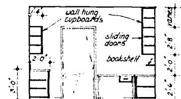
elevation H — student projects
