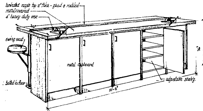
combination desk and work bench
