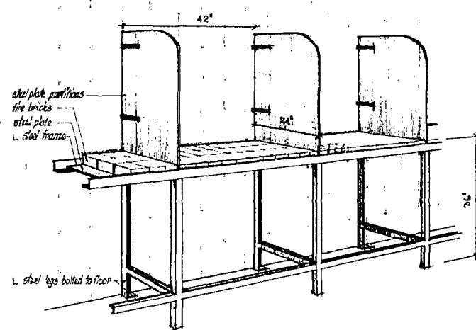
oxy - acetylene welding bench
