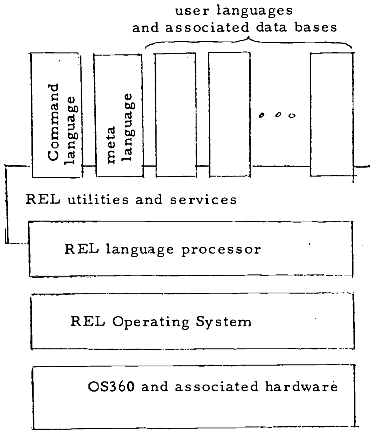
Figure 1: Schematic View of the REL System
