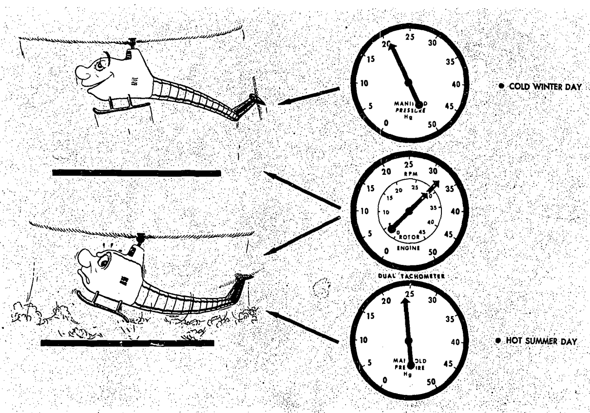
FIGURE 53.—High temperature reduces helicopter performance.
