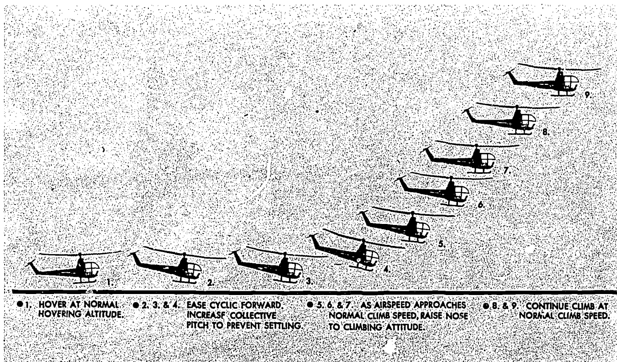
FIGURE 70.—Normal takeoff from a hover.
