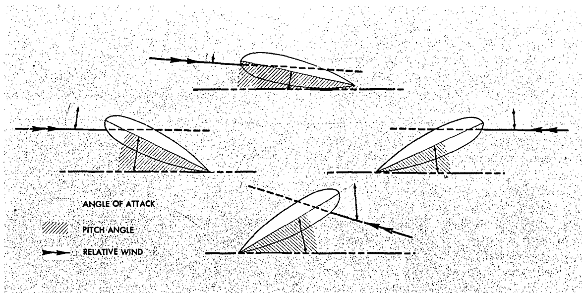
FIGURE 6.—The relationship between the angle of attack and pitch angle for various positions of the rotor blade in the plane of rotation during forward flight. Angle of attack is less than pitch angle 90^\circ to pilot's right (top); greater than pitch angle 90^\circ to pilot's left (bottom); and equal to pitch angle in the fore (left) and aft (right) positions.
