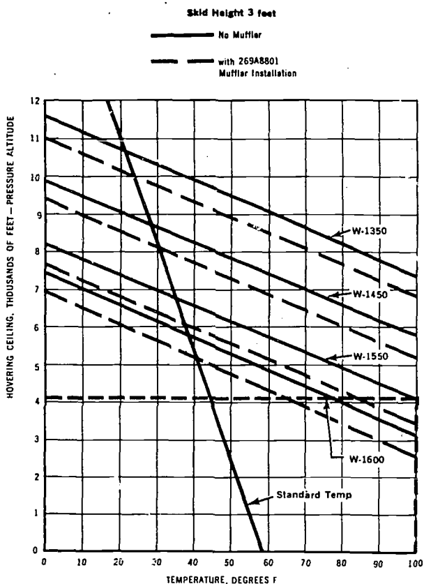
FIGURE 57.—Hovering ceiling (in ground effect) chart.
