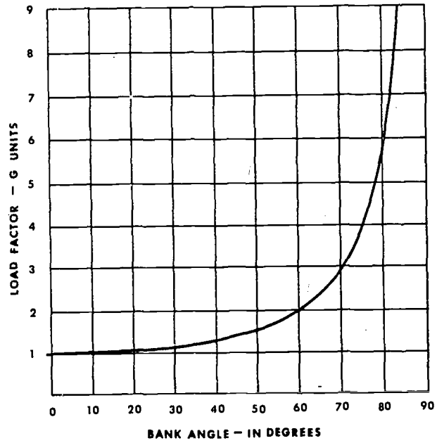
FIGURE 26.—Load factor chart.
