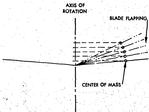
FIGURE 19.—Coriolis effect is the change in blade velocity to compensate for the change in distance of the center of mass from the axis of rotation as the blades flap.
