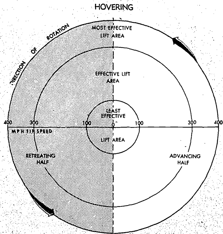
FIGURE 15.—Comparison of rotor blade speeds for the advancing blade and retreating blade during hovering and forward flight.
