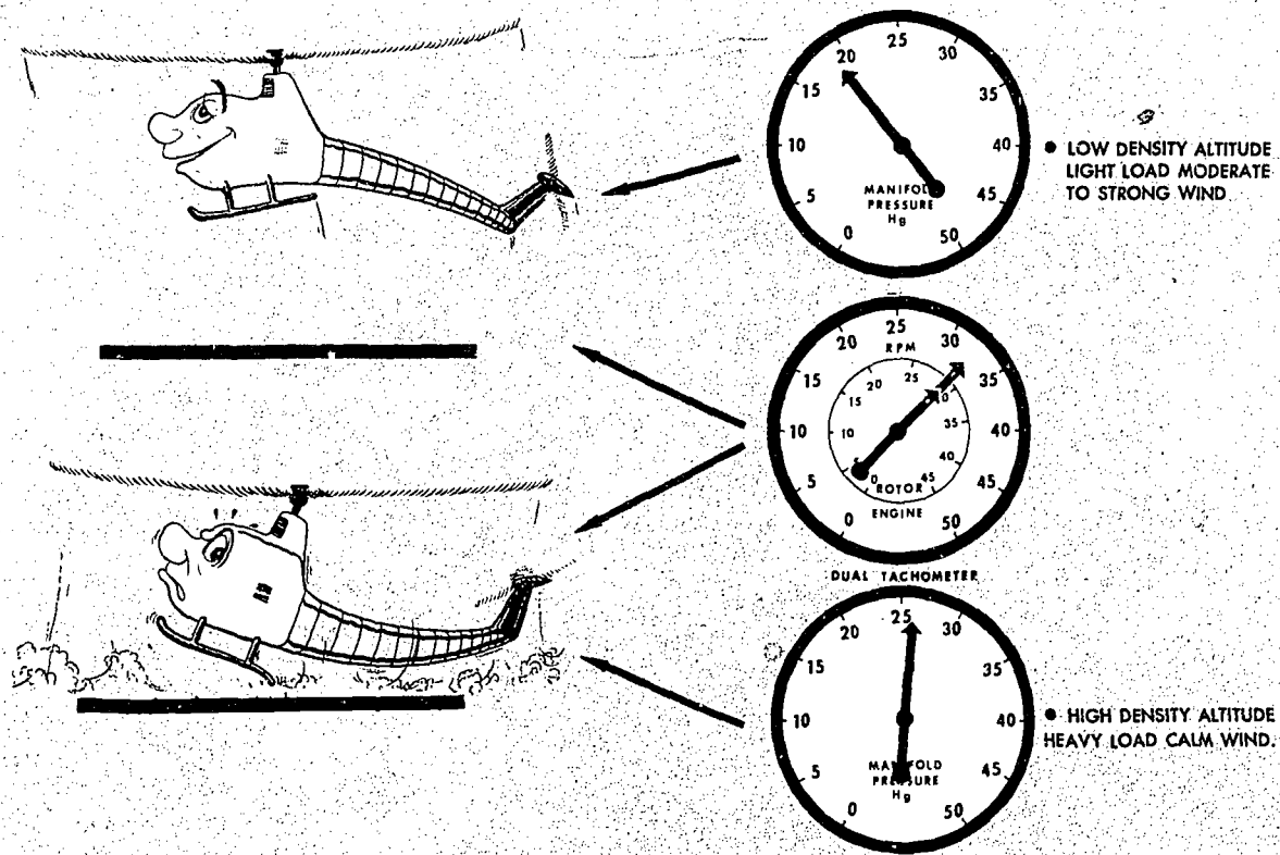
FIGURE 64.—The most adverse conditions for helicopter performance include the combination of high density altitude, heavy load (high gross weight) and calm wind.
