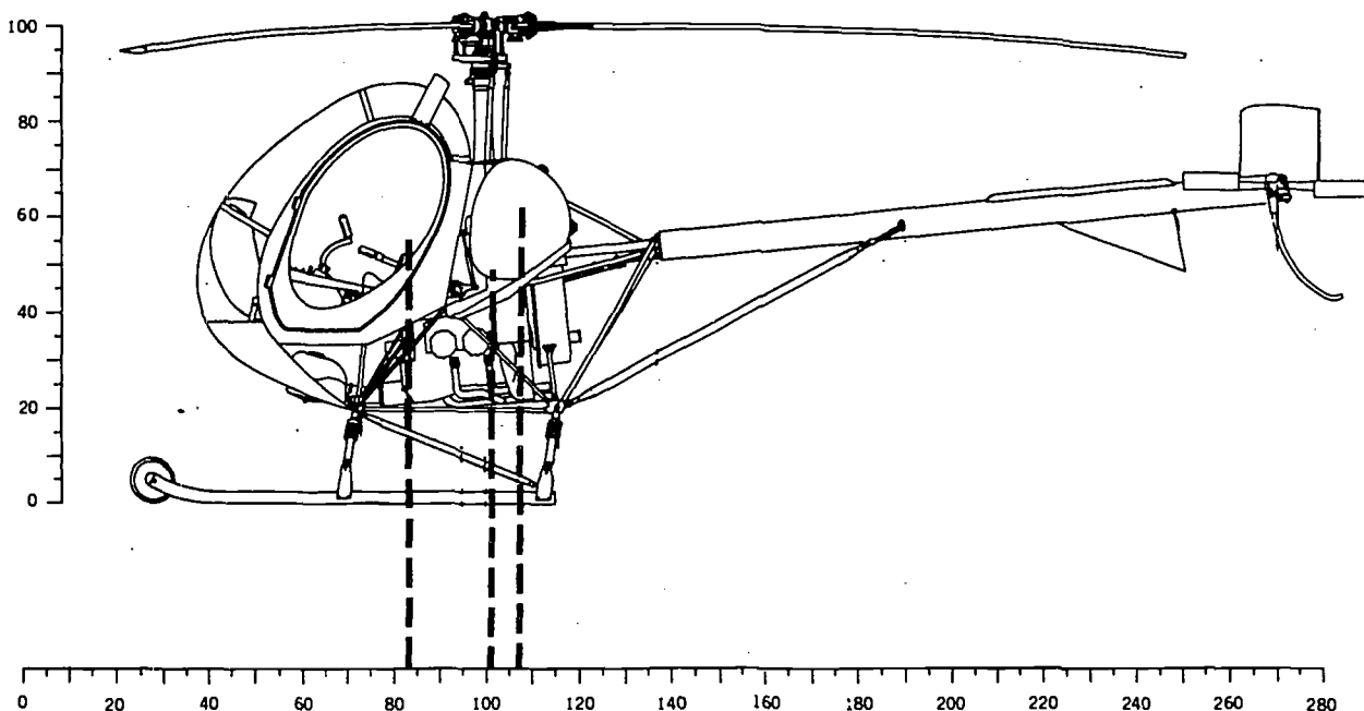
FIGURE 47.—Datum line forward of helicopter.
