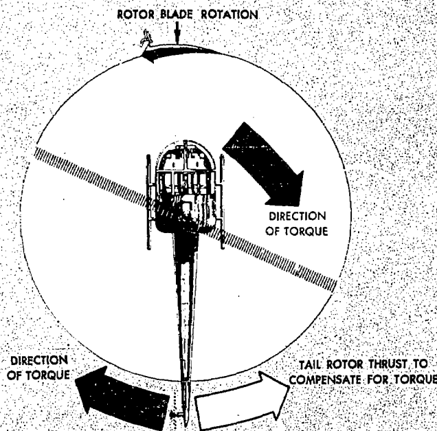
FIGURE 12.—Tail rotor thrust compensates for the torque effect of the main rotor.
