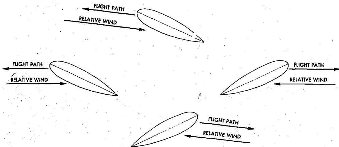
FIGURE 3.—Relationship between the flight path of an airfoil and relative wind. Relative wind is parallel and in the opposite direction to the flight path.
