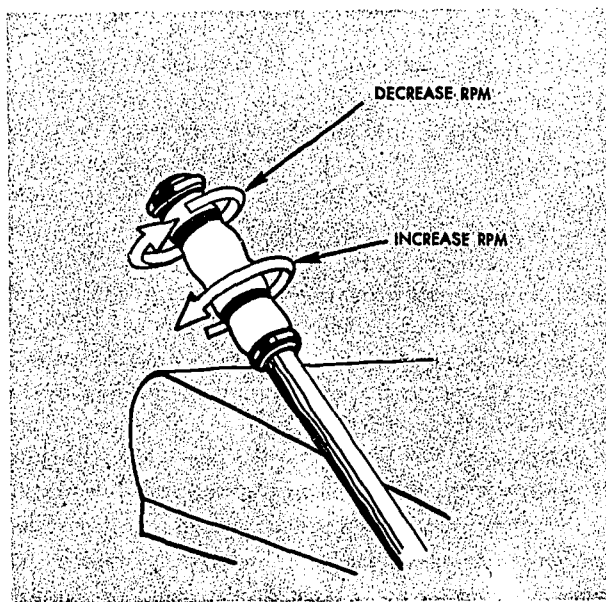
FIGURE 30.—Throttle control: Rotating the throttle outboard (viewed from the top) increases RPM; rotating it inboard decreases RPM.
