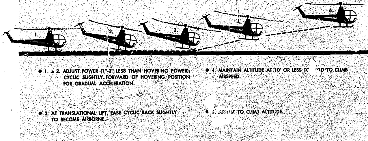
FIGURE 75.—High altitude (running) takeoff.
