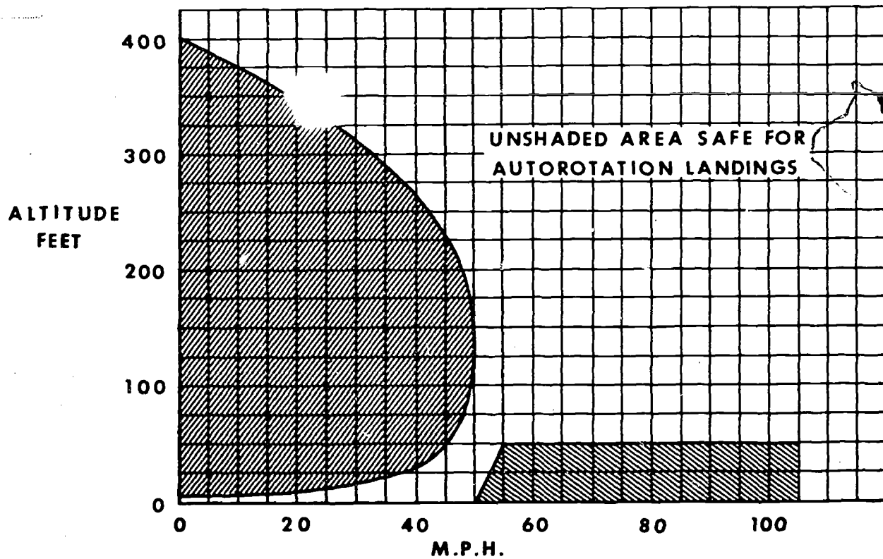
FIGURE 44.—Airspeed vs. altitude limitations chart.
