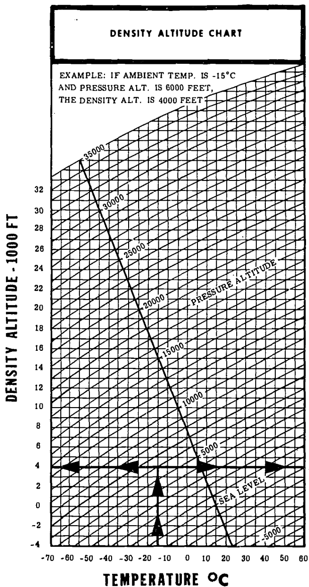
FIGURE 51.—Density altitude chart.
