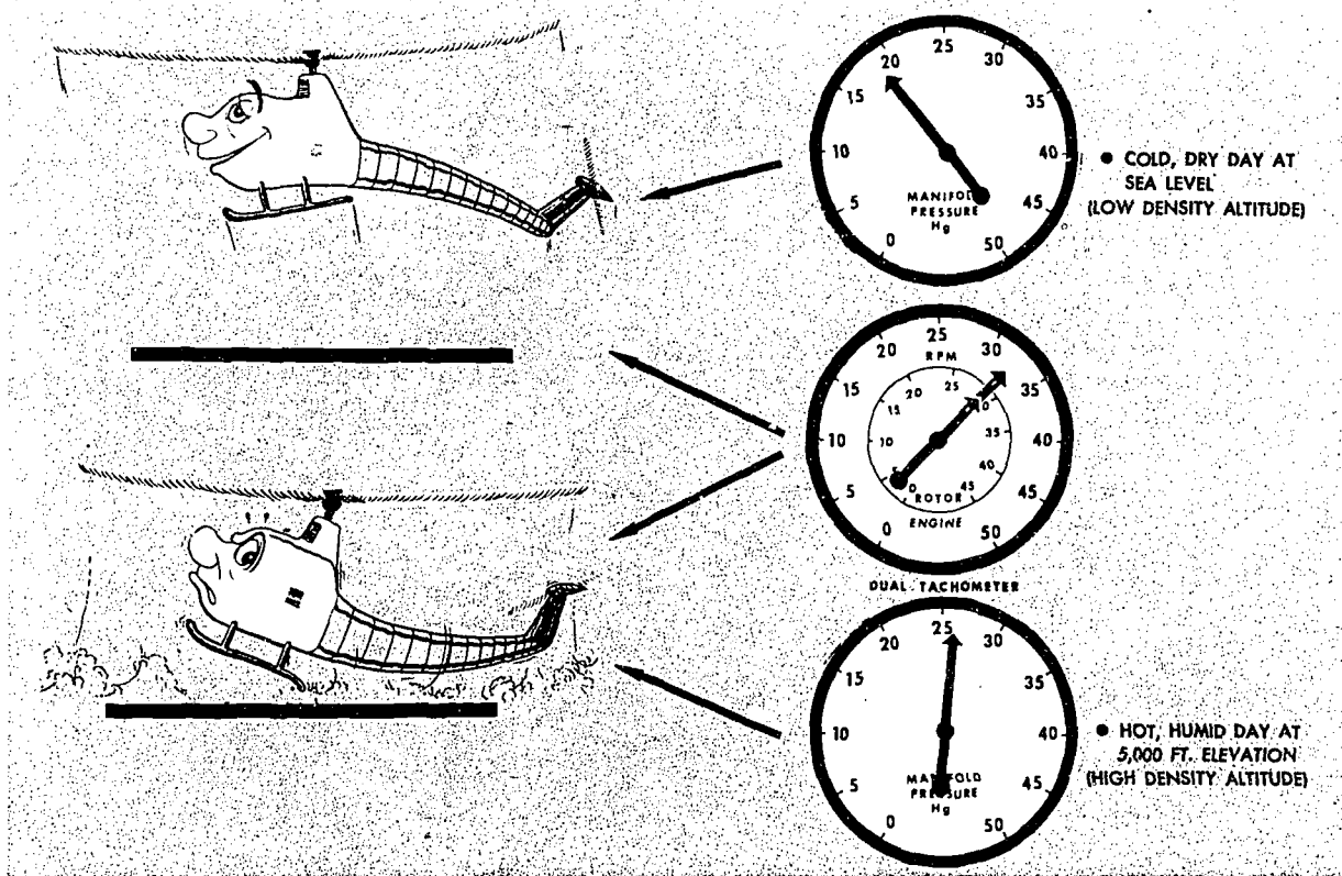
FIGURE 55.—High density altitudes reduce helicopter performance.
