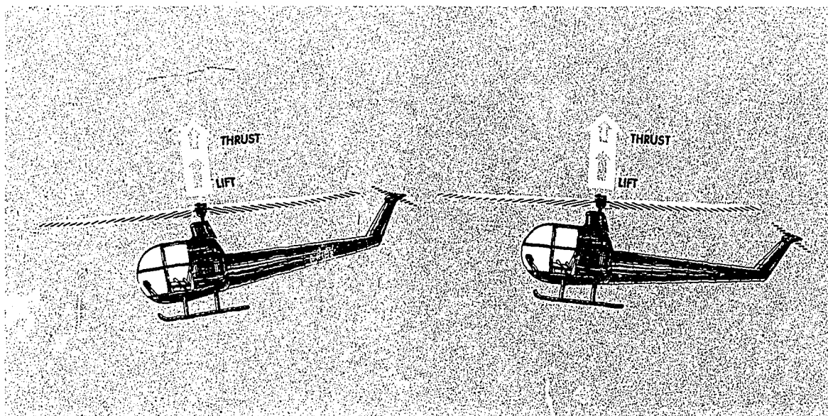
FIGURE 9.—The total lift-thrust force acts perpendicular to the rotor disc or tip-path plane.
