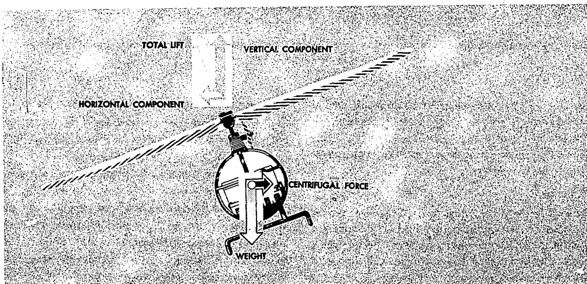
FIGURE 24.—Forces acting on a helicopter in a turn. Lift causes the helicopter to turn when it is banked.
