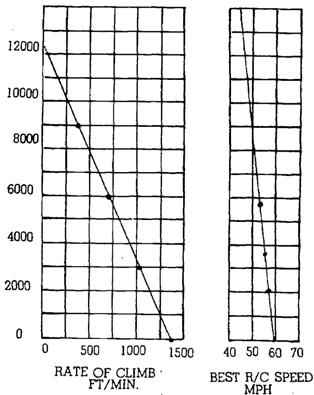
FIGURE 60.—Rate of climb and best rate of climb speed chart.
