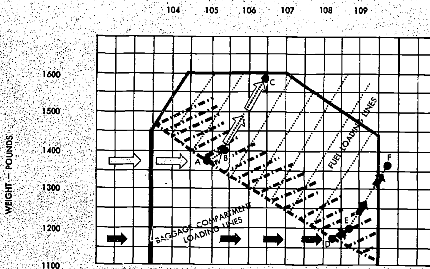
FIGURE 46.—Loading chart illustrating the solution to sample problems 1 and 2.
