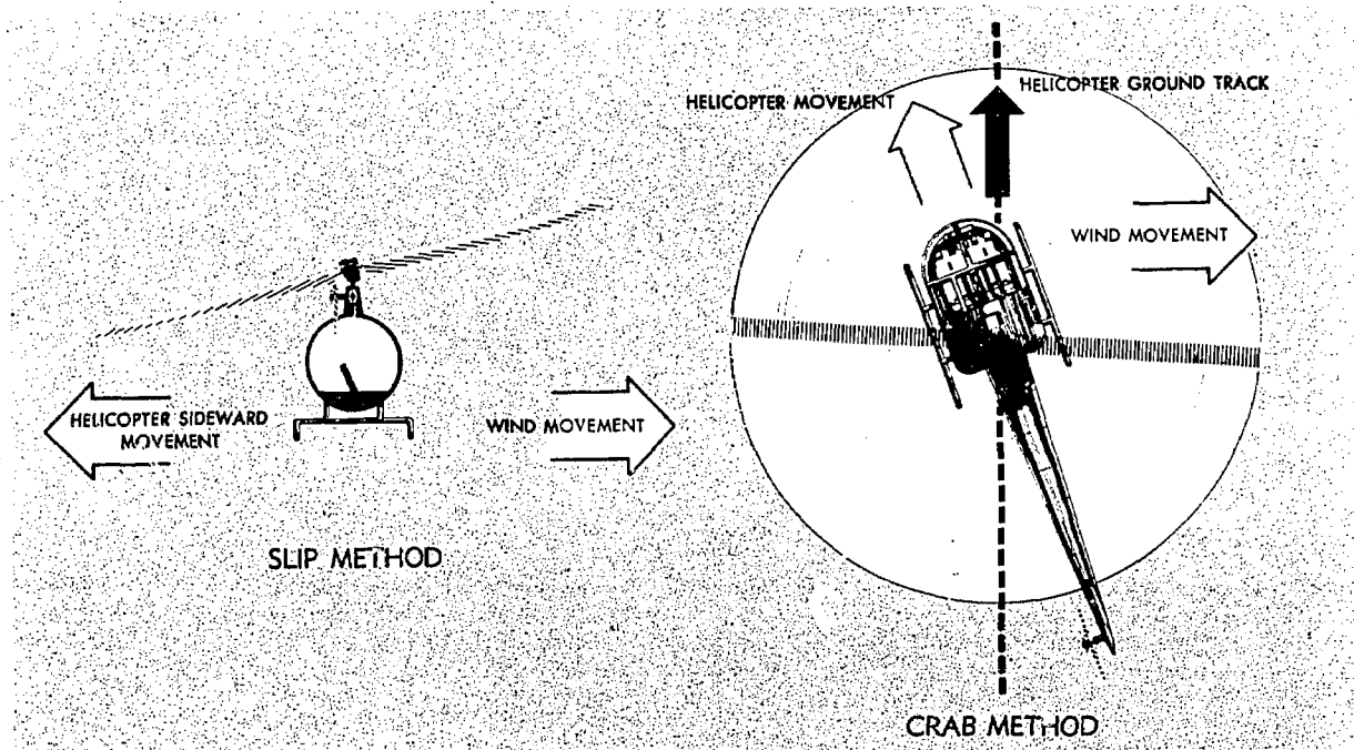
FIGURE 71.—Comparison of the slip method and crab method of wind drift correction.
