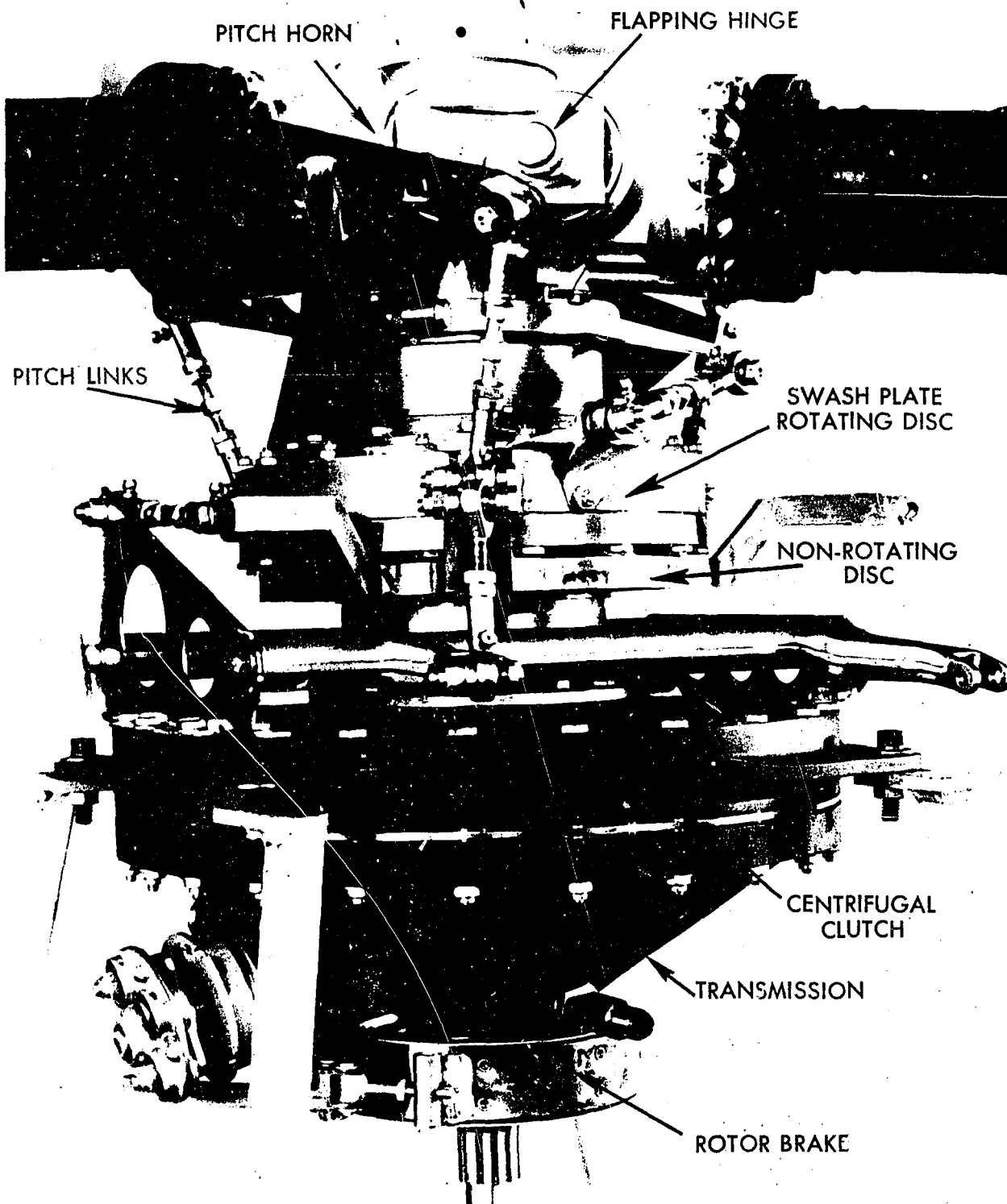
FIGURE 33.—Various components of the rotor system in one helicopter.
