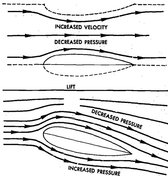
FIGURE 7.—(Top) Bernoulli's Principle: Increased air velocity produces decreased pressure; (Bottom) Lift is produced by an airfoil through a combination of decreased pressure above the airfoil (as per Bernoulli's Principle), and increased pressure beneath.
