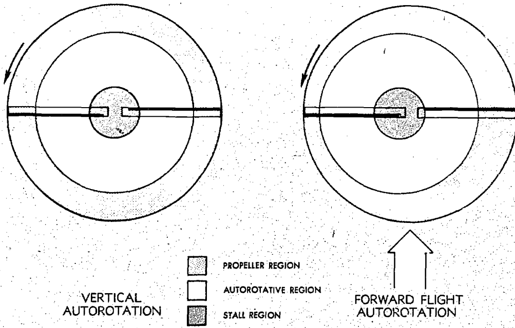
FIGURE 23.—Contribution of various portions of the rotor disc to the maintenance of RPM during an autorotation—vertical autorotation (left); forward flight autorotation (right).
