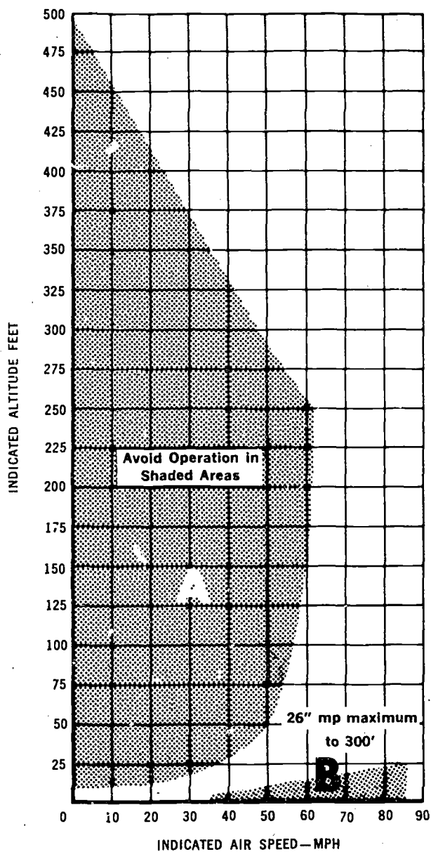
FIGURE 66.—Airspeed vs. altitude limitations chart.
