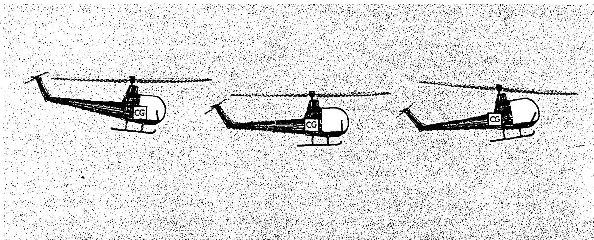
FIGURE 45.—Effect of center of gravity on cyclic stick position and helicopter attitude during hovering flight.
