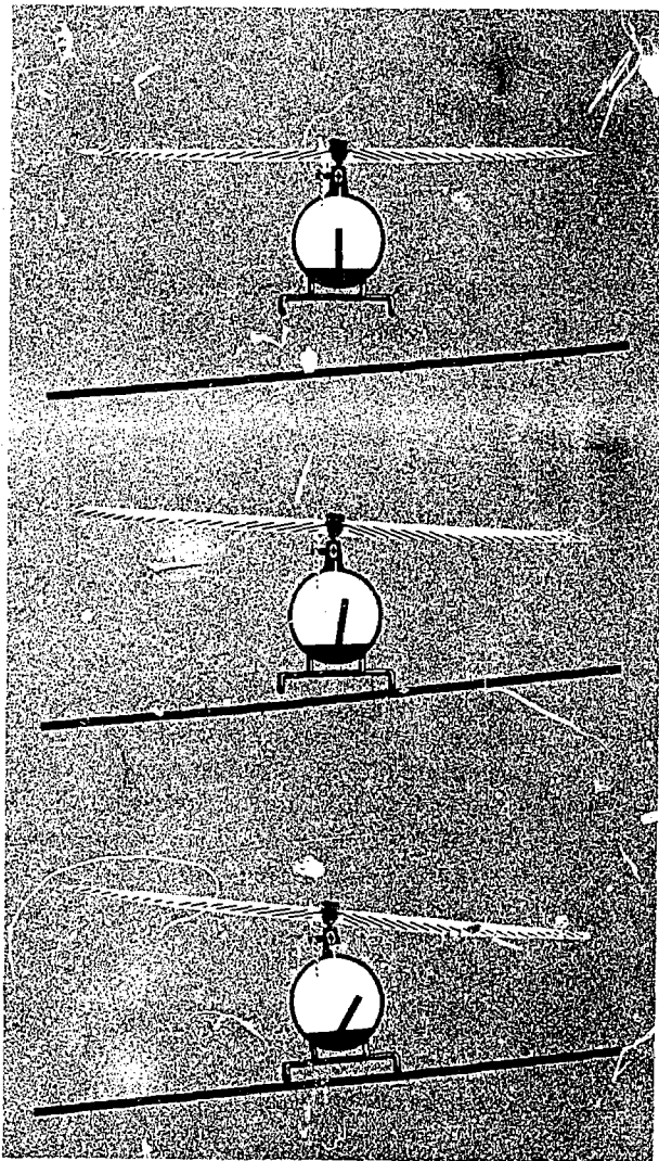
FIGURE 79.—Slope landing or takeoff.
