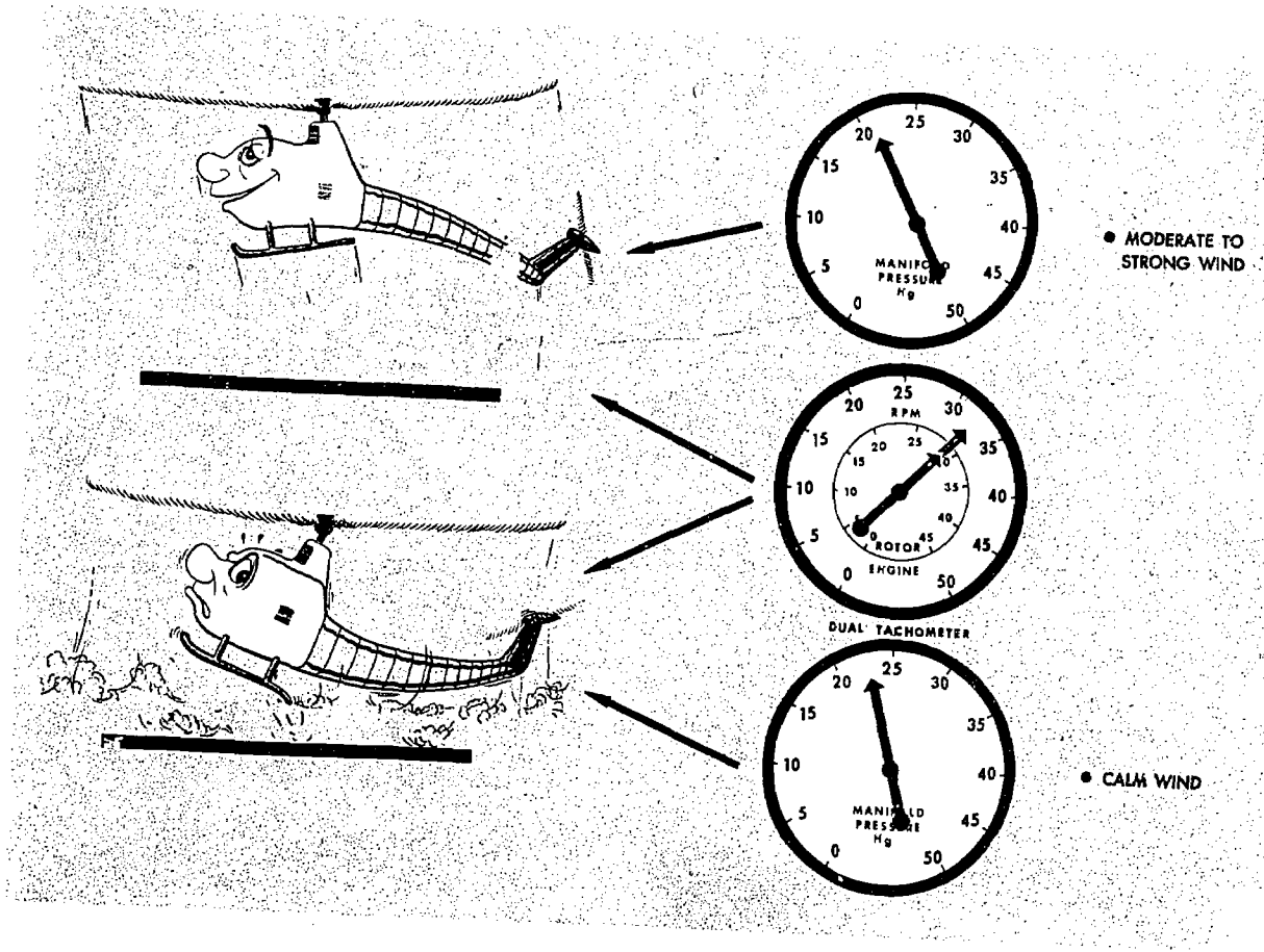
FIGURE 63.—Calm wind reduces helicopter hovering performance.
