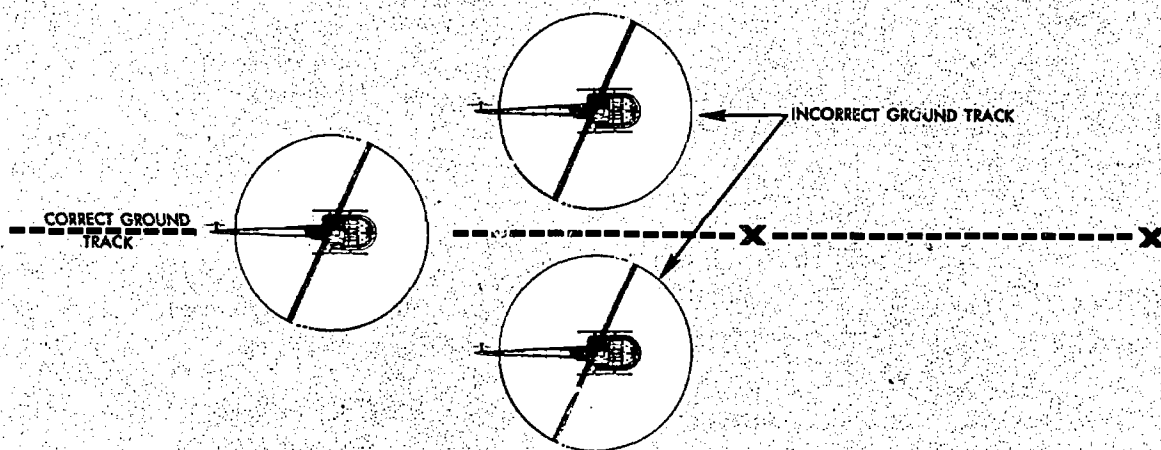
FIGURE 68.—Use of reference points in maintaining proper ground track in forward or rearward hovering flight.
