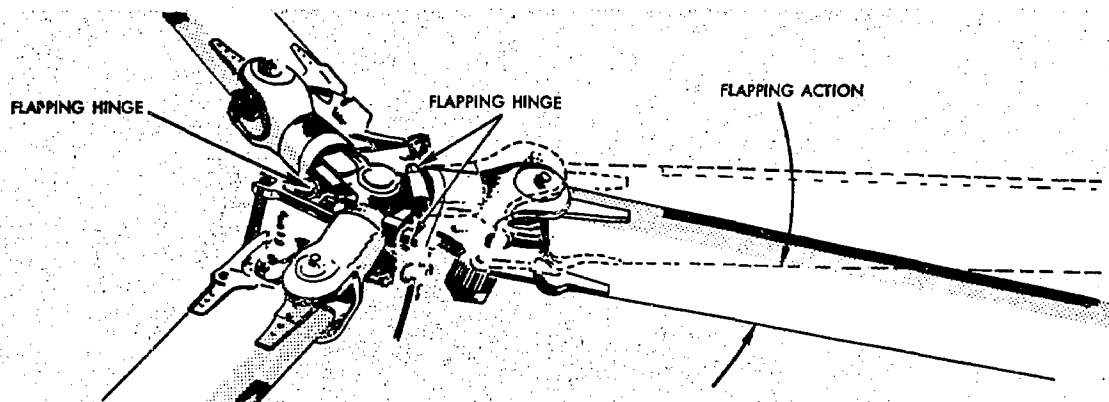
FIGURE 16.—Flapping action about the flapping hinges. Drag hinges can also be seen.
