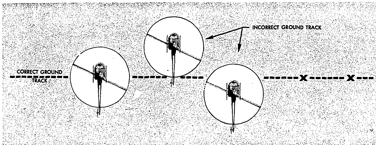
FIGURE 69.—Use of reference points in maintaining proper ground track in sideward hovering flight.
