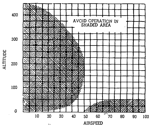
FIGURE 43.—Airspeed vs. altitude limitations chart.
