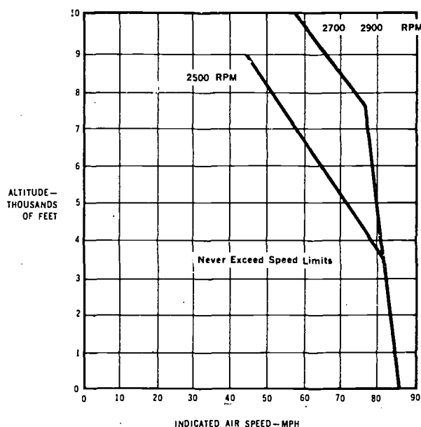
FIGURE 65.—Chart showing never-exceed ( V_{ne} ) speed limits.
