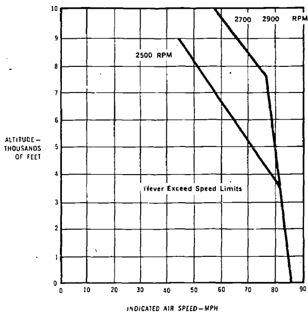
FIGURE 39.—Chart showing never-exceed ( V_{no} ) speed limits.
