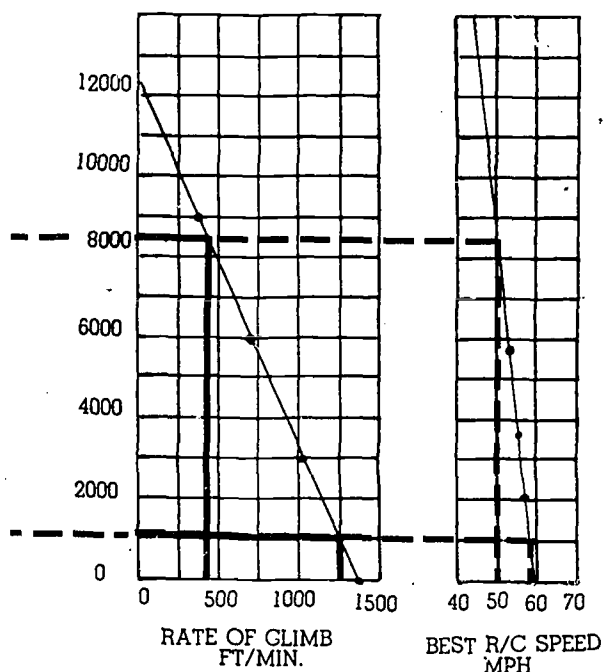
FIGURE 42.—Rate of climb and best rate of climb speed chart.
