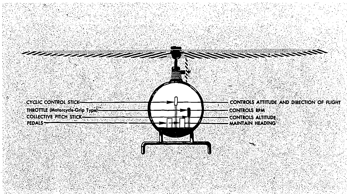
FIGURE 27.—Controls of the helicopter and the principal function of each control.
