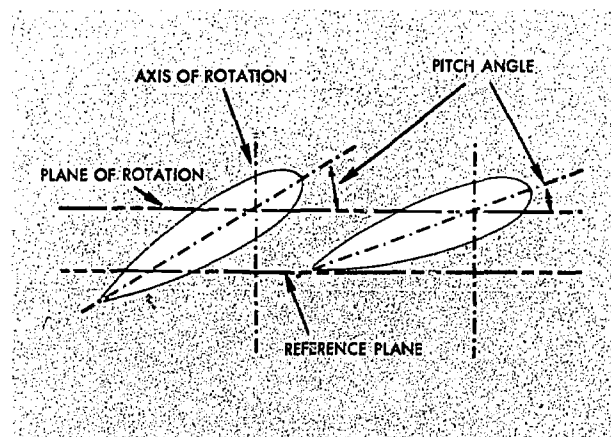
FIGURE 4.—The pitch angle of a rotor blade is the angle between the chord line and a reference plane determined by the rotor hub or the plane of rotation.
