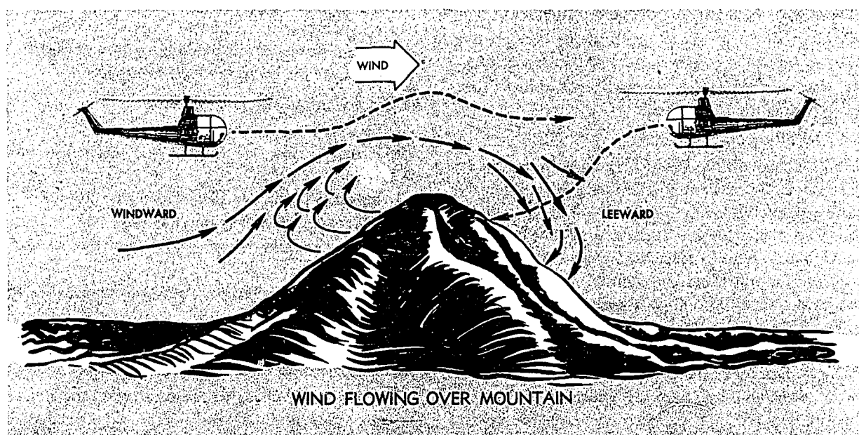
FIGURE 67.—Windflow over mountains and its effect on aircraft in flight.
