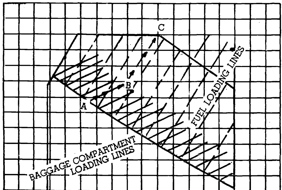
FIGURE 41.—Loading chart.
