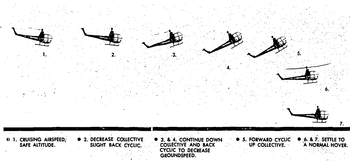
FIGURE 78.—Rapid deceleration or quick stop.
