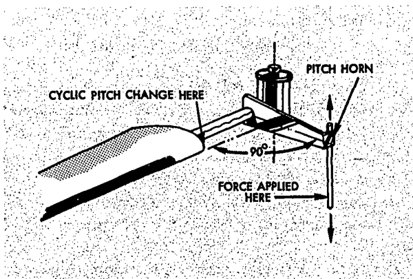
FIGURE 34.—Rotor blade pitch horns are located 90^\circ ahead of or behind (depending on the manufacturer) the rotor blade so that helicopter reaction will be in the direction of cyclic stick displacement.
