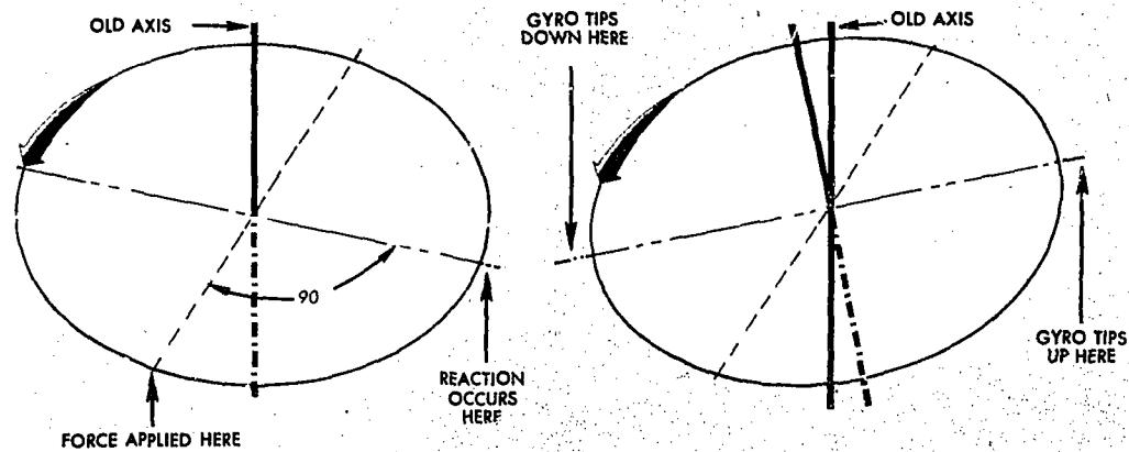
FIGURE 13.—Gyroscopic Precession Principle: When a force is applied to a spinning gyro, the maximum reaction occurs 90^\circ later in the direction of rotation.
