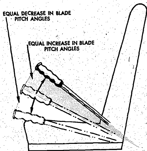
FIGURE 28.—Collective pitch stick movement produces equal changes in blade pitch angles.
