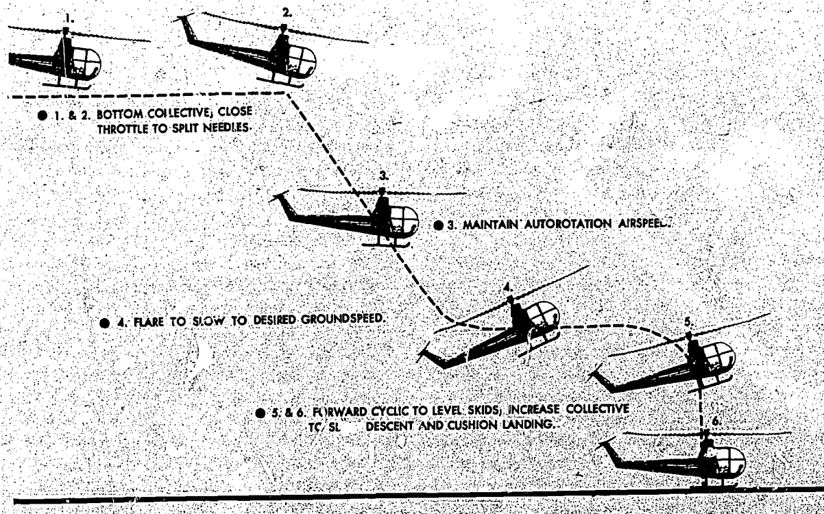
FIGURE 77.—Flare autorotation and touchdown.
