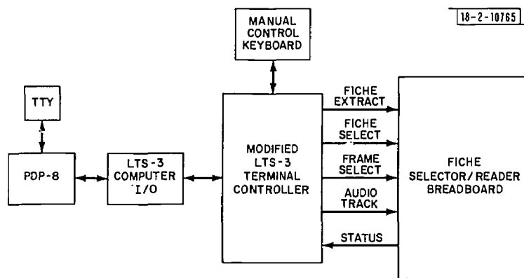
Fig. 2. LTS-4 breadboard control system.
