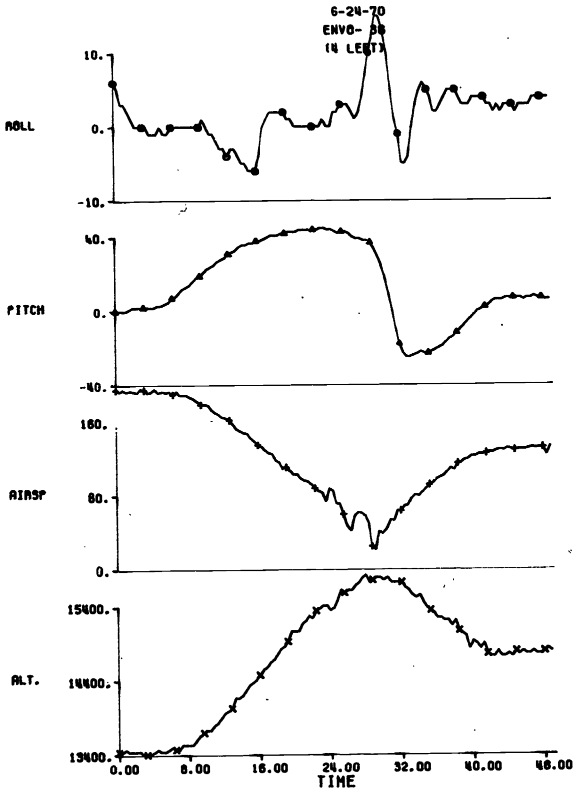
Figure 72. Stall
