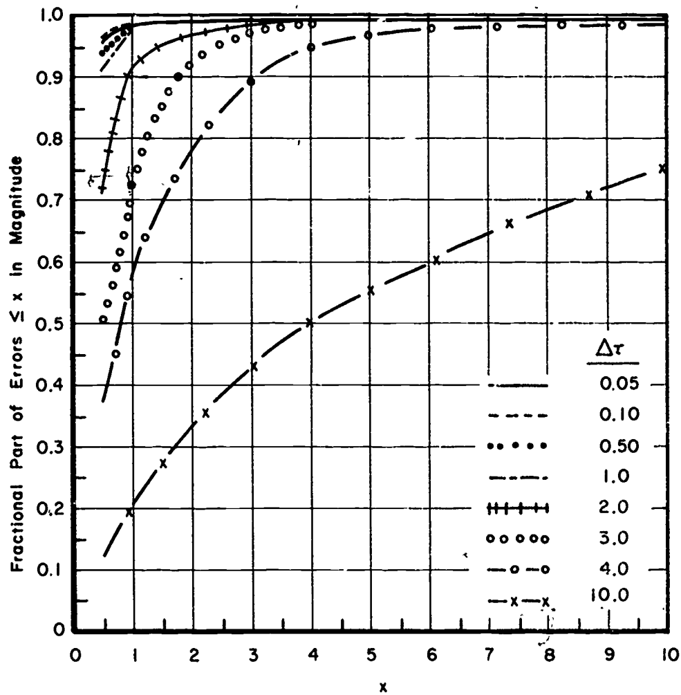
Figure 9. Sampling Interval Plot for Pitch (Lazy 8, N = 46)
