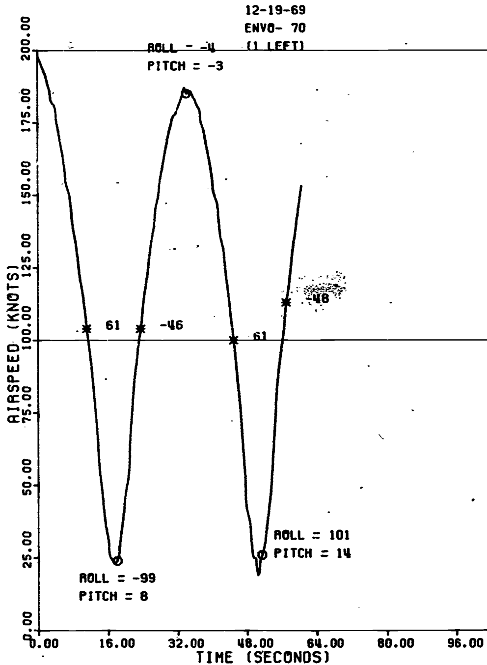
Figure 41. Airspeed Plot
