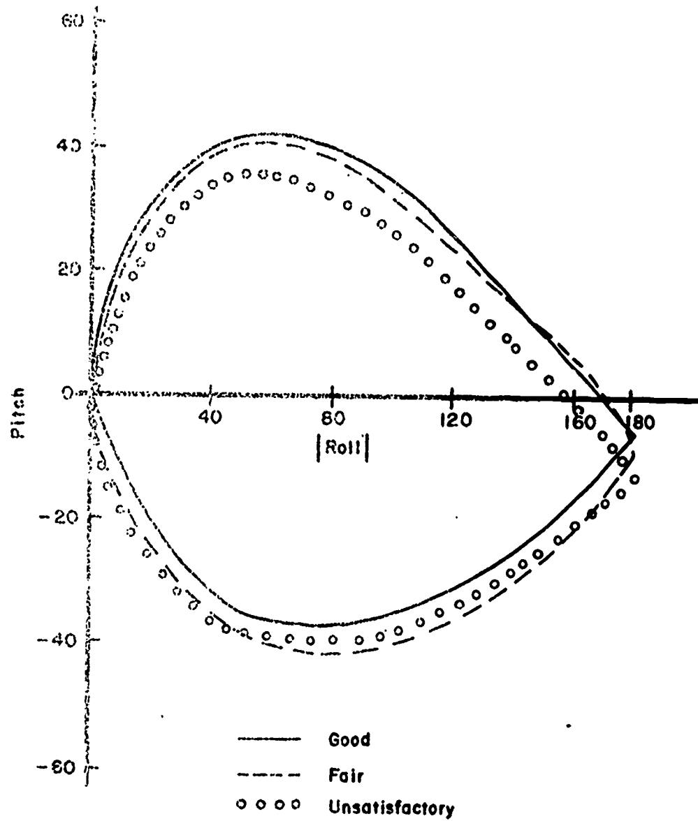
Figure 68. Average Student Barrel Roll Performances
