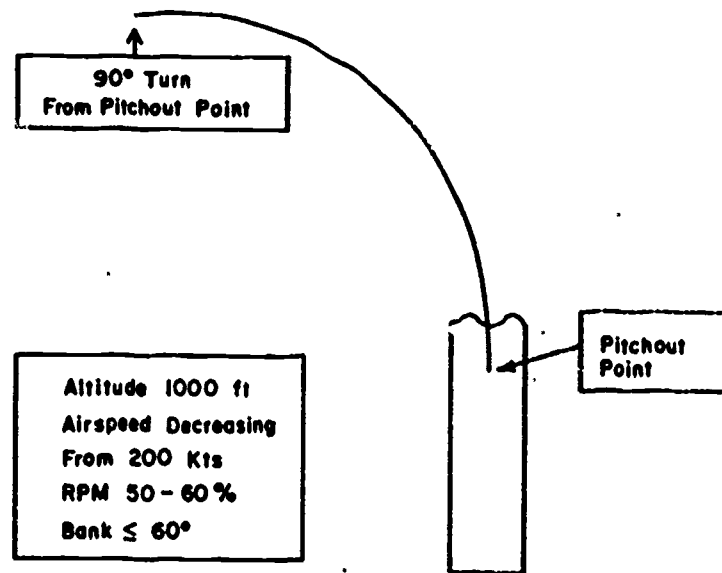
Figure D. Pitchout and 1st Quarter Turn Phase of 360° Overhead Pattern
