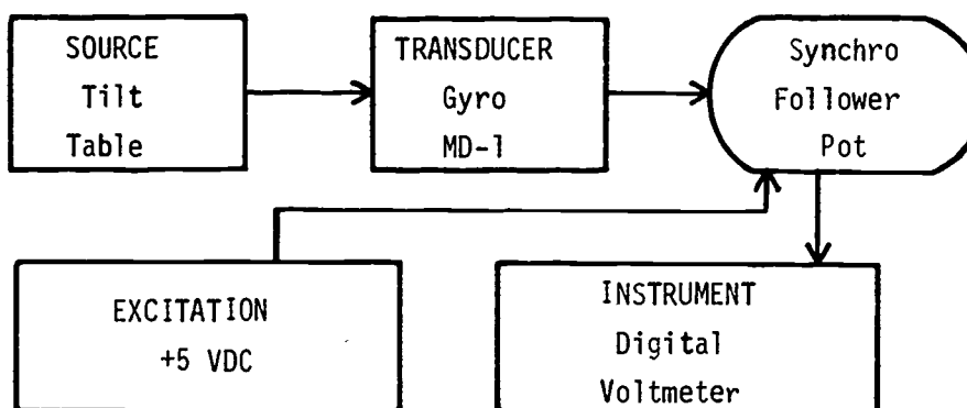
Calibration Block Diagram
