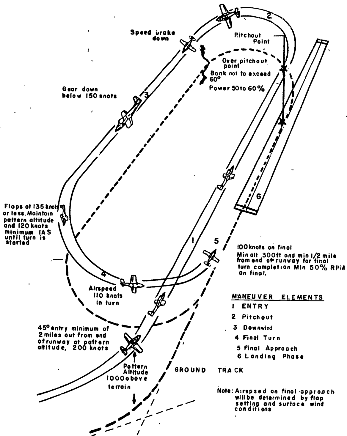
Figure 13. Normal Landing Maneuver Profile
