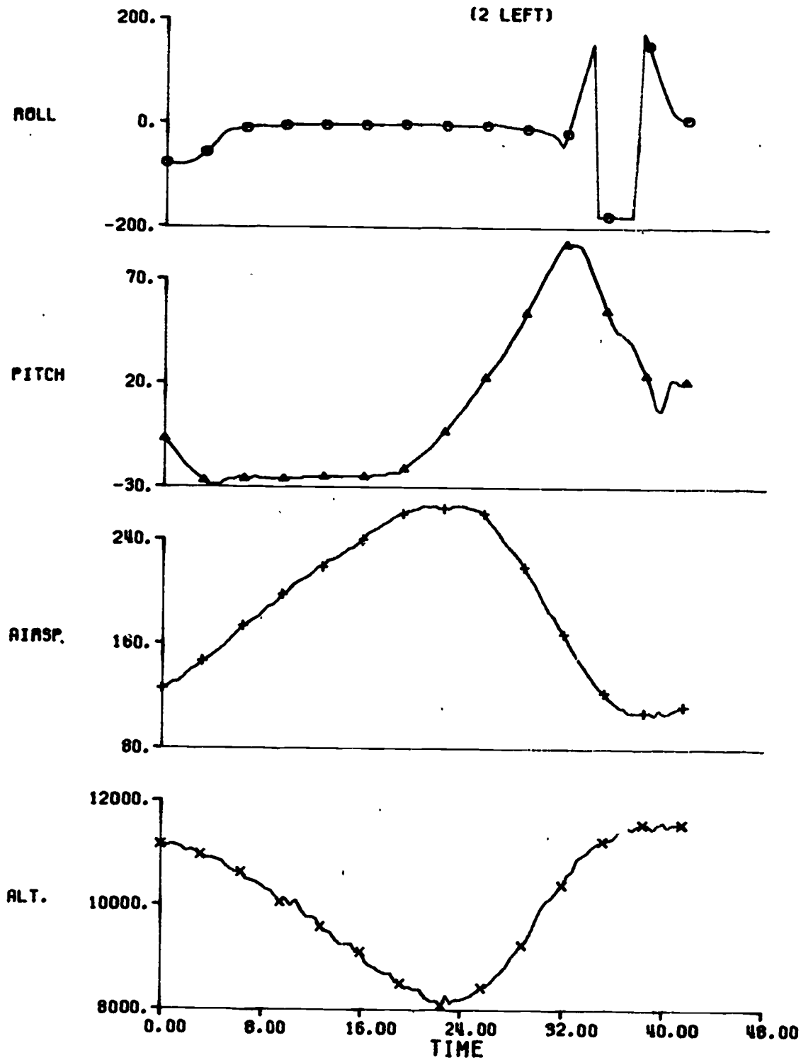
Figure 75. Immelmann
