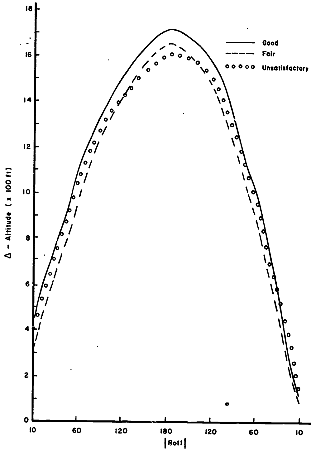
Figure 69. Average Altitude Excursions for Student Barrel Rolls
