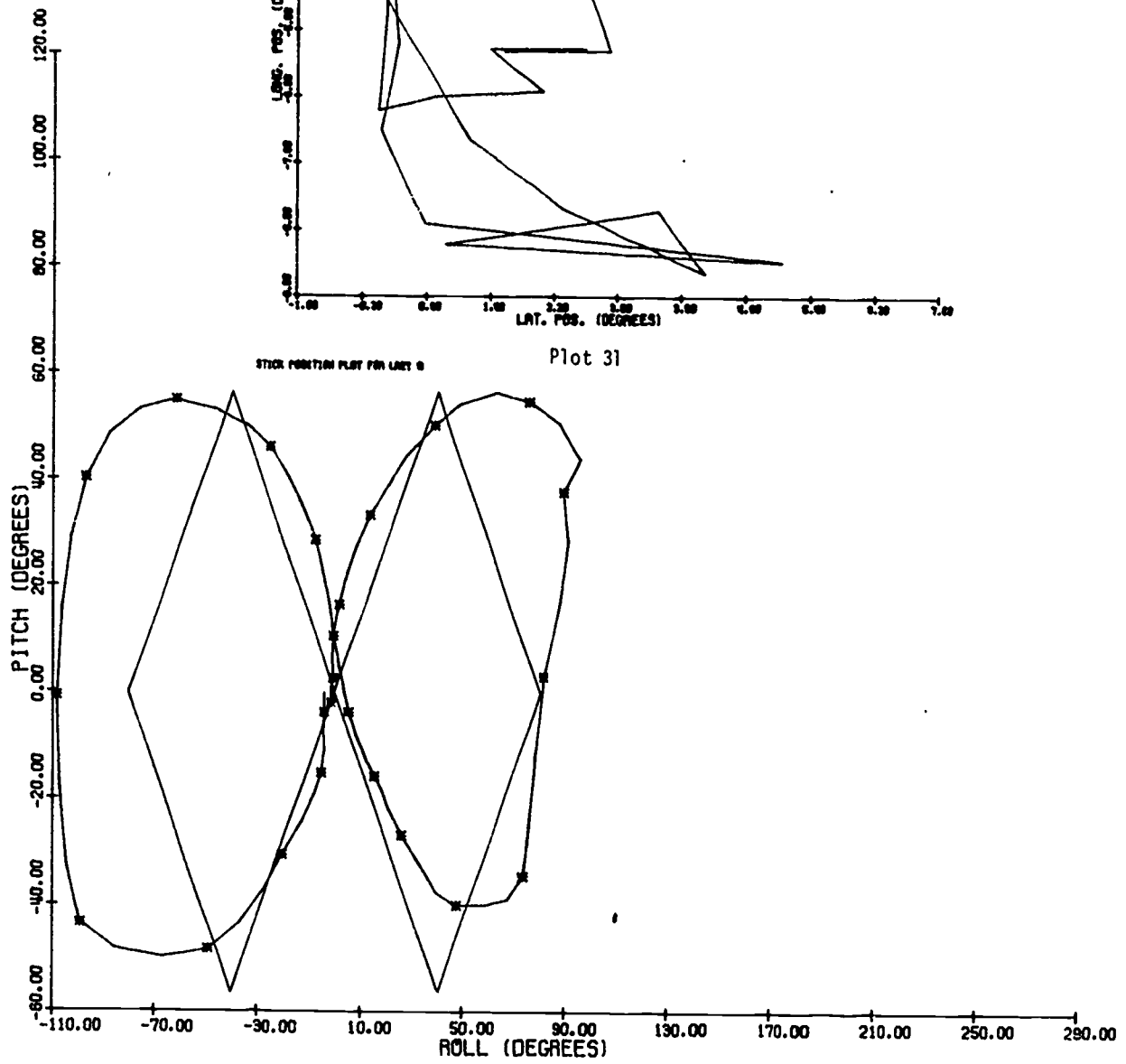
ROLL VS. PITCH FOR LAZY 8
