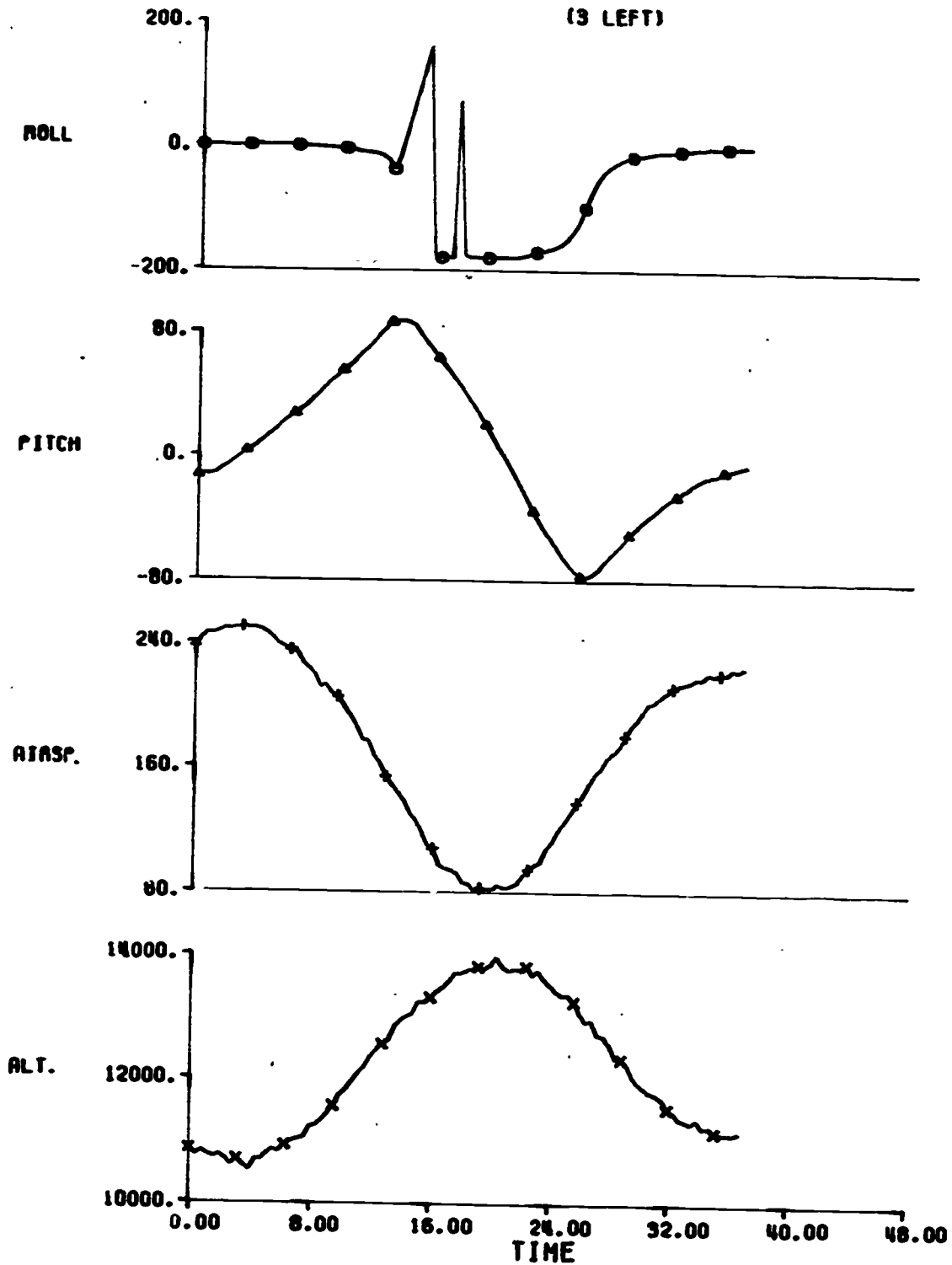
Figure 71. Loop
