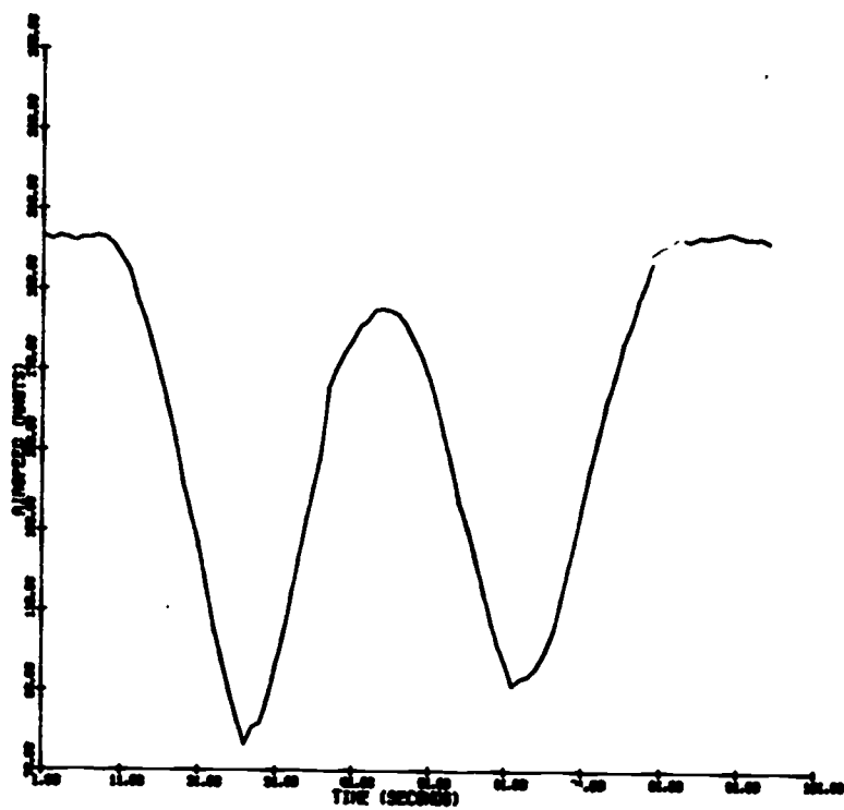
Figure 23. Airspeed vs Time for Lazy 8
