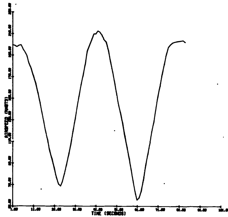
Figure 30. Airspeed vs Time for Lazy 8
