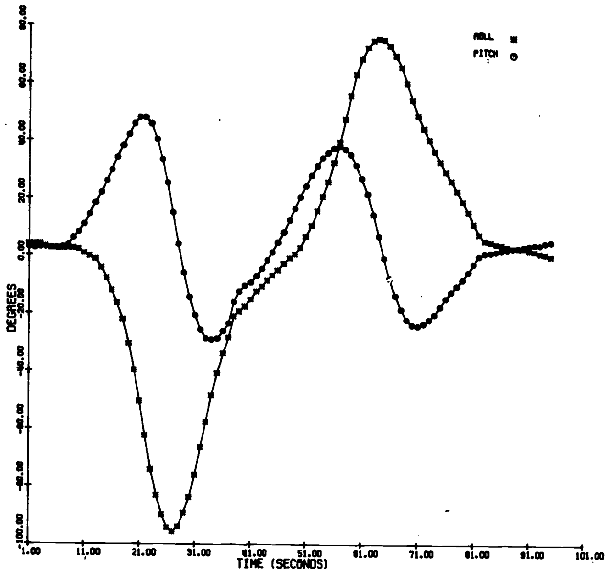
Figure 21. Roll and Pitch vs Time for Lazy 8
