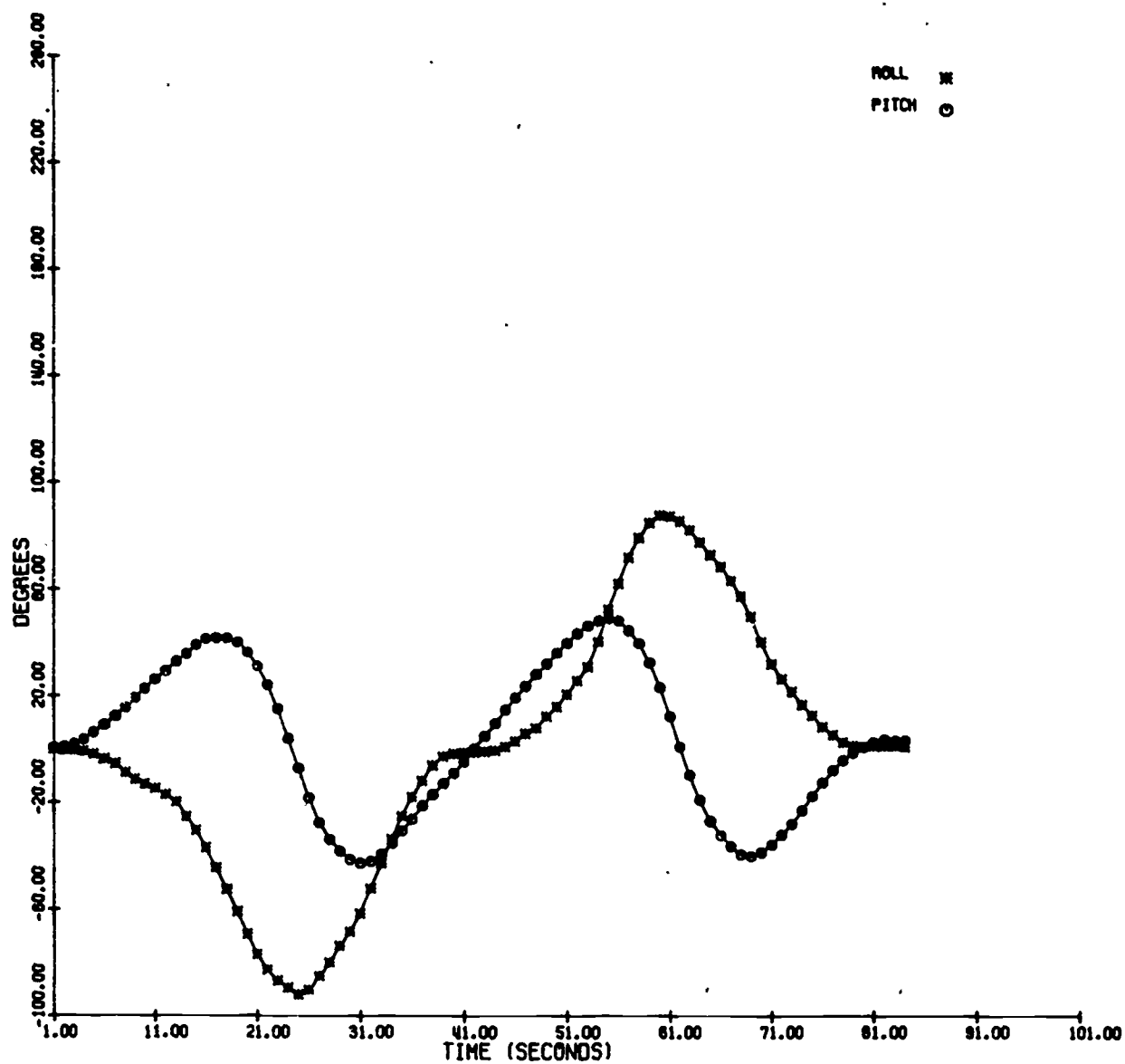
Figure 28. Roll and Pitch vs Time for Lazy 8
