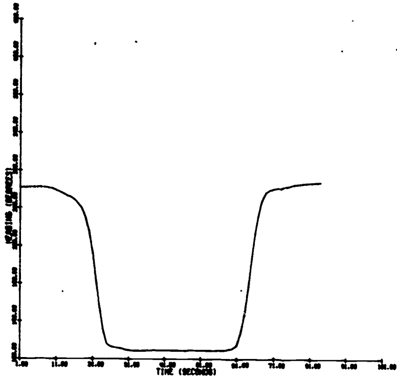
Figure 31. Heading vs Time for Lazy 8
