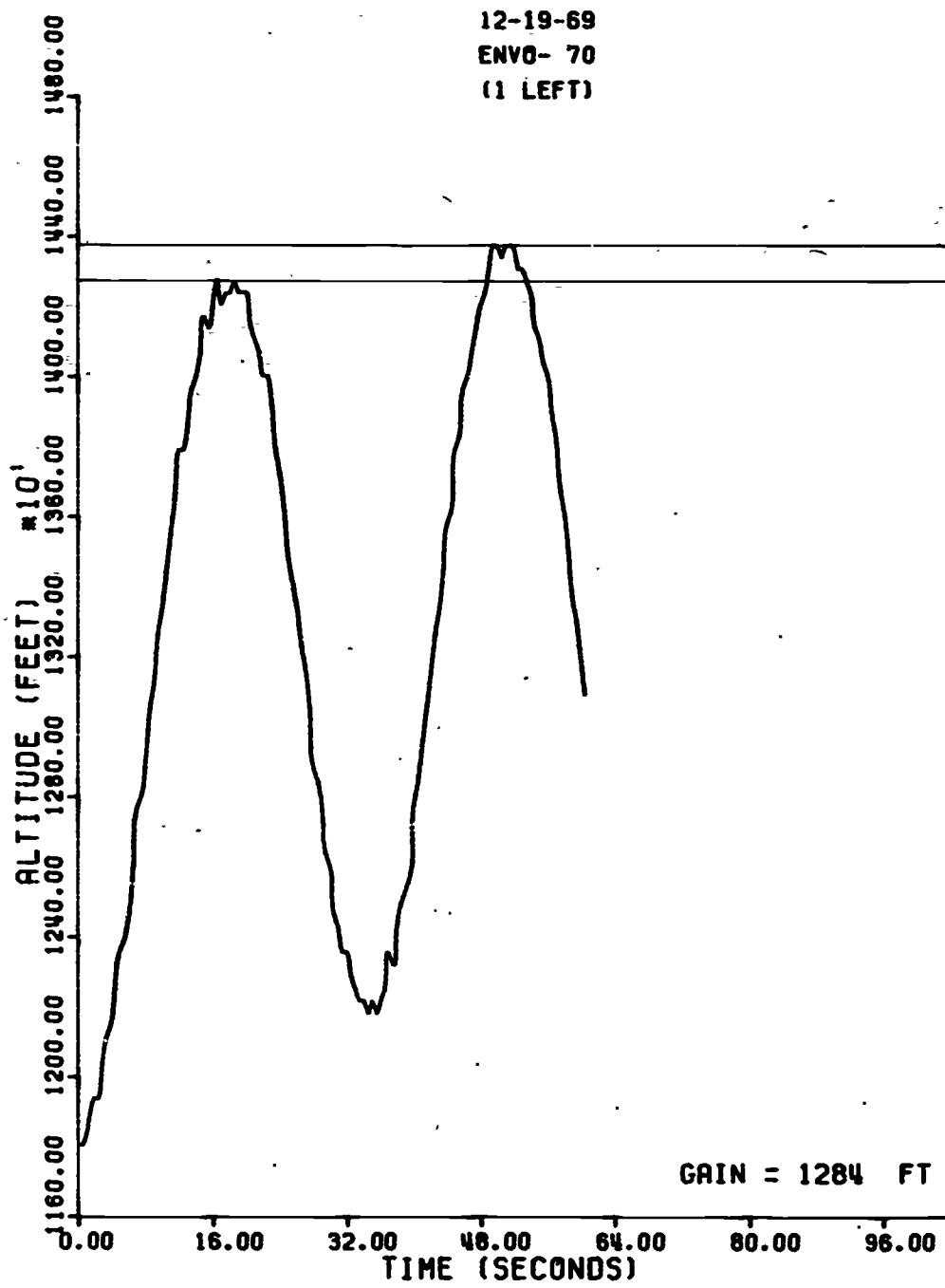
Figure 42. Altitude Plot
