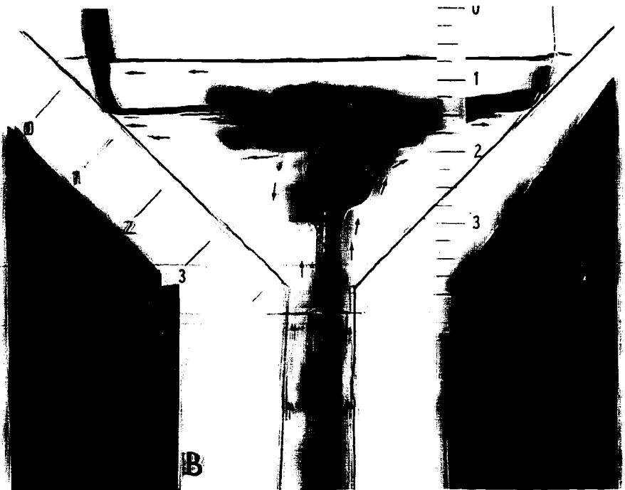
In a laboratory study of thermal convection patterns, crystals in fluids simulating natural minerals and molten rock, rise from a heated base to the cooled roof and then drop in teardrop-like density currents and flow patterns.
