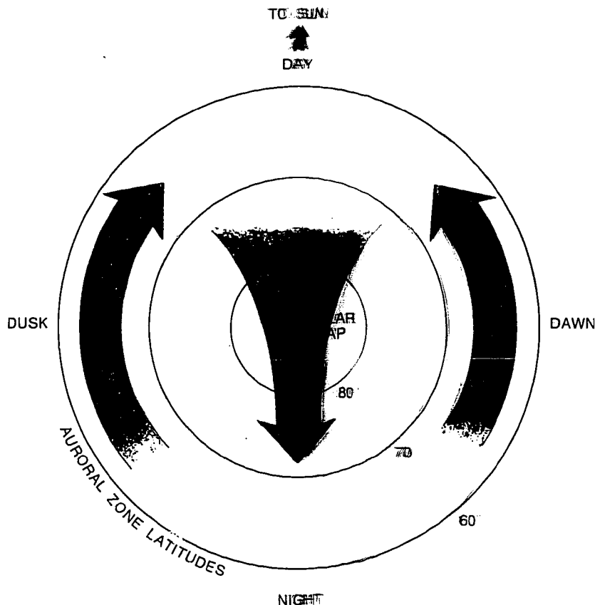
At the earth's high latitudes, the magnetospheric plasma moves in paths away from the sun across the polar cap and returns toward the sun in the auroral zone latitudes (around 60° to 70° geomagnetic), in the twilight regions of dawn and dusk.
