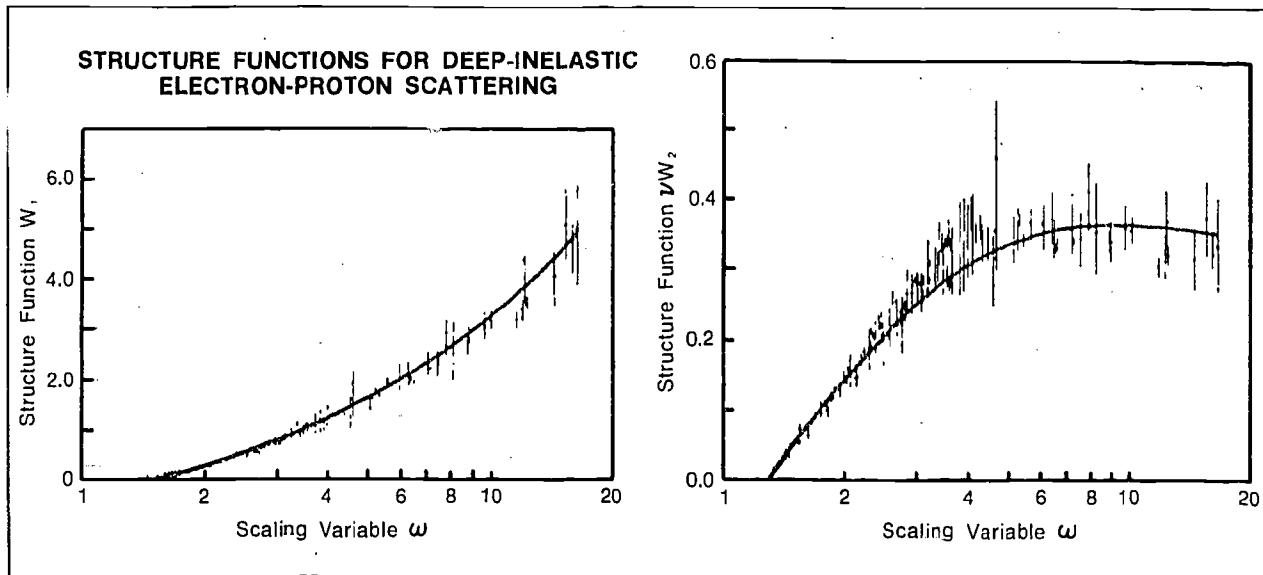
These experimental measurements show the "structure" functions that determine the inclusive cross section for deep inelastic scatterings. Arbitrary points points on these graphs are measured at grossly different values of energy and momentum transfer, but at neighboring values of their dimensionless ratio—the scaling variable \omega . The fact that these points define approximately smooth curves rather than scatter uniformly over the graph is a verification of the scaling hypothesis.
