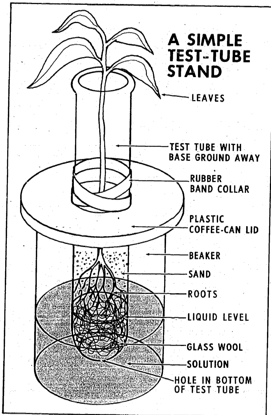
Figure 4 - A simple test tube stand.
