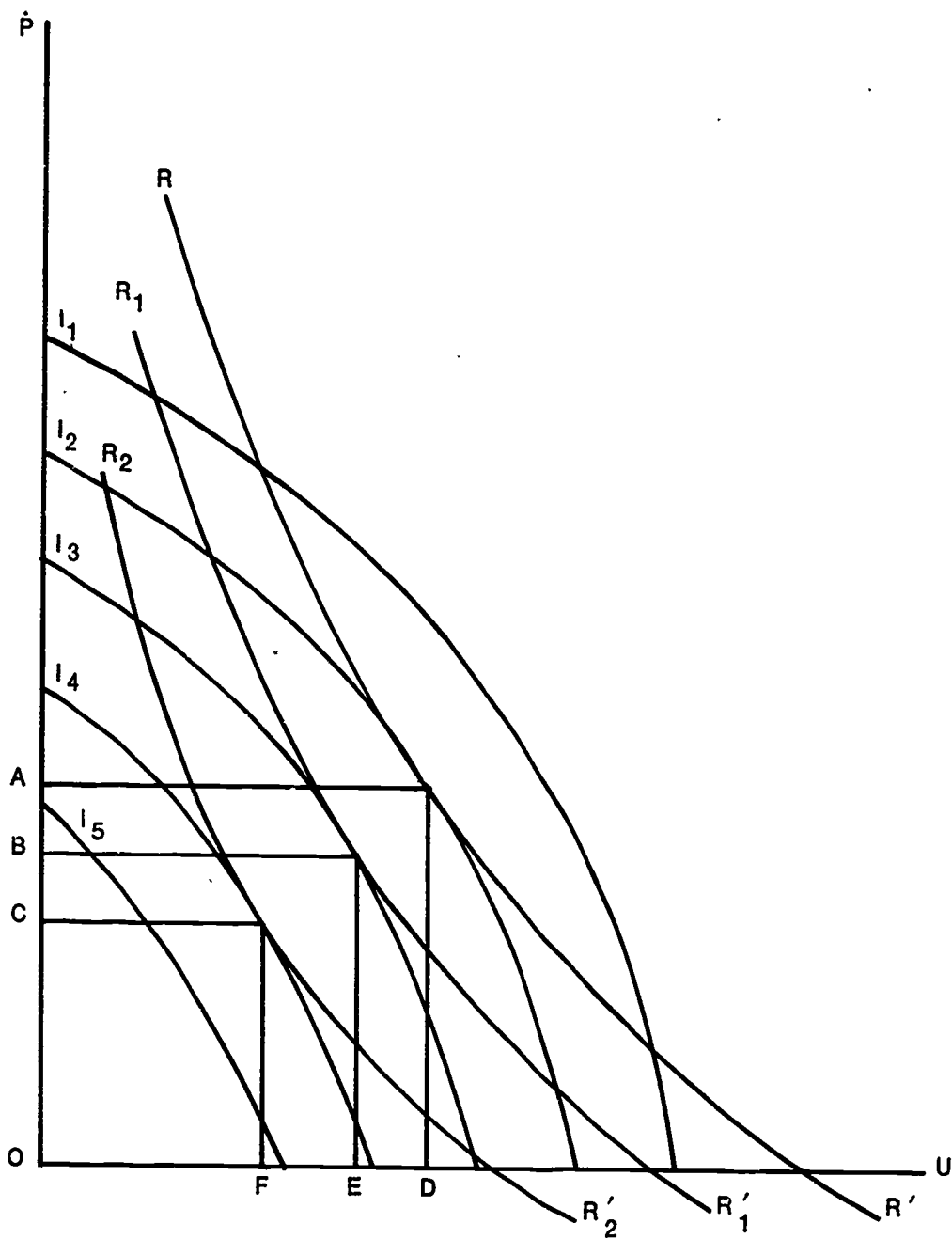
FIGURE 2.4 Price inflation and unemployment: the behavioural trade-off functions and the policy-makers' preference functions
