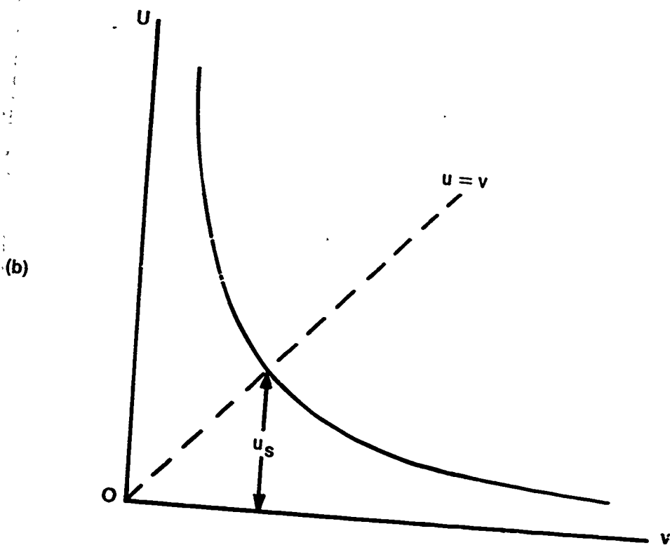
FIGURE 3.2 The cyclical relationship of the unemployment rate, u , and the vacancy rate, v , (a) to relative labour demand, d , and (b) to each other
