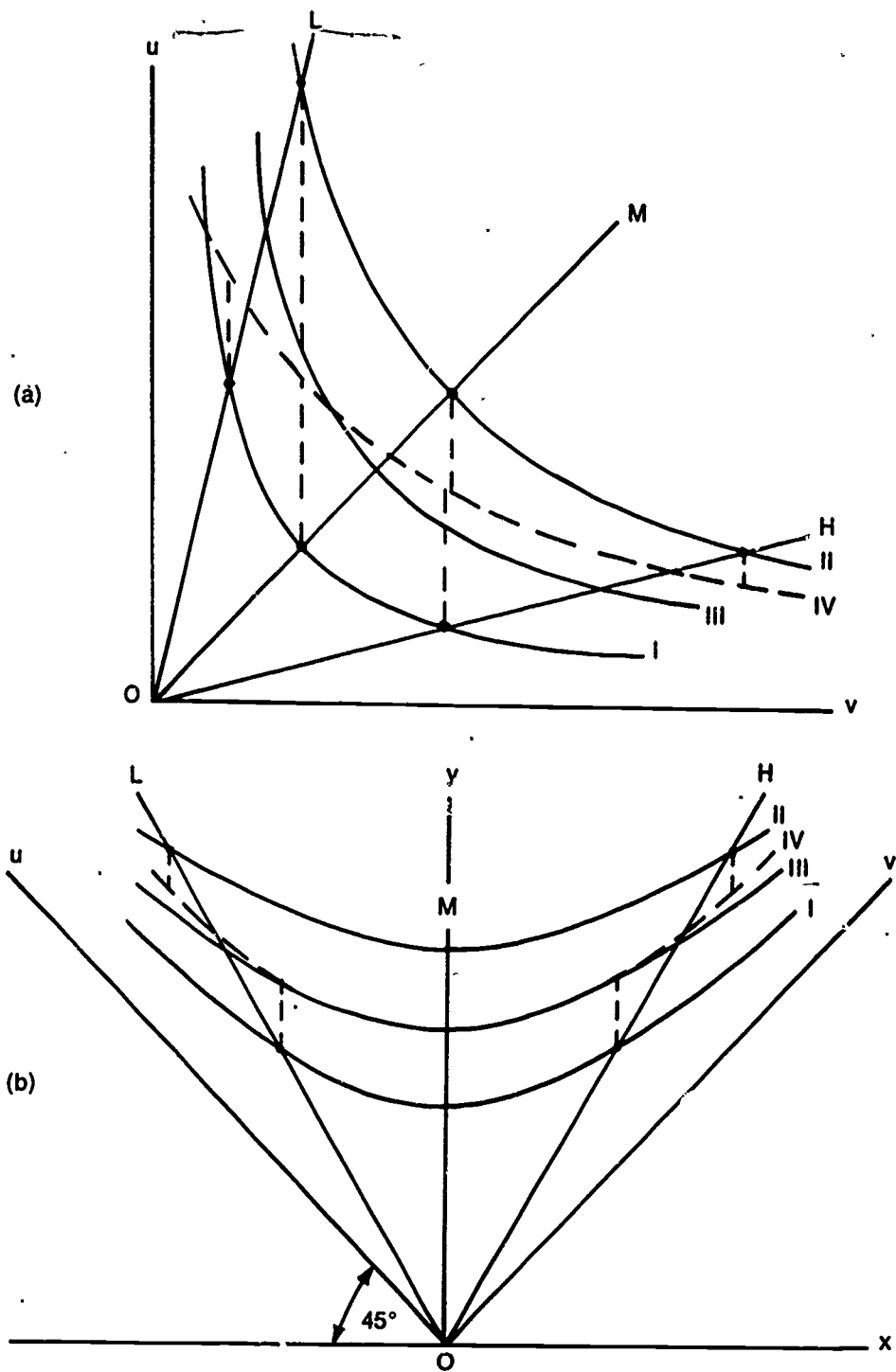
FIGURE 4.1 The effect of minimizing the residuals in the unemployment-vacancy relationship in the cases of (a) a hyperbolic function and (b) a parabola rotated by 45^\circ
