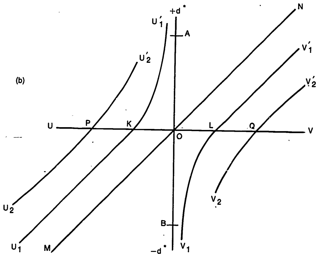
FIGURE 2.2 The Dow-Dicks-Mireaux system of functions: (a) the unemployment-vacancy functions; (b) the unemployment-demand and vacancy-demand functions
