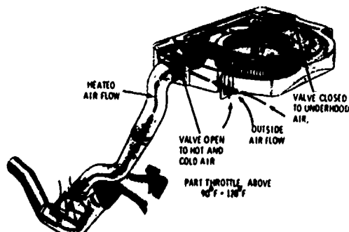
THERMOSTATIC AIR CLEANER ABOVE 90-120°F.
