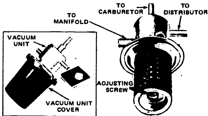
VACUUM CONTROL VALVE ADJUSTMENT
