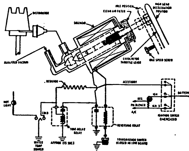
COMBINATION EMISSION CONTROL (C.E.C.) SYSTEM
