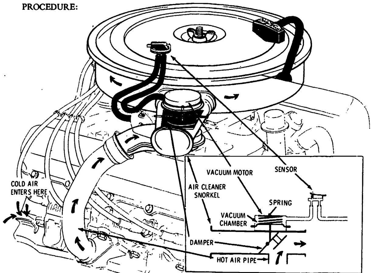
THERMOSTATICALLY CONTROLLED AIR CLEANER ASSEMBLY
