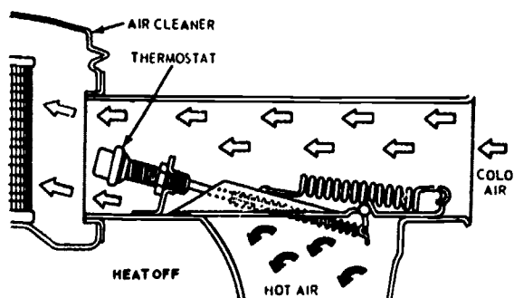
TEMPERATURE OPERATED DUCT & VALVE ASSEMBLY
