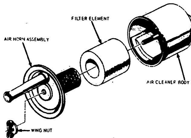
1966-67 THERMACTOR AIR PUMP AIR CLEANER
