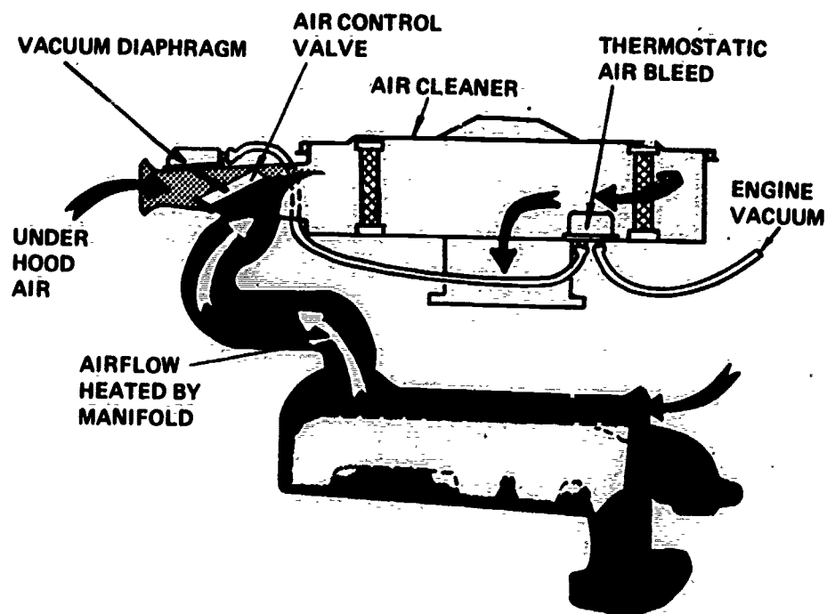
BASIC CHRYSLER HEATED AIR INLET SYSTEM
