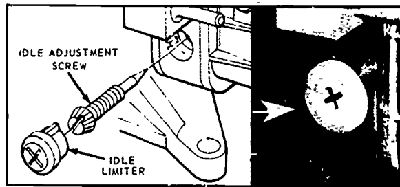
HOLLEY COBRA JET CARBURETORS IDLE MIXTURE SCREWS & LIMITER STOPS
