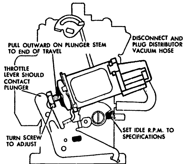
C.E.C. VALVE ADJUSTMENT (TYPICAL)
