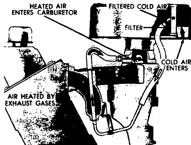
ANTI-ICING DEVICE
