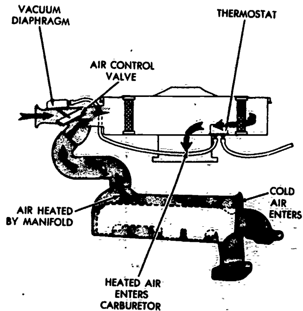
THERMOSTATIC CONTROLLED AIR CLEANER
