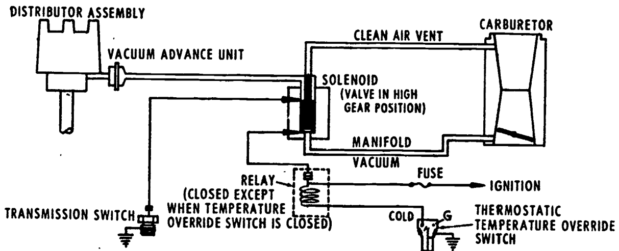
TYPICAL T.C.S. SYSTEM (OVERRIDE RELAY AND SWITCH ON VEGA ONLY)
