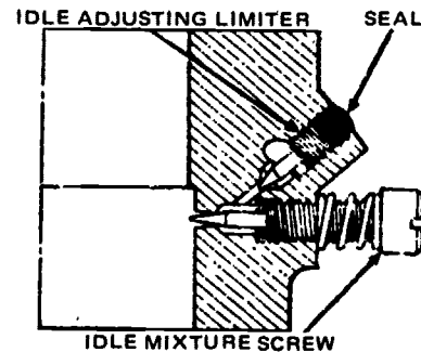
CARTER CARBURETORS IDLE MIXTURE SCREW, LIMITER & SEAL
