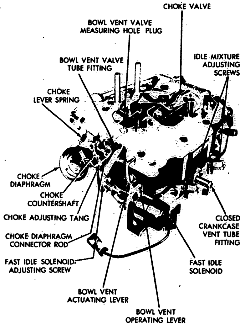
CARTER THERMO-QUAD CARBURETOR
