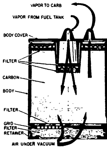
TWO TUBE CANISTER
