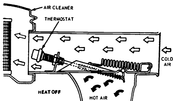
DUCT AND VALVE ASSEMBLY
