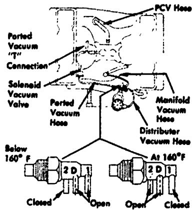
COOLANT TEMPERATURE OVERRIDE SWITCH
