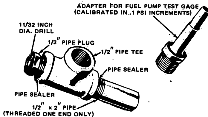
AIR-SUPPLY PUMP TEST GAGE ADAPTER
