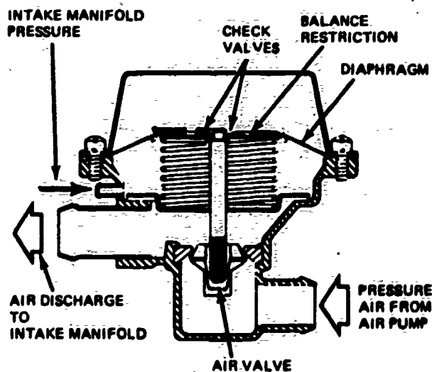
ANTI BACK-FIRE VALVE AIR GULP TYPE
