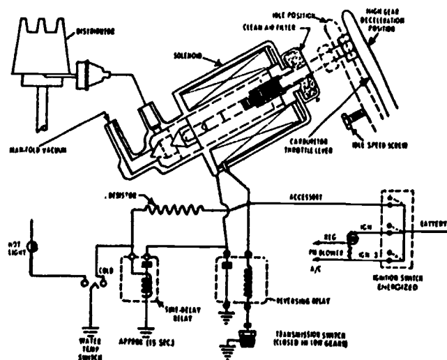
COMBINATION EMISSION CONTROL (C.E.C.) SYSTEM
