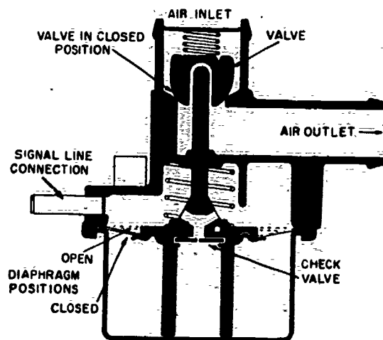
INTAKE AIR BLEED VALVE
