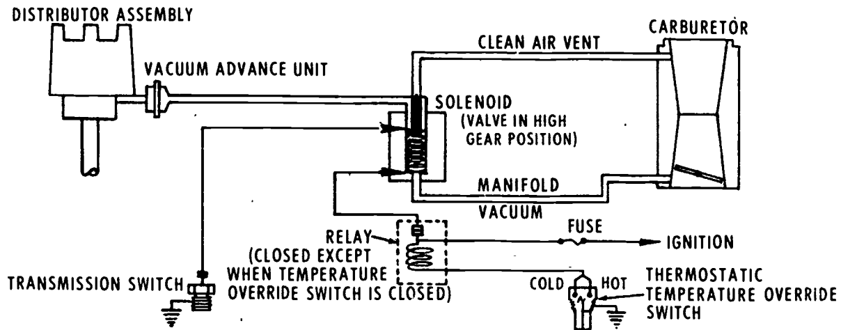
LAYOUT OF TYPICAL TRANSMISSION CONTROL SYSTEM (TEMPERATURE OVERRIDE SWITCH AND RELAY ON CHEVROLET, PONTIAC AND OLDSMOBILE ONLY)
