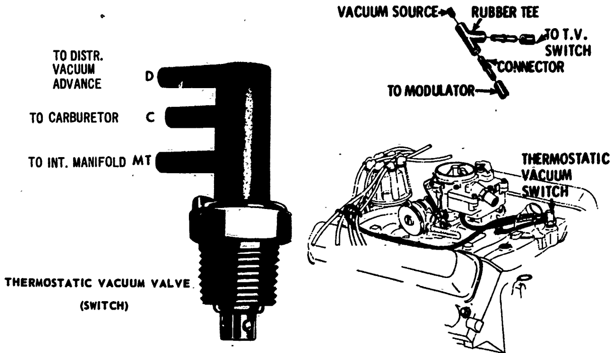
THERMOSTATIC VACUUM VALVE HOSE ROUTING (TYPICAL)
