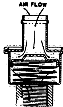
CHECK VALVE OPEN POSITION
