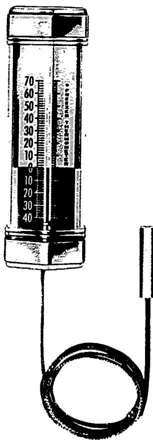
FIGURE 27.—Remote-reading thermometer.
