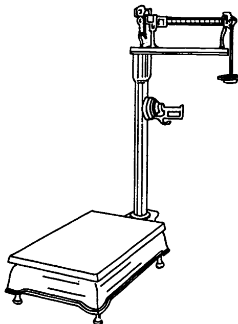
FIGURE 4.—Floor model beam-type scales.
