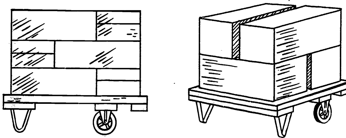
FIGURE 30.—Methods of stacking cased and boxed foods.
