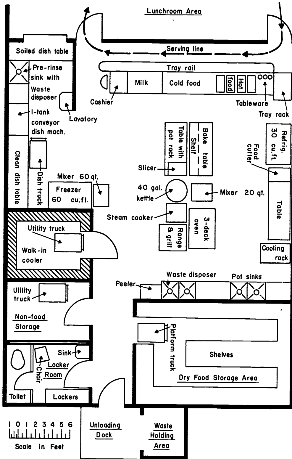
FIGURE 17.—Recommended kitchen layout for a school lunch operation designed to provide 350 to 500 meals a day.
