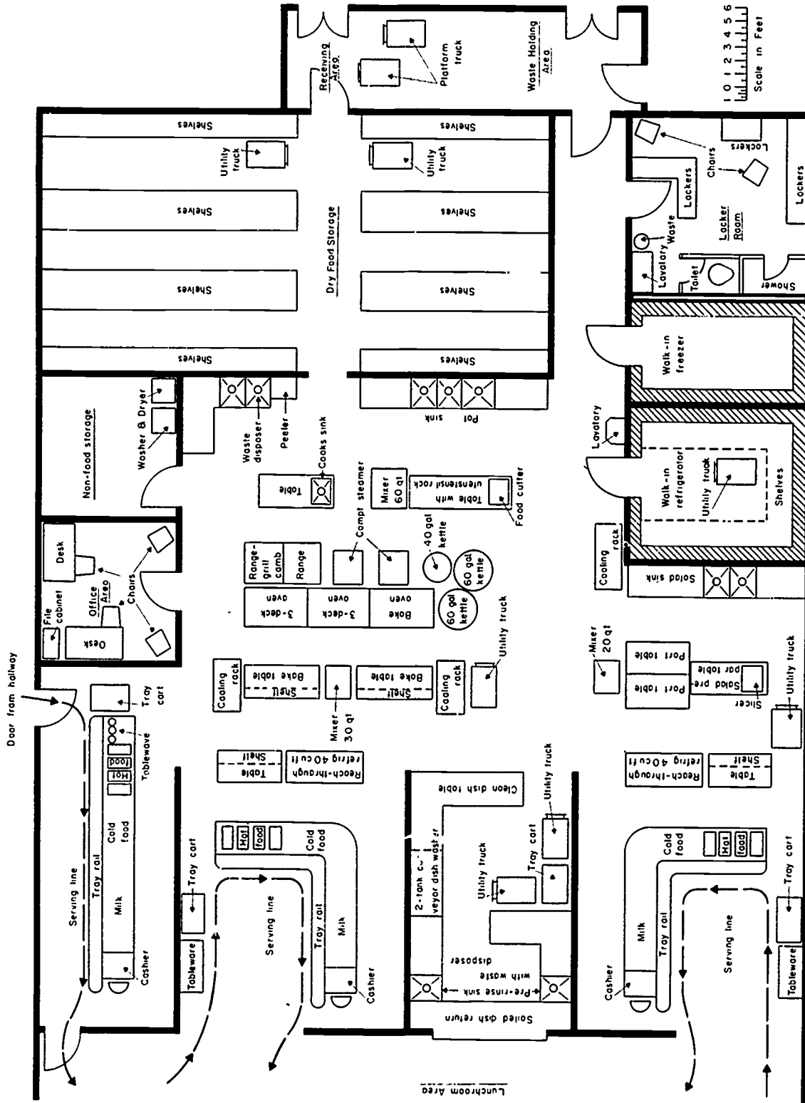
FIGURE 19.—Recommended kitchen layout for a school lunch operation designed to provide 1,400 to 2,000 meals a day.
