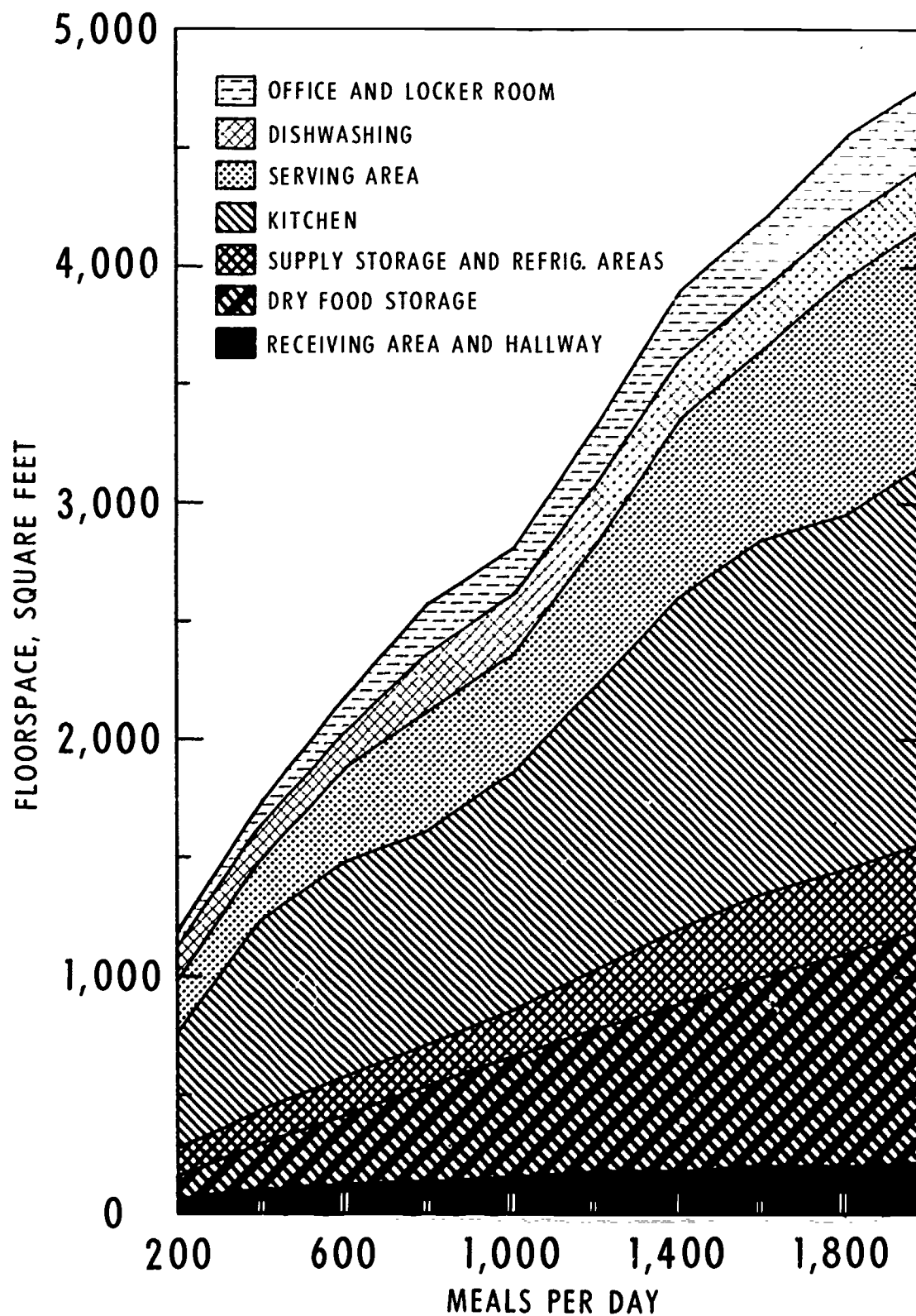
FIGURE 1.—Approximate space requirements for operating areas in various sizes of school lunch facilities.
