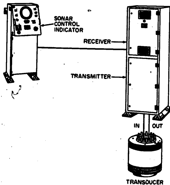
Figure 6-1.—Simplified active sonar system. 71.47
