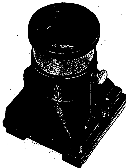
Figure 5-9.— Grid mount assembly and slide viewer.
