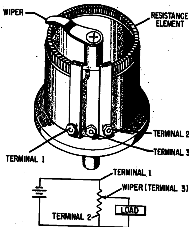
33.75(71) Figure 10-9.— Potentiometer.
