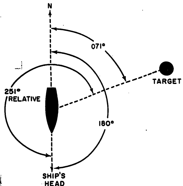
45.29(71)G.2 Figure 3-9.—Target at 071° true.
