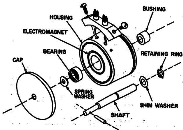
71.59 Figure 7-9.—Magnetic brake—exploded view.
