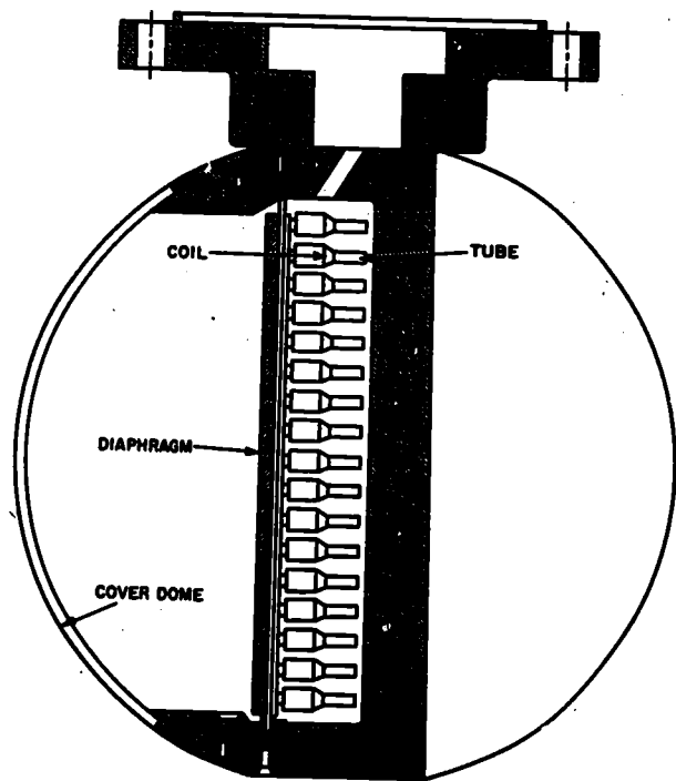
71.48 Figure 6-2.—Searchlight magnetostrictive transducer.
