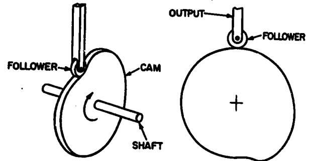
71.105 Figure 7-7.—Flat cam and cam follower.
