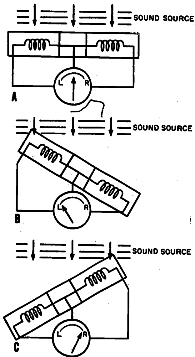
71.54 Figure 6-8.—Operation of the RLI.
