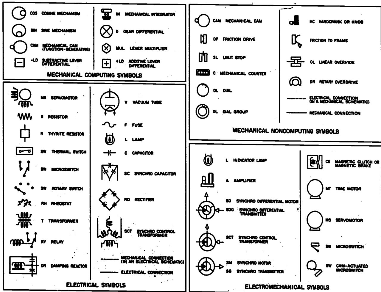
13.5(71) Figure 7-12.— Identifying symbols and their abbreviations.
