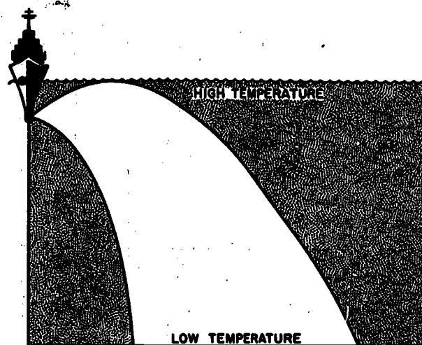
71.27 Figure 4-13.—A refracted sound beam.
