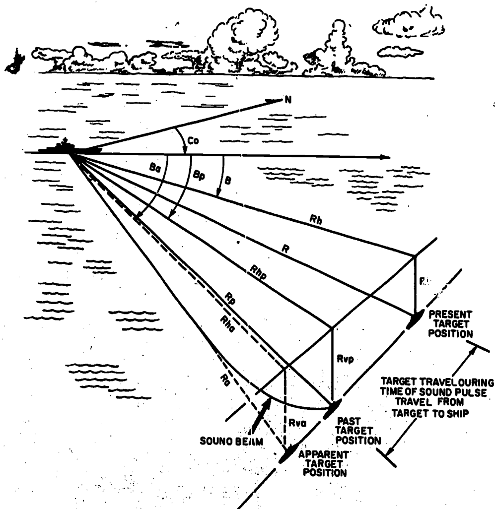
Figure 7-3.—Sonar position quantities.
