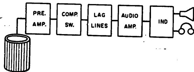
71.55 Figure 6-9.—Block diagram of an array-type passive sonar.
