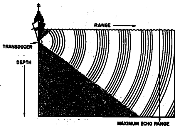
71.26 Figure 4-12.—Sound travel in water of constant temperature.
