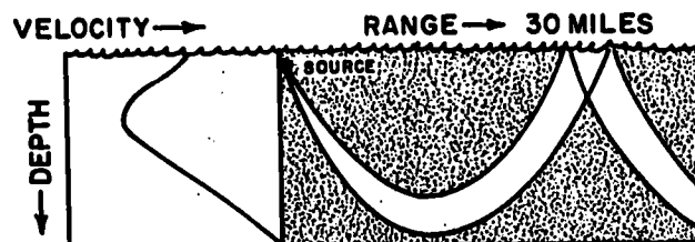
51.8 Figure 4-22.—Convergence zone.
