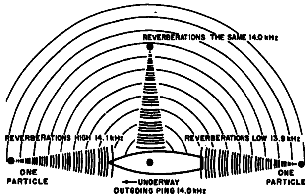
71.39 Figure 4-25.— Illustration of doppler.
