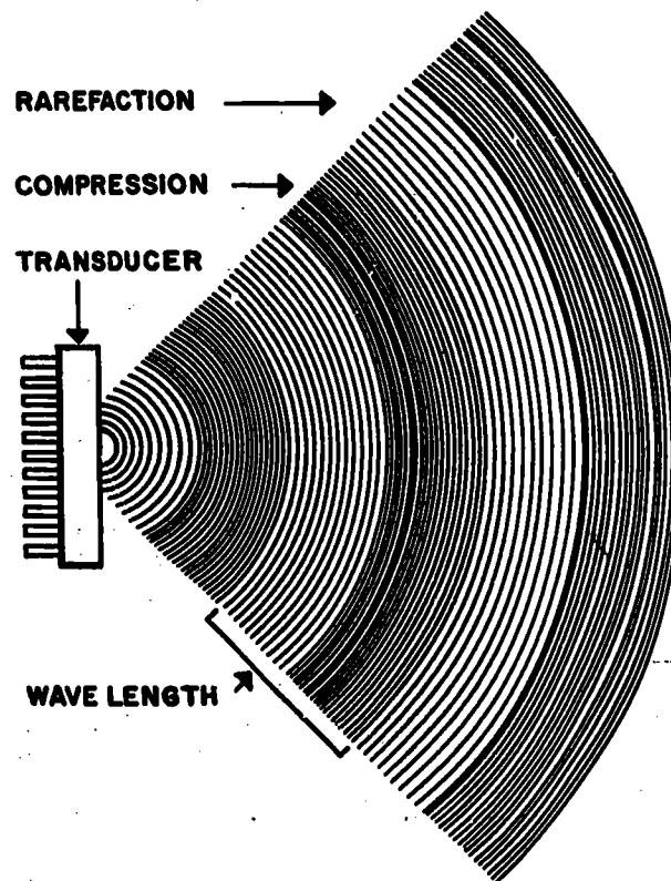
Figure 4-4.—Longitudinal waves.
