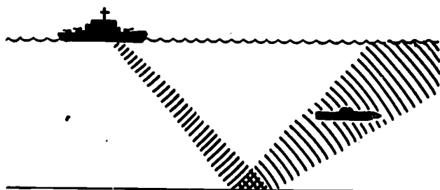
51.7 Figure 4-23.—Bottom bounce effect.
