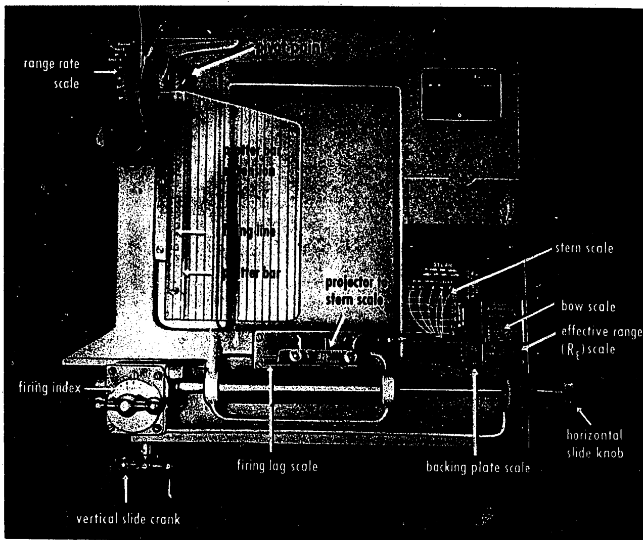
Figure 7-16.— Tactical range recorder.
