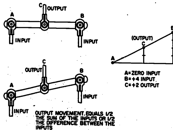
Figure 7-5.—Lever differential.
