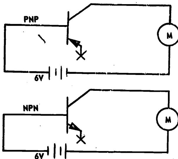
71.99 Figure 10-22.—Transistor leakage current test.
