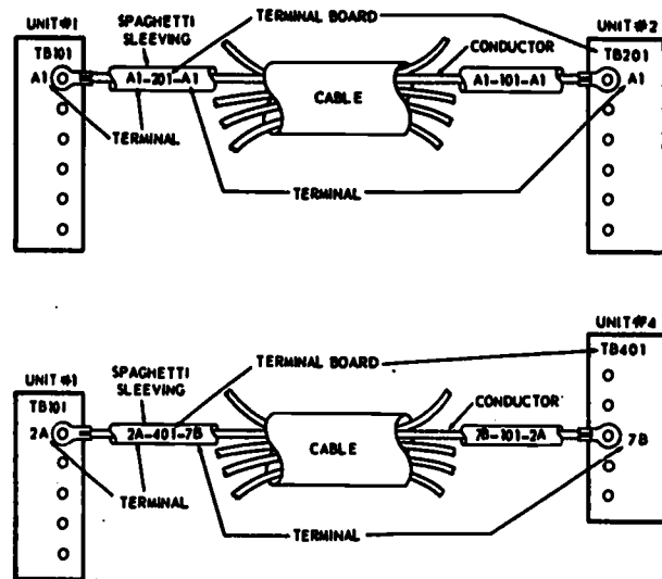
Figure 10-6.—Conductor and terminal markings.
