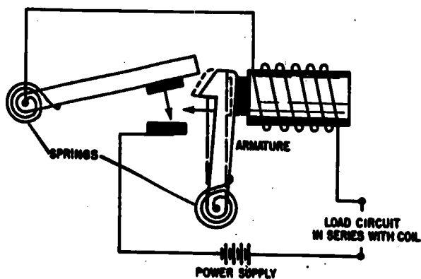
71.97 Figure 10-12.—Magnetic circuit breaker.
