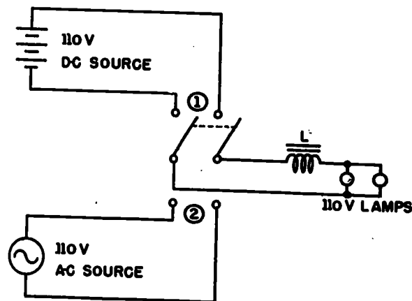
71.95 Figure 10-10.— Inductance in a-c and d-c circuits.
