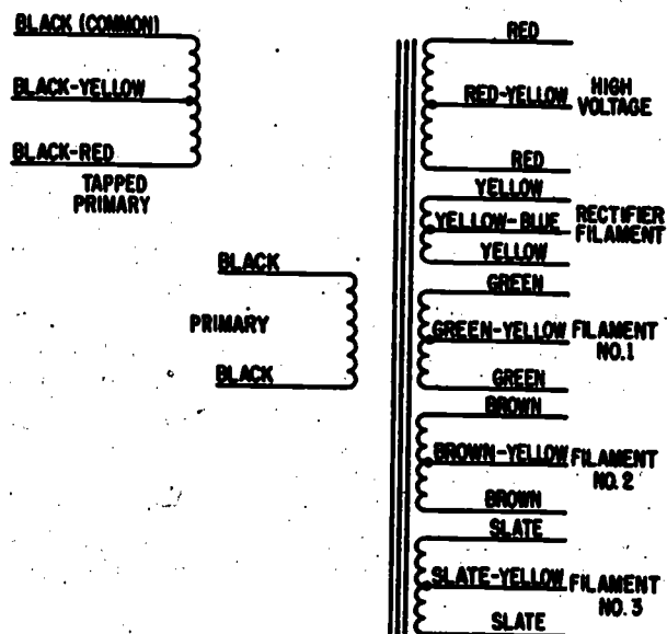
20.379(71) Figure 10-13.—Color coding of small power transformer leads.
