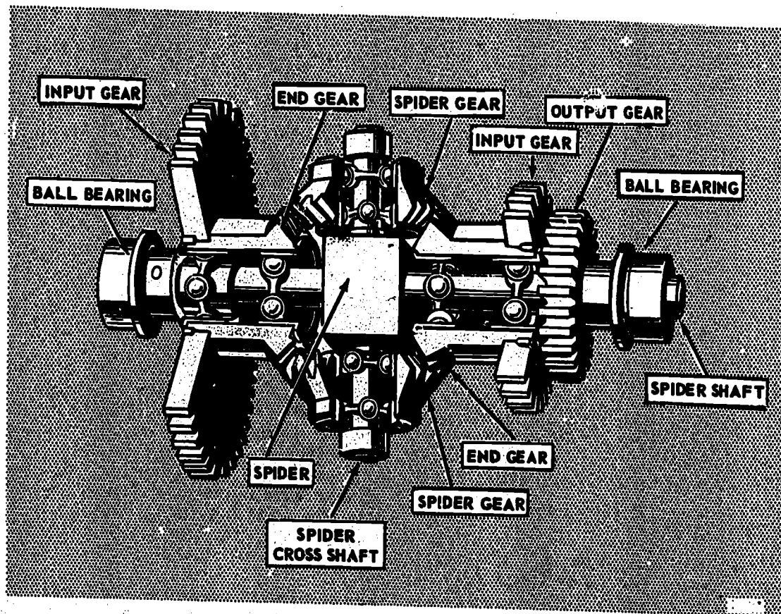
12.87 Figure 7-4. — Bevel gear differential.
