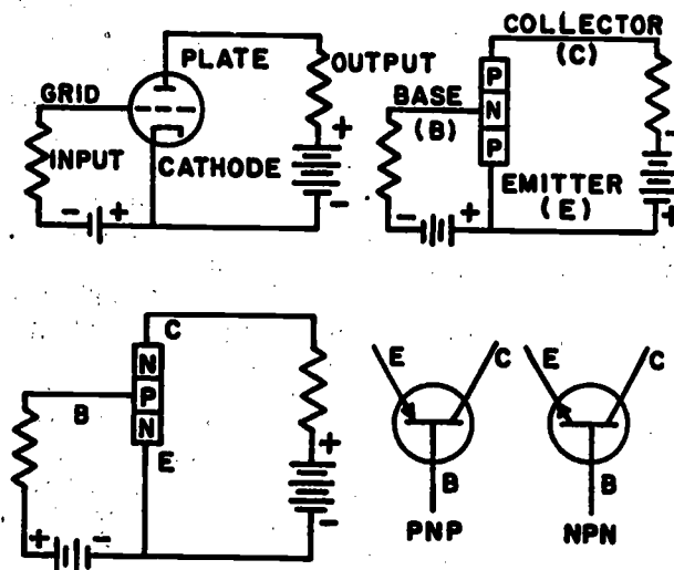
Figure 10-21.— Corresponding elements in triode and transistor.
