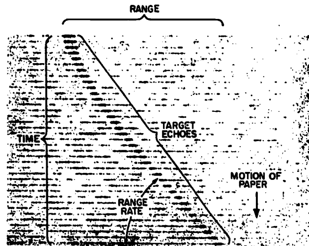
71.64 Figure 7-17.—TRR target traces.
