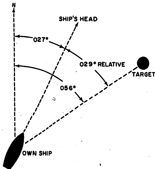
45.29(71)F.2 Figure 3-8.—Target at 056° true.
