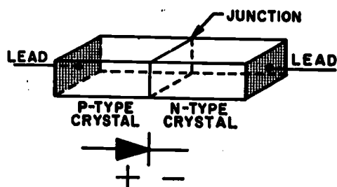
Figure 10-20.— Junction diode.
