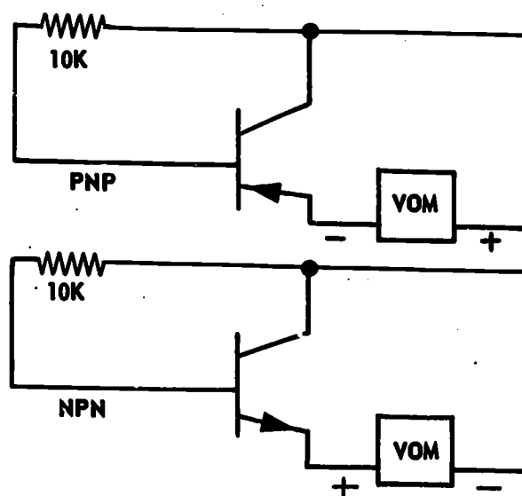
Figure 10-23.—Transistor gain test.
