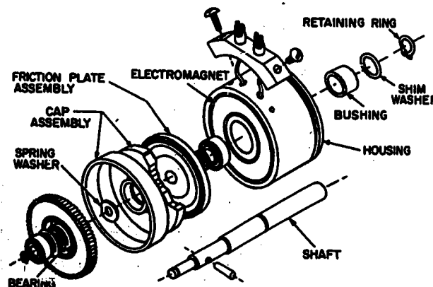
71.60 Figure 7-10.—Magnetic clutch—exploded view.
