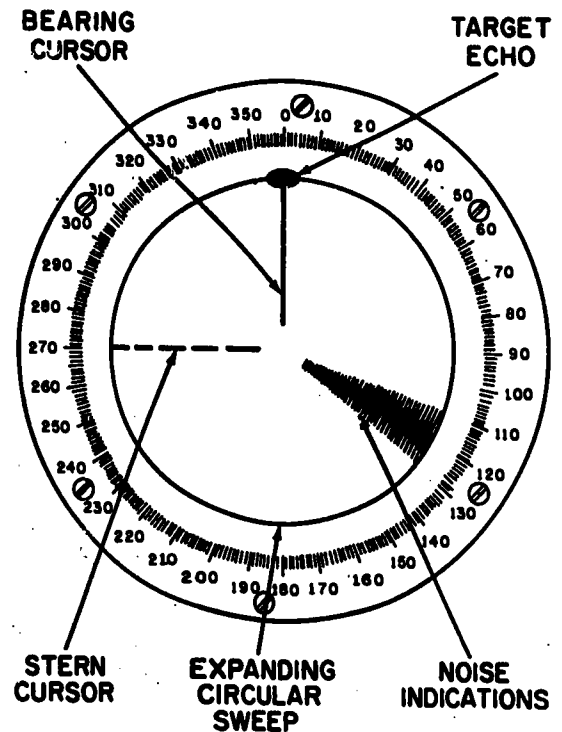
45.29(71)J Figure 3-6.— Stern line indicator.
