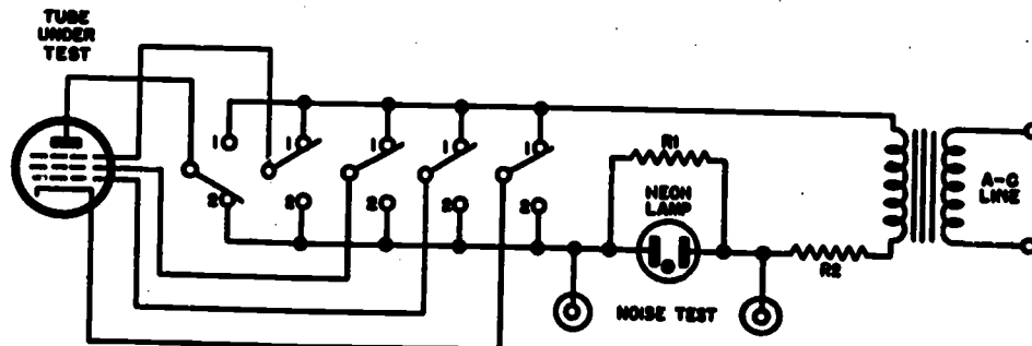
Figure 10-19.—Basic circuit used for short circuit and noise tests. 1.75
