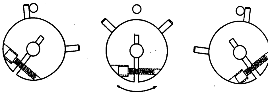
71.106 Figure 7-8.—Mechanical stop.
