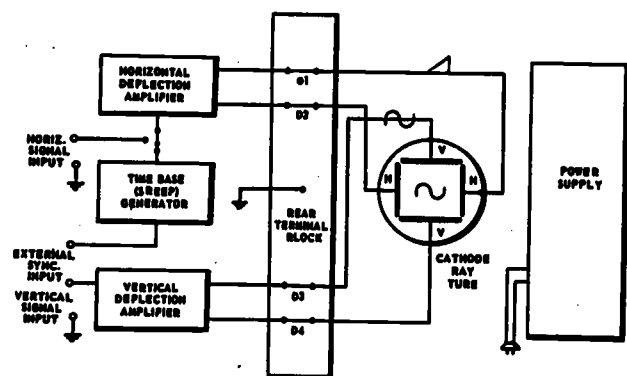
20,324 Figure 10-4.—Block diagram of a CRT oscilloscope.
