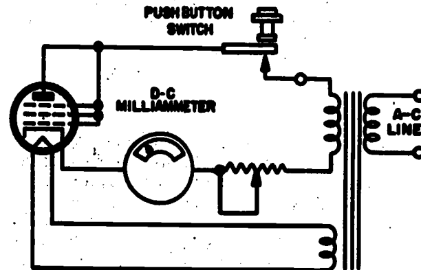
Figure 10-17.—Basic circuit used for emission test.
