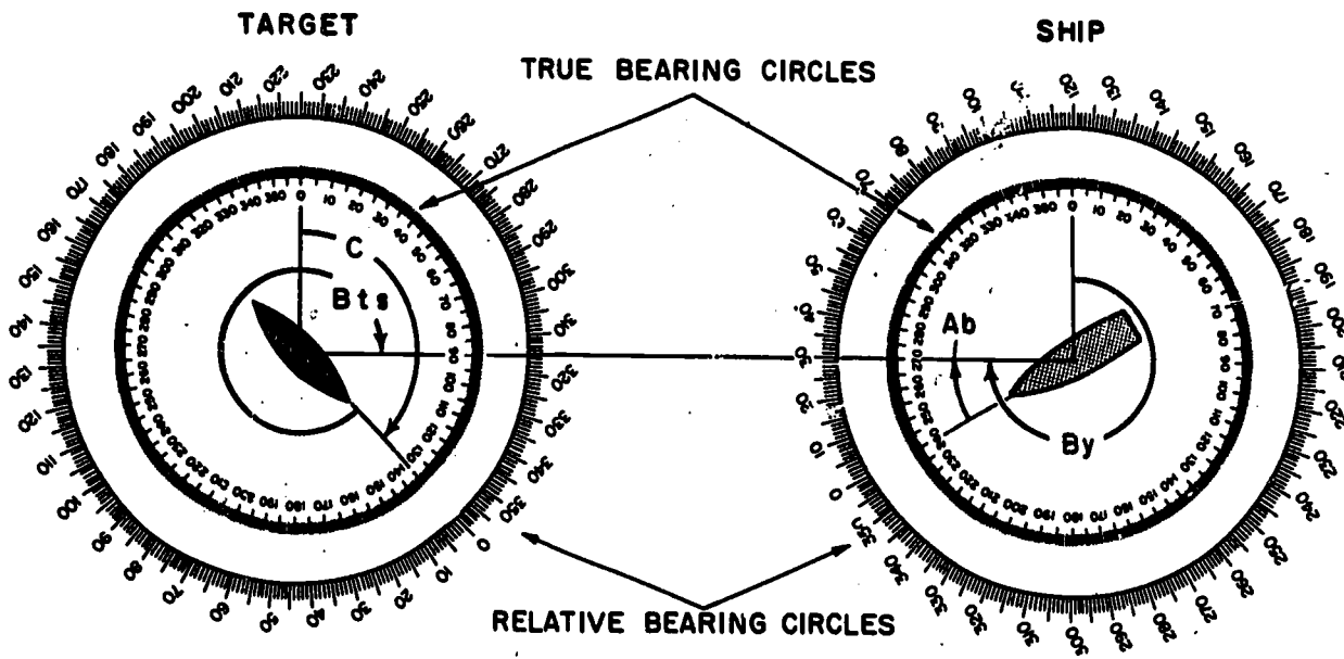
Figure 3-15.—Computing target angle.
