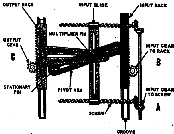
12.91 Figure 7-6.—Screw multiplier.
