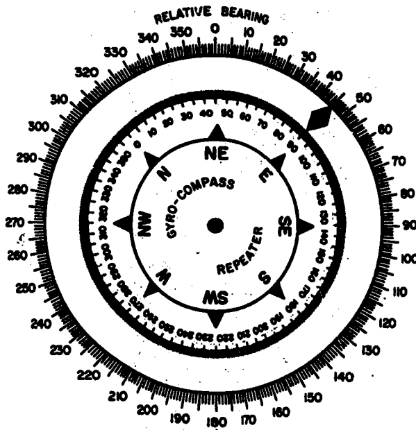
45.29(71)K Figure 3-5.— Bearing and course indicator.
