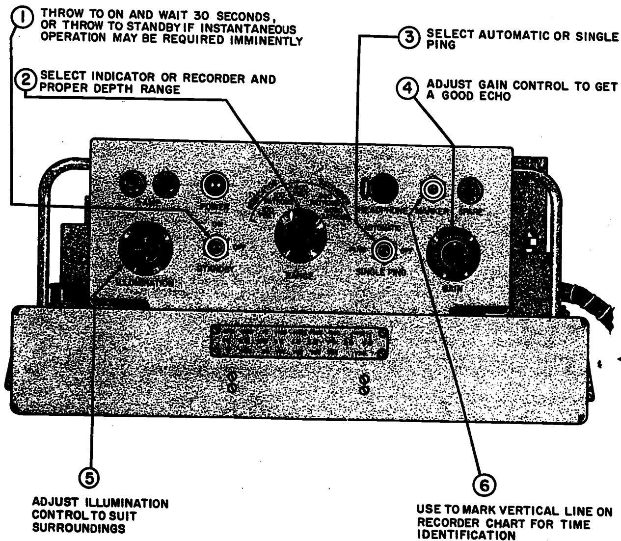
71.58 Figure 6-15.—Fathometer control panel.
