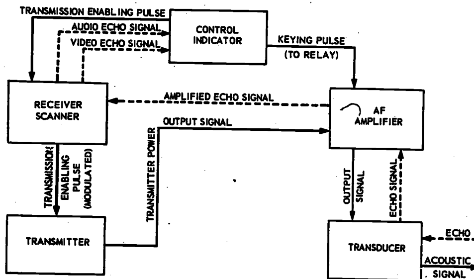
71.51 Figure 6-5.—Sonar system—block diagram.
