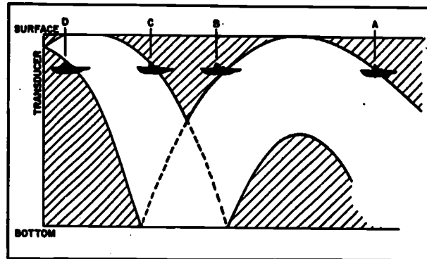
71.28 Figure 4-20.—Shallow water effect on transmitted sound.
