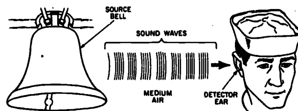
71.18 Figure 4-1.—The three elements of sound.
