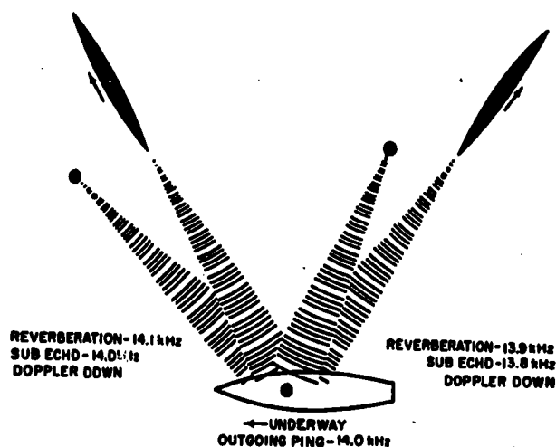
Figure 4-28.—Doppler down.
