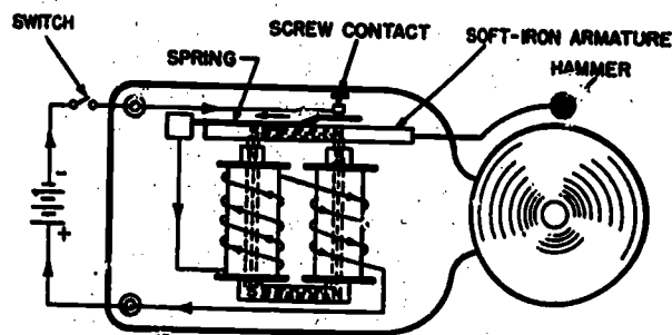
71.96 Figure 10-11.— Electric bell.
