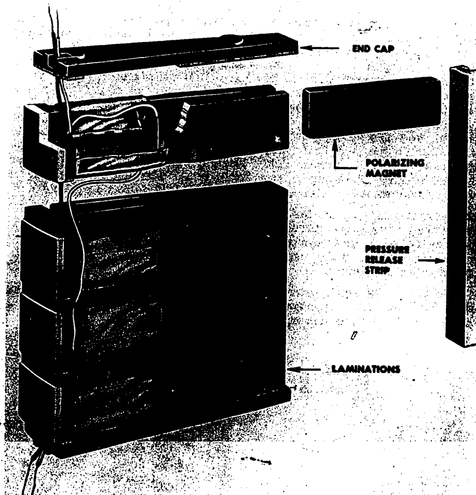
71.50 Figure 6-4.— Exploded view of one scanning sonar transducer stave.
