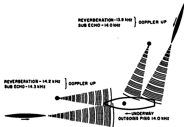
71.41 Figure 4-27.— Doppler up.
