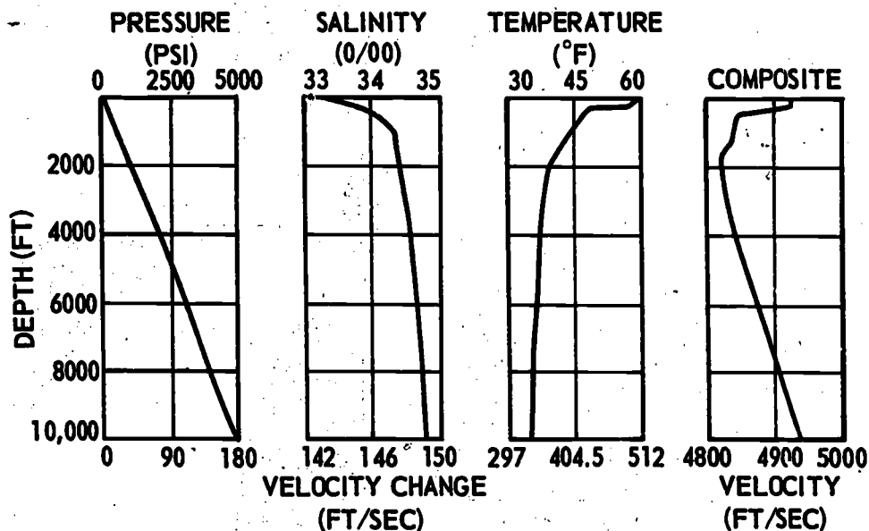
35.5(71) Figure 4-14.—Normal curves for pressure, salinity, and temperature.
