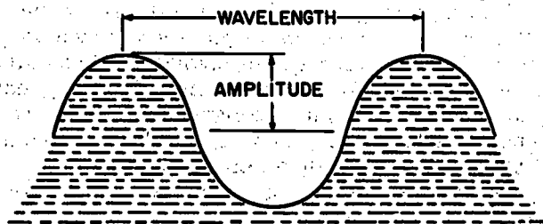
Figure 4-3.—Elements of a wave.
