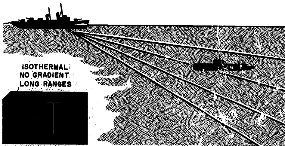
Figure 5-15. — Sound pulse travel through isothermal water conditions.
