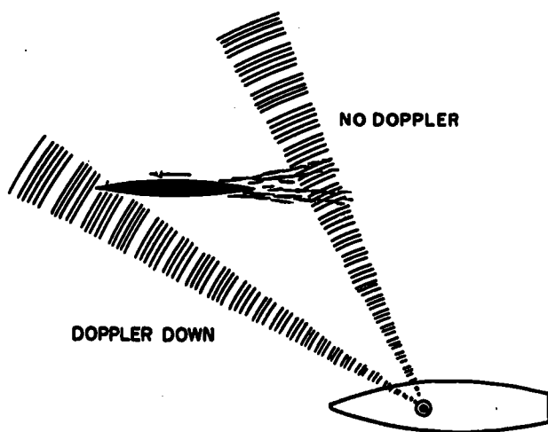
71.44 Figure 4-30.— Value of doppler.
