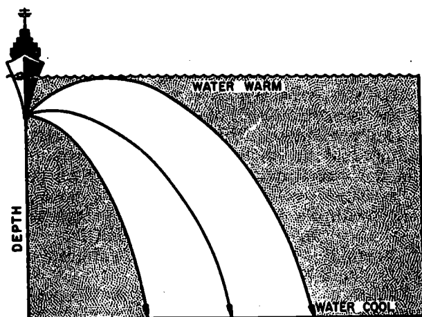
71.31 Figure 4-17.—Negative thermal gradient tends to bend sound downward.
