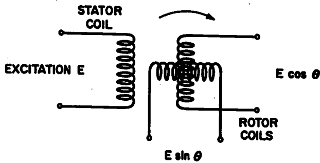
12.105(71) Figure 7-11.— Electrical resolver—schematic symbol.
