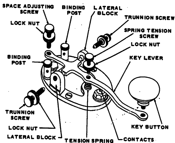
Figure 8-1.—Hand key.
