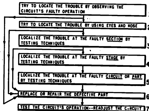
12,259(71) Figure 10-5.—Troubleshooting procedure.
