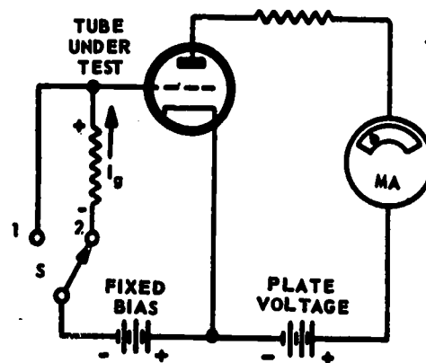
1.76 Figure 10-18.—Basic circuit used for gas test.
