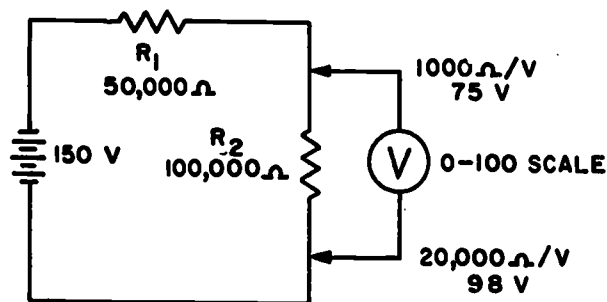
Figure 10-3.—Effect of sensitivity on meter accuracy. 71.125
