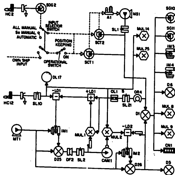
71.61 Figure 7-13.—Use of symbols in a sectional diagram.
