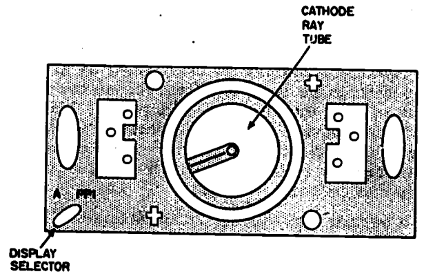
35.10 Figure 6-11.—Azimuth indicator of an array-type passive sonar.
