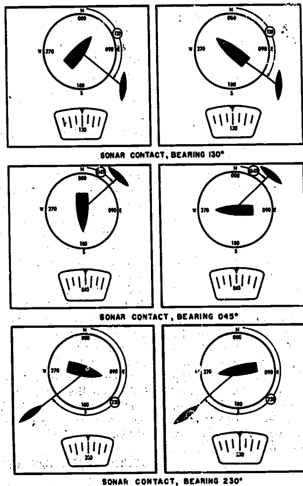
71.3 Figure 3-1.— True bearings are independent of ship's head.
