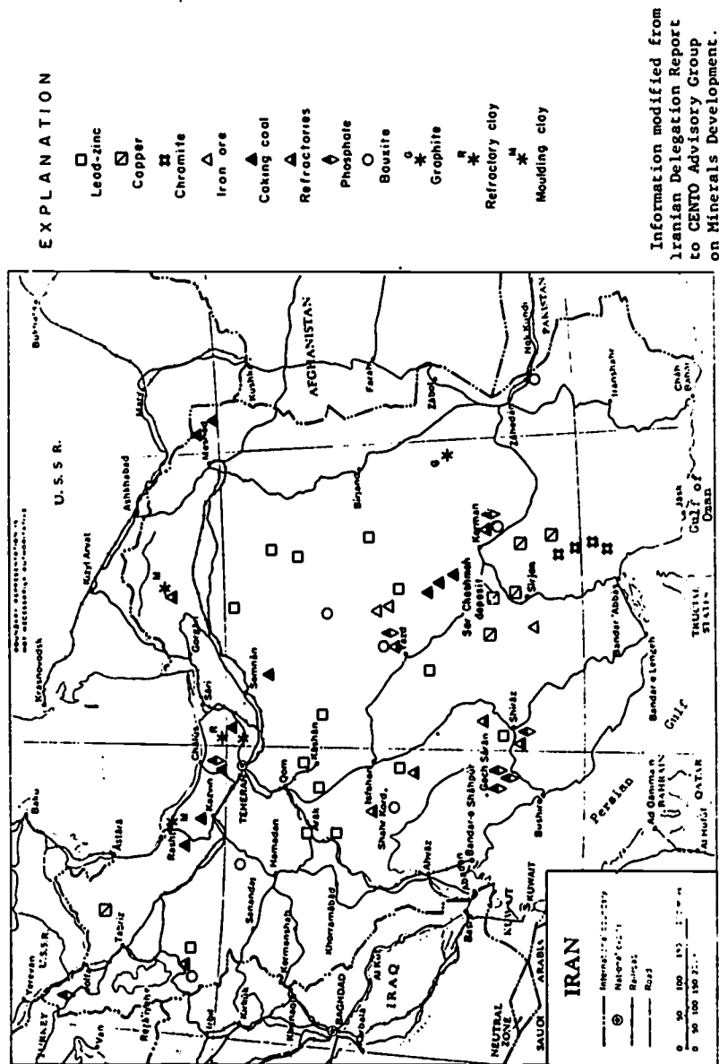
FIGURE 1. Significant mineral localities in Iran.
