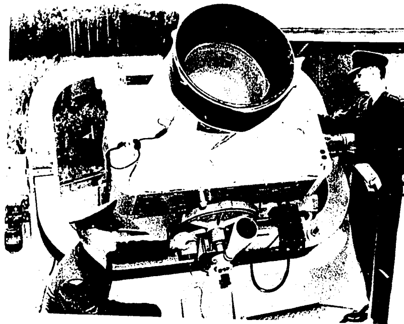
Figure 21. Baker-Nunn Camera.
