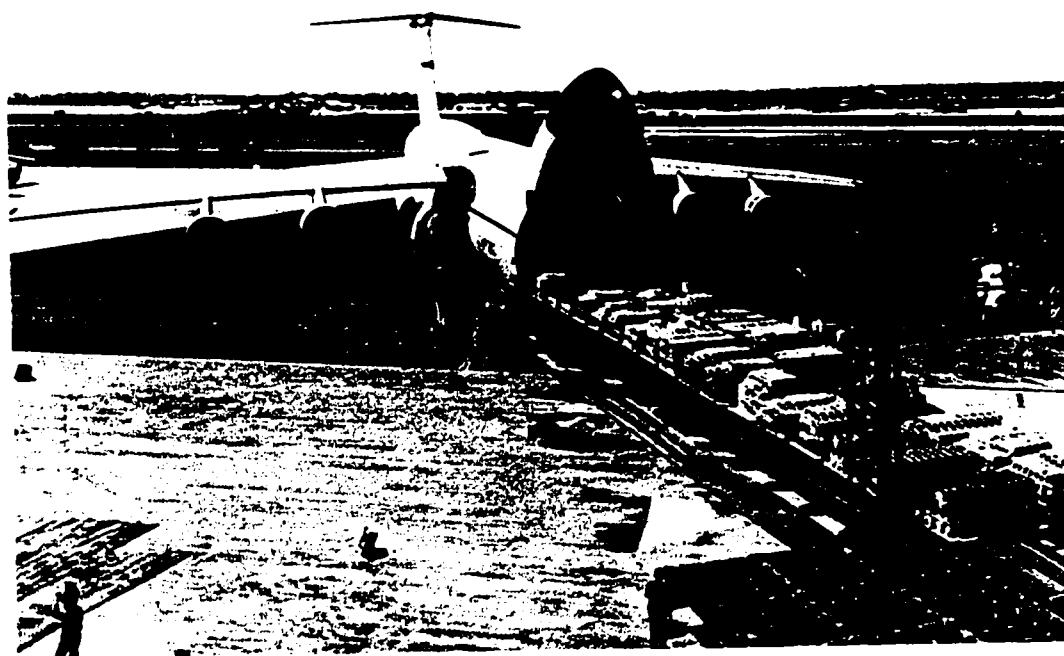
FIGURE 10. GALAXY loading through nose from air-transportable deck, which can be flown into a newly-established airbase in sections in C-5s and quickly assembled to speed loading and unloading of other C-5s arriving the next day.
