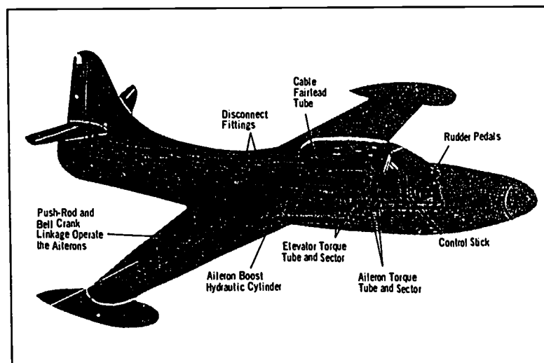
Figure 21. CONTROL LINKAGES—diagram of a typical system.
