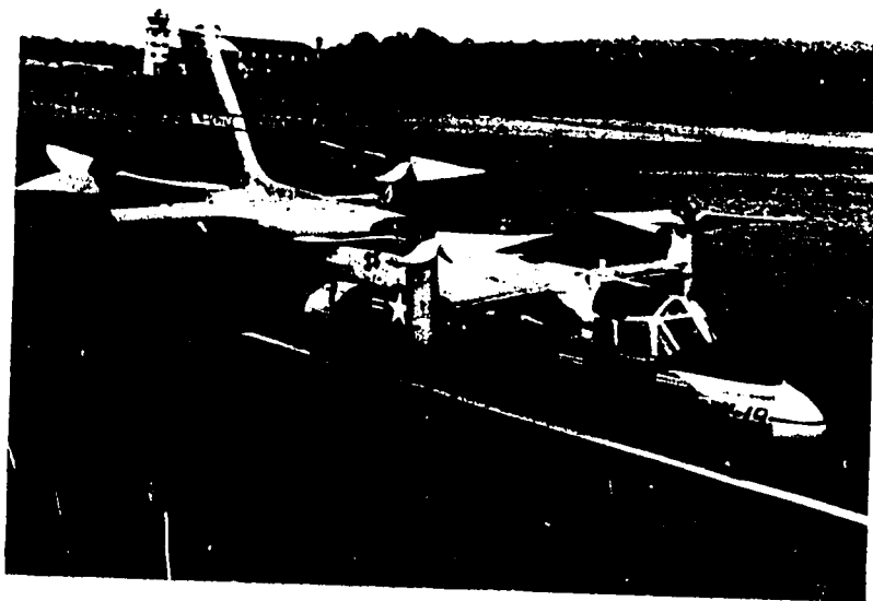
Figure 81. TILTING PROPELLER PODS were features of the X-19, shown here ready for vertical takeoff. Note the width of the propeller blades.
