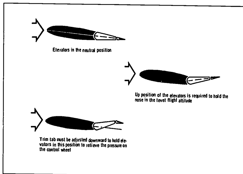
Figure 17. A TRIM TAB, and how it works.
