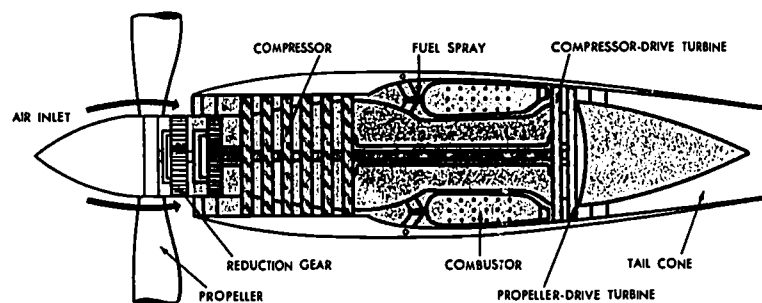
Figure 30. TURBOPROP. This diagram shows turboprop unit with air intake surrounding propeller hub. Compare with Figure 31.
