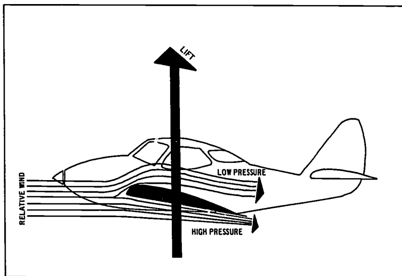
Figure 13. LIFT, according to Bernoulli's Law.
