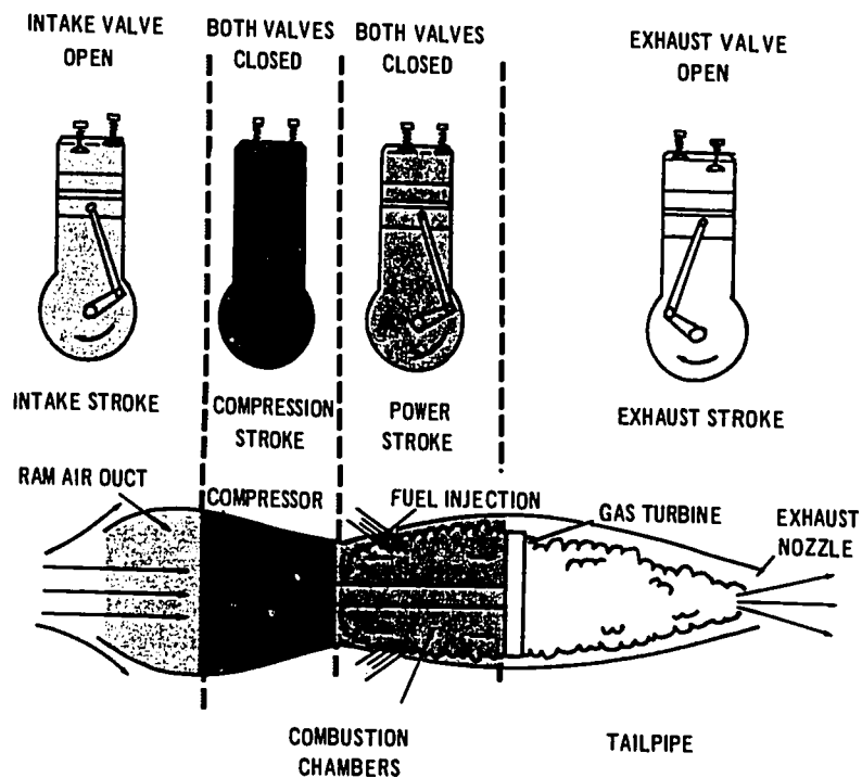
Figure 24. COMPARISON of a reciprocating and a jet engine.
