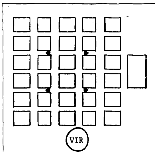
Figure 32. In this arrangement, four microphones are suspended from the ceiling in the approximate positions shown. The front two are directed toward the teacher with the back two toward the class.
