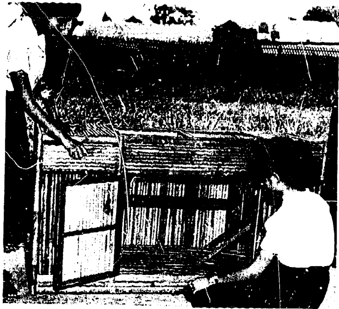
Attractive cupboards can be made of bamboo where it is plentiful. These Thailand workers show drawer, shelf, and sink space in a kitchen unit.
