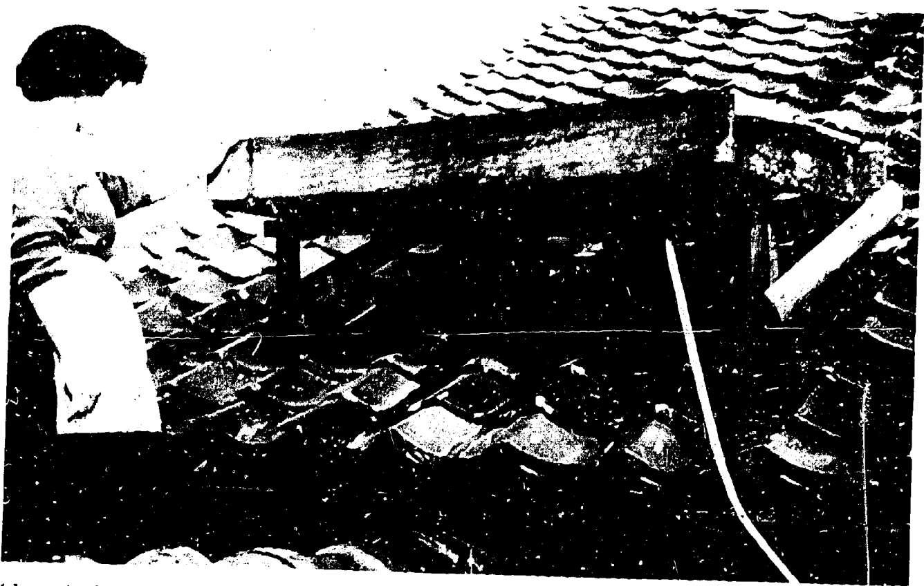
Solar water heaters in Japan catch rainwater from the roof and hold it for the sun to heat. It is then piped into the home.
