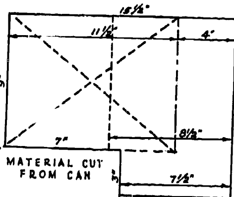
Strip behind door - 1 side of one door
