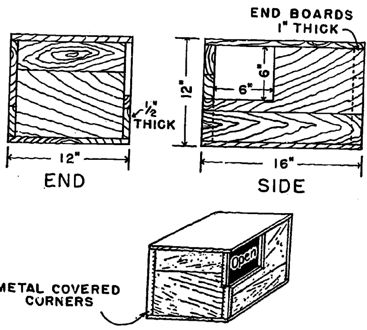
Construction details for a wooden nest box.
