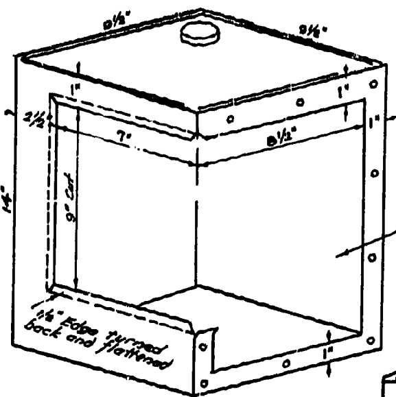
CUTTING DIAGRAM - LEFT CAN RIGHT CAN REVERSED
