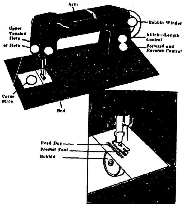
The parts of a sewing machine.
