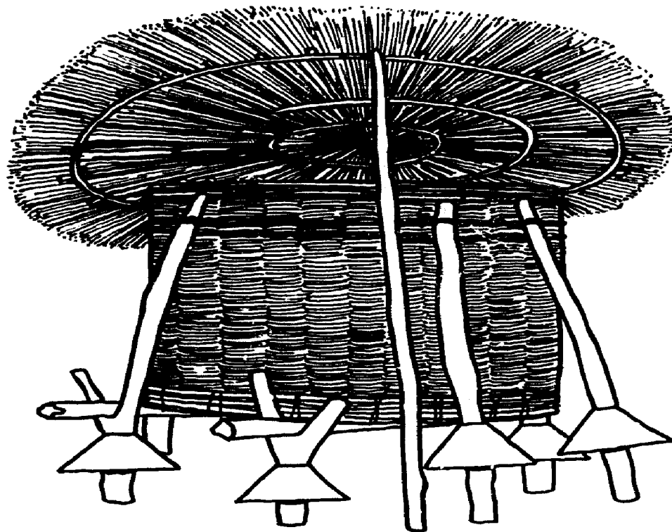
Raising grain storage off the ground and using a cover to protect it from rain helps save grain. Metal shields on the legs protect this storage against rodents.
