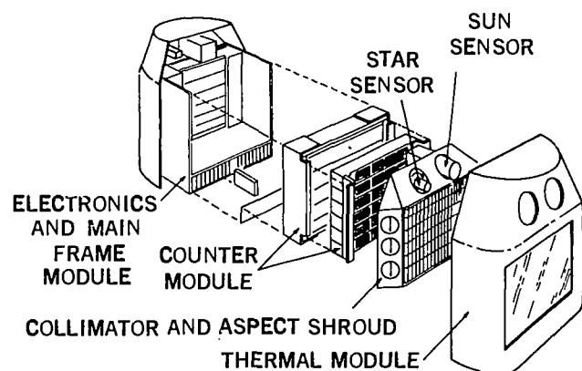
Figure 14. Exploded view of the X-ray detectors mounted in the top of the SAS. Each detector has a different collimator to provide two levels of resolution as the spacecraft spins.
