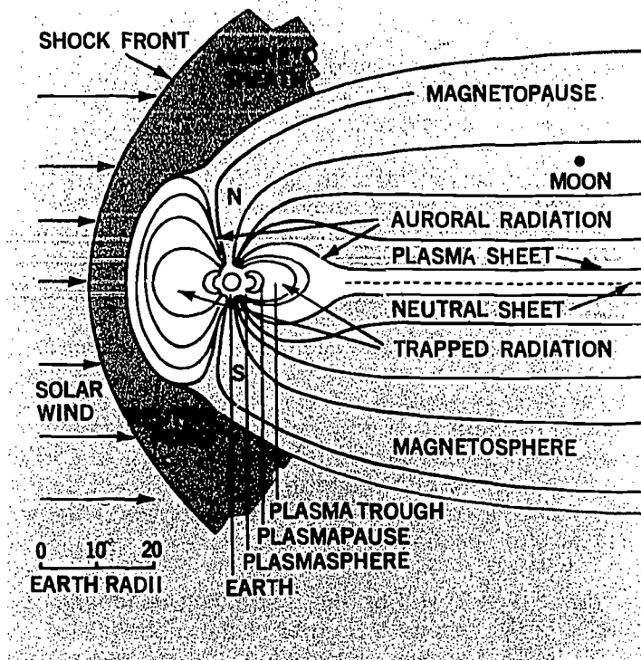
Figure 2. A detailed view of the Earth's magnetosphere and the shock front created when the solar wind hits it.
