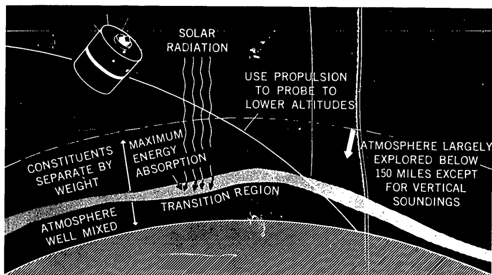
Figure 7. The mission of the Atmosphere Explorer takes it deep into the Earth's transition region.
